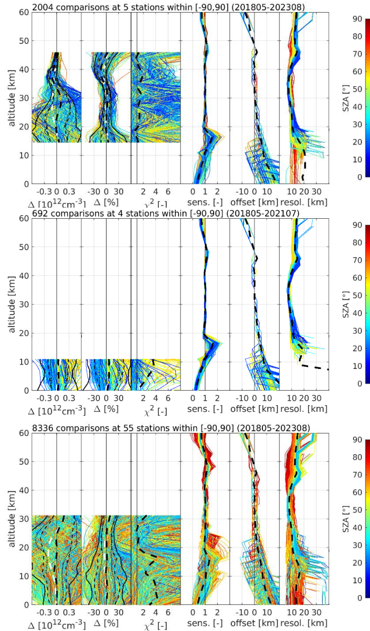
Figure 29: Comparison between S5P L2_O3_PR RPRO/OFFL ozone number density profile data and all co-located ground-based reference measurements, originating from stratospheric lidars (top), tropospheric lidars (middle), and ozonesondes (bottom). Every plate shows six graphs, respectively, from left to right: the difference and the percent relative difference between S5P and ozonesonde (left panels) or lidar (right panels) data, the chi-square profile, the vertical sensitivity, the altitude registration offset, and the averaging kernel FWHM associated with the S5P retrieval. The colour scale indicates the TROPOMI solar zenith angle. Black dashed lines show mean values (thick lines) and standard deviations (thin lines, around the mean), while white dashed lines indicate the mean difference between the a-priori profile and the reference measurement. Dotted black lines indicate the total ex-ante (inductive) uncertainty of TROPOMI and the reference measurements combined (around the mean difference).
