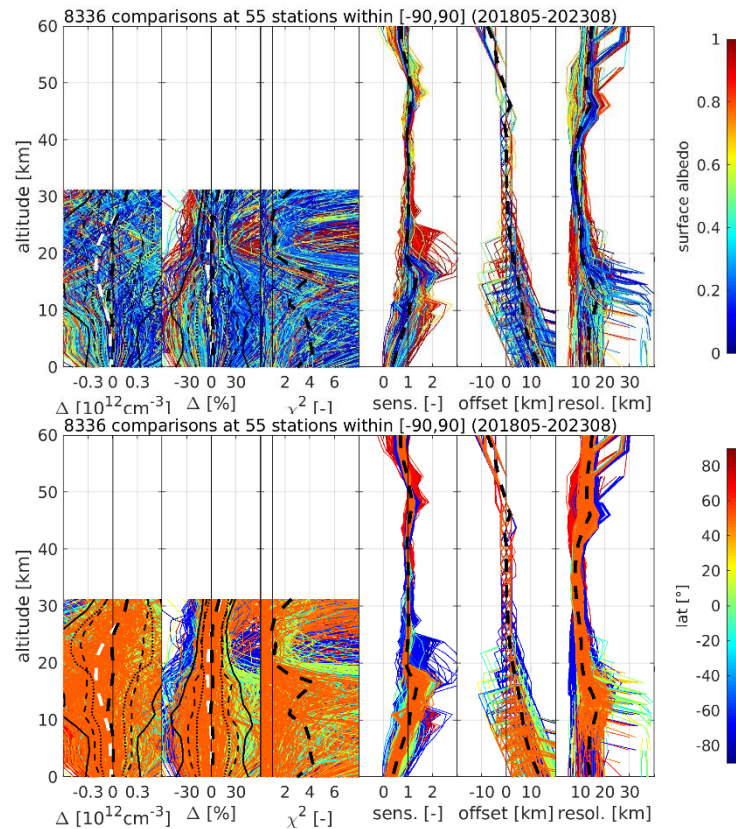
Figure 30: Comparison between S5P RPRO/OFFL ozone number density profiles and co-located ozonesonde data (L2 v2.4.0, May 2018 to August 2023). Every plate shows six graphs, respectively, from left to right: the difference and the percent relative difference between S5P and ozonesonde data, the chi-square profile, the vertical sensitivity, the altitude registration offset, and the averaging kernel FWHM associated with the S5P retrieval. The colour scale indicates the latitude (right) and surface albedo (left). Black dashed lines show mean values (thick lines) and standard deviations (thin lines, around the mean), while grey dashed lines indicate the mean difference between the a-priori profile and the reference measurement. Dotted black lines indicate the total ex-ante (inductive) uncertainty of TROPOMI and the reference measurements combined (around the mean difference).
