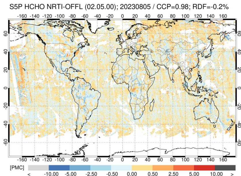
Figure 66: Difference between S5P V02.05.00 NRTI and OFFL HCHO column data for 2023/08/05 (binned to 0.5^\circ \times 0.5^\circ resolution). The difference is only calculated for columns above 0.5 Pmolec/cm 2 and a q_a\_value above 0.5. PMC stands for Pmolec/cm 2 .
