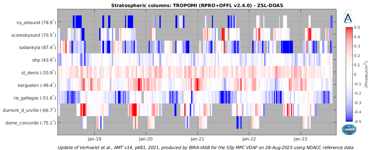
Figure 41: Time series – from August 2018 until August 2023 – of S5P RPRO+OFFL L2_NO 2 and NDACC ZSL-DOAS NO 2 stratospheric column differences, weekly averaged [Pmole/cm 2 ]. For the current report, only the SAOZ data sets covering the full mission lifetime are shown.
