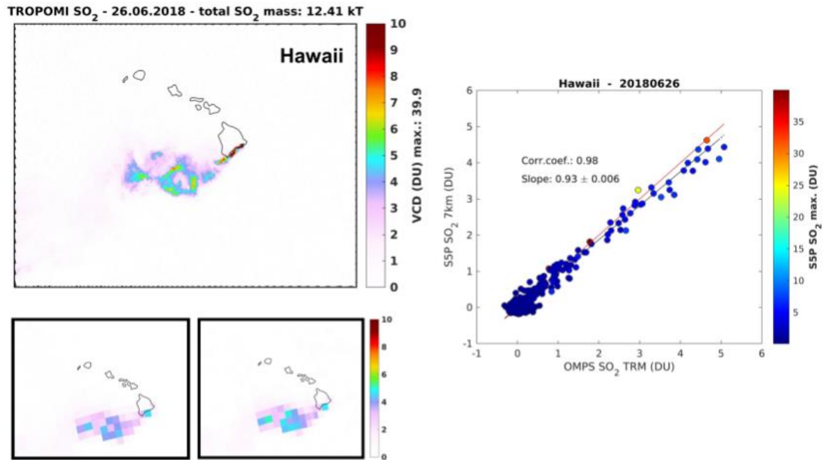
Figure 68: Comparison of TROPOMI and OMPS measurements of the volcanic plume of Kilauea on 26 June 2018. The large figure shows the original TROPOMI data. The two small figures show the spatially degraded TROPOMI data and the OMPS data. The figure right shows the correlation plot of the degraded TROPOMI data versus the collocated OMPS data. Courtesy of C. Li and N. Krotkov, NASA/GSFC.
