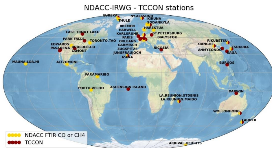
Figure 77: Geographical distribution of NDACC and TCCON FTIR stations measuring atmospheric carbon monoxide column data. Some stations contribute to the two networks.
