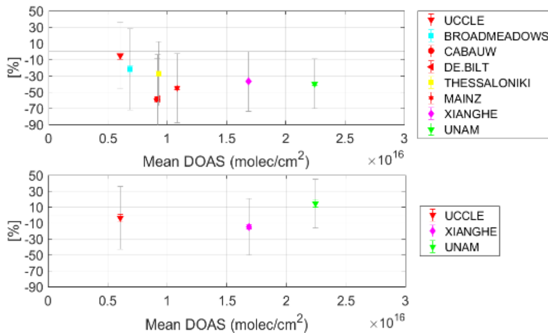
Figure 56: Bias at each station (in %) as a function of the mean DOAS total columns ( 10^{16} molec/cm 2 ). The grey bars are the systematic uncertainty on the differences, and the coloured error bars are the 2- \sigma error on the bias. Top panel: DOAS is the normal product without any modification. Bottom panel: DOAS data after Rodgers and Connor (2003) is applied (a priori substitution and smoothing with the TROPOMI averaging kernels).
