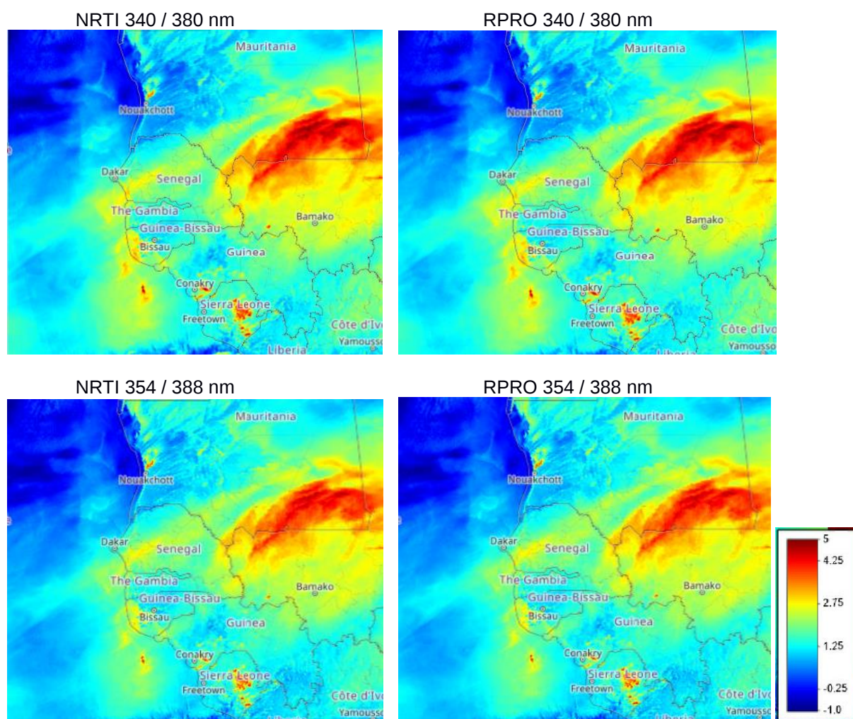
Figure 110: Comparison of the S5P TROPOMI near real time and reprocessed UVAI for a selected area on October 4, 2022 for the two wavelength pairs (top: 340 / 380 nm, bottom: 354 / 388 nm).
