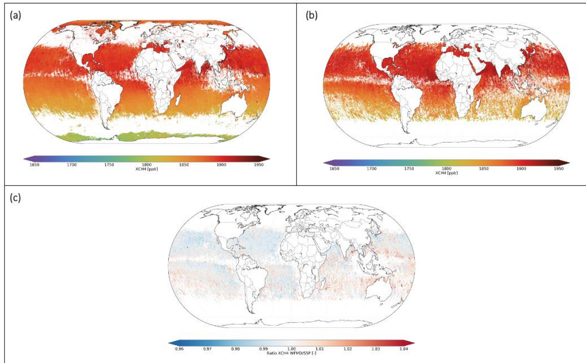
Figure 82: Global distribution of XCH 4 measured by TROPOMI retrieved with (a) WFMD-DOAS retrieval algorithm, (b) the pre-operational retrieval algorithm and (c) the ratio of both. Daily collocations are averaged to a 0.1 x 0.1-degree grid for the year 2022.
