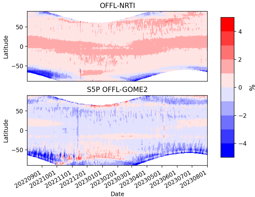
Figure 18: Time series of the differences between the different gridded (level-3) total ozone column data sets. Upper panel: S5P OFFL versus S5P NRTI (both v2.4.1 and above). Lower panel: S5P OFFL versus GOME-2 (MetOp-B and MetOp-C, processors GDP 4.8 and 4.9 respectively, but these are identical for the total ozone column product).
