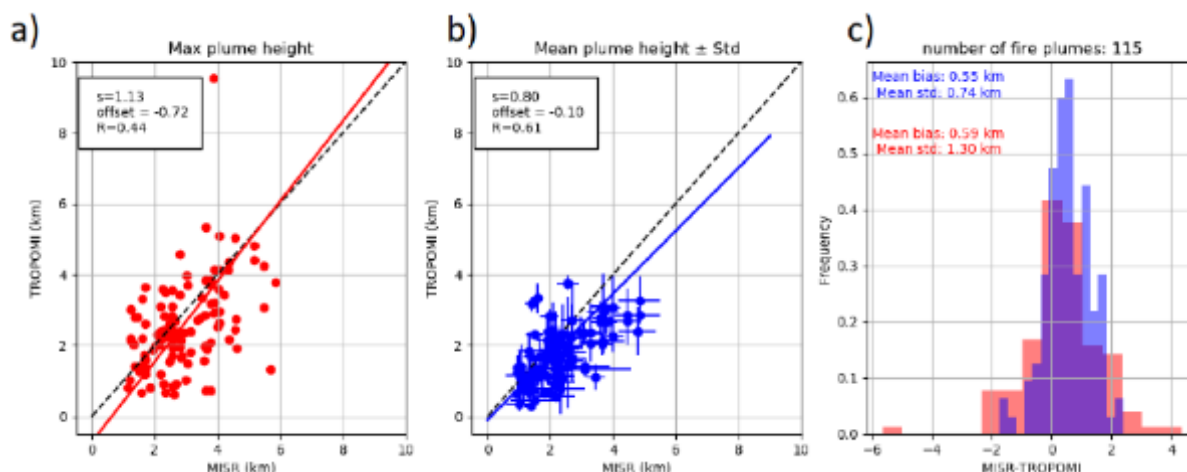
Figure 116: Comparison of TROPOMI ALH (processor version before v02.05.00) and MISR plume height for 115 fires over Northern America in 2018. See Griffin et al, 2019 for details.
