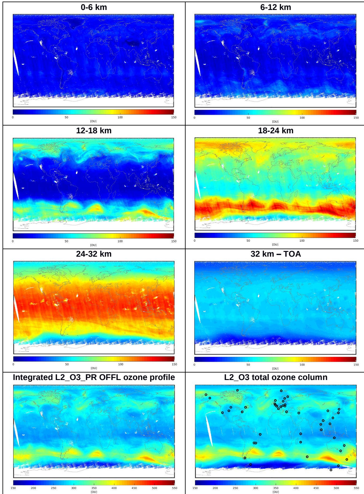
Figure 31: Upper six panels: daily global map for the six partial columns in the S5P L2_O3_PR OFFL v02.05.00 ozone profile product of August 20, 2023, as a function of altitude. The two lower maps show the total ozone column values obtained by integration of the L2_O3_PR profile data (left), and the map of L2_O3 total ozone column values for the same day (right) to check for their mutual consistency.
