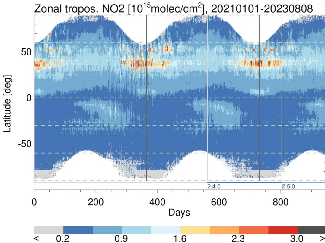
Figure 37: S5P TROPOMI NO 2 tropospheric columns [ 10^{15} molec/cm 2 ] as a function of day and latitude. The period is from January 2021 to August 2023. RPRO/OFFL V02.04.00 and V02.05.00 data is used here. Grid box size in latitude direction is 0.5°. The light grey vertical lines mark processor version changes, the grey lines the beginning of each year.
