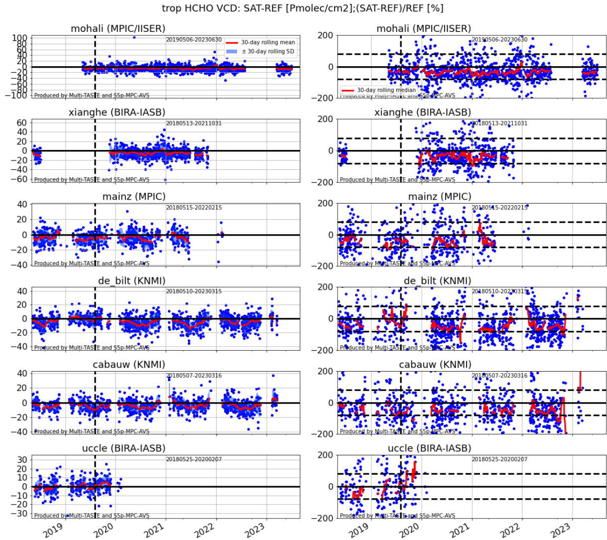
Figure 54: Time series of the difference [Pmolec/cm 2 ] and relative difference [%] between S5P RPRO+OFFL and MAX-DOAS HCHO column data at six stations. Data was obtained from the VDAF Automated Validation Server on 2023/08/25. Dashed line: pixel size switch at 2019/08/06.
