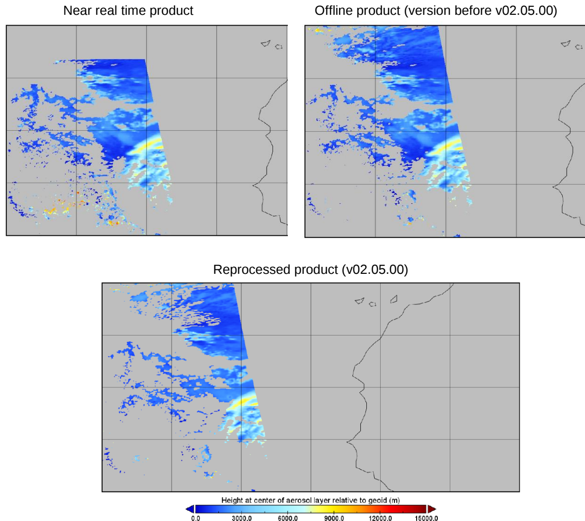
Figure 111: Comparison of different ALH data products for a desert dust event over the Atlantic on 30 August 2021 (orbit 20107). The differences in the number of processed pixels is caused by slightly different selection criteria for the different versions.
