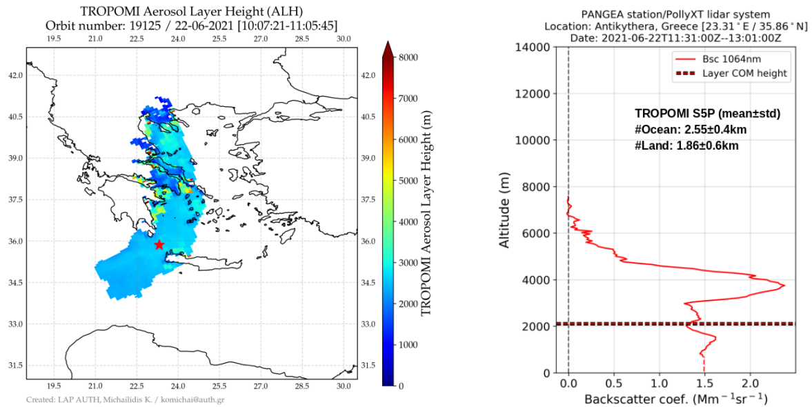
Figure 120: Left: TROPOMI ALH (processor version v02.04.00) retrievals (orbit 19125) over Greece during dust event on 22 June 2021. The red star indicates the position of the Antikythera (PANGAEA) station. Right: Lidar backscatter profile at 1064 nm. The horizontal dashed-dotted red line represents the calculate profile centre of mass. The AER_LH retrievals from TROPOMI are shown in the inbox text.
