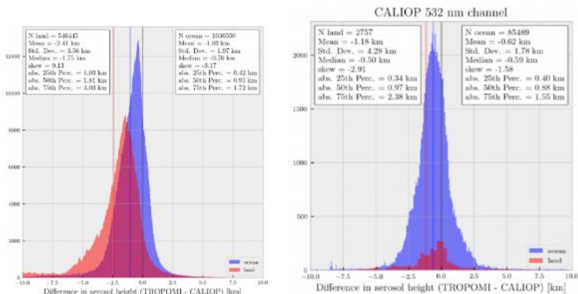
Figure 115: Histogram of differences between CALIOP weighted extinction height and TROPOMI ALH from collocated data between 1 May 2018 and 28 February 2019 (left). The right panel shows the same histogram, but for pixels that were screened for a minimal cost function (chi-squared) smaller than 1E5.
