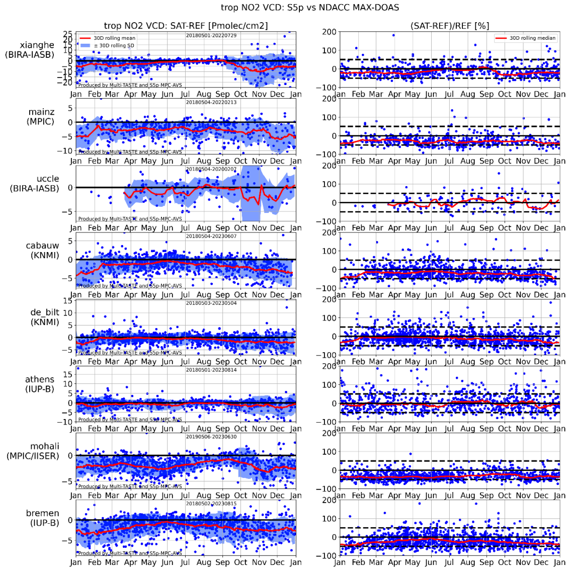
Figure 38: Seasonal cycle (with data mapped to one generic year) of the difference between S5P RPRO+OFFL and MAX-DOAS NO 2 tropospheric column data at 8 stations. Difference (left) and relative difference (right). On the left column, the lowest 2.5% data is not shown for visibility. Data was obtained from the VDAF Automated Validation Server on 2023/08/28.
