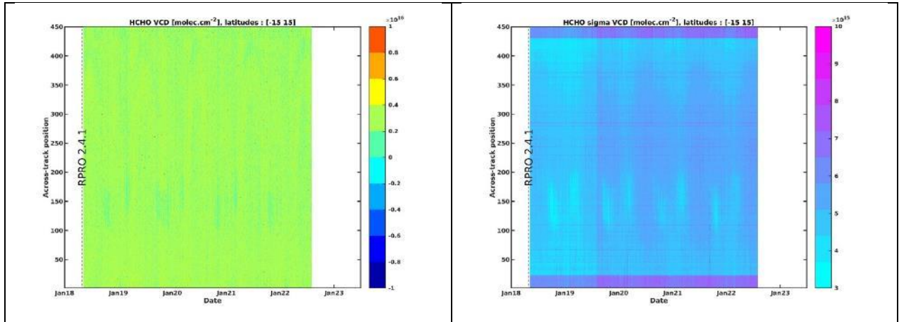
Figure 64: S5P TROPOMI HCHO column data (left) and their standard deviation (right) as a function of day (x-axis) and across-track position (y-axis). Data are averaged in the reference sector (the remote Equatorial Pacific). Results are shown for the reprocessed data collection 3.
