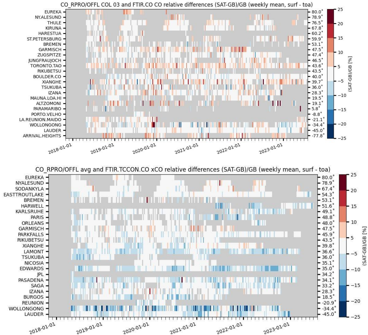
Figure 78: Relative bias between S5P L2_CO OFFL and ground-based CO column data at NDACC (top), TCCON (bottom) FTIR stations. Over the April 2018 – August 2023 time period the plots do not show a clear meridian dependence or temporal change in the weekly averaged biases. Colour bar gradients are chosen such that they match with the measurement's uncertainties.
