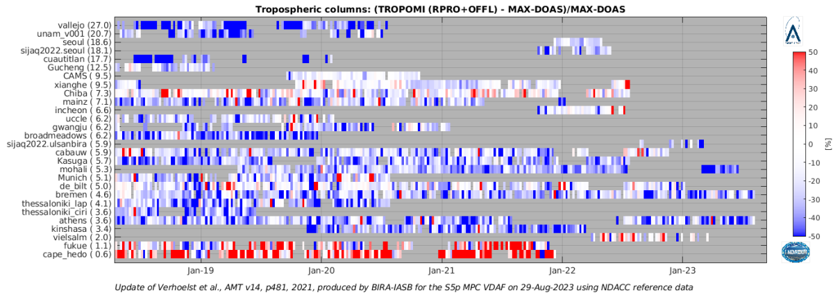
Figure 34: Time series – from May 2018 until July 2023 – of the weekly averaged relative difference [%] between S5P RPRO+OFFL v2.4 and MAX-DOAS NO 2 tropospheric column data. Stations are ordered by median tropospheric column, in brackets
