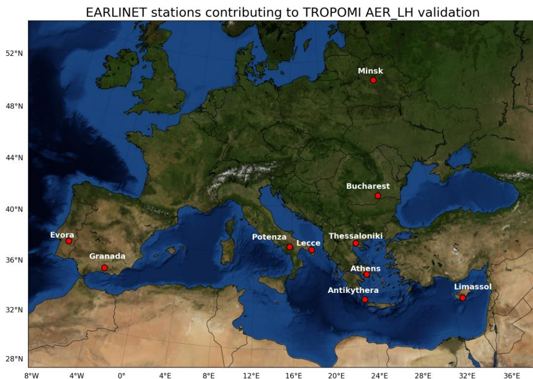
Figure 118: Geographical distribution of EARLINET ground-based stations for which co-locations with S5P L2 AER_LH data were used (period May 2018 – August 2023).
