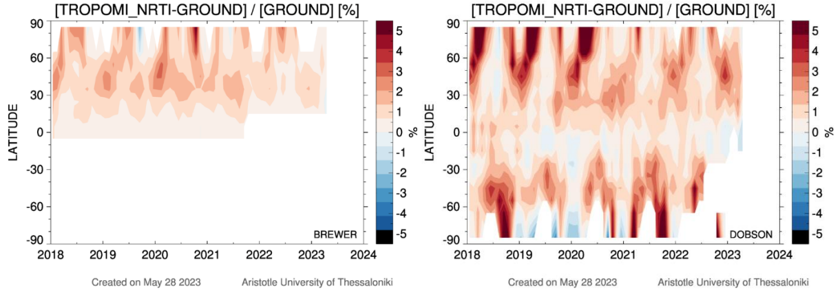
Figure 14: Time and latitude resolved analysis of the differences between NRTI total ozone and Brewer measurements (left-hand panel) and Dobson measurements (right-hand panel). Strong seasonal features in the Dobson comparisons are due (1) to the use of a fixed effective temperature in the Dobson measurement processing, and (2) due to the poorer representation of difficult surface albedo conditions before the adoption of the GE_LER surface albedo product in July 2020.
