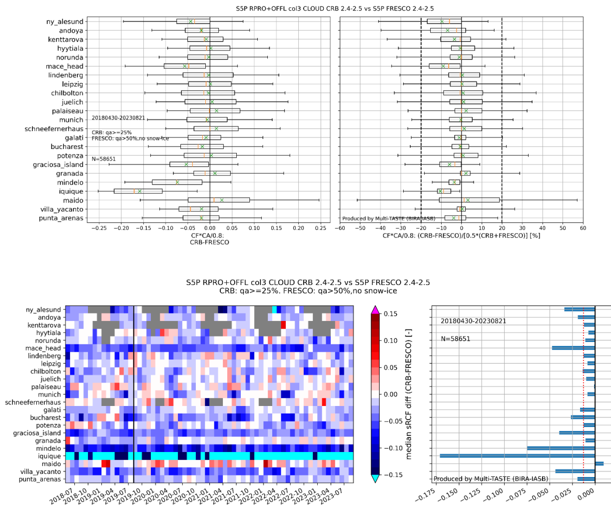
Figure 94. Top left. Box plots of S5P CLOUD CRB OFFL cloud fraction minus S5P FRESCO OFFL cloud fraction, after both have been rescaled to a cloud albedo of 0.8. Left: same but for the normed relative difference. The 20% bias requirement is indicated in dashed lines. Bottom left: monthly median of scaled cloud fraction difference, per month and per station. Indicated is the pixel size switch (2019/08/06). Bottom right: Median of scaled cloud fraction differences per station. The red dashed line gives the median of these median differences.
