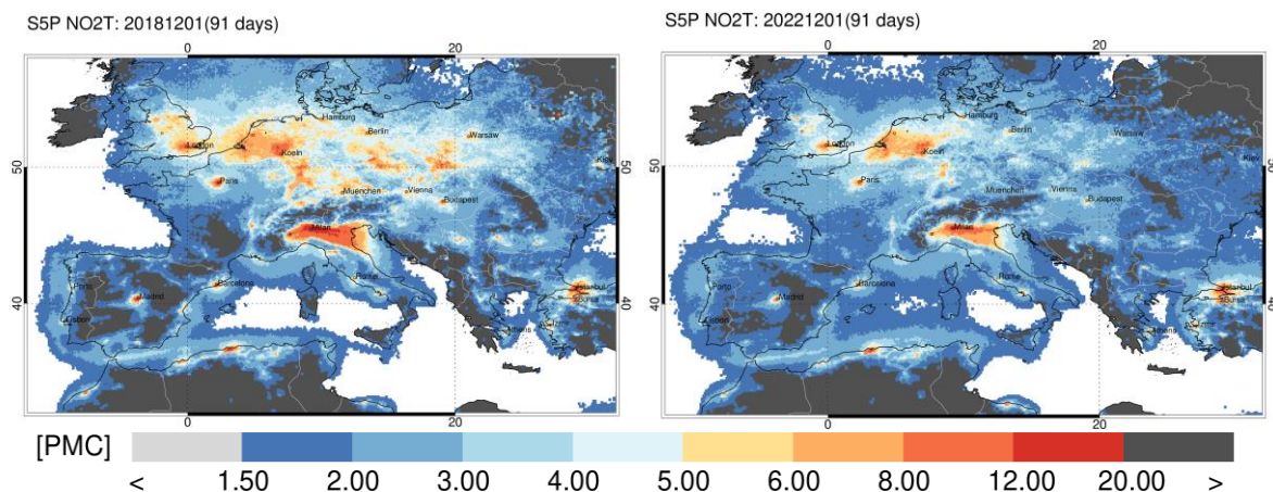
Figure 39: S5P RPRO/OFFL tropospheric NO 2 over central Europe. The data is binned on a grid of 0.1° latitude/longitude for Nov/Dec/Jan 2018/2019 and 2022/2023 (V2.4.0). A q_a\_value > 0.75 and a cloud fraction CF < 0.2 are used to reduce the amount of data and exclude cloudy scenes. 1 PMC stands for 1 Pmolec/cm 2 .
