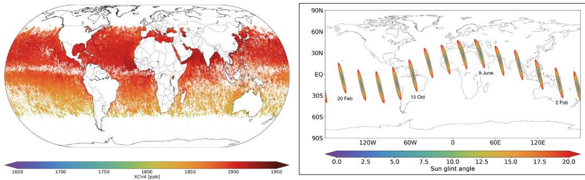
Figure 90: (left) Annual coverage of XCH 4 retrievals over the ocean for the year 2022, and (right) seasonal cycle of the sun-glint geometry.
