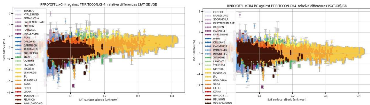
Figure 87: Dependence of the S5P-TCCON relative difference on surface albedo. The left column shows the standard S5P product and the right column the bias corrected S5P product. The bias correction removes the surface albedo dependence of the standard S5P product.
