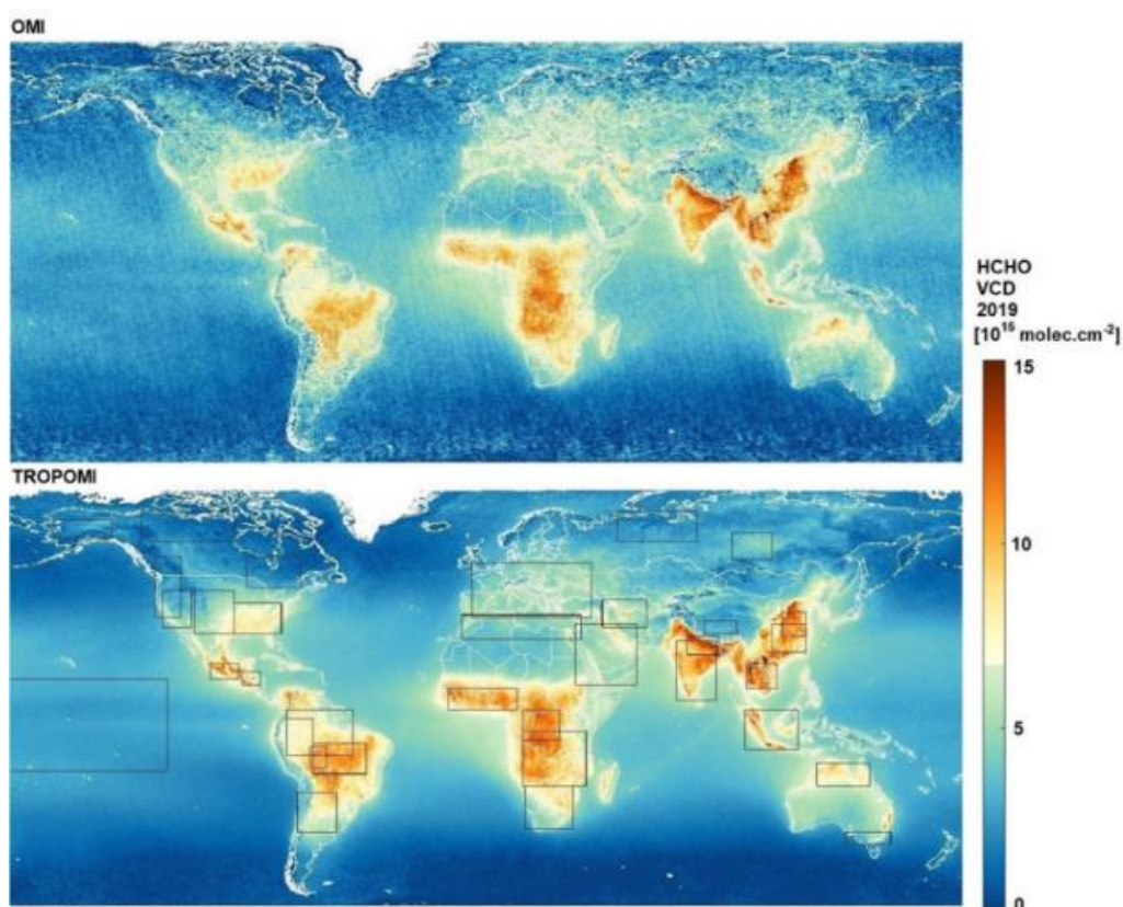
Figure 62: Average HCHO tropospheric column ( N_{v\_clear} ) retrieved from OMI (upper panel) and S5P TROPOMI (lower panel) in 2019. Limits of the regions selected for the comparisons are identified on the TROPOMI map. The same grid is used for both dataset ( 0.05^\circ ). Data are filtered using the recommended product quality flags.
