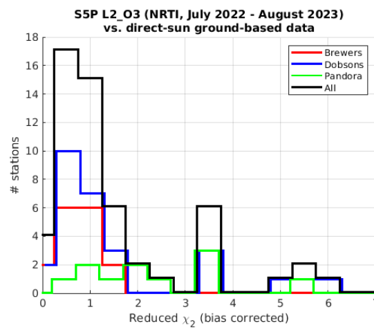
Figure 15: Histogram of the \chi_r^2 values (one per reference instrument) for S5P NRTI total ozone versus different ground-based instruments.
