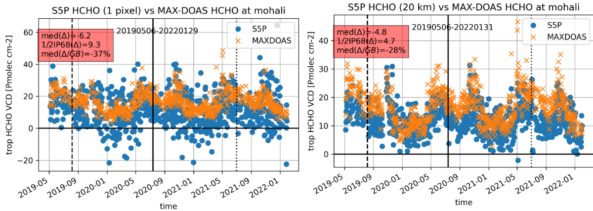
Figure 55: Time series of HCHO columns [Pmolec/cm 2 ] from S5P RPRO+OFFL and MAX-DOAS data at the Mohali station. (Left) Single S5P pixel, \pm 0.5 h MAX-DOAS averaging, (Right) 20 km area average for \geq 10 pixels, \pm 3 h averaging. Data processed 2022/02/28.
