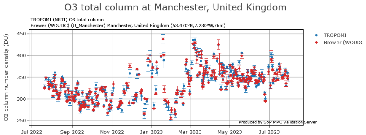
Figure 17: Time series of S5P TROPOMI NRTI (v2.4.1) and Brewer total ozone data at the station of Manchester in the United Kingdom (data courtesy J. Rimmer, University of Manchester).
