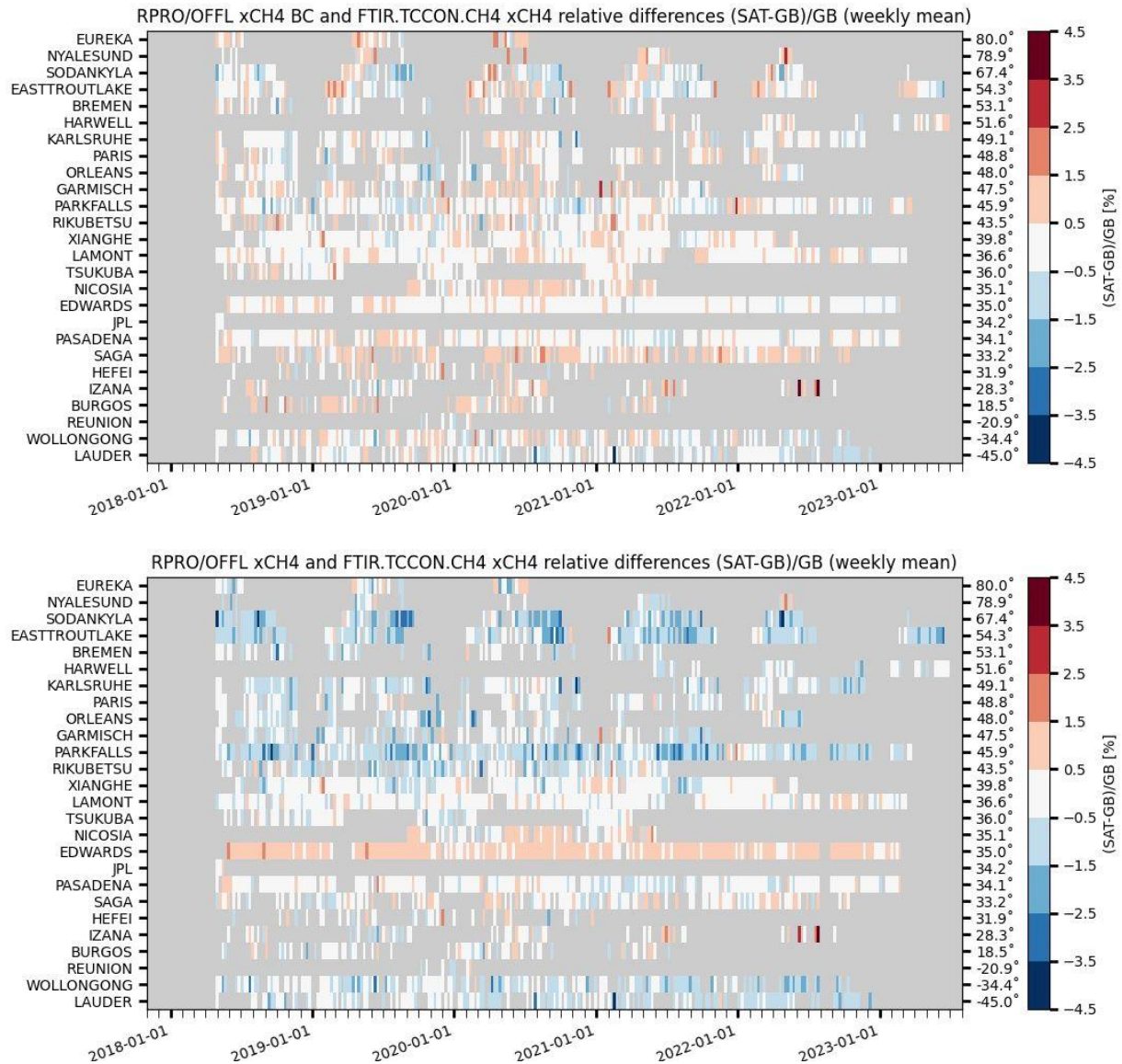
Figure 84: Mosaic plots of relative biases between S5P L2_CH4 RPRO+OFFL and ground-based CH4 TCCON column data for the bias corrected (top) and standard (bottom) methane products. Over the April 2018 – August 2023 time period the plots do not show a clear meridian dependence or temporal change in the weekly averaged biases. Colour bar gradients are chosen such that they match with the measurement's uncertainties.
