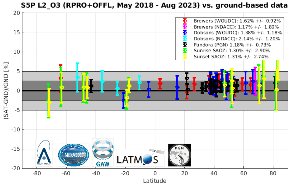
Figure 4: Meridian dependence of the median (the circular markers) and spread ( \pm 1 sigma, the error bars) of the percent relative difference between S5P TROPOMI L2_O3 (RPRO+OFFL up to August 2023) and ground-based (GND) ozone column data, represented at individual stations from the Antarctic to the Arctic and per measurement type (Brewer, Dobson, Pandora, and ZSL-DOAS). The values in the legend correspond to the median and spread of all median (per station) differences. For clarity, sunrise and sunset ZSL-DOAS results are represented separately (offset by -0.5^\circ and +0.5^\circ in latitude).
