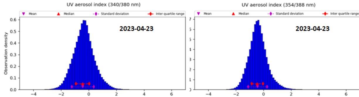
Figure 109: Frequency distribution of the UVAI (left: 340/380nm, right: 354/388 nm) for April 23, 2023.
