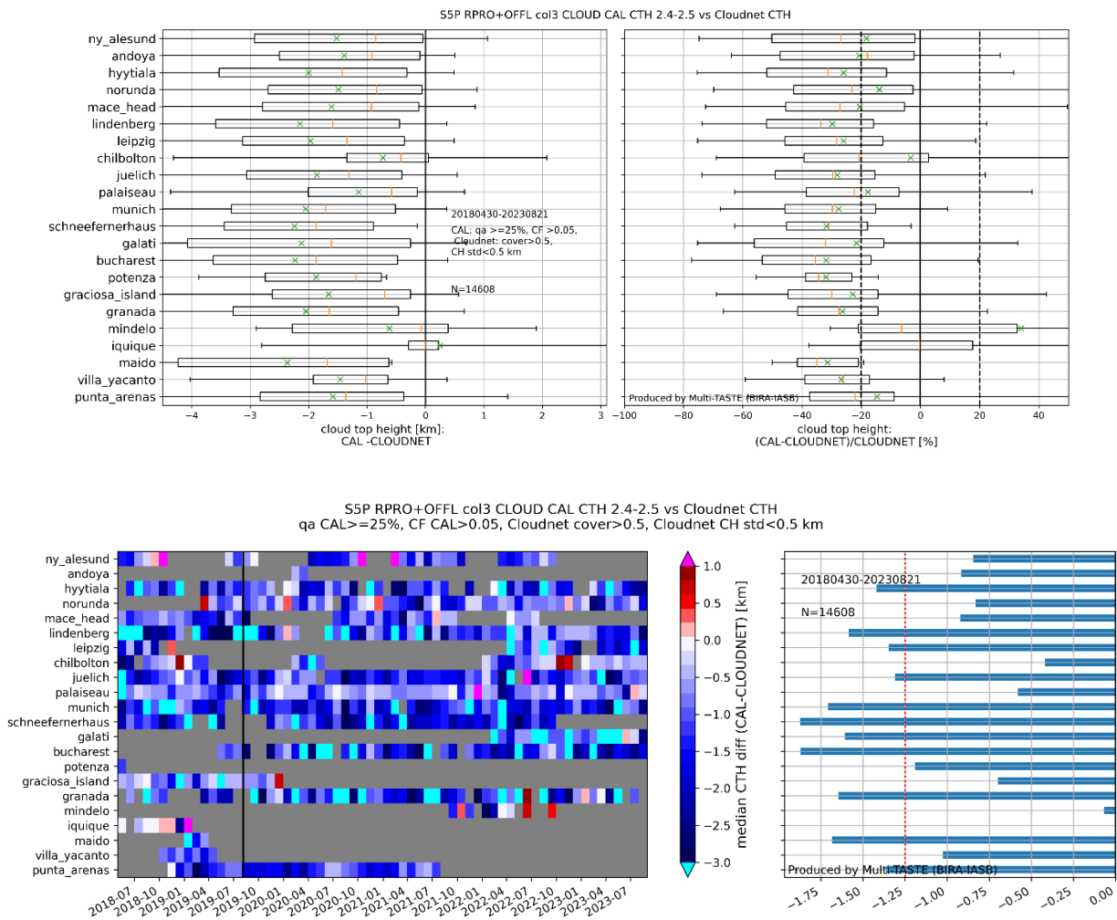
Figure 98: Top panel: Boxplots of S5P L2_CLOUD CAL CTH minus CLOUDNET CTH, per station. Boxplot conventions: box bounds are at first and third quartile. Orange line is median. Whiskers are at 5 and 95 percentiles. Green cross is mean. Right panel: Similar as upper panel but now for the relative difference. Sensing date range is indicated on the plot. Bottom left panel: monthly median of CLOUD CAL CTH-CLOUDNET CTH, per station. Pixel size switch (2019/08/06) is indicated on the plot. Right panel: median difference per station. The red dashed line gives the median over the median differences.
