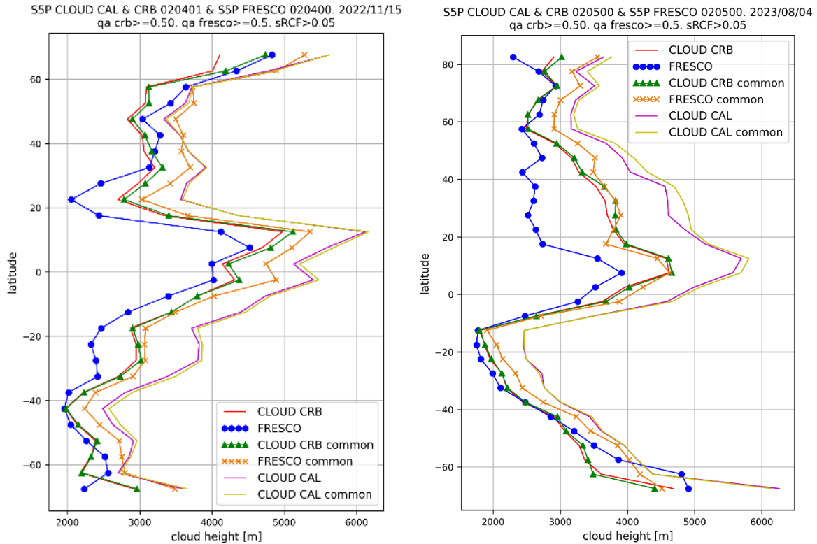
Figure 96: Latitudinal variation of zonal means of cloud height of S5P CLOUD OCRA/ROCINN_CRB, S5P FRESCO and ROCINN_CAL at two days. Selection criteria: qa\_value > 0.5 , no invalid values, sRCF > 0.05 . 'common' means the subset of valid pixels common to CLOUD and FRESCO.
