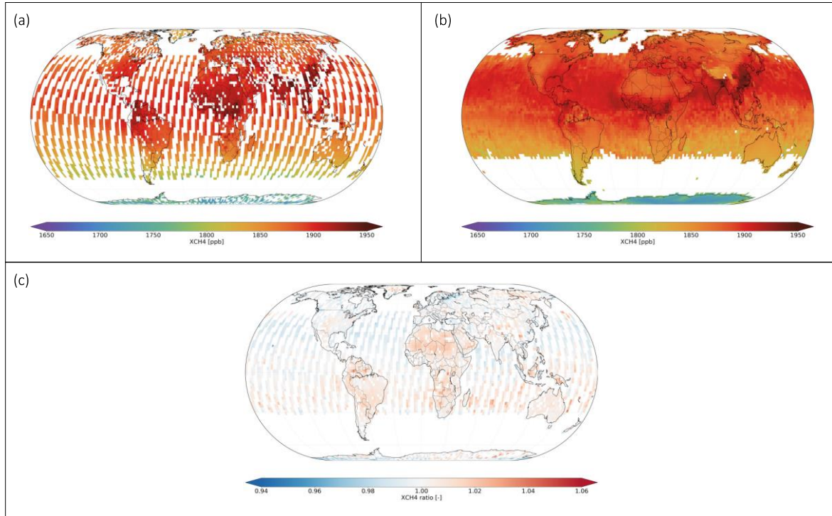
Figure 81: Global distribution of XCH 4 measured by (a) GOSAT and (b) TROPOMI and (c) the ratio of GOSAT to TROPOMI XCH 4 . Daily collocations are averaged to a 2x2 degree grid for the year 2022.
