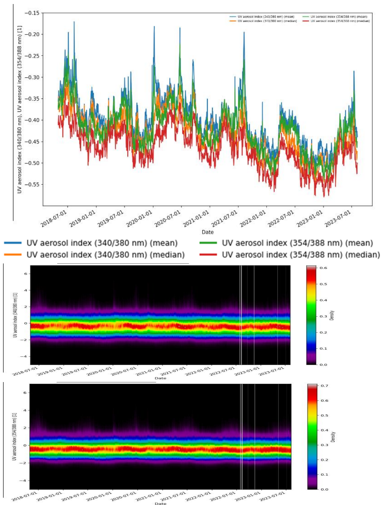
Figure 108: Comparison of the global daily mean and median for both L2_AER_AI UVAI wavelength pairs (340/380 and 354/388 nm), for the reprocessed data set from 20 July 2018 through August 2023. Middle and bottom: Corresponding histograms for both wavelength pairs.
