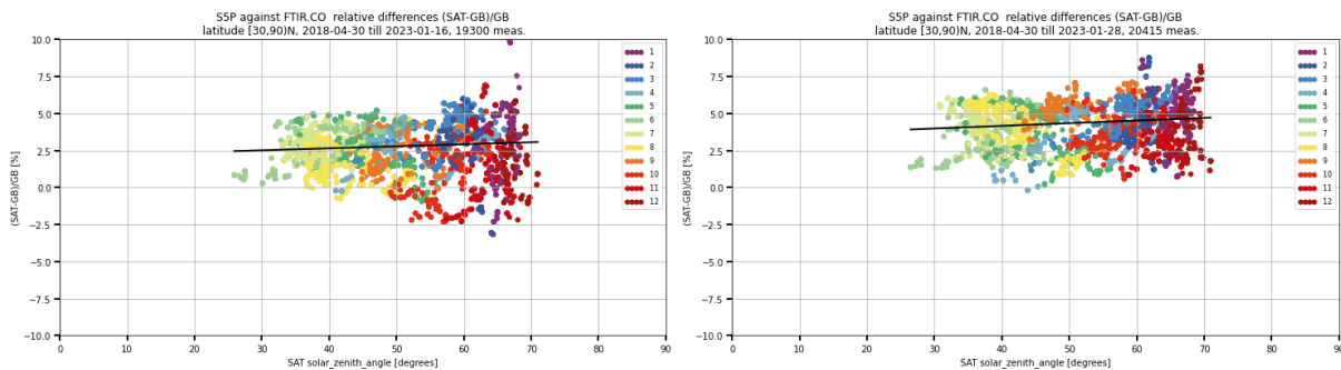
Figure 80 Left: similar to Figure 79 , but with a rolling median (21 day window) applied to reduce the scatter and to show seasonal dependences of the relative differences. The right plot shows the comparisons where the NDACC profiles are smoothed with the Tropomi averaging kernel which reduces the seasonal dependence.
