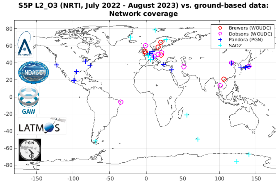
Figure 11: Geographical distribution of Brewer, Dobson, Pandora and ZSL-DOAS ground-based stations for which co-locations with S5P L2_O3 NRTI ozone data have been used (July 2022 until August 2023).
