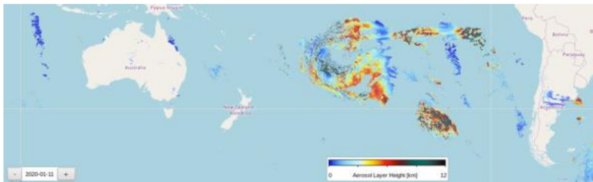
Figure 123: TROPOMI AER_LH product (processor version before v02.05.00) on 11 January 2020 over the south Pacific, showing the altitude as derived by the S5P AER_LH algorithm of the fires smoke from Australian bush fires.
