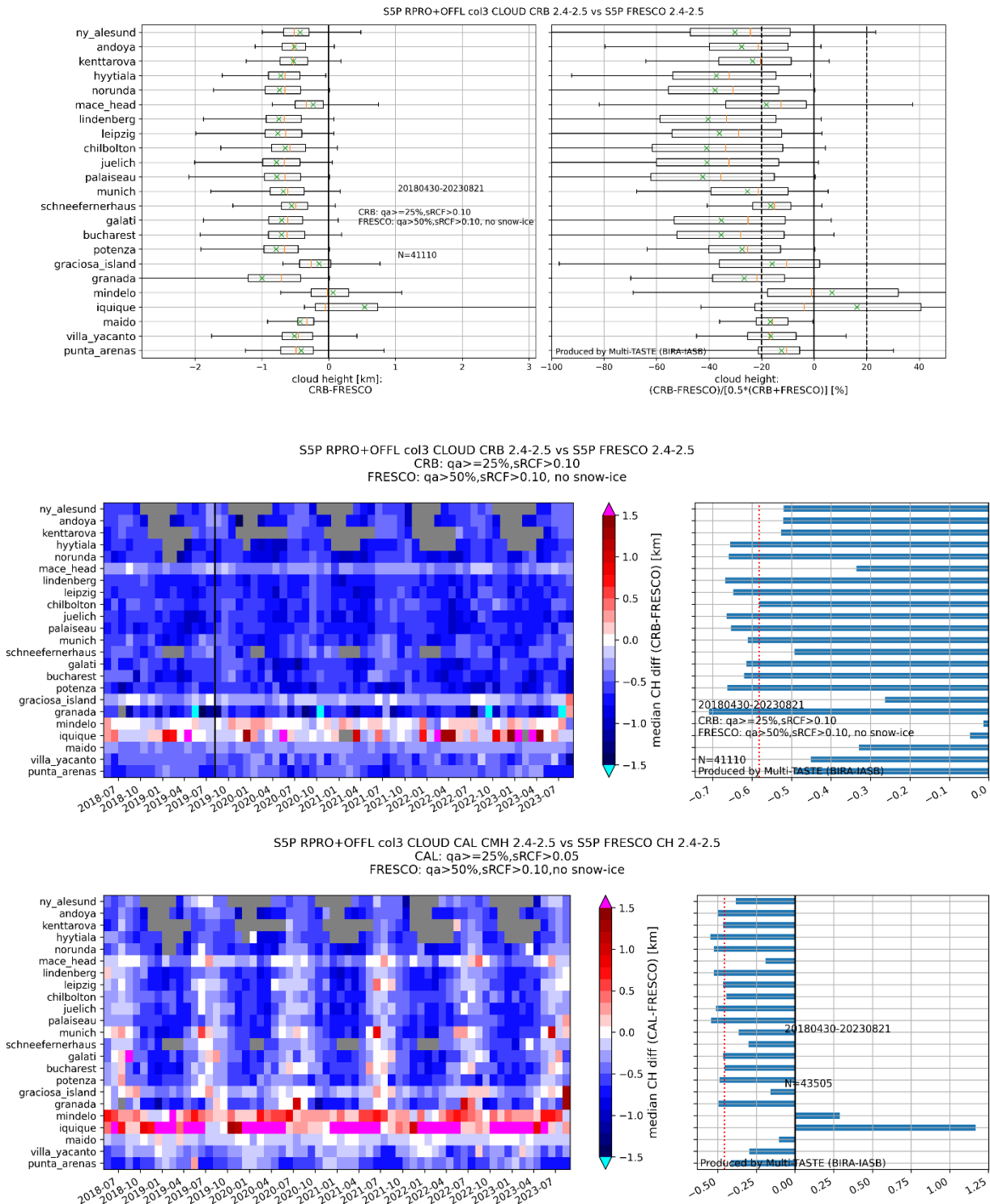
Figure 97: Top. Boxplots of S5P CLOUD CRB CH minus S5P FRESCO CH (left) and of the normed difference (right). Middle. Monthly median difference per station of CRB CH-FRESCO CH (left), and overall median difference (right). Bottom. Monthly median difference per station of CAL CMH-FRESCO CH (left), and overall median difference (right). Indicated is the pixel size switch (2019/08/06).
