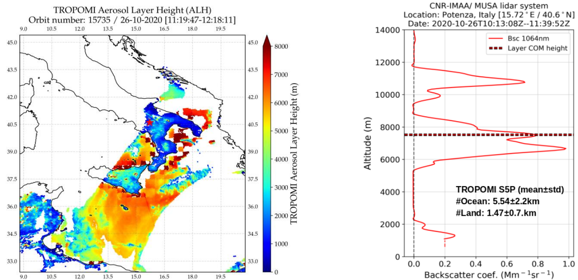
Figure 121: Left: TROPOMI ALH (processor version v02.04.00) retrievals (orbit 15735) for smoke event originated from N. America, over Italy. The red star indicates the position of the Potenza (CNR-IMAA) station. Right: same as in Figure 120.
