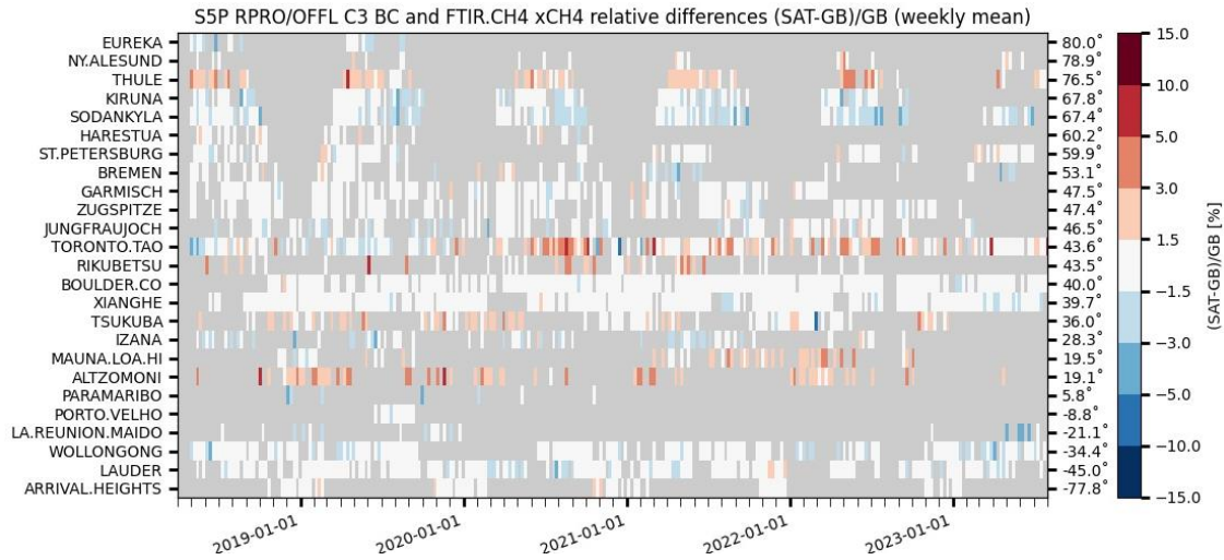
Figure 85 Mosaic plots of relative biases between S5P L2_CH4 RPRO+OFFL and ground-based CH4 NDACC column data for the bias corrected methane products. Over the April 2018 – August 2023 time period the plots do not show a clear meridian dependence or temporal change in the weekly averaged biases.
