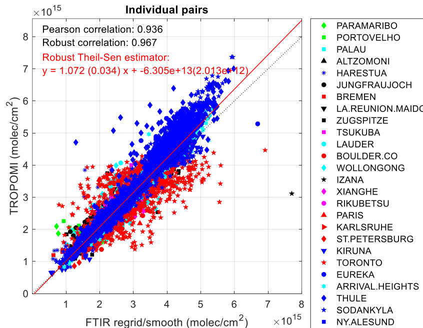
Figure 43: Scatter plot of co-located S5P TROPOMI and NDACC FTIR stratospheric \text{NO}_2 column data.
