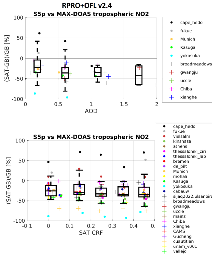
Figure 36: Relative differences between S5p TROPOMI RPRO+OFFL and MAX-DOAS NO 2 tropospheric columns as a function (upper panel) of MAX-DOAS AOD and (lower panel) S5p cloud radiance fraction (CRF). The time frame is from May 2018 until end February 2023.
