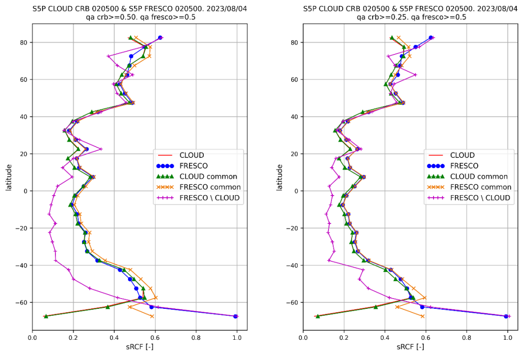
Figure 93. Latitudinal variation of zonal means of scaled radiometric cloud fraction of S5P OCRA/ROCINN CRB and S5P FRESCO-S for day 2023/08/04. Two quality filter criteria are used for CRB: the standard qa\_value > 0.5 , and a looser qa\_value > 0.25 .
