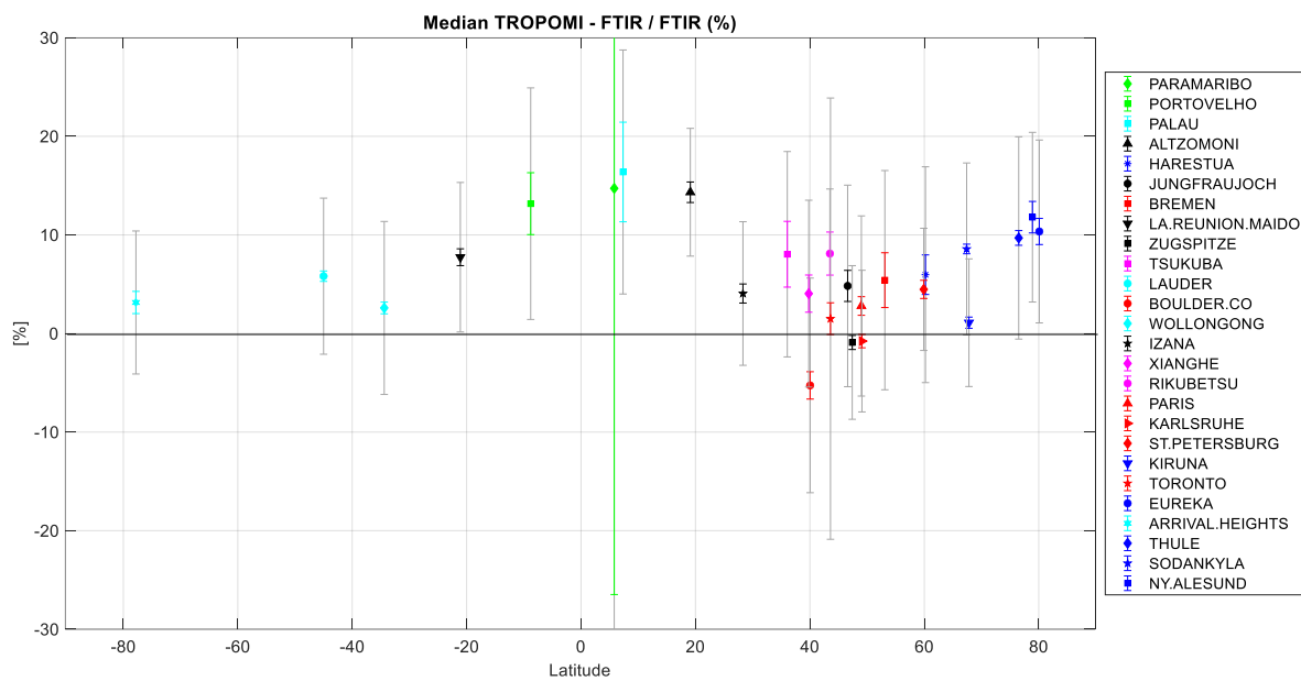
Figure 42: Median bias at each NDACC FTIR station as a function of latitude, calculated as the median of the percentage difference between S5P L2_NO2 and the FTIR NO 2 stratospheric column measurement. The grey bars are the scaled MAD (see Sect. 6.2.1), and the coloured bars are the \pm 2\sigma error on the bias.
