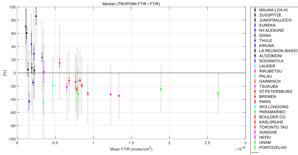
Figure 53: Percent bias between S5P L2_HCHO and NDACC FTIR HCHO column data at each station as a function of the mean FTIR total column ( 10^{16} molec/cm 2 ). The grey bars are the systematic uncertainty on the difference, and the coloured error bars are the 2- \sigma errors on the bias. The temporal range is May 2018 to November 2023 (updated from Vigouroux et al. (2020), Fig. 3).
