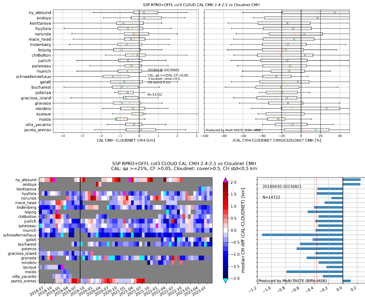
Figure 99: Top panel: Boxplots of S5P L2_CLOUD CAL CMH minus CLOUDNET CMH, per station. Boxplot conventions: box bounds are at first and third quartile. Orange line is median. Whiskers are at 5 and 95 percentiles. Green cross is mean. Right panel: Similar as upper panel but now for the relative difference. Sensing date range is indicated on the plot. Bottom left panel: monthly median of CLOUD CAL CMH-CLOUDNET CMH, per station. Pixel size switch (2019/08/06) is indicated on the plot. Right panel: median difference per station. The red dashed line gives the median over the median differences.
