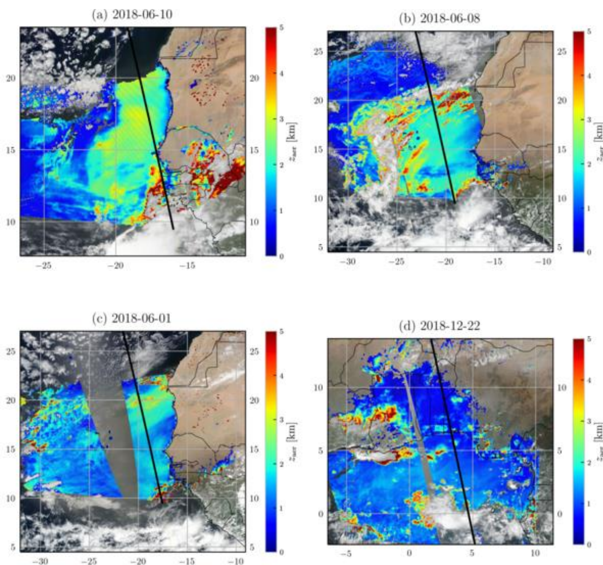
Figure 112: Details of the selected validation cases, showing the ALH (processor version before v02.05.00) on a VIIRS RGB background. The black line represents the Calipso track.
