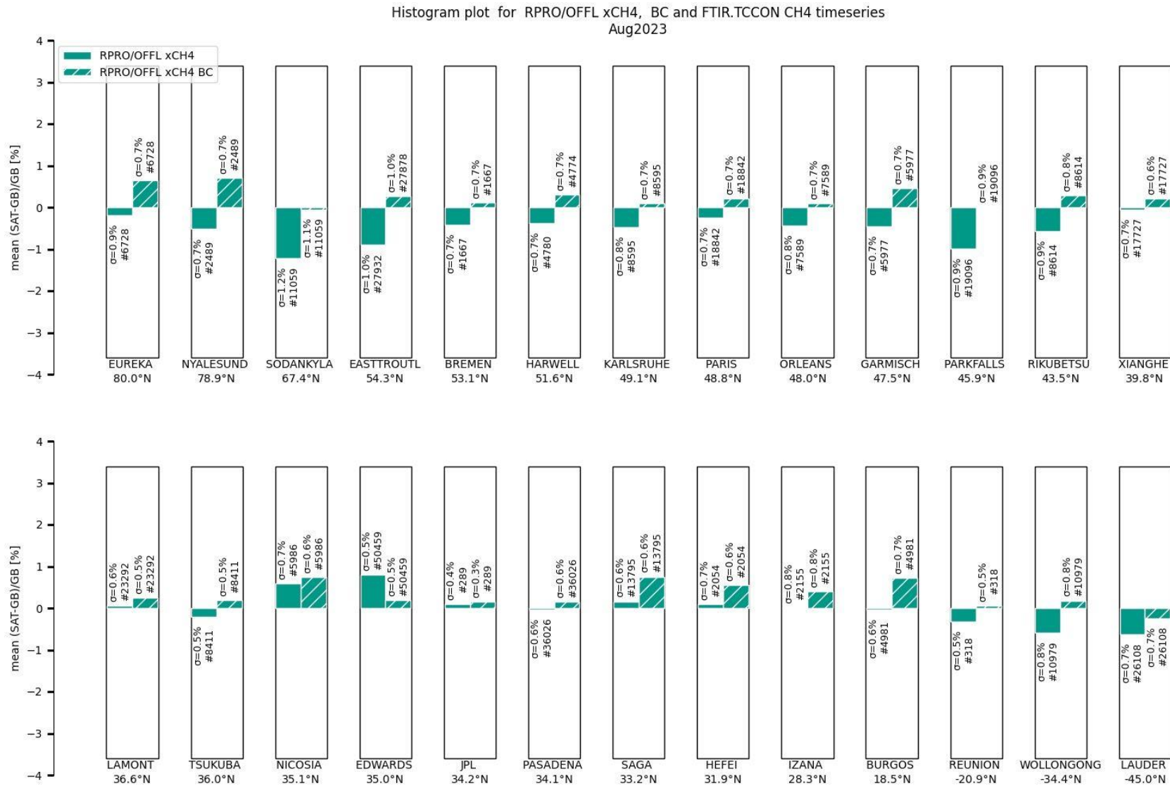
Figure 86: Chart of relative mean difference between S5P L2_CH 4 and FTIR CH 4 column data at 24 TCCON stations within the time range April 2018 until August 2023. The stations are sorted with decreasing latitude. The relative mean difference of the standard and bias-corrected xCH 4 products never exceeds the mission requirements (bias below 1.5 %).
