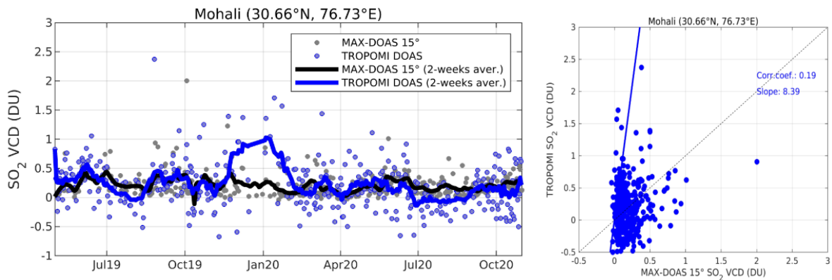
Figure 72: Comparison of TROPOMI SO 2 VCDs to MAX-DOAS measurements (daily means) at Mohali (India) from June 2019 to November 2020. The following selection criteria were applied: distance < 25km, CF<0.2, AMF>0.2, time window +/- 1h around overpass. Courtesy of N. Theys (BIRA-IASB), data provided by, Vinod Kumar, Vinayak Sinha, Sebastian Donner, Steffen Dörner, Thomas Wagner.
