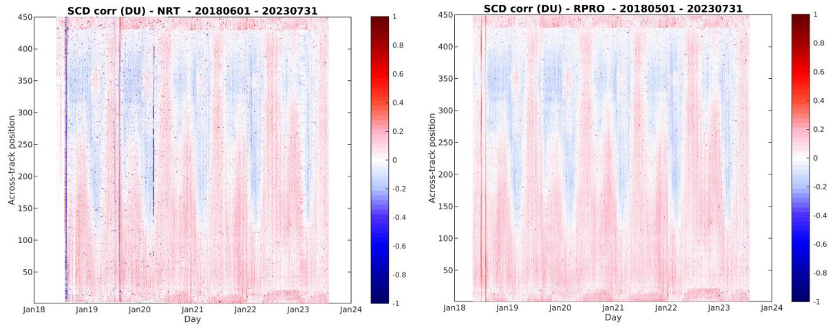
Figure 76: Comparison of the NRT (left) and offline (right) SO 2 data products. Shown are the time series of background corrected SO 2 SCDs for all 450 detector rows from June 2018 to August 2023. Most of the short time features (vertical coloured lines) are caused by individual strong volcanic eruptions. For the NRT product, a strong spike occurs in early April 2020, which is caused by a downlink issue that corrupted an irradiance file. Courtesy of Nicolas Theys, BIRA-IASB.
