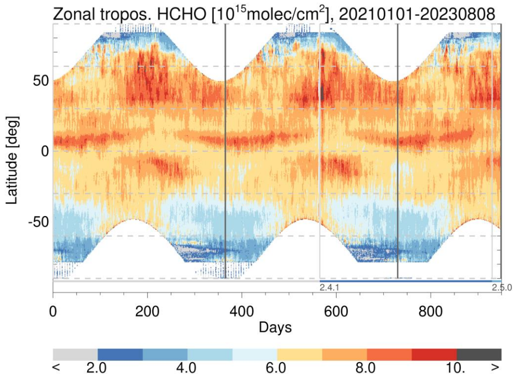
Figure 65: S5P TROPOMI HCHO column data [ 10^{15} molec/cm 2 ] as a function of day and latitude. The period is from January 2021 to August 2023. Grid box size in latitude direction is 0.5°. The grey vertical lines mark the processor version changes, the black lines the beginning of each year.
