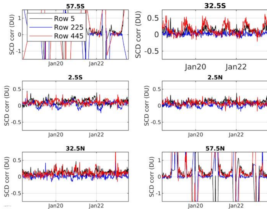
Figure 75: Temporal evolution of the averaged SO 2 SCD for selected 5° latitude bands and 3 detector rows from December 2018 to August 2023. The values are close to zero and show relatively small day-to-day variations. The larger variations in August 2019 are caused by strong volcanic eruptions. Courtesy Nicolas Theys (BIRA-IASB).
