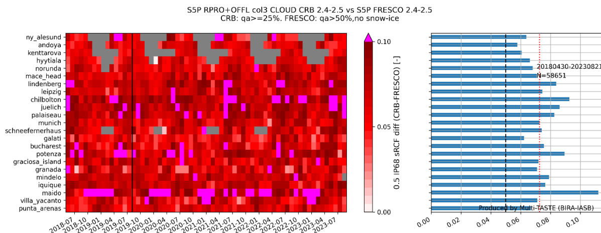
Figure 95. Left. Monthly \frac{1}{2} IP68 of scaled cloud fraction difference of CLOUD OFFL vs FRESCO OFFL, per month and per station. Indicated is the pixel size switch (2019/08/06). The UPAS version change to 2.5.0 does not impact CLOUD and is therefore not indicated. Right: \frac{1}{2} IP68 of scaled cloud fraction difference (CLOUD CRB-FRESCO), per station.
