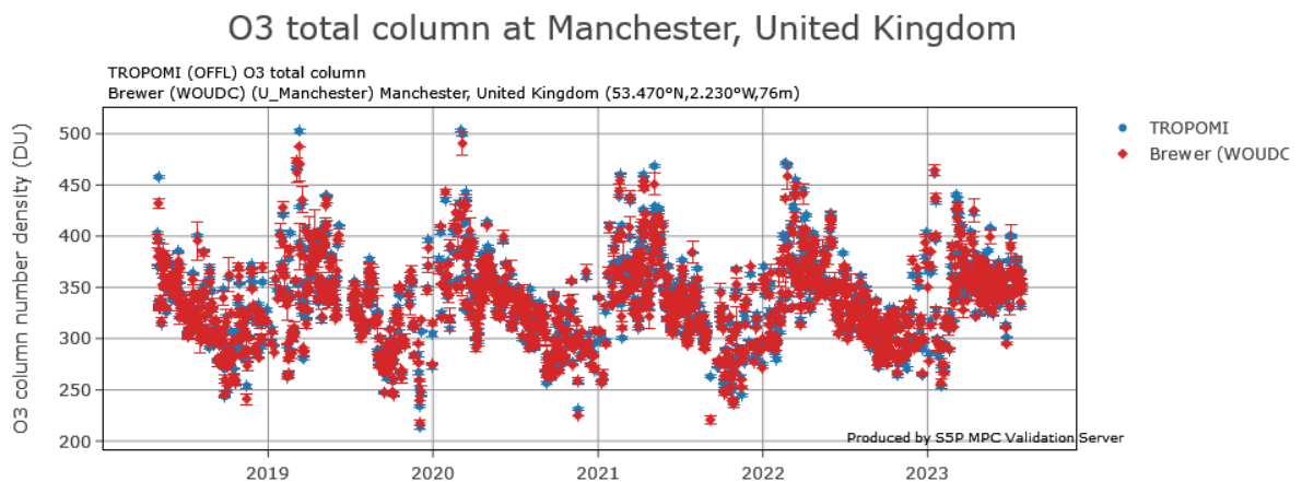
Figure 10: Time series of S5P TROPOMI OFFL and Brewer total ozone data at the station of Manchester in the United Kingdom (data courtesy J. Rimmer, University of Manchester).
