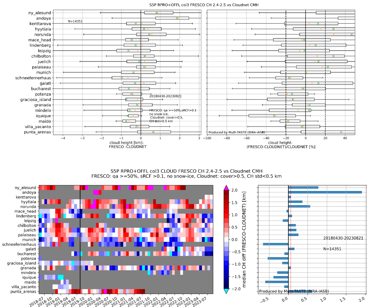
Figure 101: Upper panel: Boxplots of S5P L2_CLOUD FRESCO RPRO+OFFL v1.3-v1.4 CH minus CLOUDNET CH (upper left) and of the relative difference (upper right), per station. The same conventions as for Table 17 apply. Sensing time range is indicated on the figure. Bottom left panel: monthly median of FRESCO CH-CLOUDNET CH, per station. Pixel size switch (2019/08/06) is indicated on the plot. Bottom right panel: Median difference per station. The red dashed line indicates the median of the median differences.
