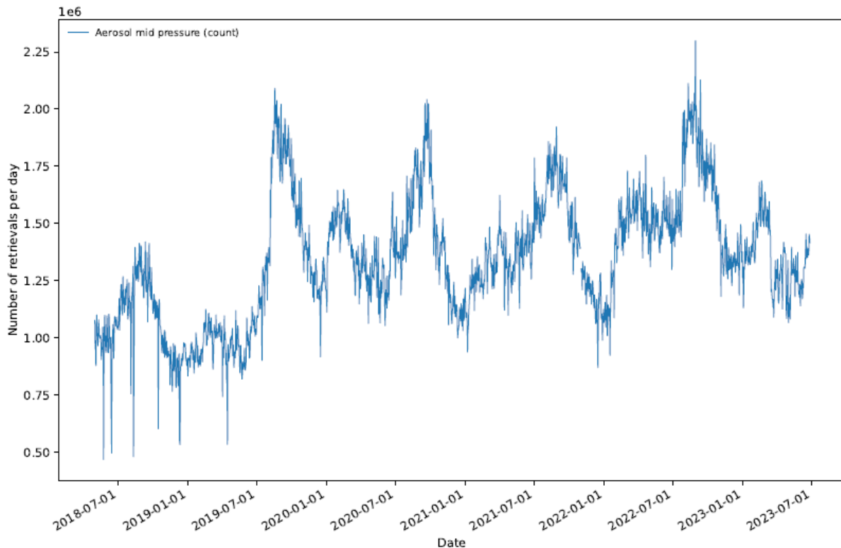
Figure 122: Number of successfully processed ALH pixels per day from June 2018 to July 2023 (RPRO data).
