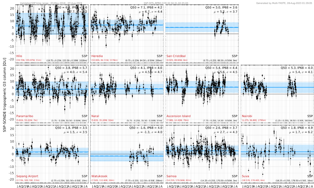
Figure 22: Time series of the absolute difference between spatially and temporally co-located S5P and ozonesonde tropospheric O 3 column data. The blue line and shaded area shows the median value and the range between the 16% and 84% percentiles. Positive values indicate a high bias of S5P w.r.t. the reference.
