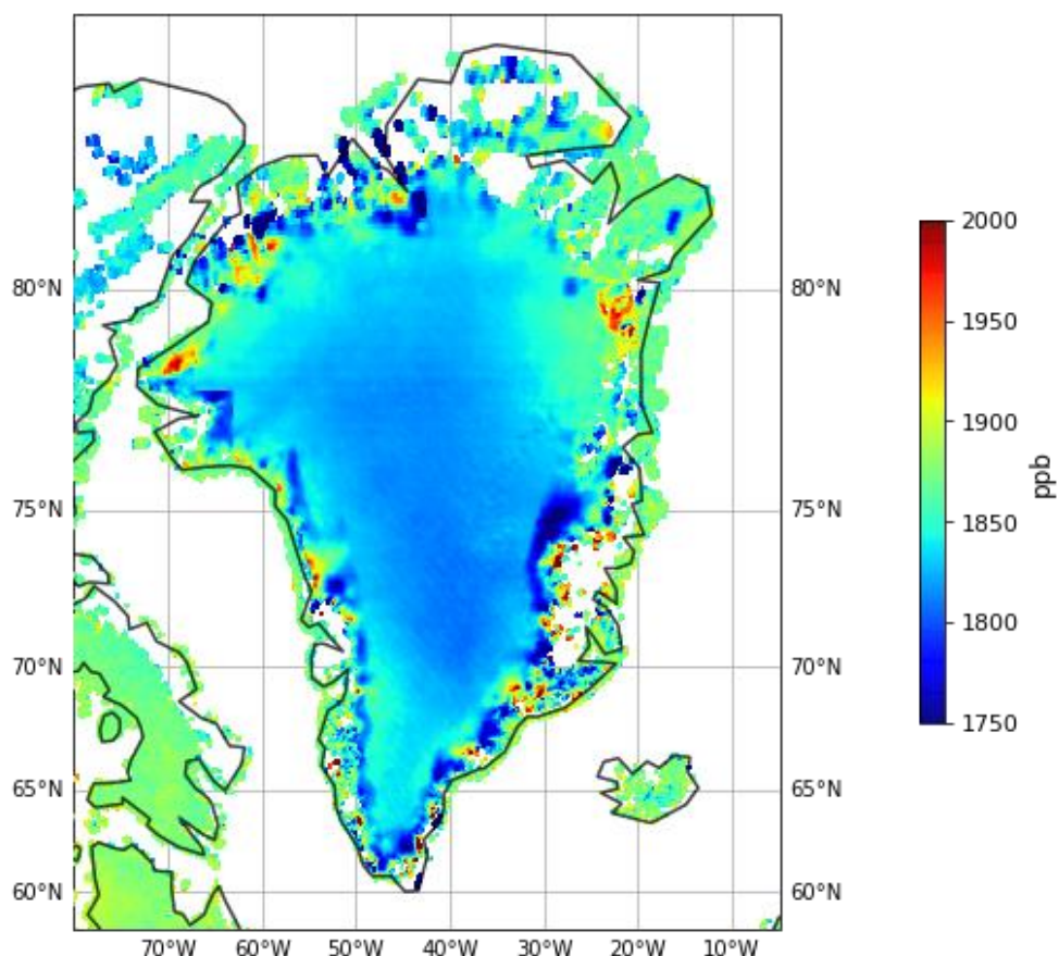
Figure 89: Map showing XCH 4 concentrations above Greenland and parts of North America for three years averaged data with pixels with qa_value > 0.5. The XCH 4 pixels in Greenland shows outliers along the mountain and coastline regions. Similar features are observed at the Antarctic.
