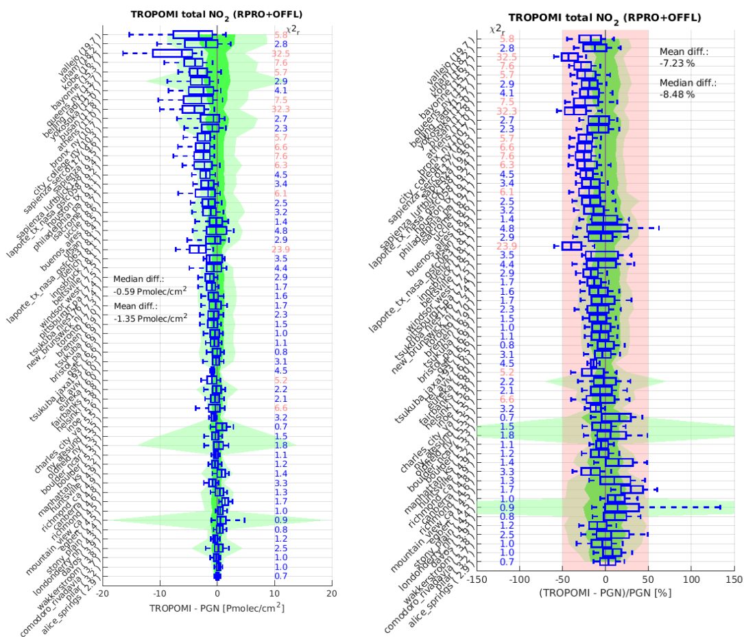
Figure 46: Box-and-whisker plots summarizing the bias and spread [Pmolec/cm 2 ] (left) and relative bias and spread [%] (right) between S5P TROPOMI RPRO+OFFL and PGN Pandora NO 2 total column data. Conventions of the boxplots are identical to Figure 33 . Stations are ordered by median total column. The time frame is May 2018 to August 2023. Poor reduced \chi^2 s (i.e. those above 5) are marked in red.
