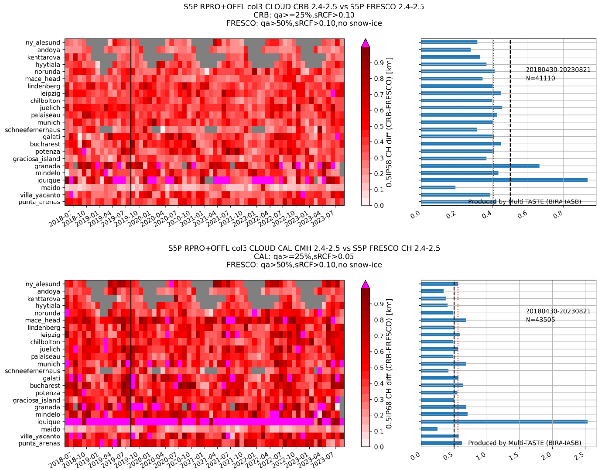
Figure 102: Top. Left: Monthly \frac{1}{2} IP68 of the cloud height difference of CLOUD CRB OFFL vs FRESCO OFFL, per month and per station. Indicated is the pixel size switch (2019/08/06). Right: \frac{1}{2} IP68 of S5P CLOUD CRB CH minus S5P FRESCO CH. Sensing date range is indicated on the figure. Bottom. Similar but for CLOUD CAL CMH vs FRESCO CH.
