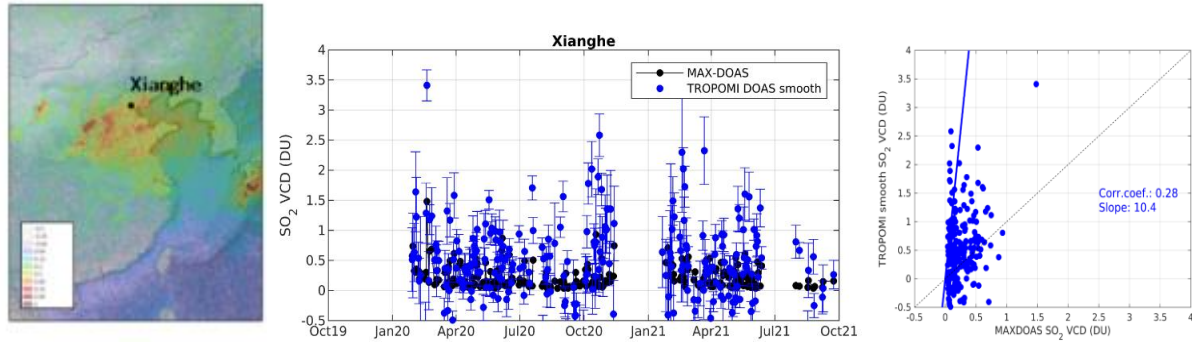
Figure 69: Comparison of TROPOMI SO 2 VCDs to MAX-DOAS measurements (daily means) at Xianghe (China). The following selection criteria were applied: distance < 25km, CF<0.2, AMF>0.2, time window +/- 1h around overpass. Courtesy of N. Theys (BIRA-IASB).
