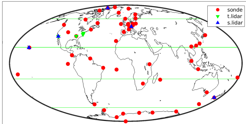
Figure 26: Geographical distribution of the ozonesonde and tropospheric (t.) and stratospheric (s.) lidar stations with which co-locations with S5P L2_O3_PR data have been identified and used in the data comparisons reported hereafter.
