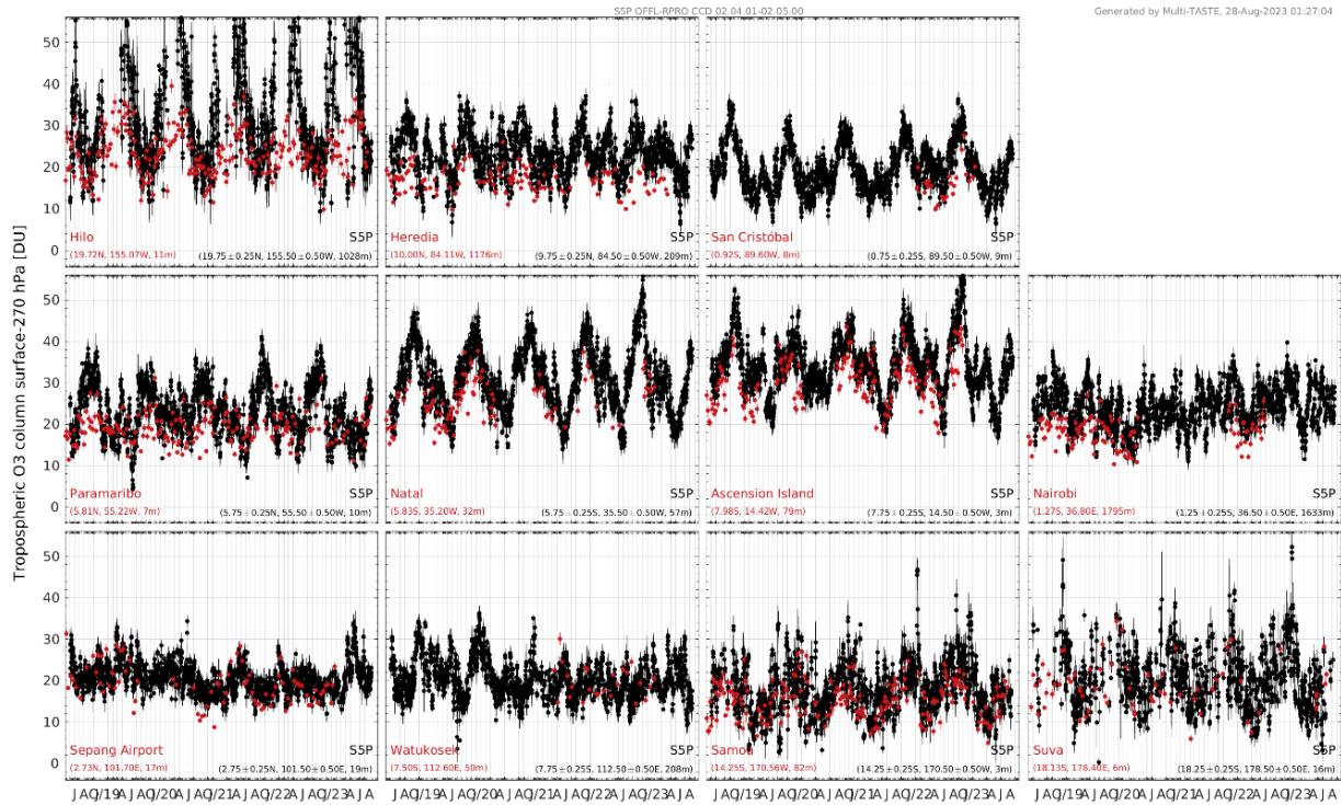
Figure 21: Time series of spatially co-located tropospheric O 3 column data by ozonesonde (red) and by S5P RPRO+OFL v02.04.01-02.05.00 (black). All data were screened following recommendations by the data providers.
