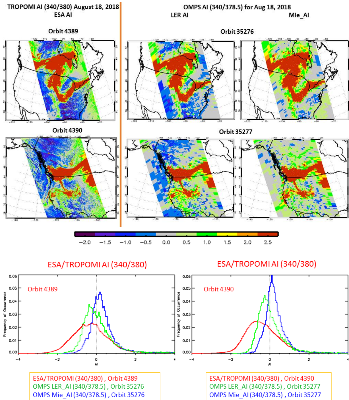
Figure 106: Comparison of UVAI from TROPOMI and OMPS for an observation of a biomass burning plume (18 Aug. 2018). For OMPS UVAI are calculated assuming either LER or Mie clouds. The UVAI for Mie clouds yields results that are more consistent. TROPOMI and OMPS LER results show very good agreement. However, the frequency distribution is broader for TROPOMI observations (courtesy of Omar Torres and Changwoo Ahn, NASA-GSFC).
