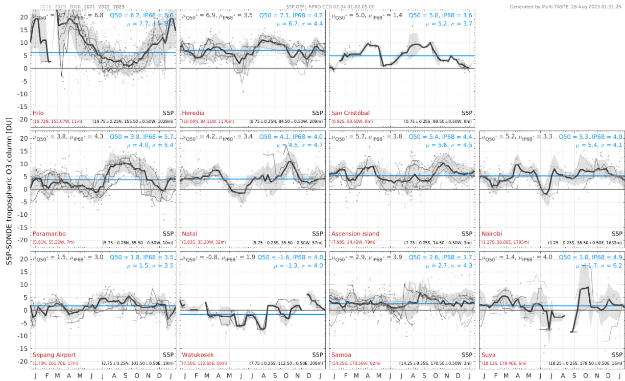
Figure 25: Annual cycle of the absolute difference between spatially and temporally co-located S5P and ozonesonde tropospheric O 3 column data. Individual comparison pairs are grey-shaded by year. Lines indicate the 29-day moving mean of the absolute difference for each year individually (thin grey) and all years combined (thin black). The blue line shows the median value over all comparison pairs. Positive values indicate a high bias of S5P w.r.t. the reference.
