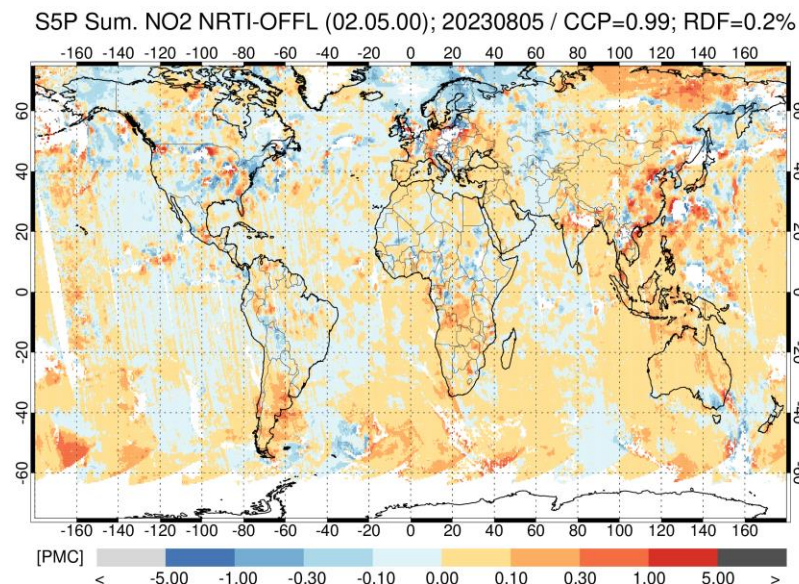
Figure 49: Difference between S5P NRTI and OFFL V2.4.0 daily total NO 2 column data (binned to 0.5°x0.5° resolution) for 2023/08/05. The difference is only calculated for columns > 0.5 Pmolec/cm 2 , cloud fractions < 0.6 and a qa_value > 0.5.
