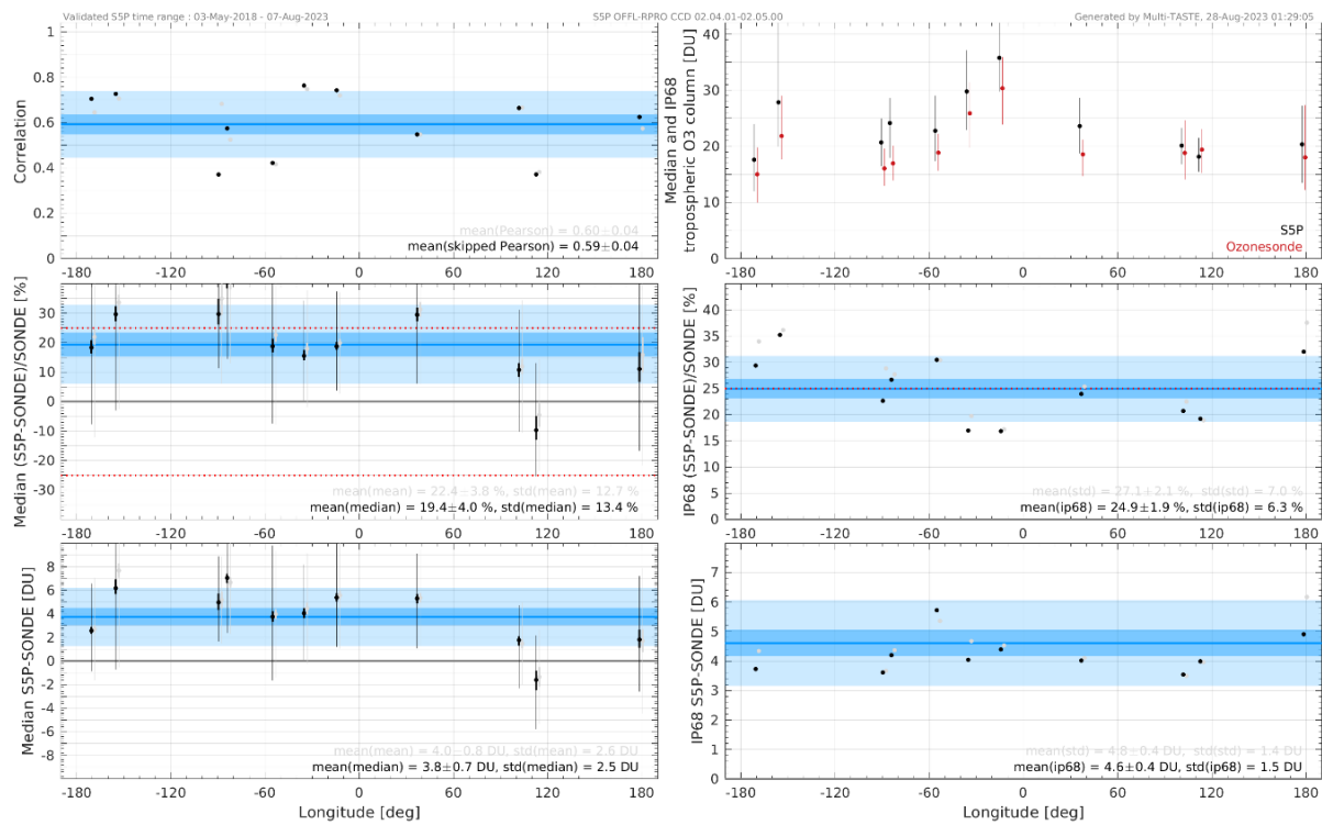
Figure 24: Overview of correlation (top left), median bias (middle & bottom left) and dispersion of the difference (middle & bottom right) of S5P tropospheric O 3 column data for each SHADOZ station (black markers). Black vertical bars represent the 68% interpercentile of the difference. The mean, standard error of the mean (1 \sigma ) and standard deviation (1 \sigma ) of the quality indicator across the network are shown as a horizontal blue line and shaded areas.
