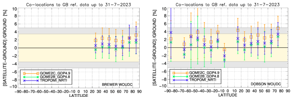
Figure 13: Comparison of the mean percentage differences between three satellite products (S5P TROPOMI L2_O3 NRTI, GOME-2B GDP 4.8 and GOME-2C GDP4.9) and ground-based total ozone data, versus latitude. The Brewer network comparisons are shown at the left-hand panel and the Dobson network comparisons are depicted at the right-hand panel, both datasets are downloaded from WOUDC. The period of data used for these plots is January 2022 – July 2023 (i.e., not only v2.4.1 data in order to have sufficiently representative statistics).
