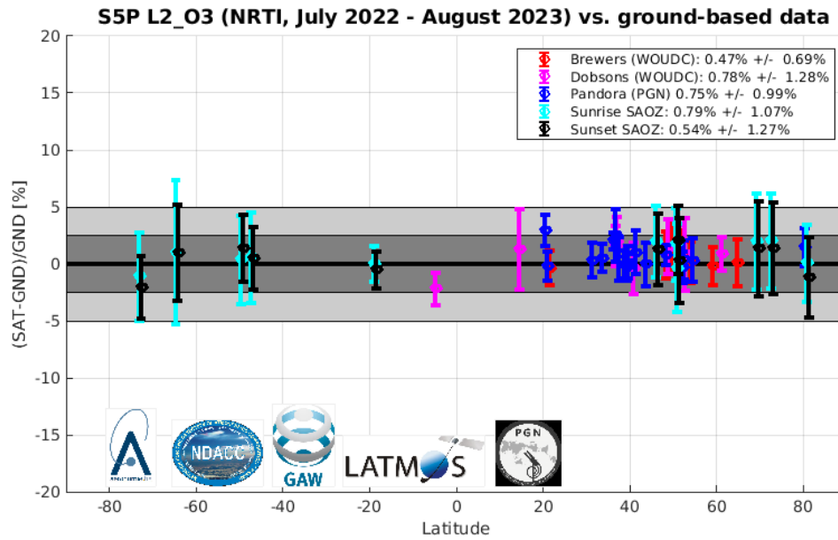
Figure 12: Meridian dependence of the median (the circular markers) and spread ( \pm 1 sigma, the error bars) of the percent relative difference between S5P TROPOMI L2_O3 (PDGS NRTI processor v2.4.1, up to August 2023) and ground-based (GND) ozone column data, represented at individual stations from the Antarctic to the Arctic and per measurement type (Brewer, Dobson, Pandora, and ZSL-DOAS). The values in the legend correspond to the median and spread of all median (per station) differences. For clarity, sunrise and sunset ZSL-DOAS results are represented separately (offset by -0.5^\circ and +0.5^\circ in latitude).
