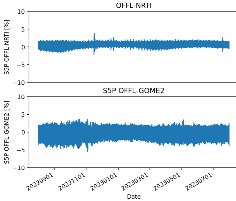
Figure 18: Time series of the differences between the different gridded (level-3) total ozone column data sets. Upper panel: S5P OFFL versus S5P NRTI (both v2.4.1 and above). Lower panel: S5P OFFL versus GOME-2 (MetOp-B and MetOp-C, processors GDP 4.8 and 4.9 respectively, but these are identical for the total ozone column product).
