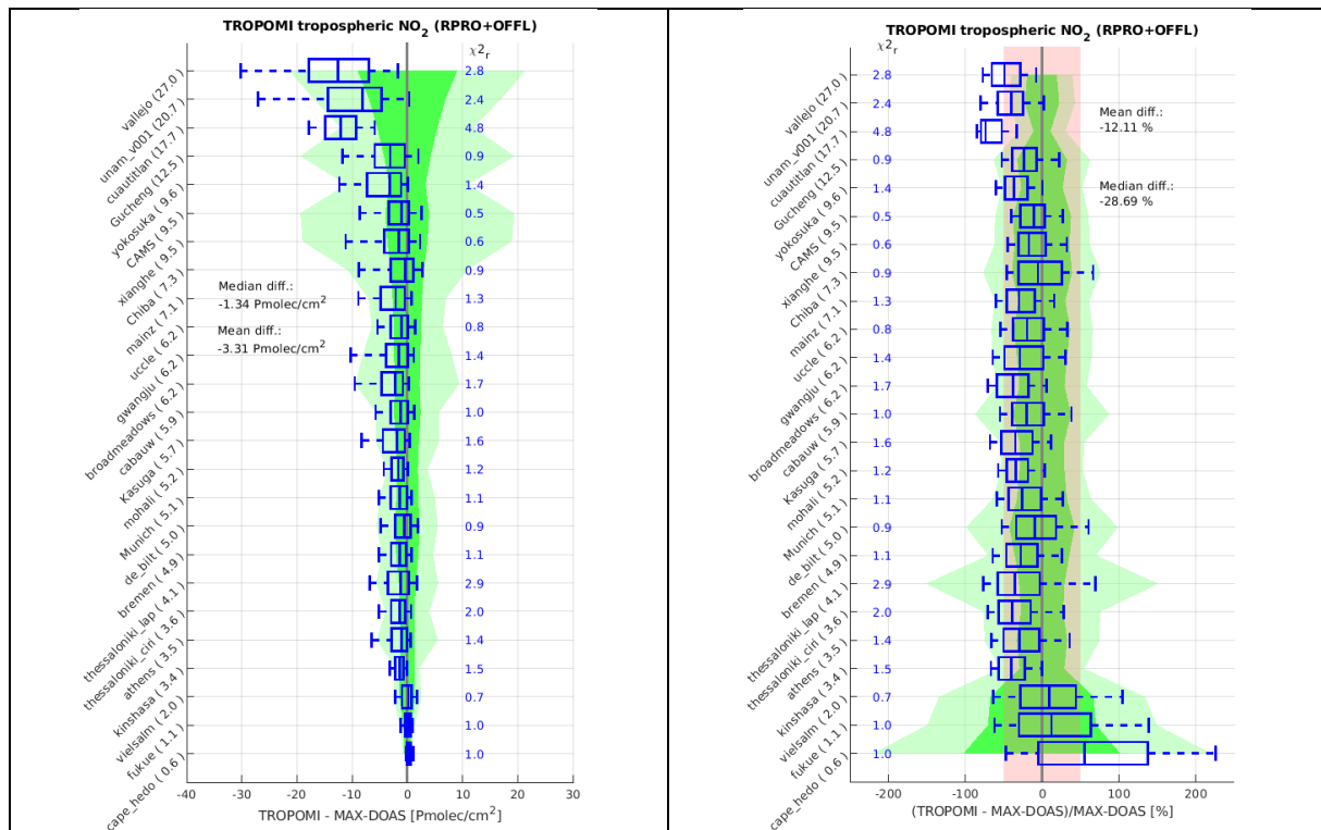
Figure 33: Box-and-whisker plots summarizing the bias and spread of the difference between S5P TROPOMI RPRO+OFFL v2.4 and MAX-DOAS NO 2 tropospheric columns (left: absolute, right: relative). Values between brackets in the labels denote the median tropospheric column at the station. The time frame is from May 2018 until July 2023 (see next figure). Stations are ordered by median tropospheric column. The median difference is represented by a vertical solid line inside the box, which marks the 25 and 75% quantiles. The whiskers cover the 9-91% range of the differences. The red shaded area represents the mission requirement of 50% for the uncertainty. Also indicated is the combined ex-ante uncertainty (green shaded areas, where dark green represents the median combined uncertainty and light green the 95% percentile), and the reduced chi 2 of the comparison for each station.
