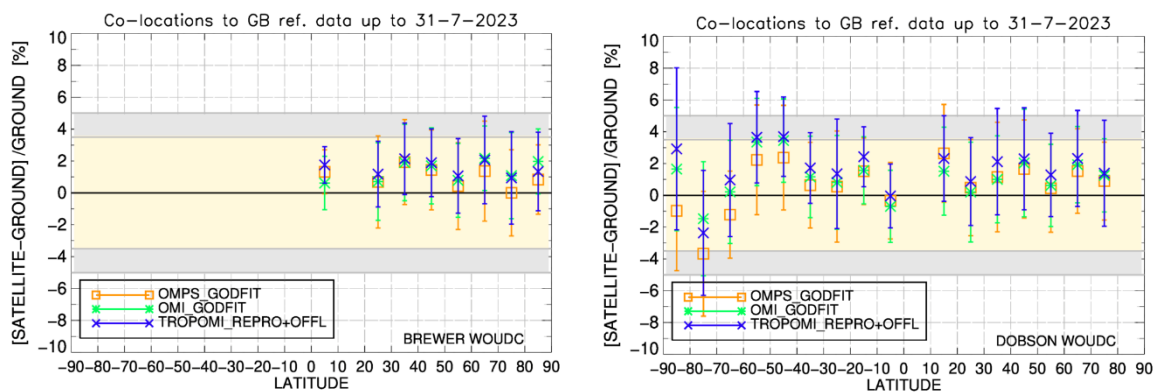
Figure 5: Comparison of the mean percentage differences between three satellite products (S5P L2_O3 OFFL, OMI GODFIT v4 and OMPS GODFIT v4) and ground-based total ozone data, versus latitude. The Brewer network comparisons are shown at the left-hand panel and the Dobson network comparisons are depicted at the right-hand panel, both datasets are downloaded from WOUDC. The period of data used for these plots is April 2018 –July 2023 (due to ground-based data availability), RPRO until 3 August 2022 and OFFL afterwards.
