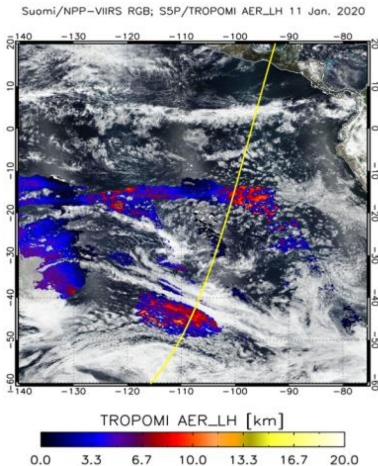
Figure 124: NPP/VIIRS RGB image with S5P/TROPOMI AER_LH on 11 January over the south Pacific with the CALIPSO track of that day overlaid in yellow.
