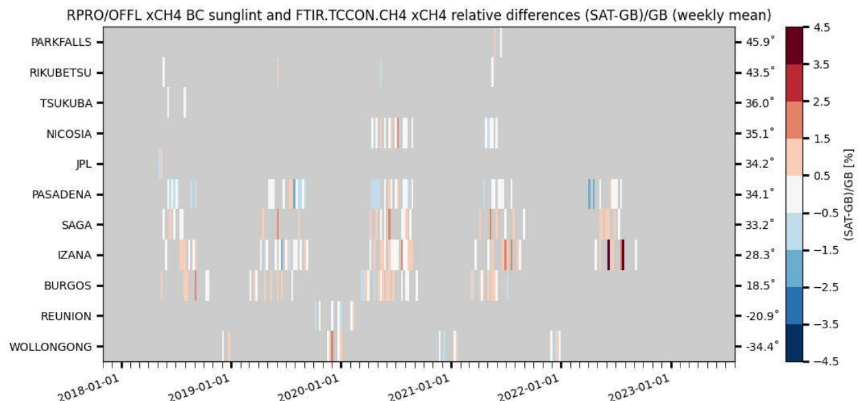
Figure 91: Mosaic plots of relative biases between S5P scientific L2_CH4 product and ground-based CH 4 TCCON column data for the bias corrected methane products.
