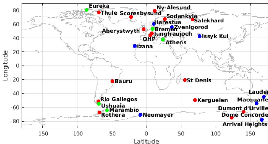
Figure 32: Geographical distribution of the NDACC ZSL-DOAS instruments routinely measuring stratospheric NO 2 and yielding co-locations with the current S5P L2_NO2 datasets. Stations marked with a red dot contribute fast delivery data coming from the LATMOS_RT facility. Blue and green dots depict the NDACC stations that contribute ZSL-DOAS data directly through the NDACC DHF and the AO project NIDFORVAL, respectively.
