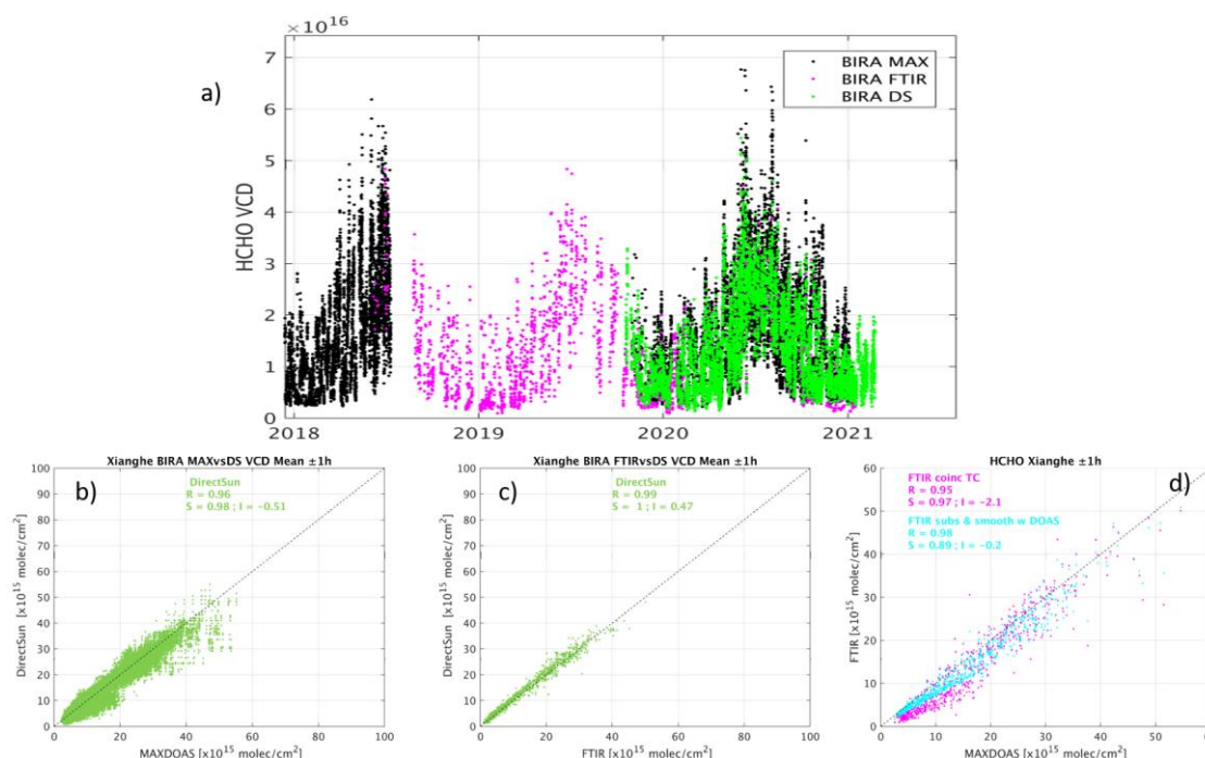
Figure 51: a) Time-series of the MAX-DOAS, FTIR and direct-sun HCHO dataset from BIRA in Xianghe; Scatter-plot between the b) direct-sun and the MAX-DOAS, c) direct-sun and FTIR and d) FTIR and MAX-DOAS for the raw comparisons and when taking into account a-priori profile substitution and smoothing.
