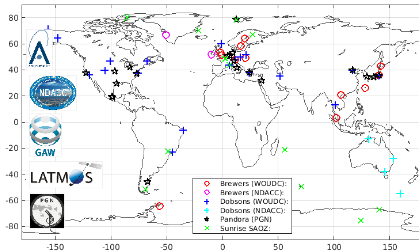
Figure 3: Geographical distribution of Brewer, Dobson, Pandora, and ZSL-DOAS ground-based stations for which co-locations with S5P L2_O3 OFFL ozone data have been used (period up to August 2023).
