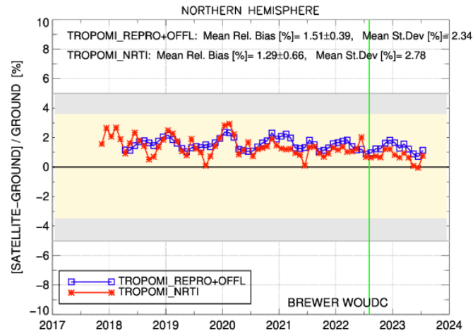
Figure 6: Time series of the monthly mean difference for the comparisons against Brewers in the Northern hemisphere for both the RPRO+OFFL product (blue) and the NRTI product (red). The green line denotes the switch to processor version 2.4.1. For the OFFL data, earlier data are reprocessed with v2.4.1, for NRTI, these data correspond to earlier processors.
