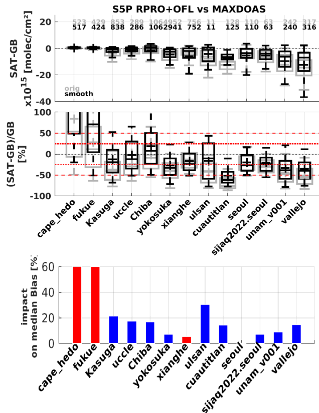
Figure 35: Box-and-whisker plots summarizing the bias and spread of the difference between S5P TROPOMI RPRO+OFFL v2.4 and MAX-DOAS NO 2 tropospheric columns (grey) and the smoothed MAX-DOAS NO 2 tropospheric columns (black). The third panel presents bar plot summarizing the change on the median bias between the original comparisons and the smoothed ones. Absolute values of the relative median biases are shown, where reductions are marked in blue bars and increases in red bars. The time frame is for all available data from May 2018 until February 2023. The median difference is represented by a vertical solid line inside the box, which marks the 25 and 75% quantiles. The whiskers cover the 9-91% range of the differences and the crosses denotes the mean differences.
