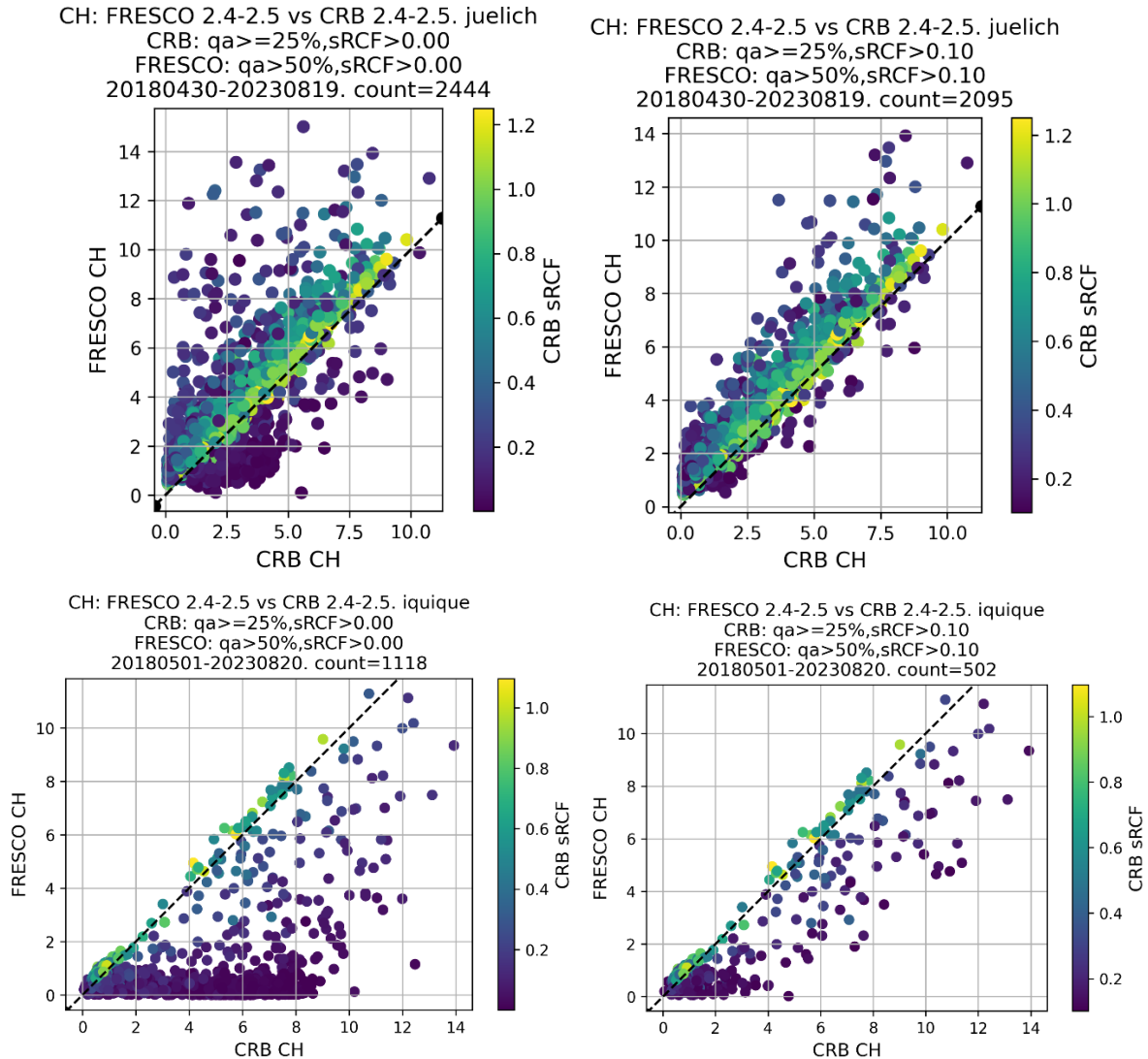
Figure 104. Scatter plot between FRESKO and CLOUD CRB cloud height, with points colored according to CRB sRCF, for the sites Juelich and Iquique, and for two screening settings: sRCF>0. For both CRB and FRESKO, and sRCF>0.1 (which is the default to calculate bias and dispersion).
