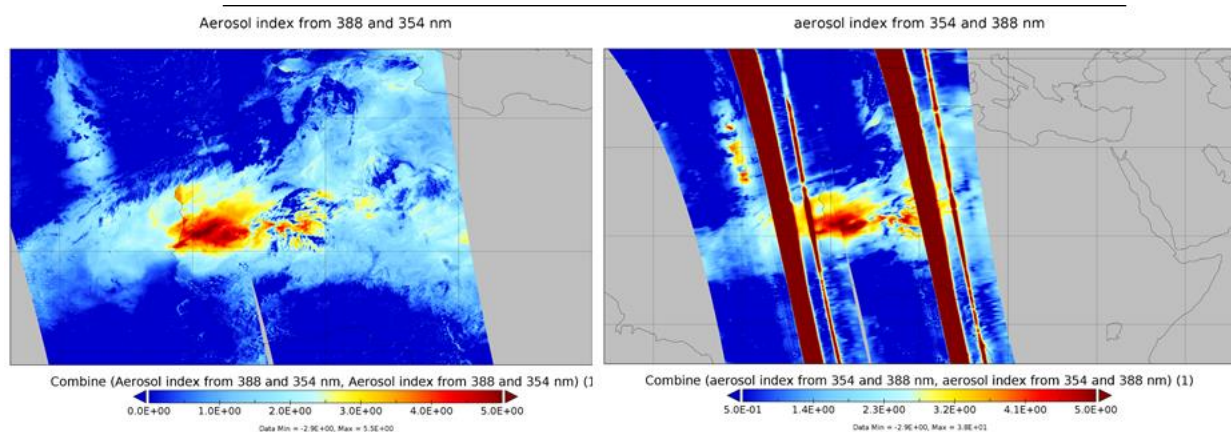
Figure 105: Comparison of S5P TROPOMI RPRO UVAI (orbits 24007 & 24008, left) and OMI OMAERO UV Aerosol Index (orbits 95097 & 95098, right) for Saharan dust on 1 June 2022. In general very good agreement is found (the stripes in north-south direction in the OMI data are caused by the OMI row anomaly and should be ignored).
