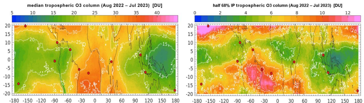
Figure 20: Median value (left) and half-width of 68% interpercentile (right) of S5P OFFL tropospheric ozone column data (CCD) over the last year of operations (Aug. 2022 – Jul. 2023). Red markers locate the eleven ground-based ozonesonde stations used in the validation analysis.
