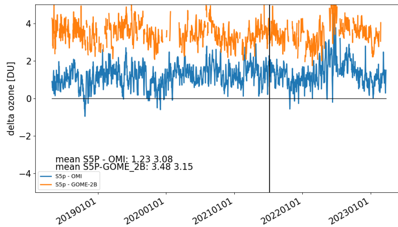
Figure 23: Difference time series of daily tropospheric O 3 column data averaged over the 20°S – 20°N tropical belt. S5P RPRO+OFFL CCD data are compared to OMI (blue) and GOME-2B (orange) satellite data; positive values indicate a high bias of S5P w.r.t. the reference. The black vertical line indicates the transition from the RPRO to OFFL data files (see Table 1 ).
