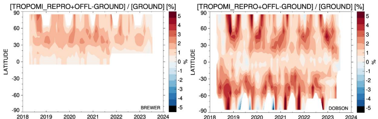
Figure 7: Time and latitude resolved analysis of the differences between RPRO+OFFL total ozone and Brewer measurements (left-hand panel) and Dobson measurements (right-hand panel). Strong seasonal features in the Dobson comparisons are partly due to the use of a fixed effective temperature in the Dobson measurement processing.
