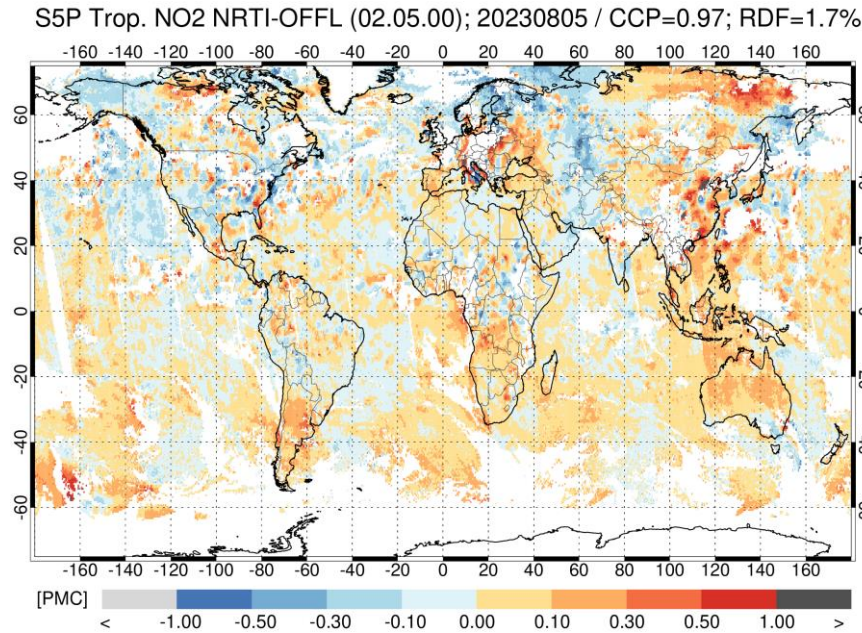
Figure 48: Difference between S5P NRTI and OFFL V2.5.0 daily tropospheric NO 2 column data (binned to 0.5°x0.5° resolution) for 2023/08/05. The difference is calculated for columns > 0.5 Pmolec/cm 2 , cloud fractions < 0.2 and a qa_value > 0.75.
