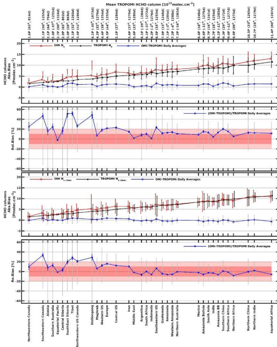
Figure 59: Absolute and relative biases between OMI and TROPOMI HCHO daily averaged tropospheric columns using cloud corrected AMF ( N_v , two upper panels) or clear sky AMF ( N_{v\_clear} , two bottom panels) for the large regions represented on Figure 55. Regions are sorted as a function of the median TROPOMI HCHO column. Values of the averaged HCHO columns are provided on the top axis, as well as the numbers of common days taken for the comparison and the latitude of the region. The median OMI (red) and TROPOMI (black) columns are plotted together with the absolute differences (in blue). Error bars represent the median deviations of the columns, or the median absolute deviations of the differences (in grey). Pink areas indicate 10 % and 20 % bias.
