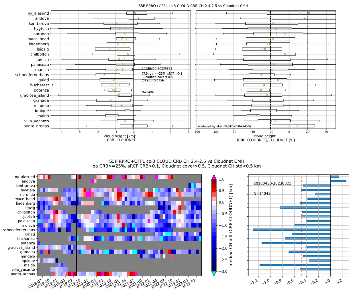
Figure 100: Upper panel: Boxplots of S5P L2_CLOUD CRB RPRO+OFFL CH minus CLOUDNET CH (upper left) and of the relative difference (upper right), per station. The same conventions as for Table 17 apply. Sensing time range is indicated on the figure. Bottom left panel: monthly median of CLOUD CRB CH-CLOUDNET CMH, per station. Pixel size switch (2019/08/06) is indicated on the plot. Bottom right panel: median difference per station. The dashed red line indicates the median over the median differences.
