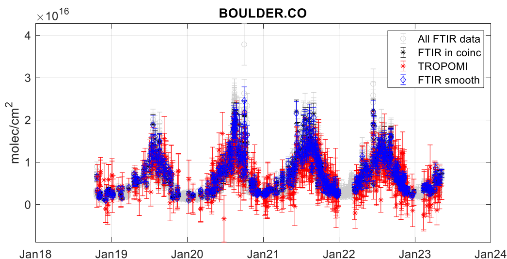
Figure 60: TROPOMI and FTIR HCHO time series at Boulder. Time frame is May 2018 to May 2023.
