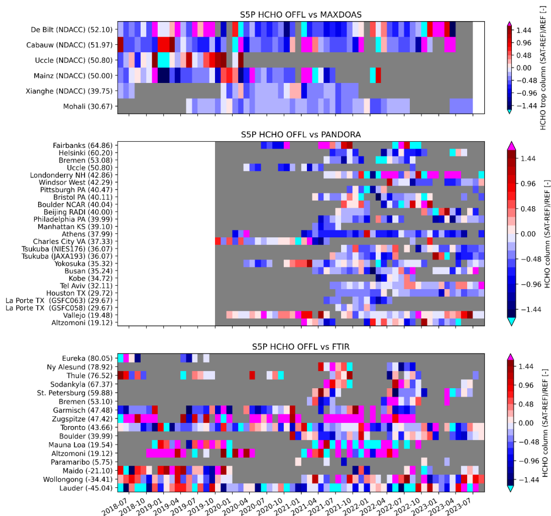
Figure 52: Time series of monthly mean relative differences [%] of S5P OFFL/RPRO V02.04.01-02.05.00 HCHO versus MAXDOAS, PANDORA, and FTIR. Time frame is May 2018 to August 2023. Data was obtained from the VDAF Automated Validation Server on 2023/08/25.
