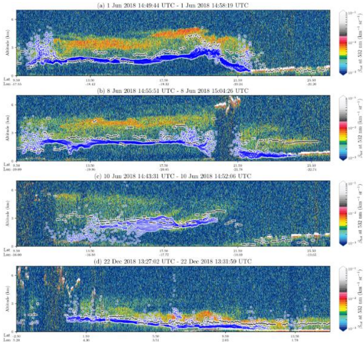
Figure 113: Curtain plots from CALIOP, showing the total attenuated backscatter at 532 nm for the four cases in Figure 112 . Plotted on top of the coloured background image of the total attenuated backscatter are the weighted extinction heights as derived from the backscatter coefficient in black-and-white, and the ALH (processor version before v02.05.00) from collocated TROPOMI pixels in blue-and-white.
