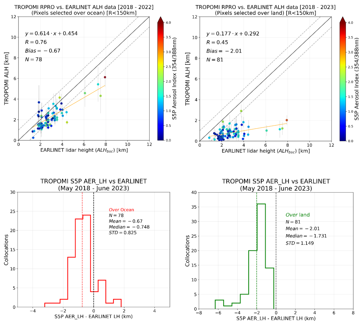
Figure 119: Top: Scatterplots of TROPOMI ALH (v02.04.00) against EARLINET data. TROPOMI pixels over ocean (left) and land (right). Also plotted on each panel are the one-to-one line (solid) and \pm 1.0 km (dashed) envelopes, the number of samples (N), bias and Pearson coefficient (R). The colour of each scatter point indicates TROPOMI retrieved UVAI (388/354nm) values, while the vertical error bars indicate the standard deviation of the spatial average of the TROPOMI ALH pixels. Co-locations cover the period from May 2018 to April 2023. EARLINET weighted extinction height is consistently lower than TROPOMI ALH. Bottom: Histogram of the differences between TROPOMI and EARLINET data sets, shown in red over the ocean pixels (left) and green for land (right) pixels.
