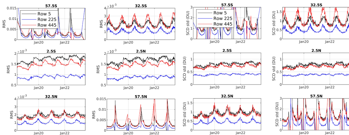
Figure 74: Temporal evolution of the measurement error (left) and the standard deviation (right) for selected 5° latitude bands and 3 detector rows from December 2018 to August 2023. Good qualitative agreement between both quantities is found indicating that the random uncertainty is well characterized by the measurement error. Larger errors (and standard deviations) are found at the edges of the detector and towards high latitudes. The jump in the RMS and standard deviations in low and mid-latitudes in August 2019 are caused by the reduction of the ground pixel size. Courtesy of N. Theys (BIRA-IASB).
