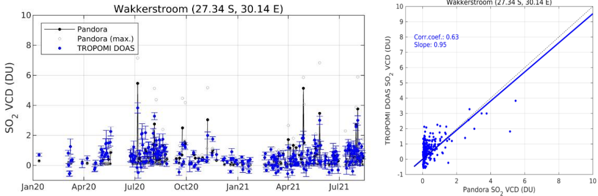
Figure 73: Comparison of TROPOMI SO 2 VCDs to preliminary Pandora measurements (daily means) at Wakkerstroom (South Afrika) from January 2020 to August 2021. The following selection criteria were applied: distance < 25km, CF<0.2, time window +/- 1h around overpass. Courtesy of N. Theys (BIRA-IASB), Martin Tiefengraber and Alexander Cede (Luftblick). Pandora data are still in demonstration phase.
