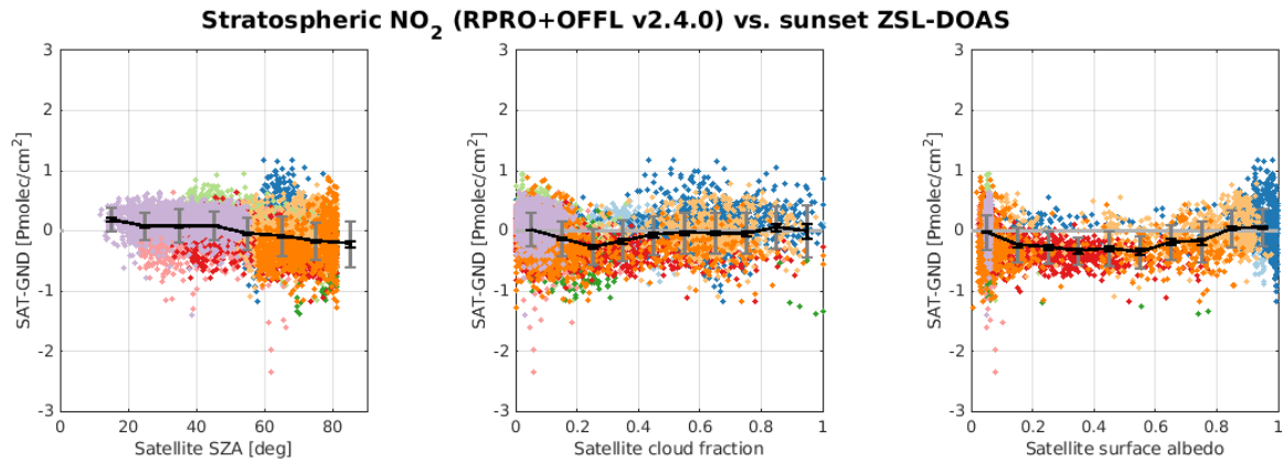
Figure 44: Difference between S5P L2_NO2 RPRO+OFFL and ground-based SAOZ stratospheric NO 2 columns as a function of the satellite solar zenith angle (SZA), satellite cloud fraction, and satellite surface albedo. Mean and standard deviation are calculated over bin widths of 10° degrees in SZA, 0.1 in CF, and 0.1 in surface albedo (solid black line and grey bars). Co-locations cover the period from May 2018 to August 2023.
