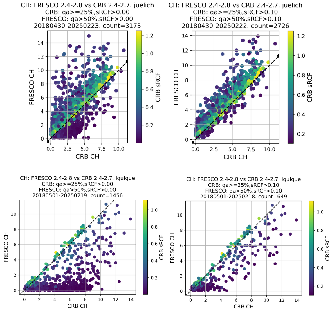
Figure 117. Scatter plot between FRESKO and CLOUD CRB cloud height, with points colored according to CRB sRCF, for the sites Juelich and Iquique, and for two screening settings: sRCF > 0. For both CRB and FRESKO, and sRCF > 0.1 (which is the default to calculate bias and dispersion).
