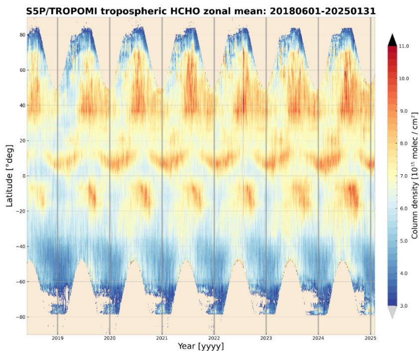
Figure 70: S5P TROPOMI HCHO column data [ 10^{15} molec/ \text{cm}^2 ] as a function of day and latitude. The period is June 2018 to January 2025 (V02.07.00). Grid box size in latitude direction is 0.5^\circ . The grey vertical lines mark the processor version changes, the black lines the beginning of each year.
