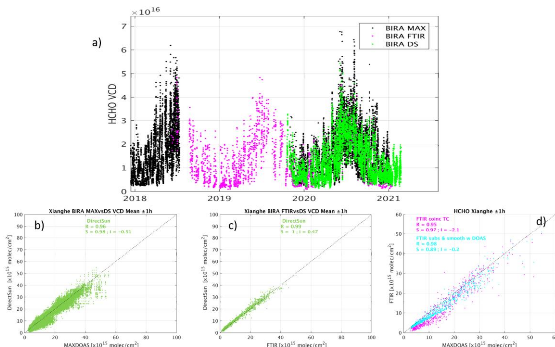
Figure 55: a) Time-series of the MAX-DOAS, FTIR and direct-sun HCHO columns in Xianghe from BIRA-IASB instruments; Scatter-plot between the b) direct-sun and the MAX-DOAS, c) direct-sun and FTIR and d) FTIR and MAX-DOAS for the raw comparisons and when taking into account a-priori profile substitution and smoothing.
