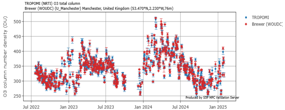
Figure 18: Time series of S5P TROPOMI NRTI (v2.4.1 and higher) and Brewer total ozone data at the station of Manchester in the United Kingdom (data courtesy J. Rimmer, University of Manchester).
