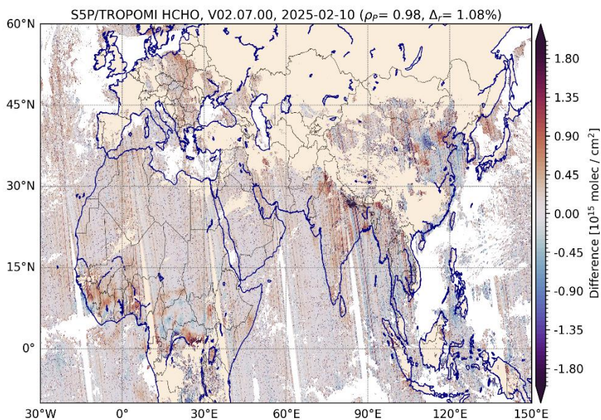
Figure 72: Difference between HCHO (V02.07.00) NRTI and OFFL column data for 2025/02/10 (binned to 0.1^\circ \times 0.1^\circ resolution). The difference is only calculated for columns above 0.5 \text{ Pmolec/cm}^2 and a q_a value above 0.5.
