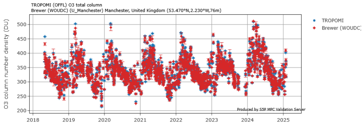
Figure 11: Time series of S5P TROPOMI OFFL and Brewer total ozone data at the station of Manchester in the United Kingdom (data courtesy J. Rimmer, University of Manchester).
