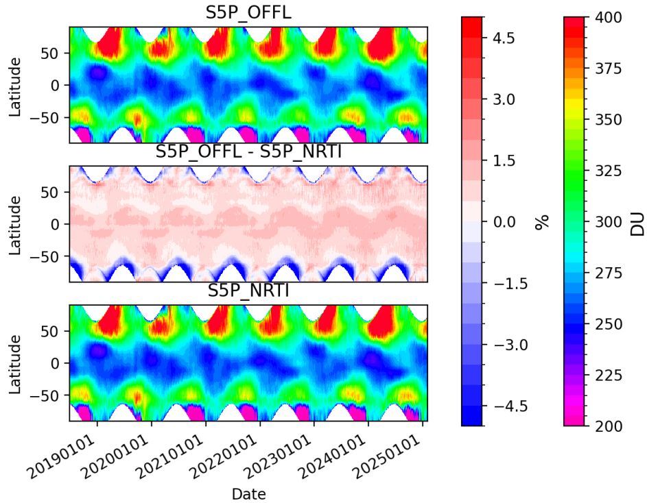
Figure 19: Time series of (the differences between) the zonal mean gridded (level-3) OFFL and NRTI total ozone column data sets.
