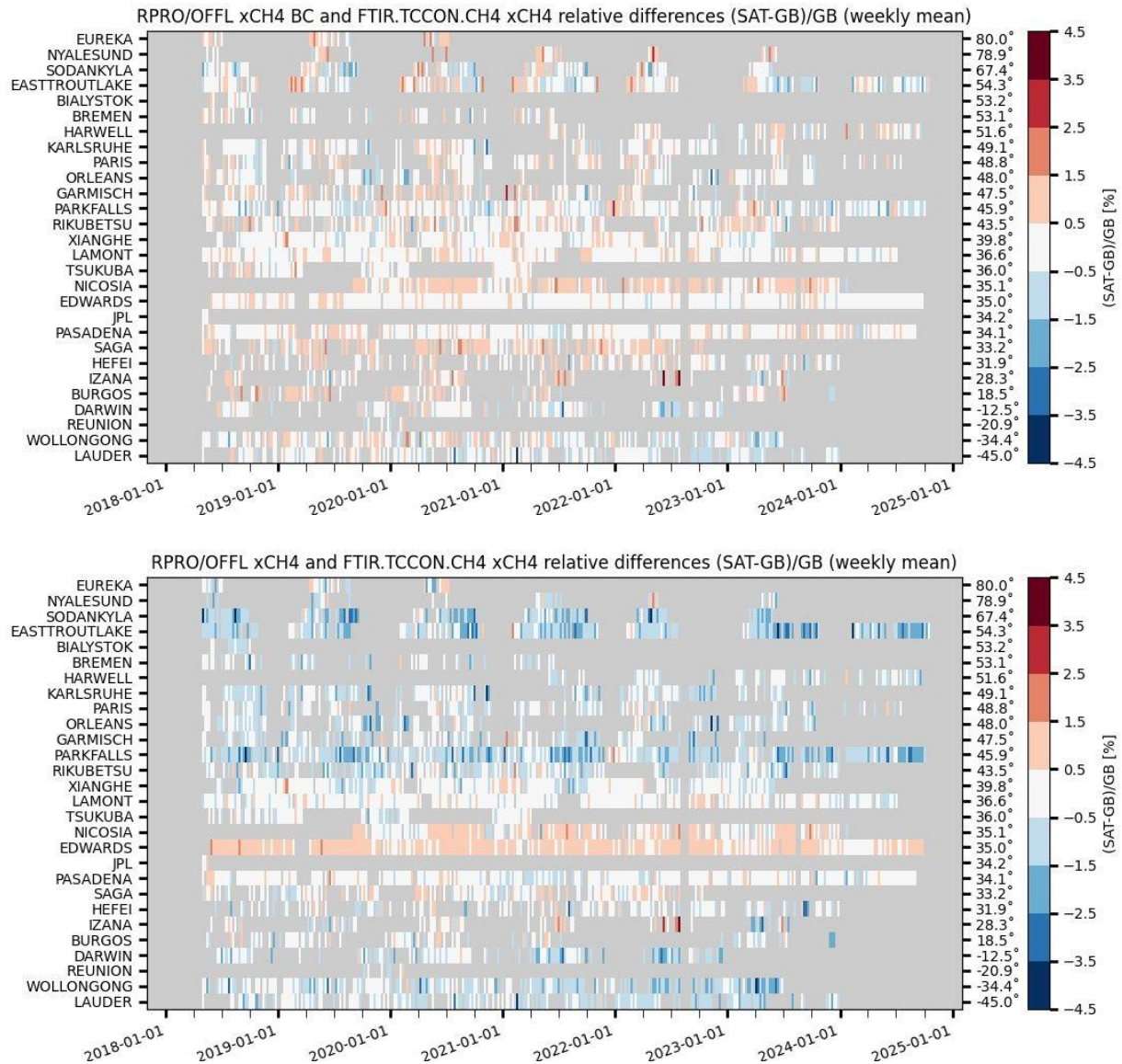
Figure 95: Mosaic plots of relative biases between S5P L2_CH4 RPRO+OFFL and ground-based CH4 TCCON column data for the bias corrected (top) and standard (bottom) methane products. Over the April 2018 – January 2025 period the plots do not show a clear meridian dependence or temporal change in the weekly averaged biases. Colour bar gradients are chosen such that they match with the measurement's uncertainties.
