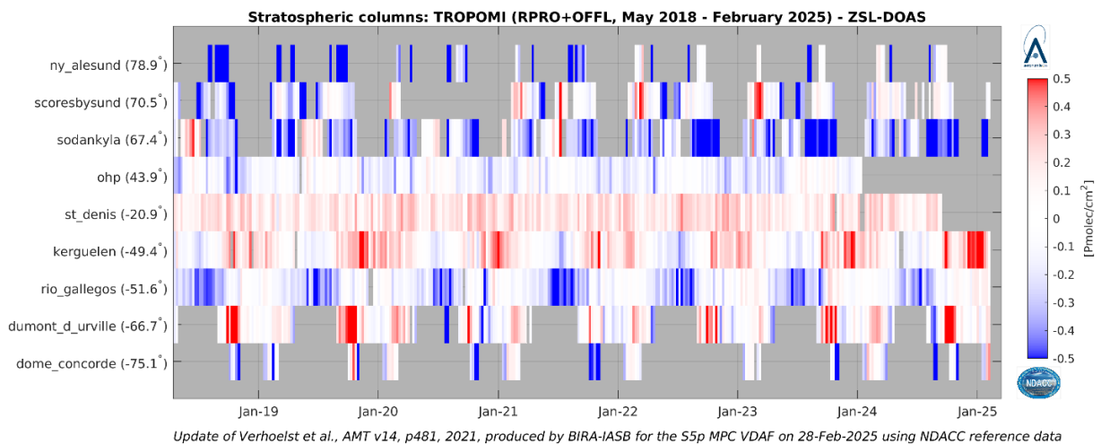
Figure 43: Time series – from May 2018 until February 2025 – of S5P RPRO+OFFL L2_NO 2 and NDACC ZSL-DOAS NO 2 stratospheric column differences, weekly averaged [Pmolec/cm 2 ]. For the current report, only the SAOZ data sets covering the full mission lifetime are shown.
