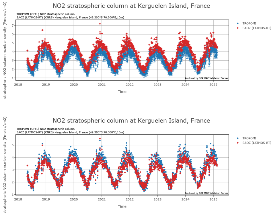
Figure 47: Time series of S5P OFFL L2_NO2 stratospheric NO2 column data (blue dots) co-located with ground-based SAOZ twilight measurements (red dots) at sunset performed by LATMOS at the NDACC southern mid-latitude station of Kerguelen Island. In the upper plot, the photochemical correction is deactivated to offset the two time-series and to better see the day-to-day variability. The time frame is May 2018 to February 2025.
