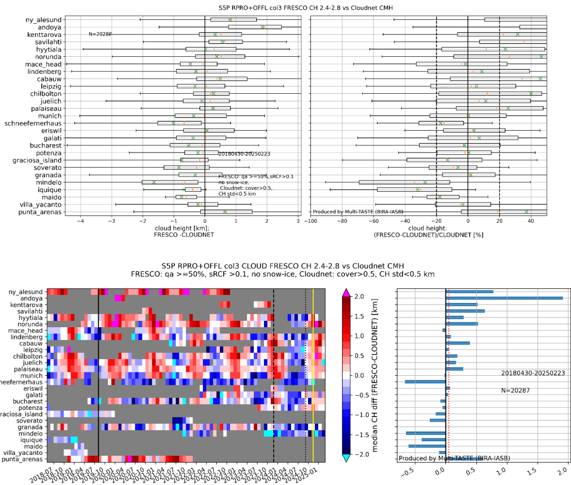
Figure 114: Upper panel: Boxplots of S5P L2_CLOUD FRESCO RPRO+OFFL v1.3-v1.4 CH minus CLOUDNET CH (upper left) and of the relative difference (upper right), per station. The same conventions as for Table 17 apply. Sensing time range is indicated on the figure. Bottom left panel: monthly median of FRESCO CH-CLOUDNET CH, per station. Pixel size switch (2019/08/06) and the following updates: FRESCO v2.6.0 (2023/11/26), FRESCO v2.7.1 (2024/09/11) and FRESCO v2.8.0 (2024/11/16) are indicated on the plot. Bottom right panel: Median difference per station. The red dashed line indicates the median of the median differences.
