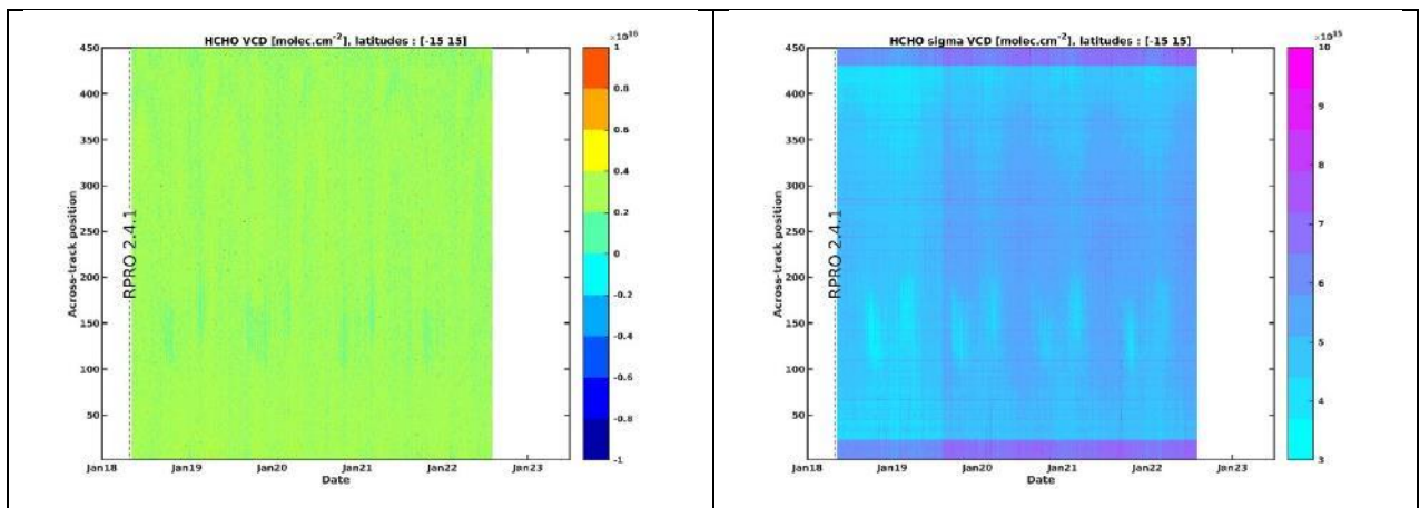
Figure 69: S5P TROPOMI HCHO column data (left) and their standard deviation (right) as a function of day (x-axis) and across-track position (y-axis). Data are averaged in the reference sector (the remote Equatorial Pacific). Results are shown for the reprocessed data collection 3.
