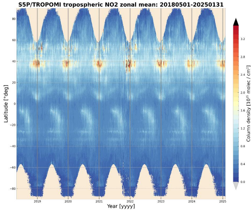
Figure 39: S5P TROPOMI NO 2 tropospheric columns [ 10^{15} molec/cm 2 ] as a function of day and latitude. The period covers six years from May 2018 to January 2025. RPRO/OFFL V02.04.00 and OFFL V02.05.00-02.08.00 data are used. Grid box size in latitude direction is 0.5°. The light grey vertical lines mark the beginning of each year.
