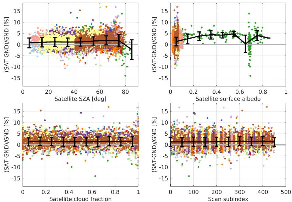
Figure 9: Dependence of the difference between S5P OFFL and ground-based Brewer total ozone data on the solar zenith angle (SZA), the surface albedo, the fractional cloud cover, and the scan sub-index of the satellite measurement. Black curve: mean and standard deviation over bins of 10 degrees of SZA, 0.1 of surface albedo, 0.05 of cloud fraction, and 50 pixels over across-track scan. Coverage of the high SZA and of the surface albedo is poor for these Brewer comparisons, but the SAOZ comparisons (not shown) which offer better coverage for these parameter ranges reveal no anomalies.
