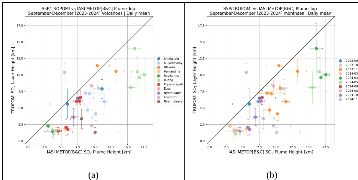
Figure 87. Scatter plots between the daily mean TROPOMI SO 2 layer height observations (y-axis) and combined IASI/Metop-[B&C] observations retrieved during volcanic eruptions of the September 2023 - November 2024 period. (a) Grouped by the volcano; (b) Grouped by the volcano eruption period.
