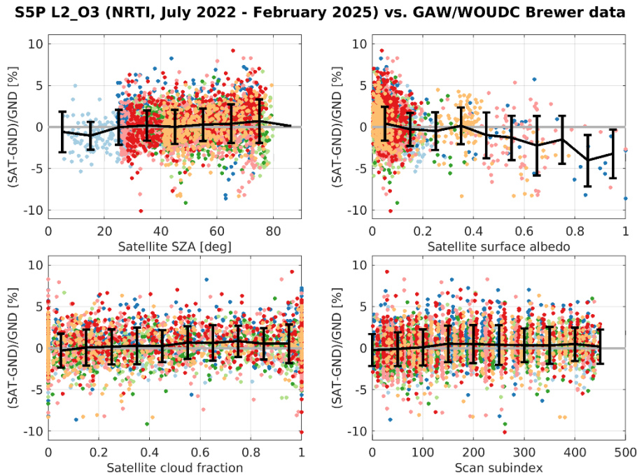
Figure 17: Dependence of the difference between S5P NRTI and ground-based Brewer total ozone data on the solar zenith angle (SZA), the surface albedo, the fractional cloud cover, and the scan sub-index of the satellite measurement. Black curve: mean and standard deviation over bins of 10 degrees of SZA, 0.1 of surface albedo, 0.05 of cloud fraction, and 50 pixels of the across-track scan. Coverage of the high SZA and of the surface albedo is poor for these Brewer comparisons, but the SAOZ comparisons (not shown) which offer better coverage for these parameter ranges reveal no anomalies.
