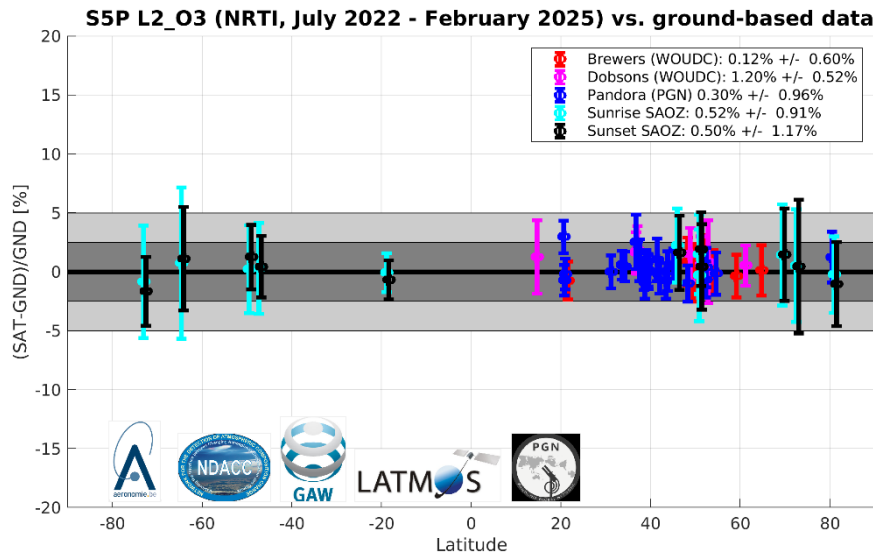
Figure 13: Meridian dependence of the median (the circular markers) and spread ( \pm 1 sigma, the error bars) of the percent relative difference between S5P TROPOMI L2_O3 (PDGS NRTI processors v2.4.1 and above, up to February 2025) and ground-based (GND) ozone column data, represented at individual stations from the Antarctic to the Arctic and per measurement type (Brewer, Dobson, Pandora, and ZSL-DOAS). The values in the legend correspond to the median and spread of all median (per station) differences. For clarity, sunrise and sunset ZSL-DOAS results are represented separately (offset by -0.5^\circ and +0.5^\circ in latitude).
