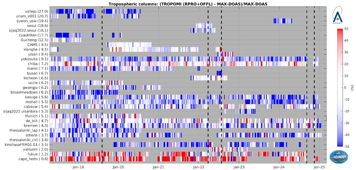
Figure 36: Time series – from May 2018 until end January 2025 – of the weekly averaged relative difference [%] between S5P RPRO+OFFL v02.04/02.05/02.06/02.07/02.08 and MAX-DOAS NO2 tropospheric column data. Stations are ordered by median tropospheric column, in brackets.
