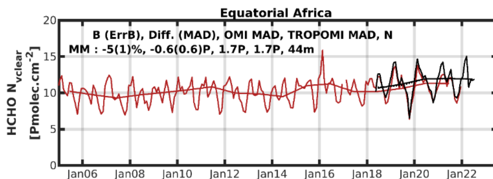
Figure 62: Example of monthly and yearly averaged HCHO columns ( N_{v\_clear} ) retrieved from OMI (October 2004–December 2021, in red) and TROPOMI collection 3 (2018–March 2023, in black) in a large region of equatorial Africa. Absolute and relative biases between OMI and TROPOMI HCHO monthly averaged columns are given at the top, as are the median deviations of the OMI and TROPOMI averaged columns.
