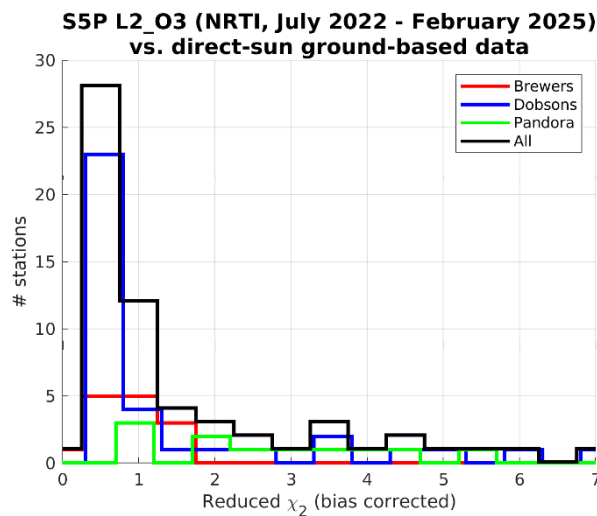
Figure 16: Histogram of the \chi_r^2 values (one per reference instrument) for S5P NRTI total ozone versus different types of ground-based measurements.
