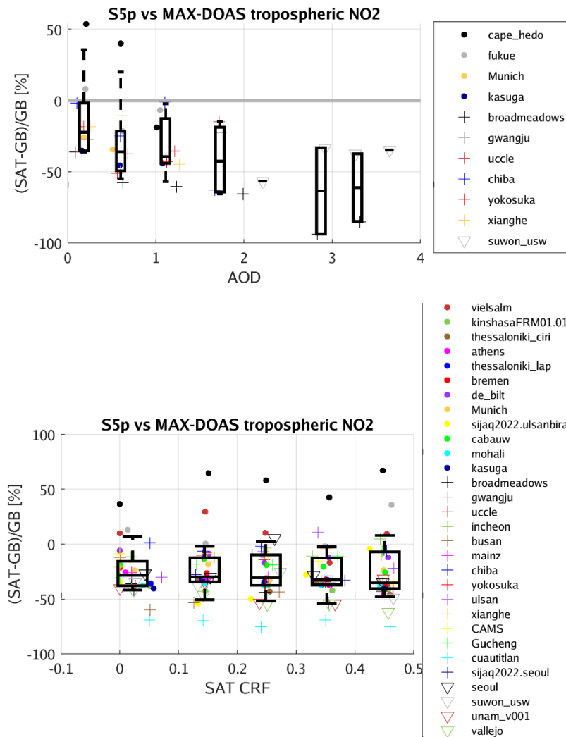
Figure 38: Relative differences between S5p TROPOMI RPRO+OFFL and MAX-DOAS NO 2 tropospheric columns as a function (upper panel) of MAX-DOAS AOD and (lower panel) S5p cloud radiance fraction (CRF). The time frame is from May 2018 until end of December 2024.
