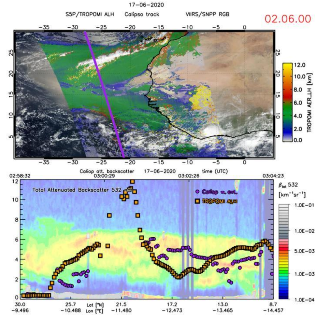
Figure 126: Same as above, but for 17 June 2020.
