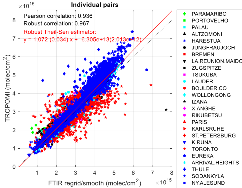
Figure 45: Scatter plot of co-located S5P TROPOMI and NDACC FTIR stratospheric NO 2 column data.
