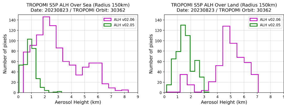
Figure 139: Frequency histograms of TROPOMI ALH retrievals for the version v02.05.00 (green) and v02.06.00 (magenta).
