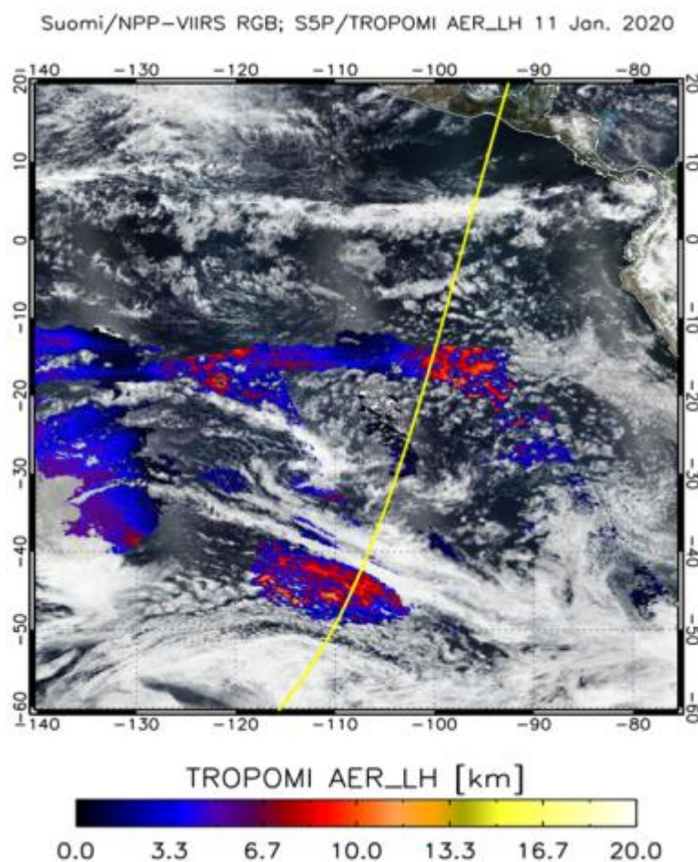
Figure 143: NPP/VIIIRS RGB image with S5P/TROPOMI AER_LH on 11 January over the south Pacific with the CALIPSO track of that day overlaid in yellow.
