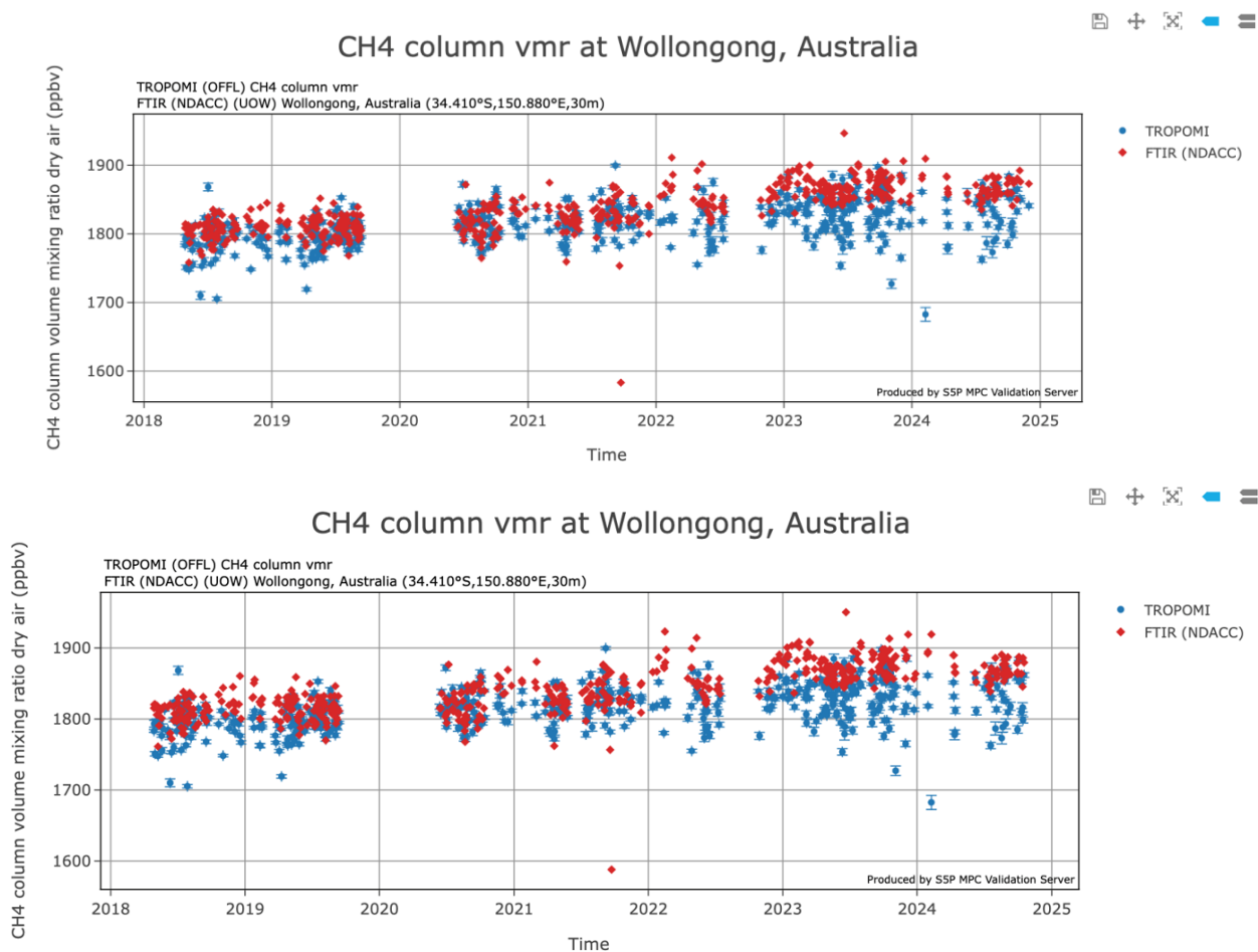
Figure 99: S5P L2_CH4 XCH 4 time series over Wollongong where an increased number of low values of XCH 4 are observed for several days and especially more frequently as of February 2023 onwards.
