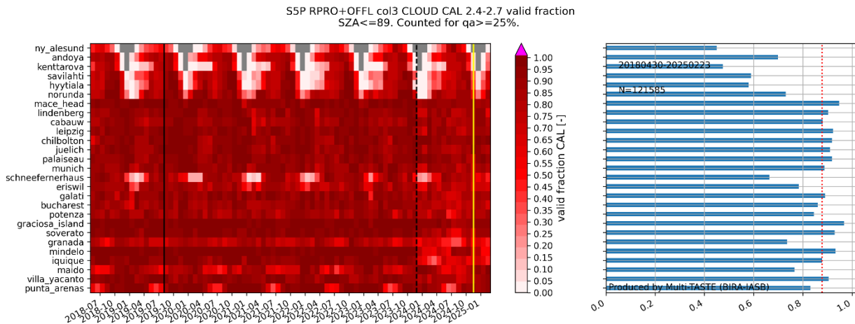
Figure 104: Fraction of valid pixels ( qa\_value \geq 25\% ) for S5P CLOUD CAL. Indicated are the pixel size switch (2019/08/06), the update to CLOUD v2.6.1 (2023/11/26) and the update to CLOUD v2.7.0 (2024/11/16).
