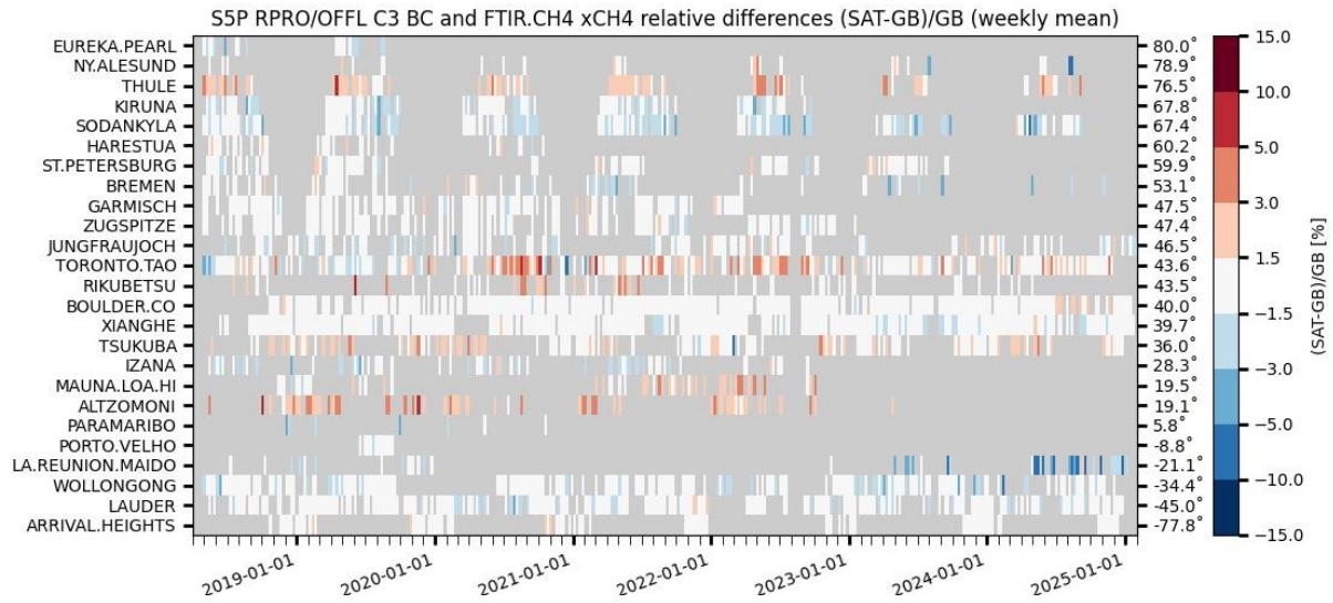
Figure 96 Mosaic plots of relative biases between S5P L2_CH4 RPRO+OFFL and ground-based CH 4 NDACC column data for the bias corrected methane products. Over the April 2018 – January 2025 period the plots do not show a clear meridian dependence or temporal change in the weekly averaged biases. At Maïdo and Wollongong an increased number of negative outliers are observed.
