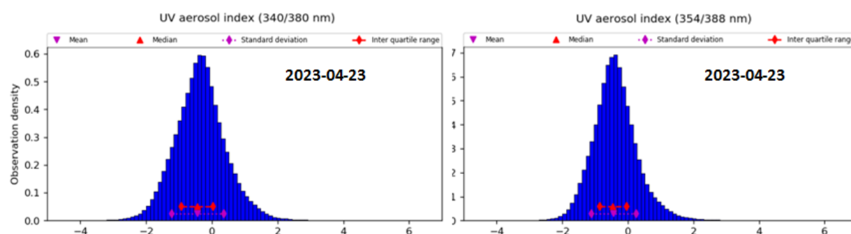
Figure 122: Frequency distribution of the UVAI (left: 340/380nm, right: 354/388 nm) for April 23, 2023.
