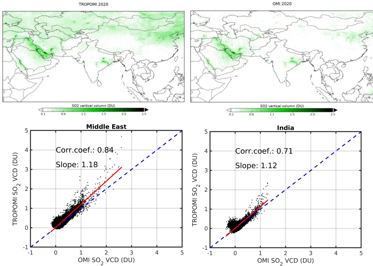
Figure 73: Top: Comparison of the average distribution (01 Jan 2020 – 31 Dec 2020) of the SO 2 VCDs derived from TROPOMI and OMI over regions with strong air pollution. Except high latitudes, both data sets show very good agreement. Bottom: Correlation plots TROPOMI versus OMI over the Middle East and India. Note that a fixed AMF of 0.4 was used for both retrievals to exclude the effect of different profile assumptions. Courtesy of Nicolas Theys, BIRA-IASB.
