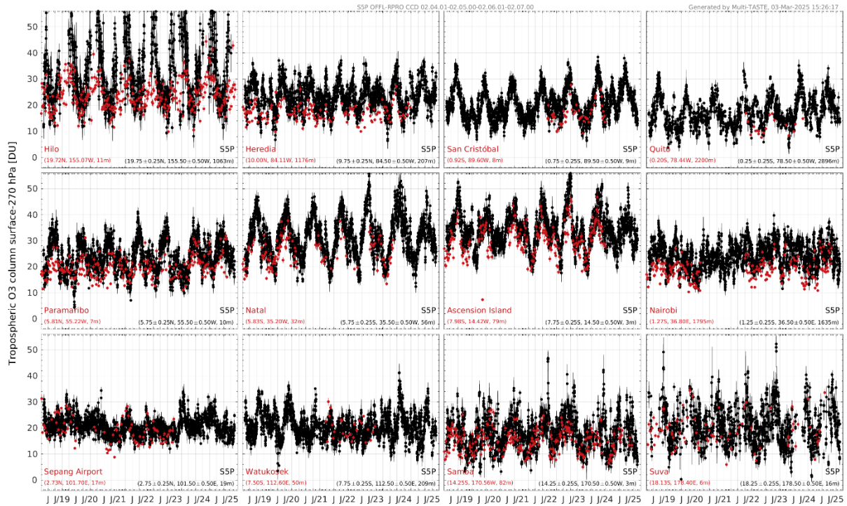
Figure 22: Time series of spatially co-located tropospheric O 3 column data by ozonesonde (red) and by S5P RPRO+OFFL v02.04.01-02.05.00-02.07.00 (black). All data were screened following recommendations by the data providers.
