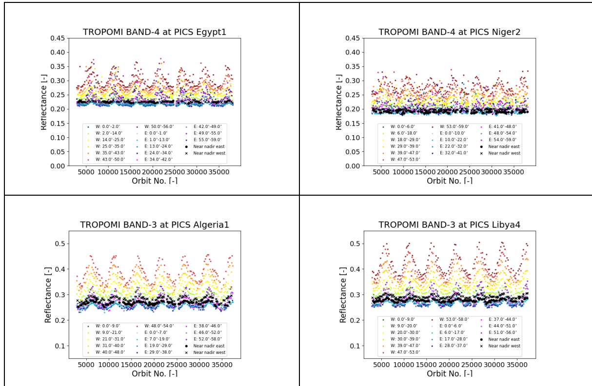
Figure 1: Reflectance derived from L1B v02.01.00 radiance and irradiance data for 436-454nm (band 4) as a function of the orbit number (May 2018 through February 2025) for PICS Egypt-1 and Niger-2 (top panels). The bottom panels show the reflectance for 338-342 nm (band 3) for Algeria-1 (left) and Libya-4 (right). The individual measurements are binned for different viewing angle sectors from 66° West (green and red dots) to 66° East (blue and purple dots).
