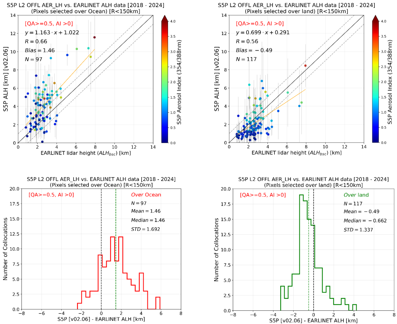
Figure 135: Top: TROPOMI ALH (v02.06.00) against EARLINET data for pixels over ocean (left) and land (right) for the period from May 2018 to August 2024. Colour-scale indicates TROPOMI retrieved UVAI (388/354nm) values, vertical error bars indicate the standard deviation of the spatial average of the TROPOMI ALH pixels. EARLINET weighted extinction height is consistently lower than TROPOMI ALH. Bottom: Histogram of absolute difference between TROPOMI and EARLINET ALHs, shown in red over the ocean pixels (left) and green for land pixels (right).
