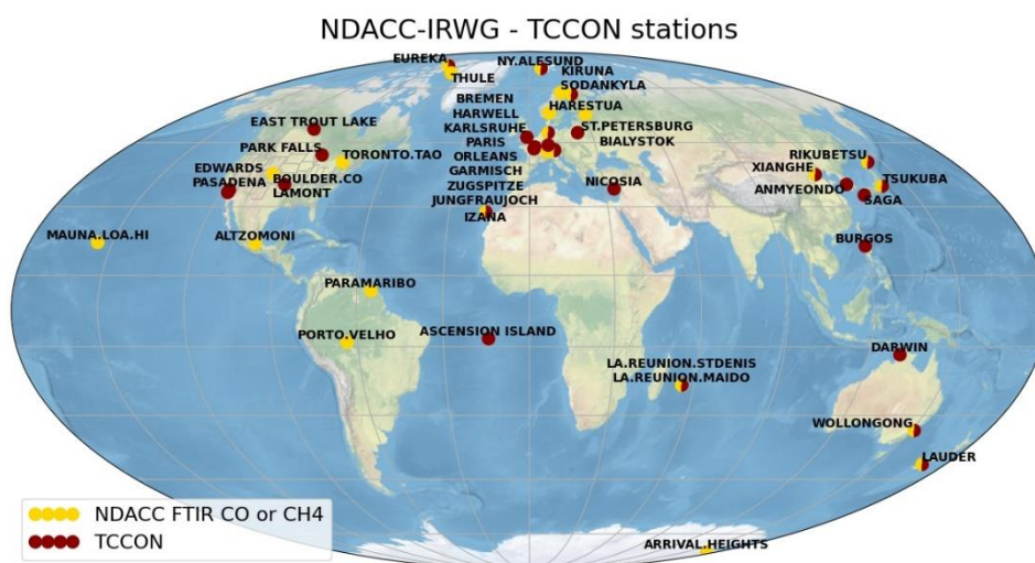
Figure 88: Geographical distribution of NDACC and TCCON FTIR stations measuring atmospheric carbon monoxide column data. Some stations contribute to the two networks.
