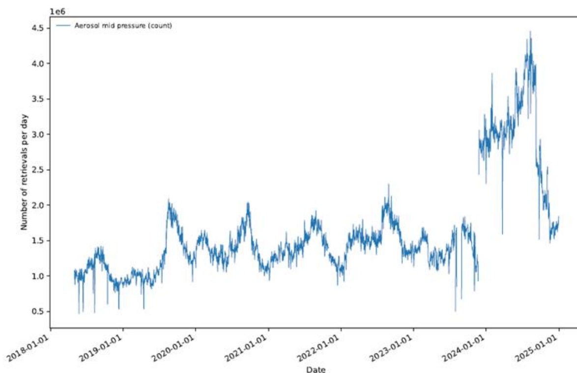
Figure 141: Number of successfully processed ALH pixels per day from June 2018 to February 2025. After the change to version 2.6 in November 2023, the number of successful retrievals increased because more retrievals succeed over land.
