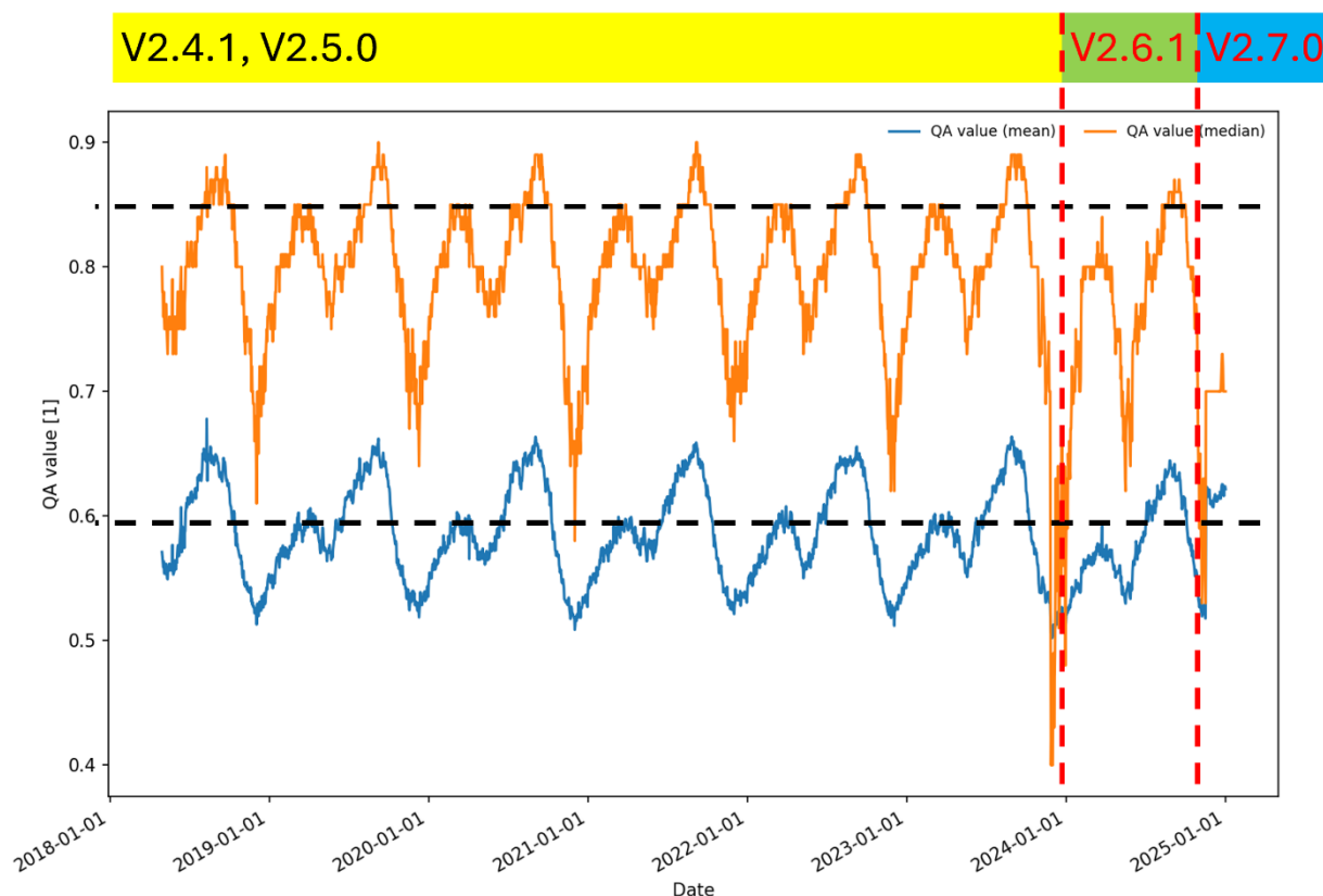
Figure 103. Global mean and median of the OCRAIROCINN_CAL QA value. Time series taken from the L2QC portal, latest update on 2024-12-31. Dashed lines are guide to the eye.
