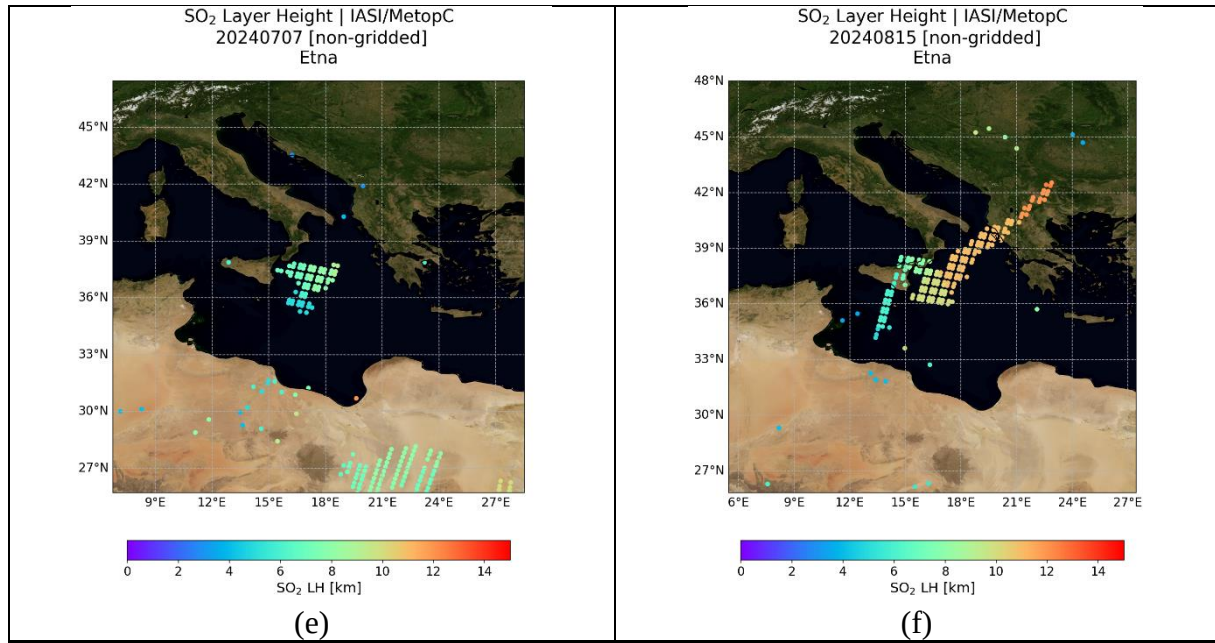
Figure 83. SO 2 layer height [km] during the Etna eruption on July 7 [lef] and August 15 [right], 2024, as sensed by (a, b) TROPOMI; (c, d) IASI/MetOp-B; (e, f) IASI/MetOp-C.
