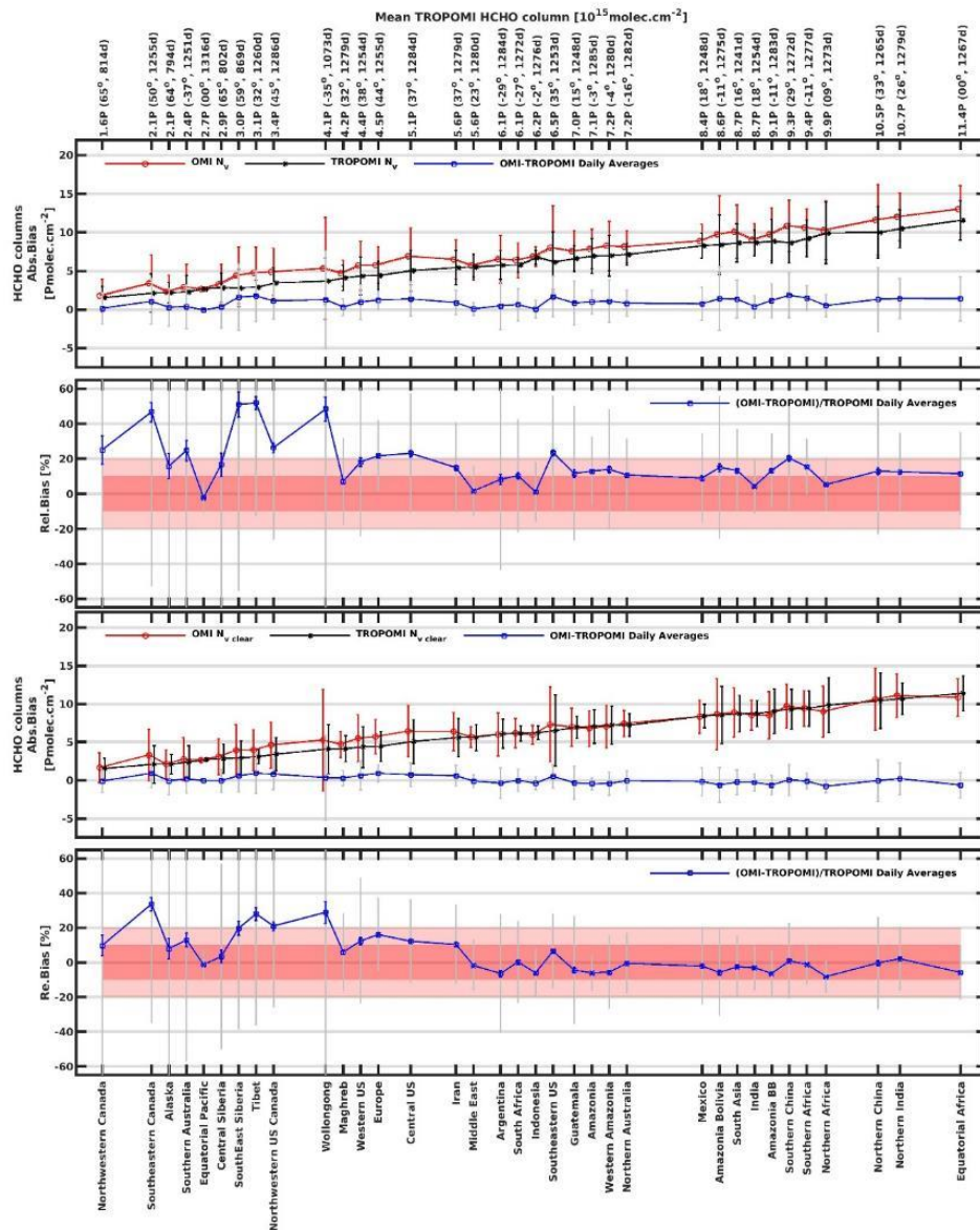
Figure 63: Absolute and relative biases between OMI and TROPOMI HCHO daily averaged tropospheric columns using cloud corrected AMF ( N_v , two upper panels) or clear sky AMF ( N_{v\_clear} , two bottom panels) for the large regions represented on Figure 55 . Regions are sorted as a function of the median TROPOMI HCHO column. Values of the averaged HCHO columns are provided on the top axis, as well as the numbers of common days taken for the comparison and the latitude of the region. The median OMI (red) and TROPOMI (black) columns are plotted together with the absolute differences (in blue). Error bars represent the median deviations of the columns, or the median absolute deviations of the differences (in grey). Pink areas indicate 10 % and 20 % bias.
