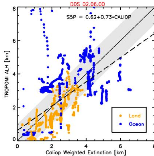
Figure 129: Comparison of ALH from TROPOMI and CALIOP weighted extinction height for the cases presented. Pixels over land are plotted in orange and pixels over water in blue.
