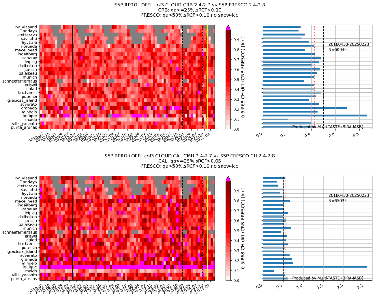
Figure 115: Top. Left: Monthly \frac{1}{2} IP68 of the cloud height difference of CLOUD CRB OFFL vs FRESCO OFFL, per month and per station. Indicated are the pixel size switch (2019/08/06) and the following updates: CLOUD v2.6.1 & FRESCO v2.6.0 (2023/11/26), FRESCO v2.7.1 (2024/09/11) and CLOUD v2.7.0 & FRESCO v2.8.0 (2024/11/16). Right: \frac{1}{2} IP68 of S5P CLOUD CRB CH minus S5P FRESCO CH. Sensing date range is indicated on the figure. Bottom. Similar but for CLOUD CAL CMH vs FRESCO CH.
