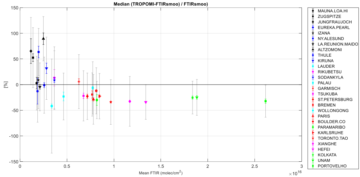
Figure 57: Percent bias between S5P L2_HCHO and NDACC FTIR HCHO column data at each station as a function of the mean FTIR total column ( 10^{16} molec/cm 2 ). The grey bars are the systematic uncertainty on the difference, and the coloured error bars are the 2- \sigma errors on the bias. The temporal range is May 2018 to January 2025 (updated from Vigouroux et al. (2020), Fig. 3).
