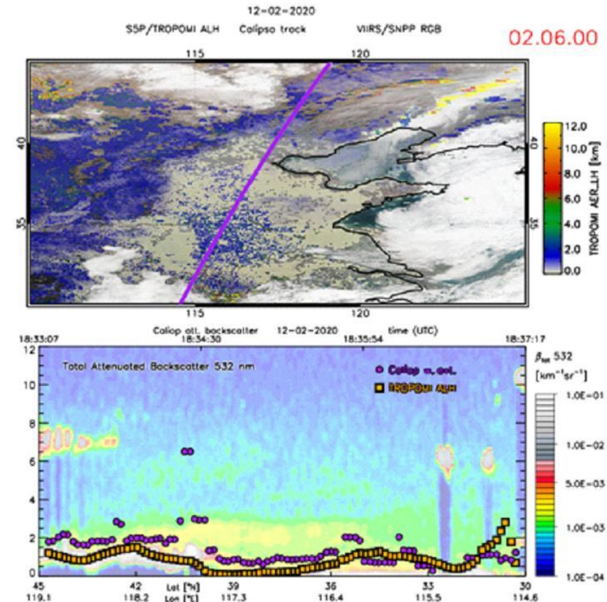
Figure 128: ALH for pollution over China on 12 February 2020 retrieved by TROPOMI (top panel) and the CALIOP total attenuated backscatter image (bottom panel). The purple line and dots show the CALIPSO track and CALIOP weighted extinction averaged along the track, respectively. In the bottom panel the ALH retrieved by TROPOMI along the CALIOP orbit track is shown by the orange squares.
