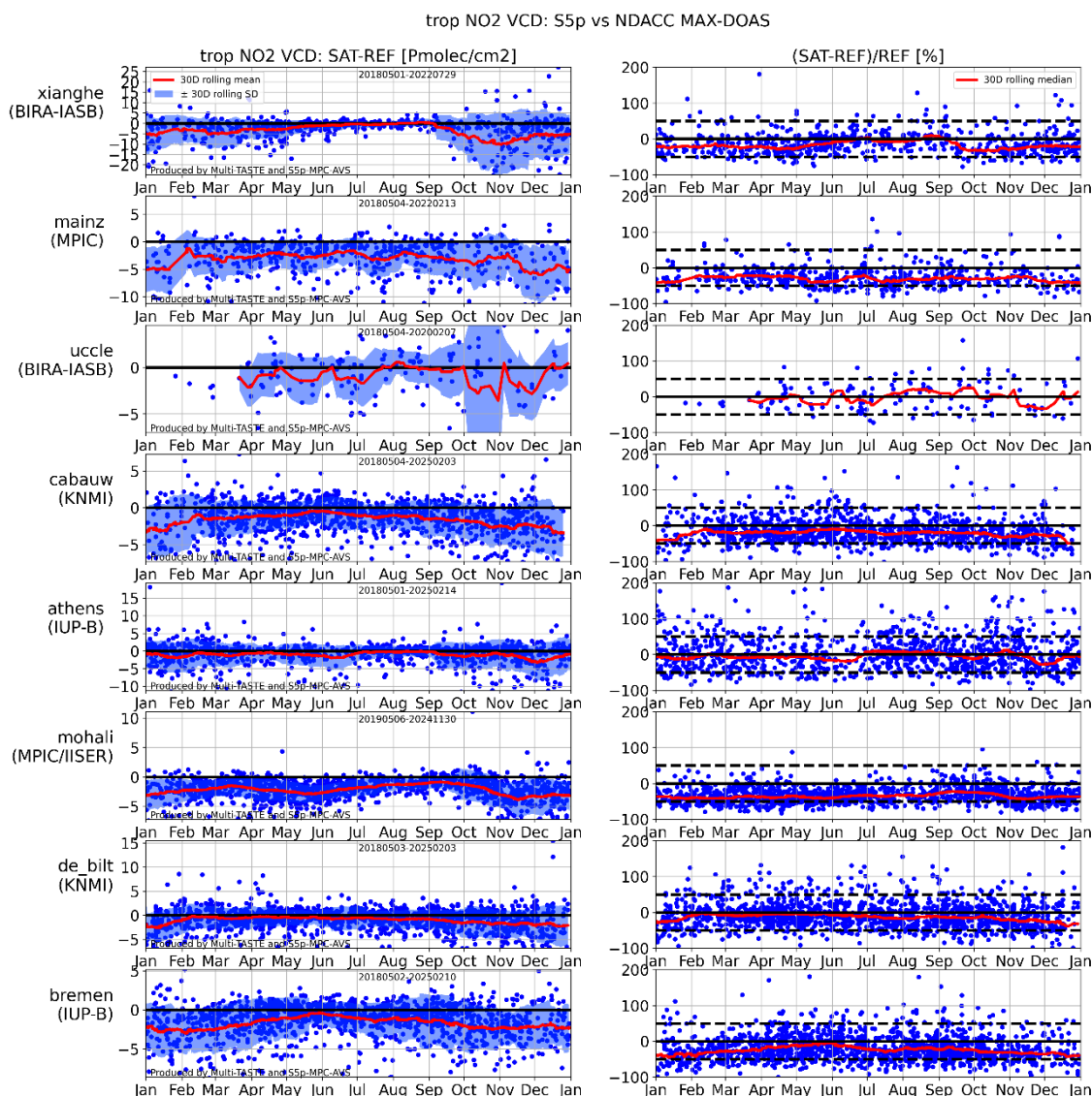
Figure 40: Seasonal cycle (with data mapped to one generic year) of the difference between S5P RPRO+OFFL and MAX-DOAS NO 2 tropospheric column data at eight stations. Difference (left) and relative difference (right). On the left column, the lowest 2.5 % data is not shown for visibility. Data was obtained from the VDAF Automated Validation Server on 2025/02/26.
