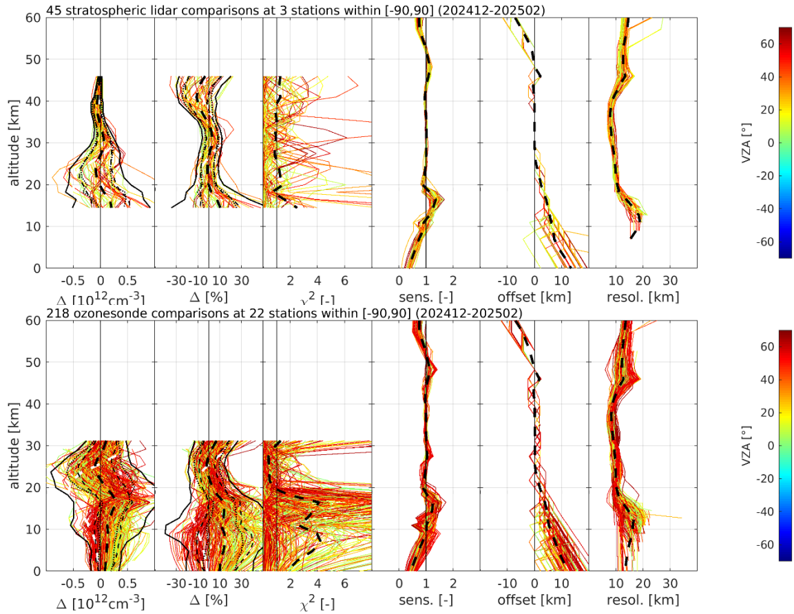
Figure 31: Comparison between S5P L2_O3_PR RPRO/OFFL ozone number density profile data and all co-located ground-based reference measurements, originating from stratospheric lidar (top) and ozonesondes for L2 v02.08 (bottom). Every plate shows six graphs, respectively, from left to right: the difference and the percent relative difference between S5P and reference data, the chi-square profile, the vertical sensitivity, the altitude registration offset, and the averaging kernel FWHM associated with the S5P retrieval. The colour scale indicates the TROPOMI viewing zenith angle (VZA). Black dashed lines show mean values (thick lines) and standard deviations (thin lines, around the mean), while white, dashed lines indicate the mean difference between the a-priori profile and the reference measurement. Dotted black lines indicate the total ex-ante (inductive) uncertainty of TROPOMI and the reference measurements combined (around the mean difference).
