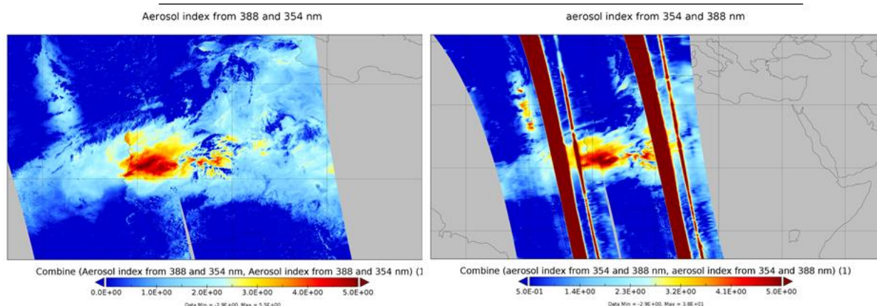
Figure 118: Comparison of S5P TROPOMI RPRO UVAI (orbits 24007 & 24008, left) and OMI OMAERO UV Aerosol Index (orbits 95097 & 95098, right) for Saharan dust on 1 June 2022. In general very good agreement is found (the stripes in north-south direction in the OMI data are caused by the OMI row anomaly and should be ignored).
