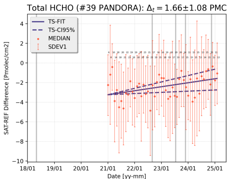
Figure 71: Time series – from January 2021 until January 2025 – of S5P RPRO+OFFL and PGN Pandora HCHO column differences, monthly averaged over all station [Pmolec/cm 2 ]. The number of stations is superimposed. Vertical grey lines show the version changes. Blue lines show the Theil-Sen regression slope and 95% confidence interval.
