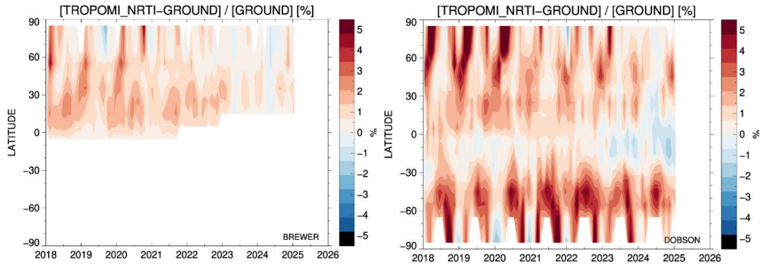
Figure 15: Time and latitude resolved analysis of the differences between NRTI total ozone and Brewer measurements (left-hand panel) and Dobson measurements (right-hand panel). Strong seasonal features in the Dobson comparisons are due (1) to the use of a fixed effective temperature in the Dobson measurement processing, and (2) due to the poorer representation of difficult surface albedo conditions before the adoption of the GE_LER surface albedo product in July 2020.
