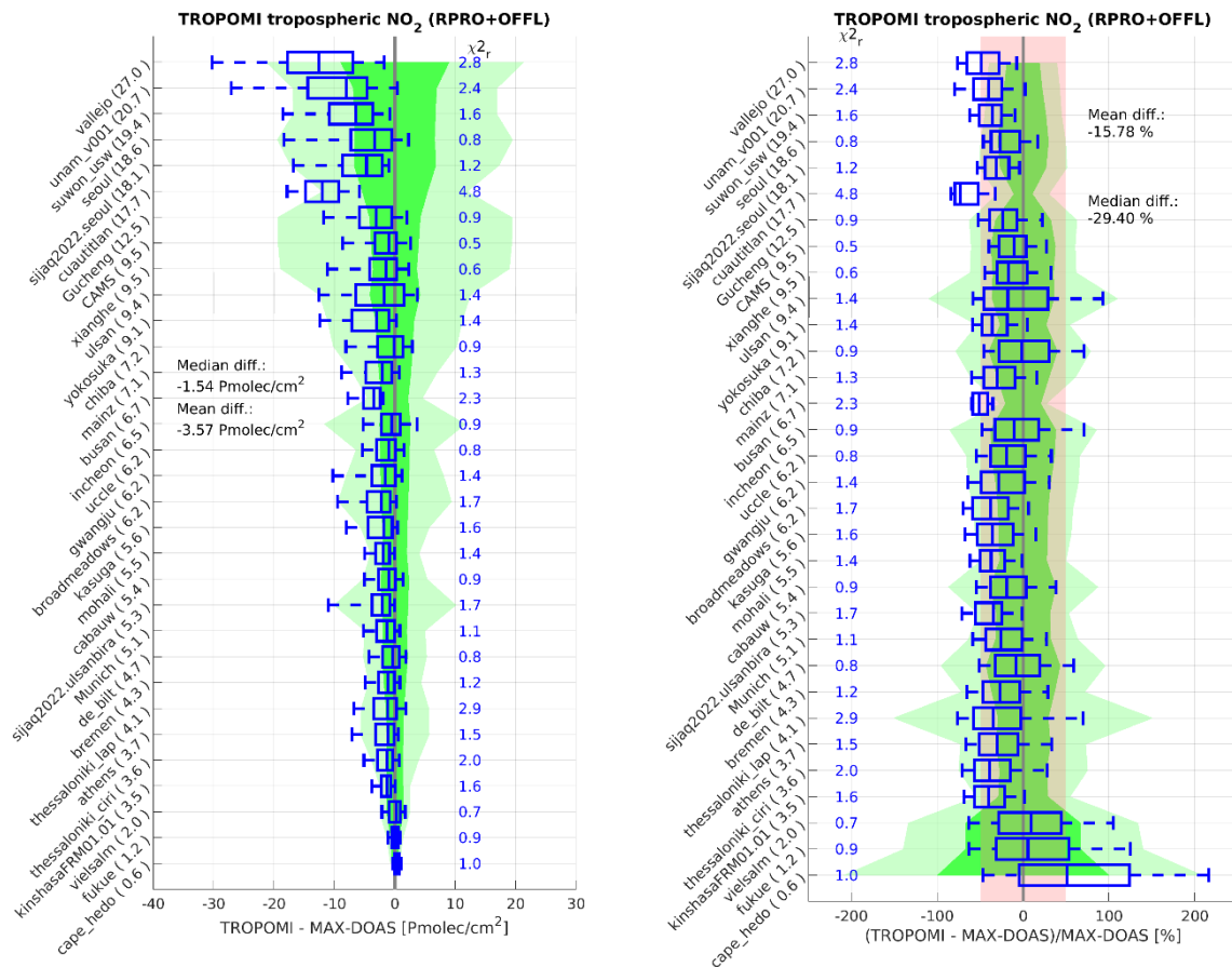
Figure 35: Box-and-whisker plots summarizing the bias and spread of the difference between S5P TROPOMI RPRO+OFFL v02.04/02.05/02.06/02.07/02.08 and MAX-DOAS NO 2 tropospheric columns (left: absolute, right: relative). Values between brackets in the labels denote the median tropospheric column at the station. The time
