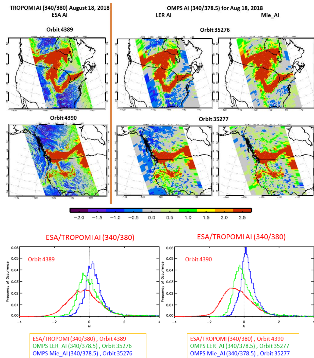
Figure 119: Comparison of UVAI from TROPOMI and OMPS for an observation of a biomass burning plume (18 Aug. 2018). For OMPS UVAI are calculated assuming either LER or Mie clouds. The UVAI for Mie clouds yields results that are more consistent. TROPOMI and OMPS LER results show very good agreement. However, the frequency distribution is broader for TROPOMI observations (courtesy of Omar Torres and Changwoo Ahn, NASA-GSFC).
