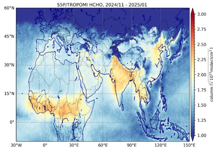
Figure 68: S5P RPRO/OFFL HCHO [-10°S, 60°N, -30°W, 150°E]. The data is binned on a grid of 0.1° latitude/longitude for Nov-Jan 2024/25. A qa\_value > 0.5 and a cloud fraction CF < 0.9 are use. Columns are shown as the third root of values to better cover the dynamics.
