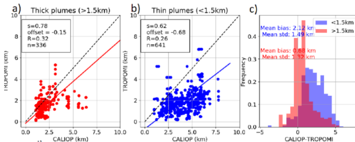
Figure 133: Comparison of TROPOMI ALH (processor version before v02.05.00) and CALIOP average aerosol layer height (top minus bottom of aerosol layer as defined by the feature mask) for collocated pixels near fires over Northern America in 2018. See Griffin et al, 2019, for details.
