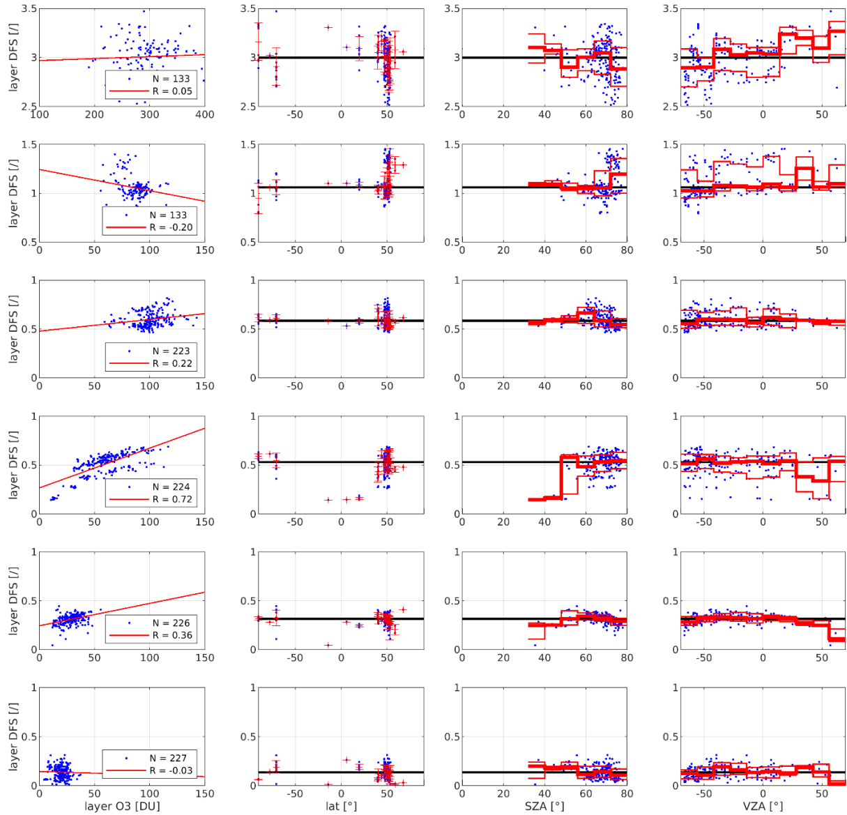
Figure 29: Correlation (R) between the six subcolumn DFS values and the six ozone subcolumns as observed by TROPOMI (first column) for the same N observations as in the previous figure. Subsequent columns show the layer-DFS as a function of latitude, SZA, and VZA. 84, 50 (thicker), and 16 % quantiles are added in red together with the overall layer mean (black line).
