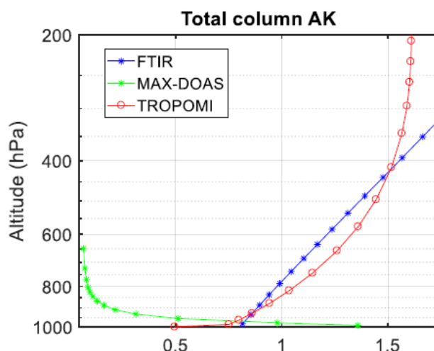
Figure 61: Typical total column averaging kernels for S5P TROPOMI and the two ground-based instrument types: FTIR (blue), MAX-DOAS (green), and TROPOMI (red). This illustrates the problem of the vertical smoothing difference error in these comparisons, as the instruments “see” different parts of the column.
