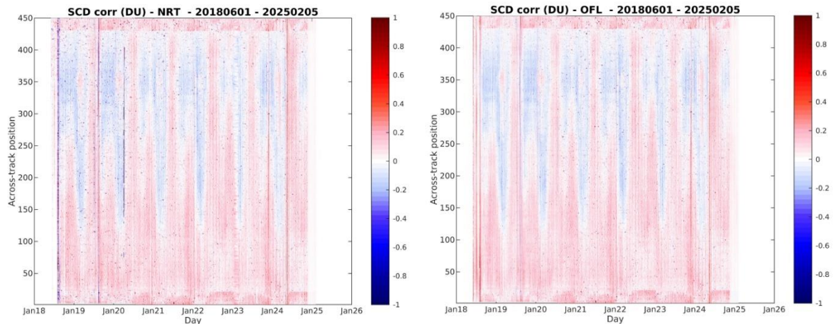
Figure 82: Comparison of the NRT (left) and offline (right) SO 2 data products. Shown are the time series of background corrected SO 2 SCDs for all 450 detector rows from June 2018 to February 2025. Most of the short time features (vertical, coloured lines) are caused by individual strong volcanic eruptions. For the NRT product, a strong spike occurs in early April 2020, which is caused by a downlink issue that corrupted an irradiance file. Courtesy of Nicolas Theys, BIRA-IASB.
