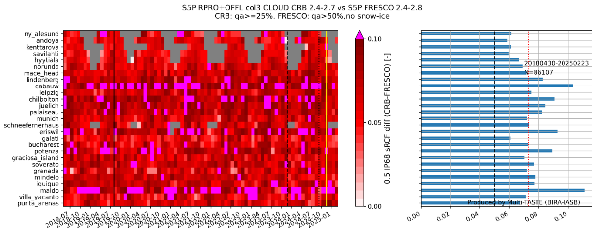
Figure 108. Left. Monthly \frac{1}{2} IP68 of scaled cloud fraction difference of CLOUD OFFL vs FRESCO OFFL, per month and per station. Indicated is the pixel size switch (2019/08/06) and the following updates: CLOUD v2.6.1 & FRESCO v2.6.0 (2023/11/26), FRESCO v2.7.1 (2024/09/11) and CLOUD v2.7.0 & FRESCO v2.8.0 (2024/11/16). Right: \frac{1}{2} IP68 of scaled cloud fraction difference (CLOUD CRB-FRESCO), per station.
