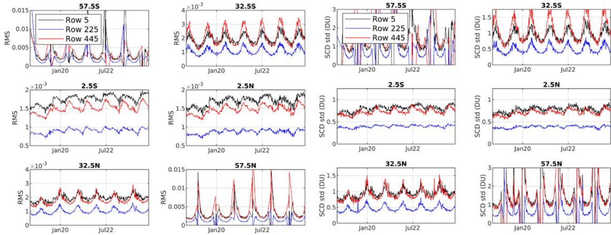
Figure 80: Temporal evolution of the measurement error (left, until November 2024) and the standard deviation (right, until February 2025) for selected 5° latitude bands and 3 detector. Good qualitative agreement between both quantities is found indicating that the random uncertainty is well characterized by the measurement error. Larger errors (and standard deviations) are found at the edges of the detector and towards high latitudes. The jump in the RMS and standard deviations in low and mid-latitudes in August 2019 are caused by the reduction of the ground pixel size. Courtesy of N. Theys (BIRA-IASB). (the figure with the RMS (left) is not updated for the new release after November 2024, because the old and new retrievals have different ways to calculate the RMS; both figures will be consistently updated after the complete reprocessing with the new version).
