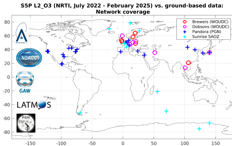
Figure 12: Geographical distribution of Brewer, Dobson, Pandora and ZSL-DOAS ground-based stations for which co-locations with S5P L2_O3 NRTI ozone data have been used (July 2022 until February 2025).
