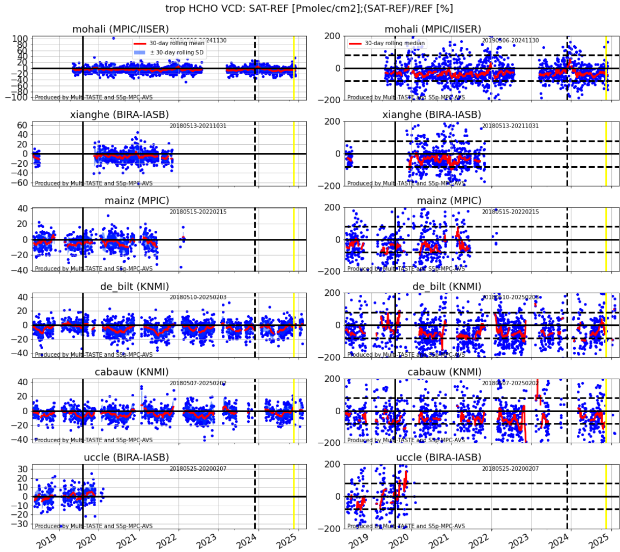
Figure 58: Time series of the difference [Pmolec/cm 2 ] and relative difference [%] between S5P RPRO+OFFL and MAX-DOAS HCHO column data at six stations. Data was obtained from the VDAF Automated Validation Server on 2025/02/26. Indicated are the pixel size switch (2019/08/16) the update to v2.6.1 (2023/11/26) and the update to v2.7.0 (2024/11/16).
