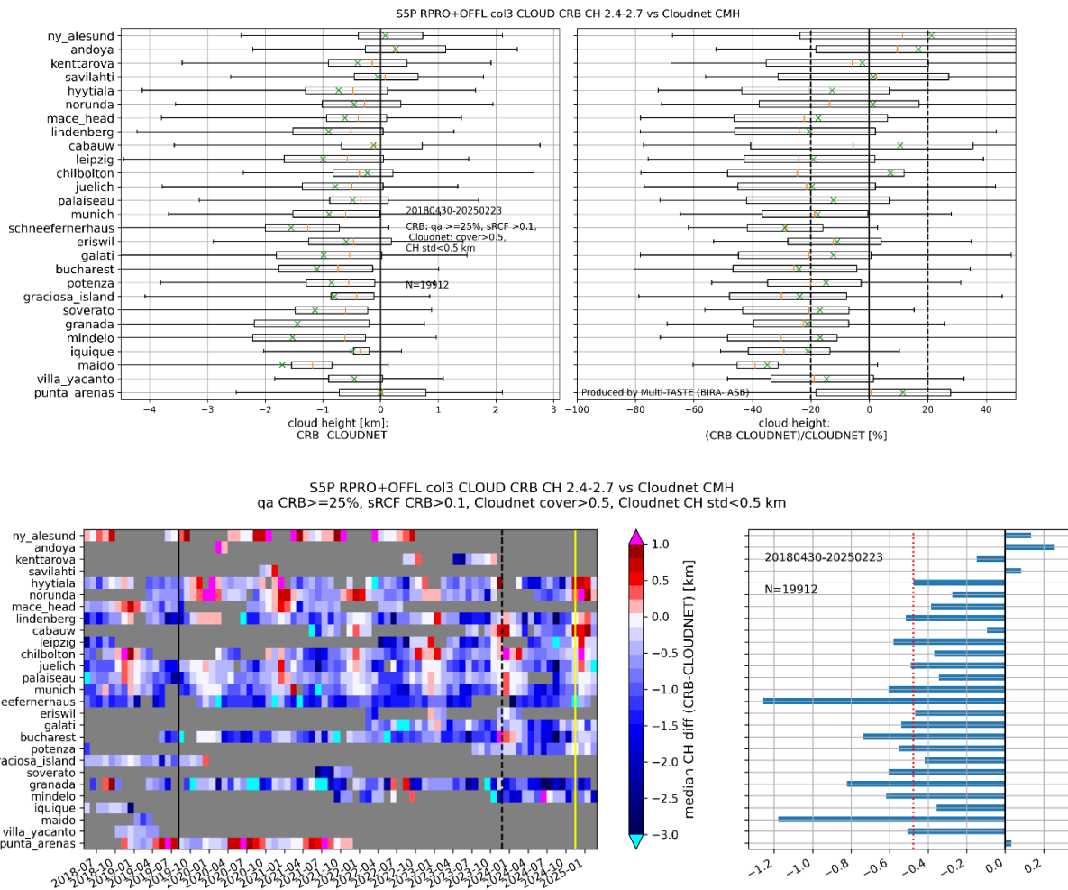
Figure 113: Upper panel: Boxplots of S5P L2_CLOUD CRB RPRO+OFFL CH minus CLOUDNET CH (upper left) and of the relative difference (upper right), per station. The same conventions as for Table 17 apply. Sensing time range is indicated on the figure. Bottom left panel: monthly median of CLOUD CRB CH-CLOUDNET CMH, per station. Pixel size switch (2019/08/06) and the following updates CLOUD v2.6.1 (2023/11/26), and CLOUD v2.7.0 (2024/11/16) are indicated on the plot. Bottom right panel: median difference per station. The dashed red line indicates the median over the median differences.
