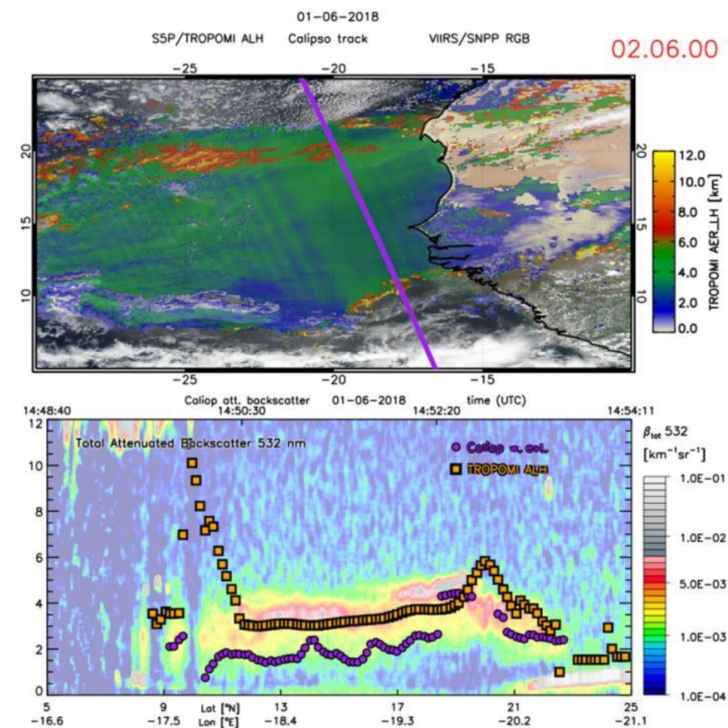
Figure 124: ALH (v02.06.00) for a desert dust case on 1 June 2018 retrieved by TROPOMI (top panel) and the CALIOP total attenuated backscatter image (bottom panel). The purple line and dots show the CALIPSO track and CALIOP weighted extinction averaged along the track, respectively. In the bottom panel the ALH retrieved by TROPOMI along the CALIOP orbit track is shown by the orange squares.
