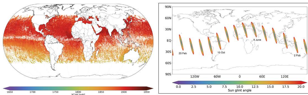
Figure 101: (left) Annual coverage of XCH 4 retrievals over the ocean for the year 2022, and (right) seasonal cycle of the sun-glint geometry.
