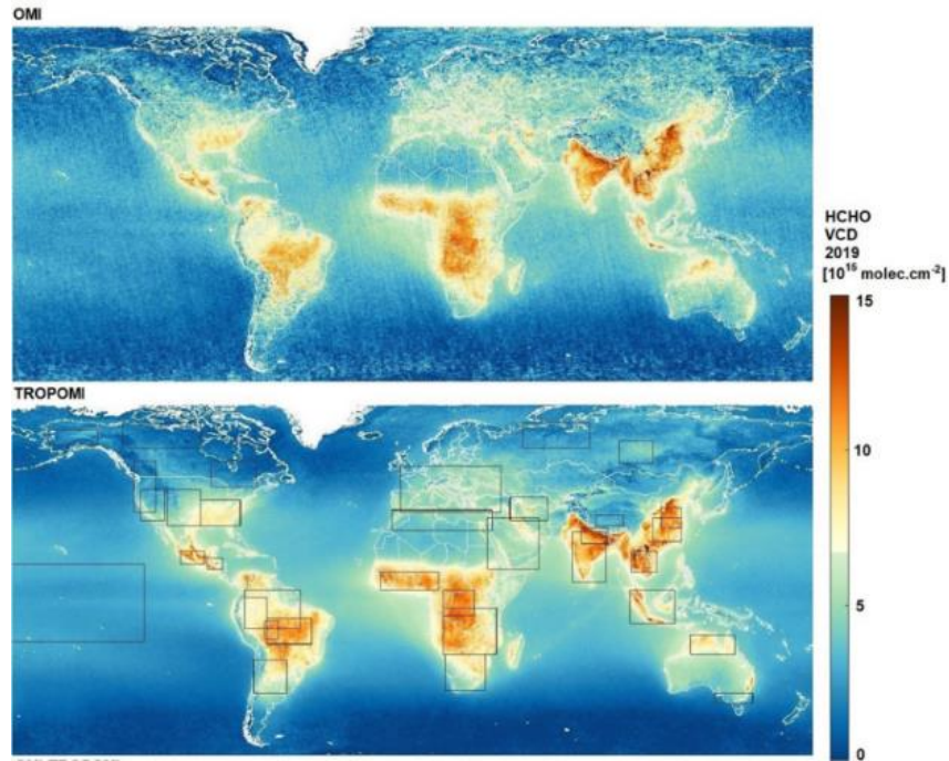
Figure 66: Average HCHO tropospheric column ( N_{v\_clear} ) retrieved from OMI (upper panel) and S5P TROPOMI (lower panel) in 2019. Limits of the regions selected for the comparisons are identified on the TROPOMI map. The same grid is used for both dataset (0.05°). Data are filtered using the recommended product quality flags.
