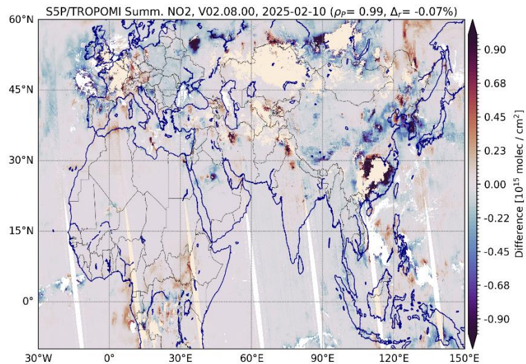
Figure 53: Difference between S5P NRTI and OFFL V2.8.0 daily total NO 2 column data for 2025/02/10. The difference is only calculated for columns > 0.5 Pmolec/cm 2 , cloud fractions < 0.6 and a qa_value > 0.5. Data was binned to 0.1° x 0.1° grid cells.
