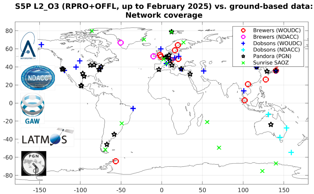
Figure 3: Geographical distribution of Brewer, Dobson, Pandora, and ZSL-DOAS ground-based stations for which co-locations with S5P L2_O3 OFFL ozone data have been used (period up to February 2025).
