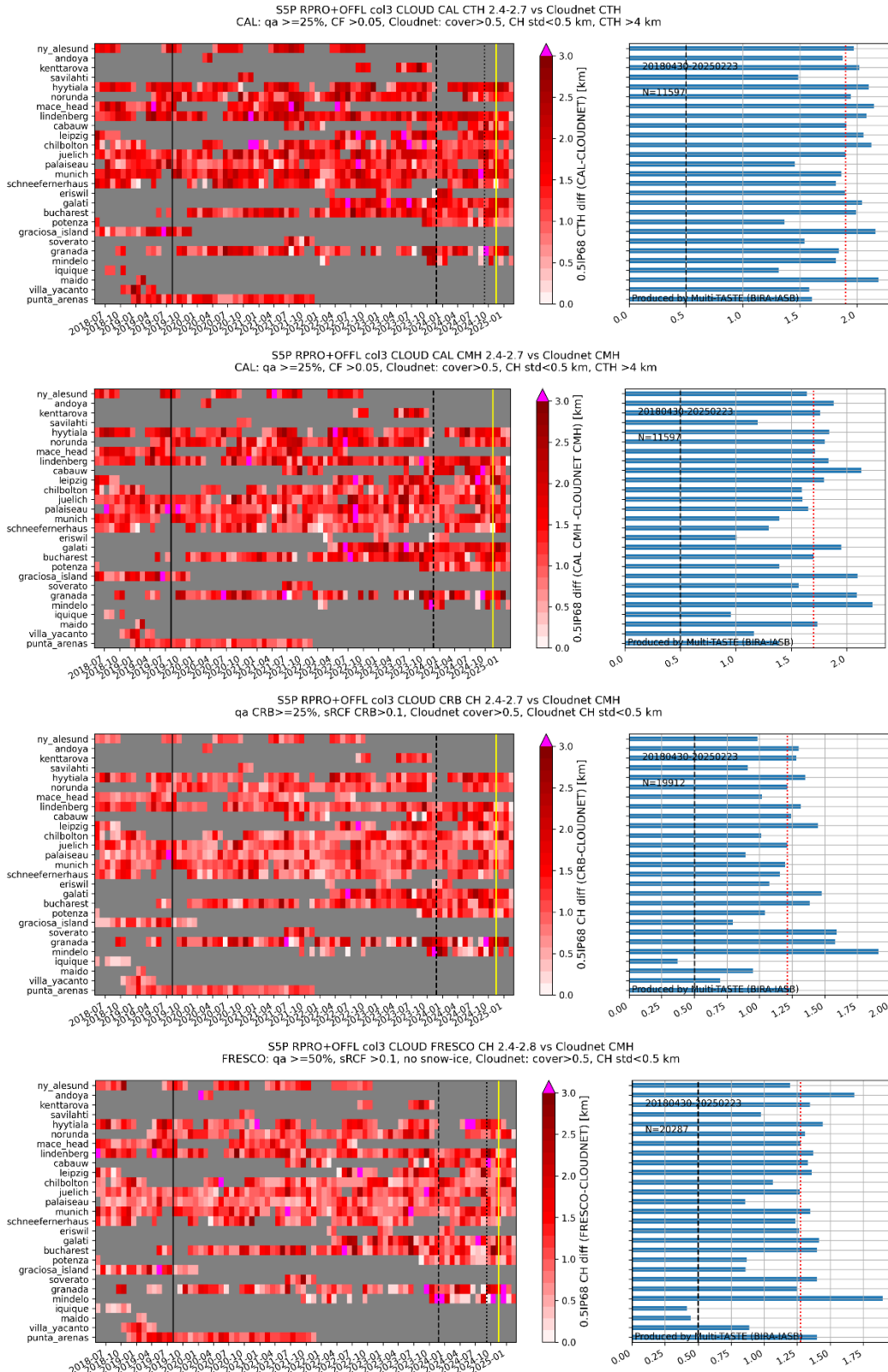
Figure 116. Monthly dispersion ( \frac{1}{2}IP68 ) per station of S5P CLOUD CAL CTH minus CLOUDNET CTH (top), S5P CLOUD CAL CMH minus CLOUDNET CMH, S5P CLOUD CRB CH minus CLOUDNET CH, and S5P FRESCO CH minus CLOUDNET CH (bottom). Indicated are the pixel size switch (2019/08/06) and the following updates: CLOUD v2.6.1 & FRESCO v2.6.0 (2023/11/26), FRESCO v2.7.1 (2024/09/11) and CLOUD v2.7.0 & FRESCO v2.8.0 (2024/11/16).
