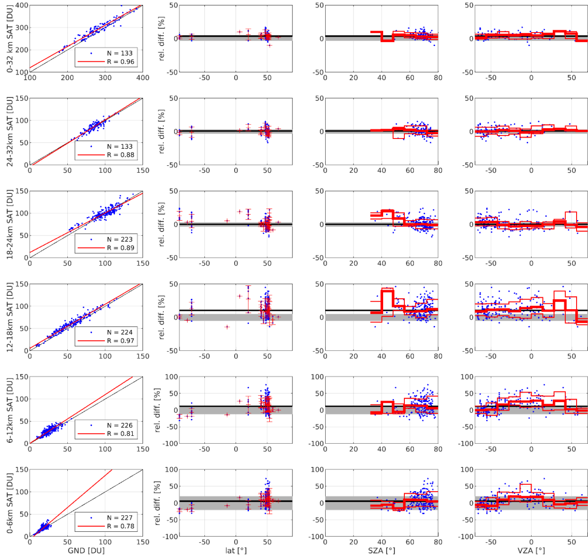
Figure 28: Correlation (R) between N lowest five ozone subcolumns as observed by TROPOMI and the coincident vertically integrated ozonesonde measurements (first column), and their overall sum (top row). Subsequent columns show the differences between satellite and ozonesonde subcolumns as a function of latitude, SZA and VZA. 84, 50 (thicker), and 16 % quantiles are added in red, together with the overall mean difference (black line), and the product requirements for each subcolumn (grey areas).
