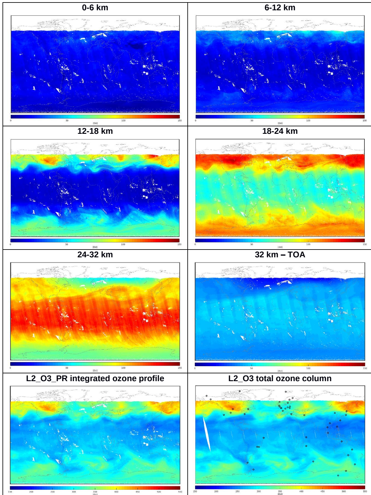
Figure 33: Upper six panels: daily global map for the six partial columns in the S5P L2_O3_PR OFFL v02.08.00 ozone profile product of January 1, 2025, as a function of altitude. The two lower maps show the total ozone column values obtained by integration of the L2_O3_PR profile data (left), and the map of L2_O3 total ozone column values for the same day (right) to check for their mutual consistency.
