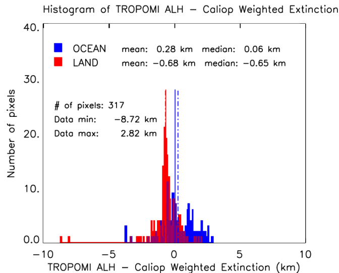
Figure 130: Histogram of the difference between the ALH from TROPOMI and CALIOP weighted extinction for the cases presented. Pixels over land are plotted in red and pixels over water in blue.
