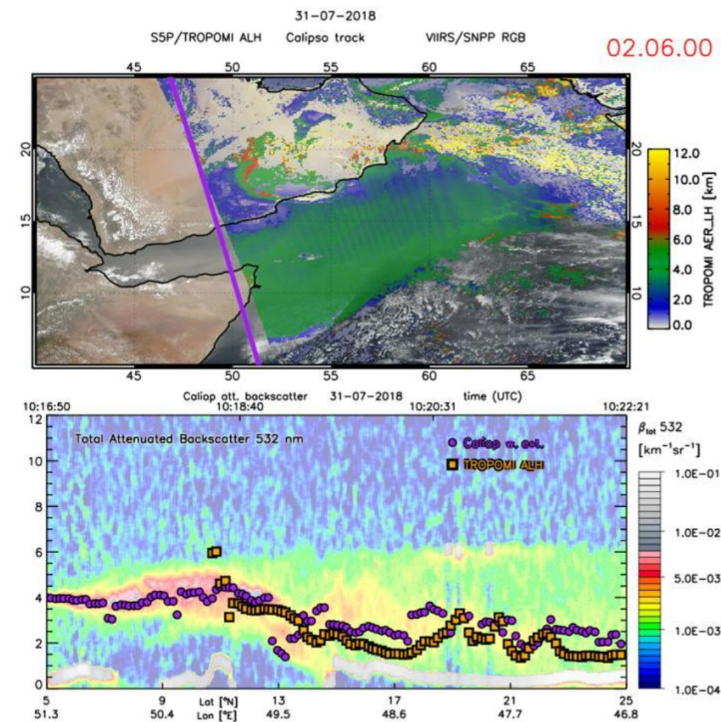
Figure 125: Same as above, but for 31 July 2018 near the Arabian Peninsula.
