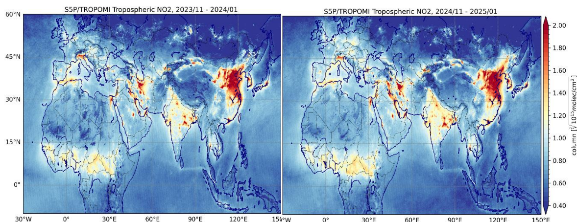
Figure 41: S5P RPRO/OFFL tropospheric NO 2 [-10°S, 60°N, -30°W, 150°E]. The data is binned on a grid of 0.1° latitude/longitude for Nov-Jan 2023/24 and 2024/25. A qa\_value > 0.75 and a cloud fraction CF < 0.2 are used to reduce the amount of data and exclude cloudy scenes. Columns are shown as the third root of values to better cover the dynamics.
