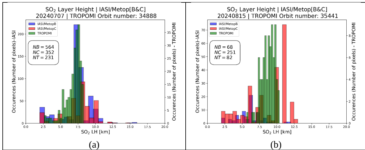
Figure 84. Histogram of the SO 2 layer height [in km] of the Etna volcano eruption on (a) July 7 and (b) August 15, 2024, as sensed by IASI/MetOp-B [blue], IASI/MetOp-C [red] and S5P/TROPOMI [green]. The left y-axis denotes the number of pixels of valid SO 2 layer height retrievals for the IASI instruments, whereas the right y-axis denotes the valid SO 2 layer height retrievals of the TROPOMI instruments. Only the retrievals corresponding to the TROPOMI lat/lon extents were selected for all instruments.
