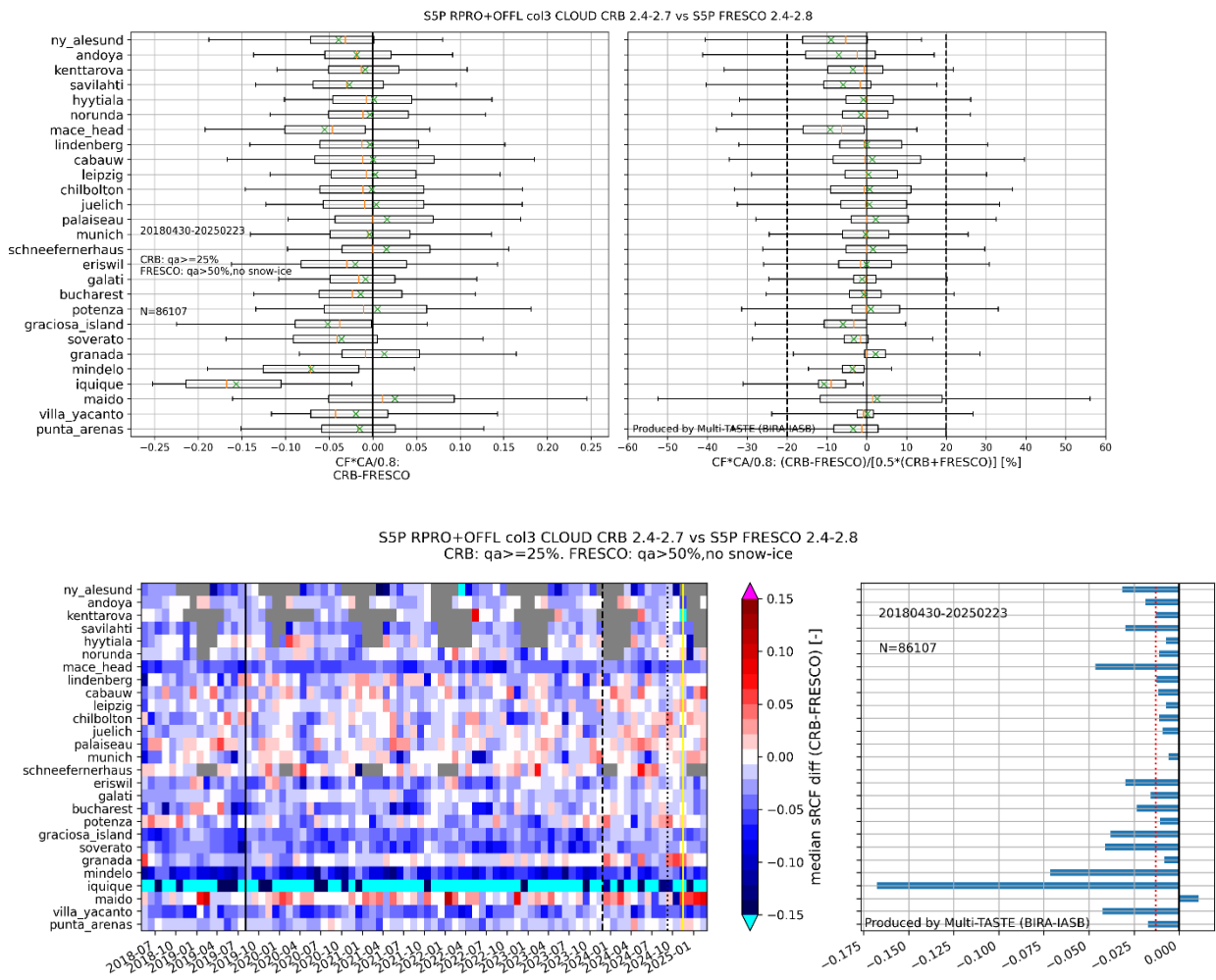
Figure 107. Top left. Box plots of S5P CLOUD CRB OFFL cloud fraction minus S5P FRESCO OFFL cloud fraction, after both have been rescaled to a cloud albedo of 0.8. Left: same but for the normed relative difference. The 20% bias requirement is indicated in dashed lines. Bottom left: monthly median of scaled cloud fraction difference, per month and per station. Indicated are the pixel size switch (2019/08/06), and the following updates: CLOUD v2.6.1 & FRESCO v2.6.0 (2023/11/26), FRESCO v2.7.1 (2024/09/11) and CLOUD v2.7.0 & FRESCO v2.8.0 (2024/11/16). Bottom right: Median of scaled cloud fraction differences per station. The red dashed line gives the median of these median differences.
