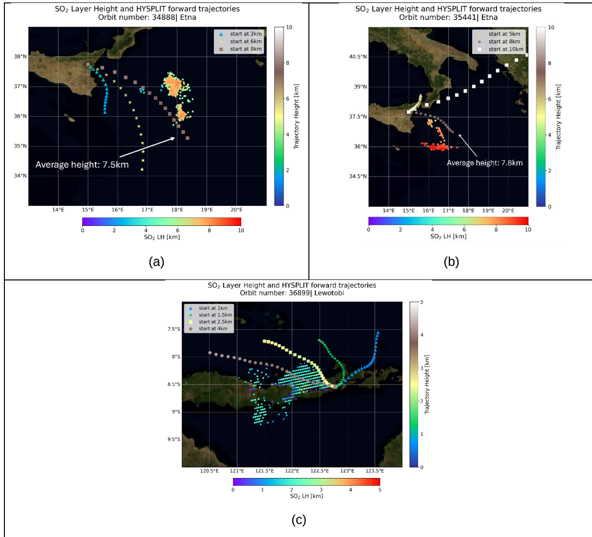
Figure 86: SO 2 _Layer_Height sensed by TROPOMI compared with the HYSPLIT air mass forward trajectories over Etna. (a) Forward trajectories start at the eruption time (00:00 on July 7, 2024, local time) and the selected heights of 2 km (blue), 6 km (yellow), 8 km (brown); (b) Forward trajectories start at the eruption time (00:30 on August 15, 2024, local time) and the selected heights of 5 km (blue), 8 km (yellow), 10 km (brown); (c) Forward trajectories start at the Lewotobi eruption time (1:30 on November 26, 2024, local time) at the selected altitudes of 1 km (blue), 1.5 km (green), 2.5 km (yellow) and 4 km (brown).
