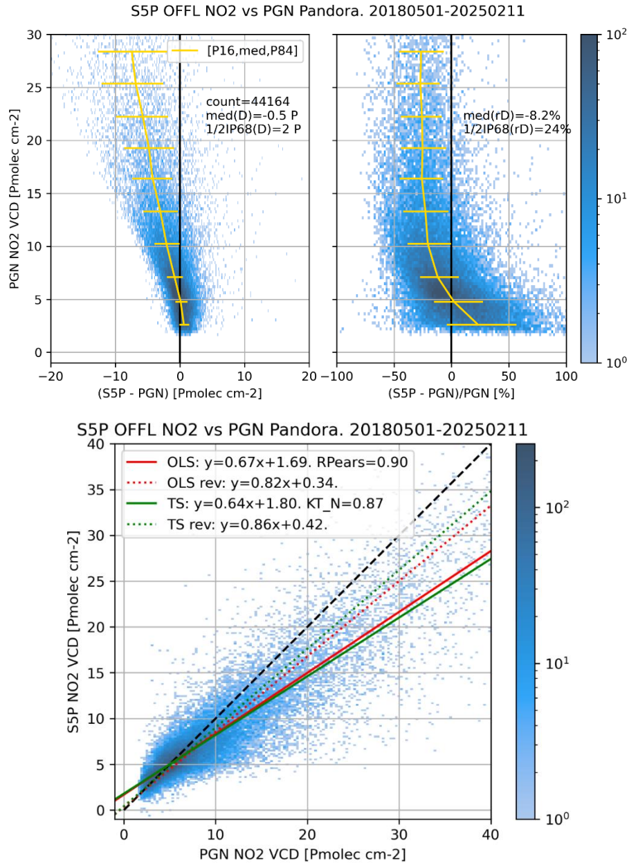
Figure 49: (Top) 2D-histogram of S5P vs PGN difference (left) and relative difference (right). The yellow line with error bar represents the median with [P16, P84] dispersion, per PGN NO2 VCD bin. (Bottom) correlation density plot of S5P vs PGN, with ordinary and robust Theil-Sen linear regression, y vs x and x vs y. RPears: Pearson correlation. KT-N: Normed Kendall-tau correlation.
