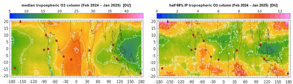
Figure 21: Median value (left) and half-width of 68% interpercentile (right) of S5P OFFL tropospheric ozone column data (CCD) over the last year of operations (February 2024 – January 2025). Red markers locate the twelve ground-based ozonesonde stations used in the validation analysis.
