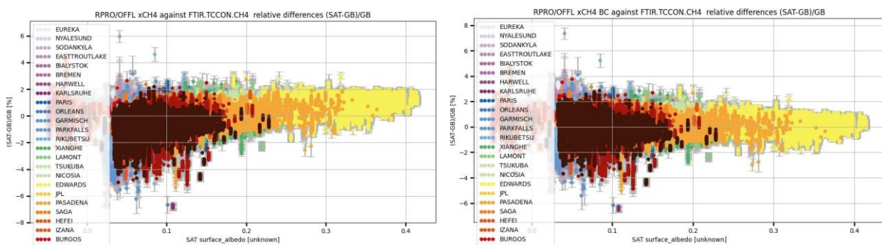
Figure 98: Dependence of the S5P-TCCON relative difference on surface albedo. The left column shows the standard S5P product and the right column the bias corrected S5P product. The bias correction removes the surface albedo dependence of the standard S5P product.
