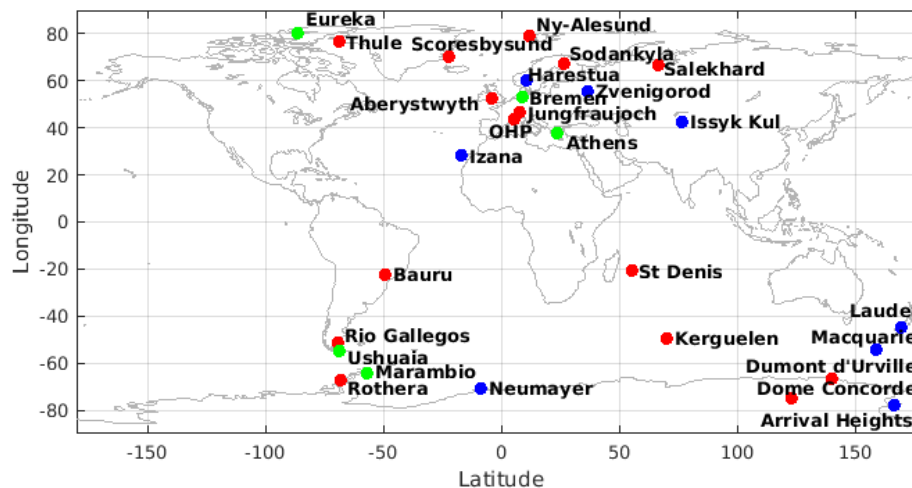
Figure 34: Geographical distribution of the NDACC ZSL-DOAS instruments routinely measuring stratospheric NO 2 and yielding co-locations with the current S5P L2_NO2 datasets. Stations marked with a red dot contribute fast delivery data coming from the LATMOS_RT facility. Blue and green dots depict the NDACC stations that contributes ZSL-DOAS data directly through the NDACC DHF and the AO project NIDFORVAL, respectively.
