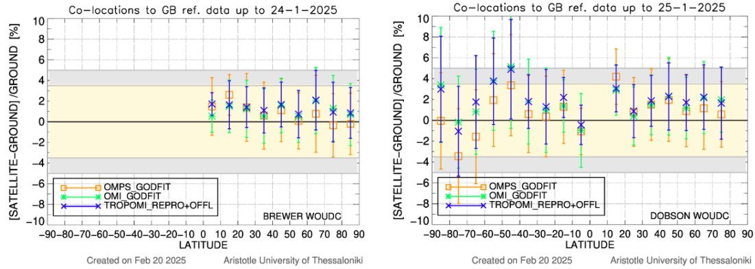
Figure 5: Comparison of the mean percentage differences between three satellite products (S5P L2_O3 OFFL, OMI GODFIT v4 and OMPS GODFIT v4) and ground-based total ozone data, versus latitude. The Brewer network comparisons are shown in the left-hand panel, and the Dobson network comparisons are depicted in the right-hand panel, both datasets are downloaded from Woudc. The period of data used for these plots is April 2018 –January 2025 (limited due to ground-based data availability). TROPOMI OFFL total ozone is reprocessed until 3 August 2022 and the operational OFFL product is used afterwards.
