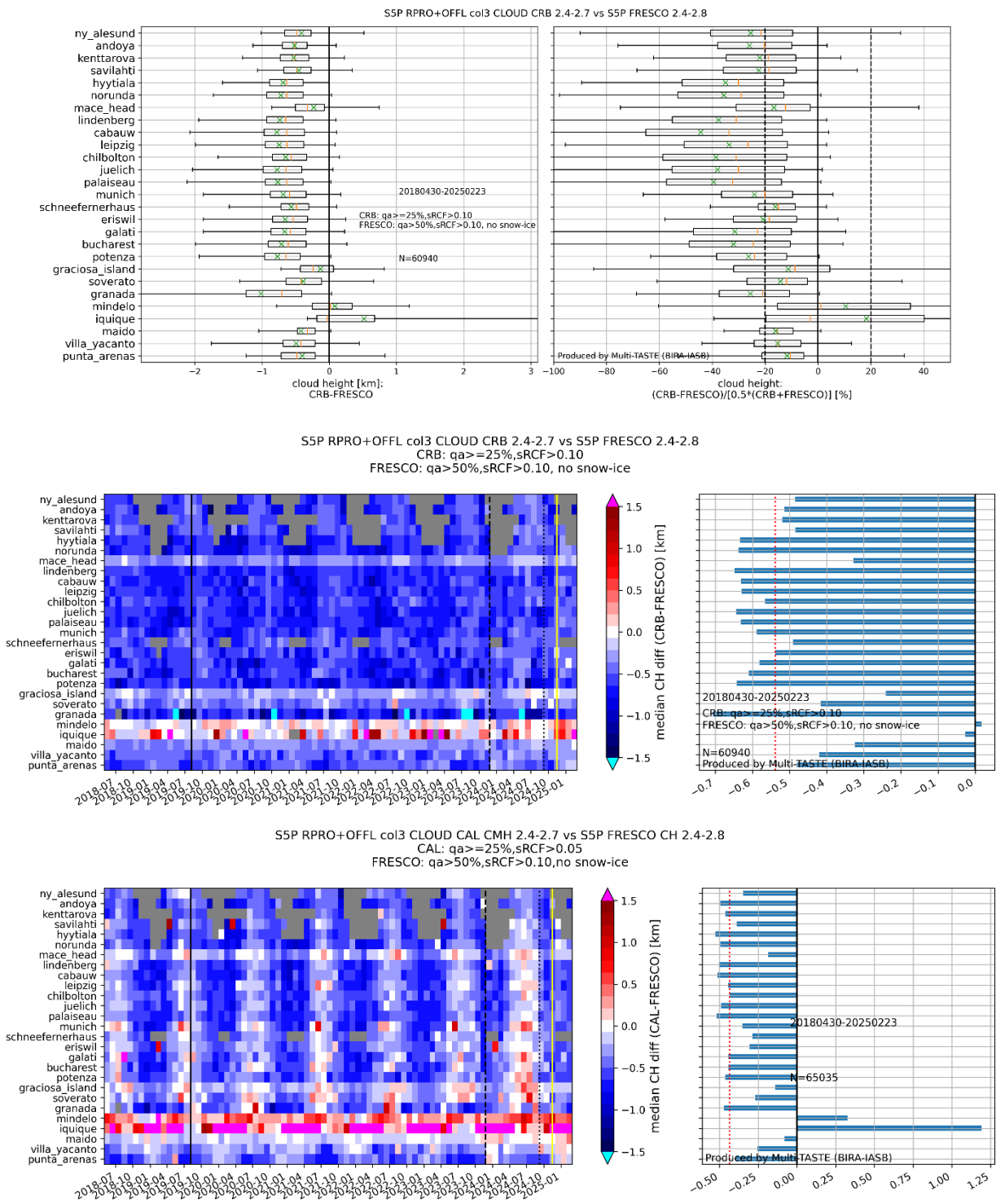
Figure 110: Top. Boxplots of S5P CLOUD CRB CH minus S5P FRESKO CH (left) and of the normed difference (right). Middle. Monthly median difference per station of CRB CH-FRESKO CH (left), and overall median difference (right). Bottom. Monthly median difference per station of CAL CMH-FRESKO CH (left), and overall median difference (right). Indicated is the pixel size switch (2019/08/06) and the following updates: CLOUD v2.6.1 & FRESKO v2.6.0 (2023/11/26), FRESKO v2.7.1 (2024/09/11) and CLOUD v2.7.0 & FRESKO v2.8.0 (2024/11/16).
