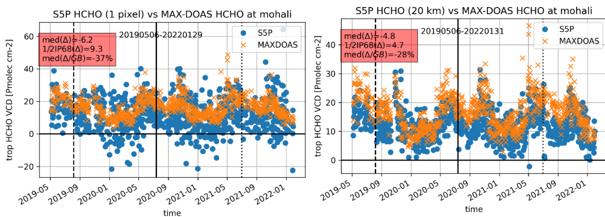
Figure 59: Time series of HCHO columns [Pmolec/cm 2 ] from S5P RPRO+OFFL and MAX-DOAS data at the Mohali station. (Left) Single S5P pixel, \pm 0.5h MAX-DOAS averaging, (Right) 20 km area average for \geq 10 pixels, \pm 3h averaging. Data was processed on 2022/02/28.
