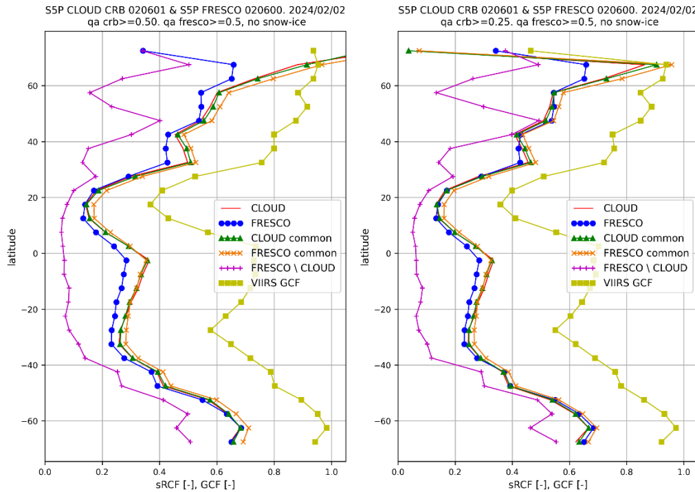
Figure 106. Latitudinal variation of zonal means of scaled radiometric cloud fraction of S5P OCRA/ROCINN CRB and S5P FRESCO-S, and geometrical VIIRS cloud fraction, for day 2024/02/02. Two quality filter criteria are used for CRB: the standard qa\_value > 0.5 , and a looser qa\_value > 0.25 .
