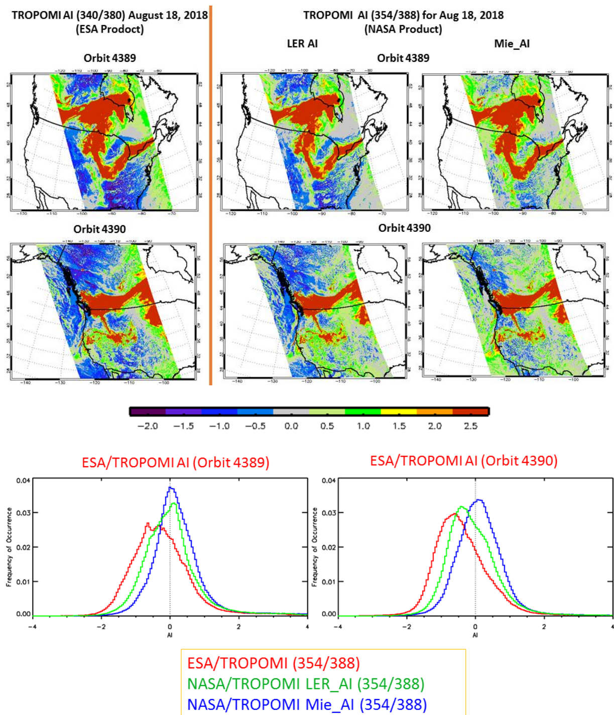
Figure 120: Comparison of UVAI from the operational TROPOMI UVAI product and TROPOMI UVAI analysed using the OMPS algorithm for an observation of a biomass burning plume (18 Aug. 2018). Like in the previous comparison, good agreement is found, but still the frequency distribution for the operational product is slightly broader than for the results using the OMPS algorithms (courtesy of Omar Torres and Changwoo Ahn, NASA-GSFC).
