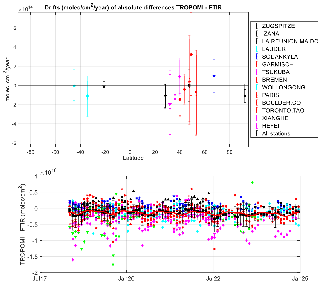
Figure 72: a (top panel): Drifts (trends in the absolute differences between the monthly means of TROPOMI and FTIR data. The smaller markers are for direct comparisons (no smoothing) and the larger ones are with smoothing (Rodgers and Connor 2003). The drift when all stations are considered simultaneously is added (92 latitude). b (bottom panel): all monthly means differences at individual sites and in black squares with error bars are shown the means of the differences (between TROPOMI and smoothed FTIR) at all sites for each month. The red curve is the regression model which includes a trend (given in Fig. 38a black square, large marker) and a seasonal cycle.
