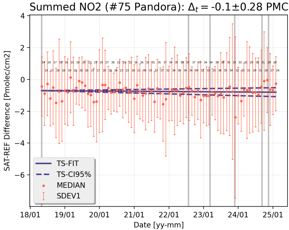
Figure 51: Time series – from May 2018 until January 2025 – of S5P RPRO+OFFL and PGN Pandora NO 2 total column differences, monthly averaged over all station [Pmolec/cm 2 ]. The number of stations is superimposed. Blue lines show the Theil-Sen regression slope and 95% confidence interval. Vertical grey lines show the version changes.
