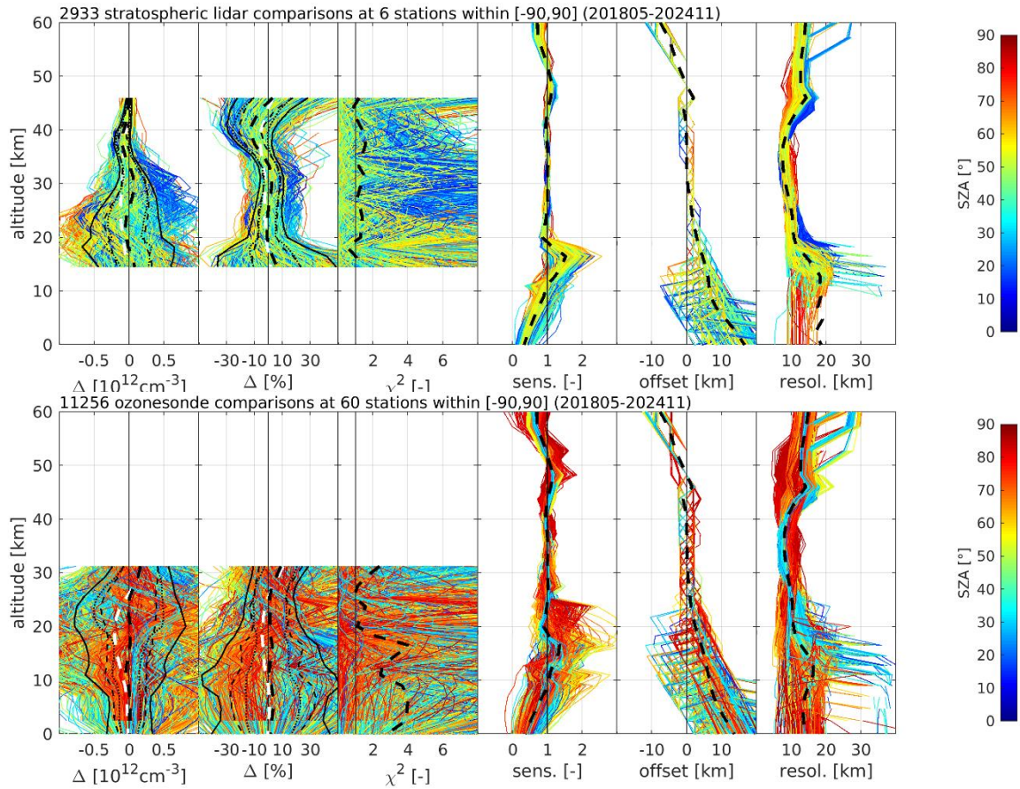
Figure 30: Comparison between S5P L2_O3_PR RPRO/OFFL ozone number density profile data and all co-located ground-based reference measurements, originating from stratospheric lidars (top) and ozonesondes (bottom) for L2 v02.04-07. Every plate shows six graphs, respectively, from left to right: the difference and the percent relative difference between S5P and reference data, the chi-square profile, the vertical sensitivity, the altitude registration offset, and the averaging kernel FWHM associated with the S5P retrieval. The colour scale indicates the TROPOMI solar zenith angle. Black dashed lines show mean values (thick lines) and standard deviations (thin lines, around the mean), while white, dashed lines indicate the mean difference between the a-priori profile and the reference measurement. Dotted black lines indicate the total ex-ante (inductive) uncertainty of TROPOMI and the reference measurements combined (around the mean difference).
