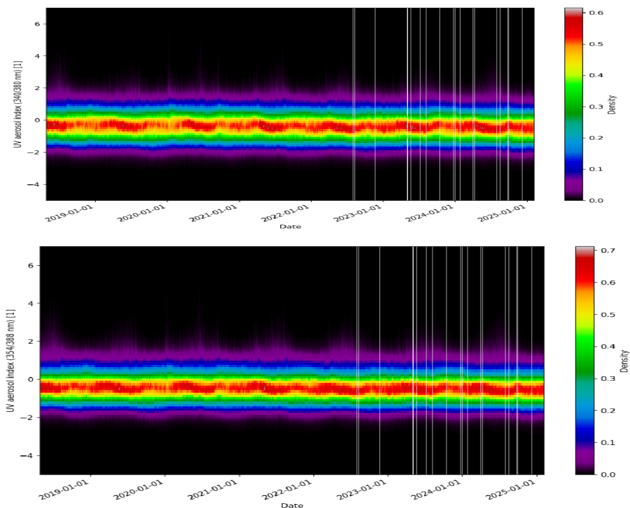
Figure 121: Comparison of the global daily mean and median for both L2_AER_AI UVAI wavelength pairs (340/380 and 354/388 nm), for the reprocessed data set from 20 July 2018 through February 2025. Middle and bottom: Corresponding histograms for both wavelength pairs.
