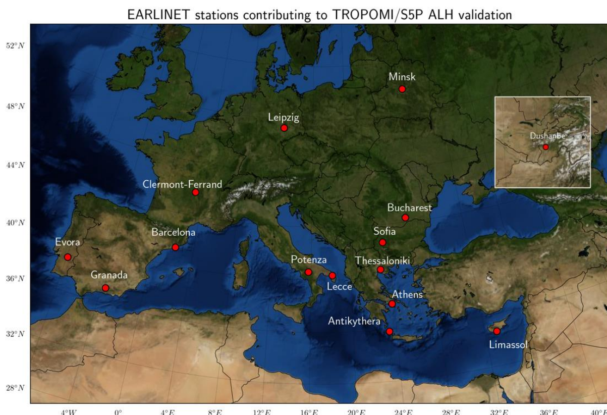
Figure 134: Geographical distribution of EARLINET ground-based stations for which co-locations with S5P L2 AER_LH data were used (period May 2018 – August 2023).
