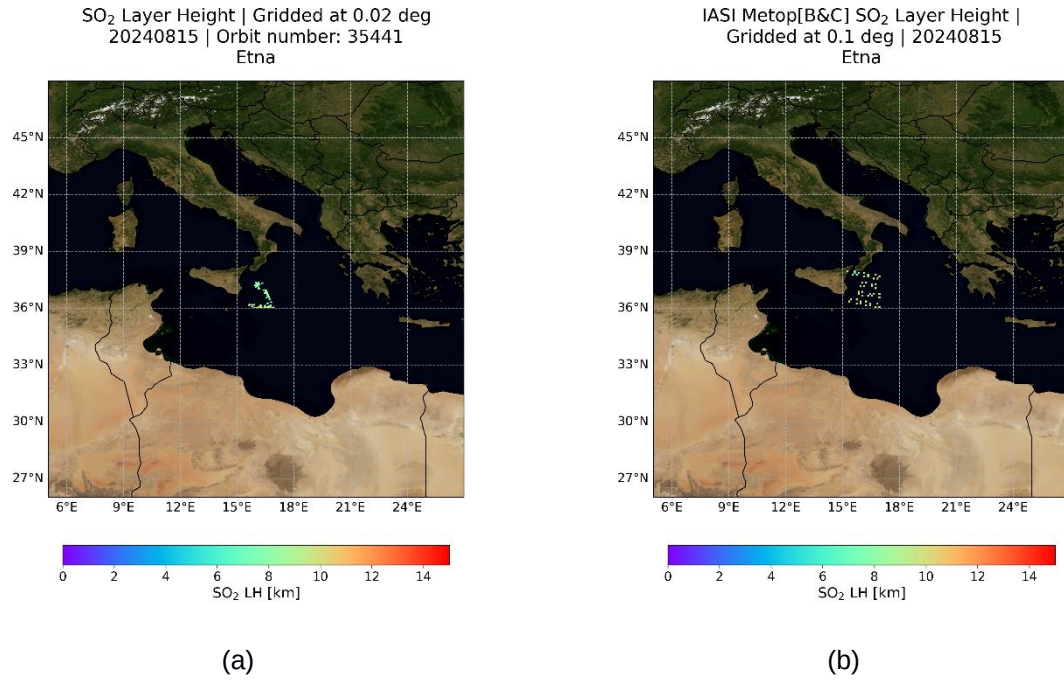
Figure 85. Gridded SO 2 layer height [in km] during the Etna volcano eruption on August 15, 2024, as sensed by (a) S5P/TROPOMI; (b) IASI/MetOp-[B&C].
