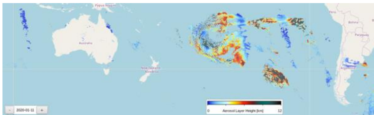
Figure 142: TROPOMI AER_LH product (processor version before v02.05.00) on 11 January 2020 over the south Pacific, showing the altitude as derived by the S5P AER_LH algorithm of the fires smoke from Australian bush fires.
