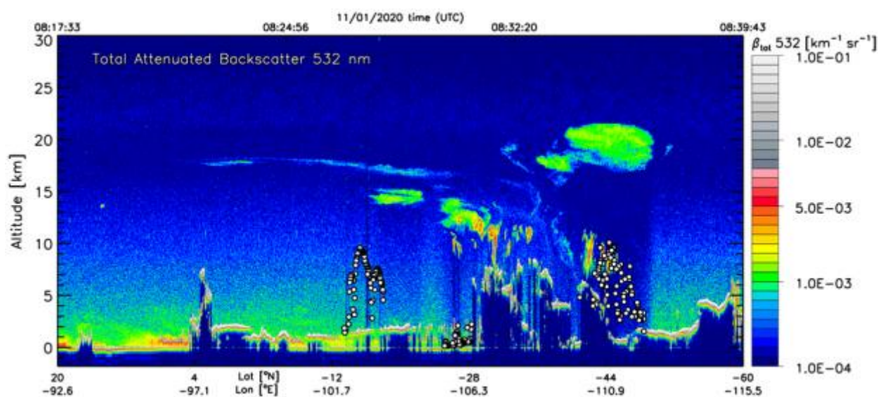
Figure 144: CALIOP aerosol backscatter rat 532 nm along the track shown in Figure 143 (eastern of Australia on 11 January 11, 2020). The yellow dots represent the TROPOMI ALH (processor version before v02.05.00).
