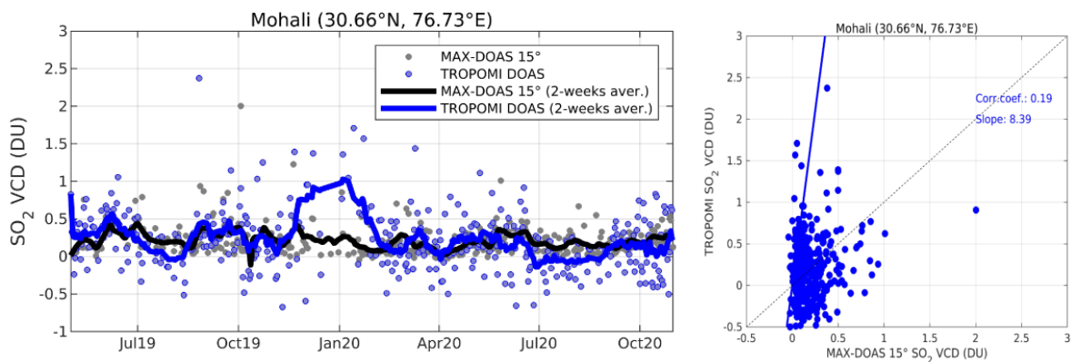
Figure 78: Comparison of TROPOMI SO 2 VCDs to MAX-DOAS measurements (daily means) at Mohali (India) from June 2019 to November 2020. The following selection criteria were applied: distance < 25km, CF<0.2, AMF>0.2, time window +/- 1h around overpass. Courtesy of N. Theys (BIRA-IASB), data provided by, Vinod Kumar, Vinayak Sinha, Sebastian Donner, Steffen Dörner, Thomas Wagner.
