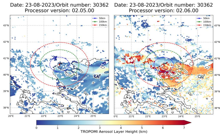
Figure 138: TROPOMI ALH spatial distribution on 23 August 2023, based on (left) V02.05.00 and (right) V02.06.00 algorithm processing version. The Thessaloniki EARLINET station is depicted with a red star. The color-coded concentric circles denote radii distances of 50, 100 and 150km from Thessaloniki lidar station.
