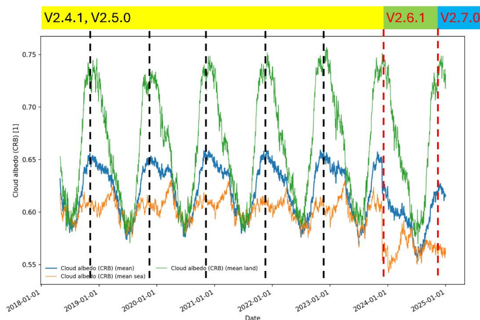
Figure 105. Global mean (all, land only, sea only) of (top) OCRA cloud fraction (OCRA prior, ROCINN_CAL and ROCINN_CRB) and (bottom) ROCINN_CRB cloud albedo. Time series taken from the L2QC portal, latest update on 2025-12-31. Dashed lines are guide to the eye.
