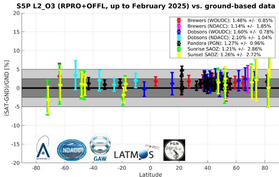
Figure 4: Meridian dependence of the median (the circular markers) and spread ( \pm 1 sigma, the error bars) of the percent relative difference between S5P TROPOMI L2_O3 (RPRO+OFFL up to February 2025) and ground-based (GND) ozone column data, represented at individual stations from the Antarctic to the Arctic and per measurement type. The values in the legend correspond to the median and spread of all median (per station) differences. For clarity, sunrise and sunset ZSL-DOAS results are represented separately (offset by -0.5^\circ and +0.5^\circ in latitude).
