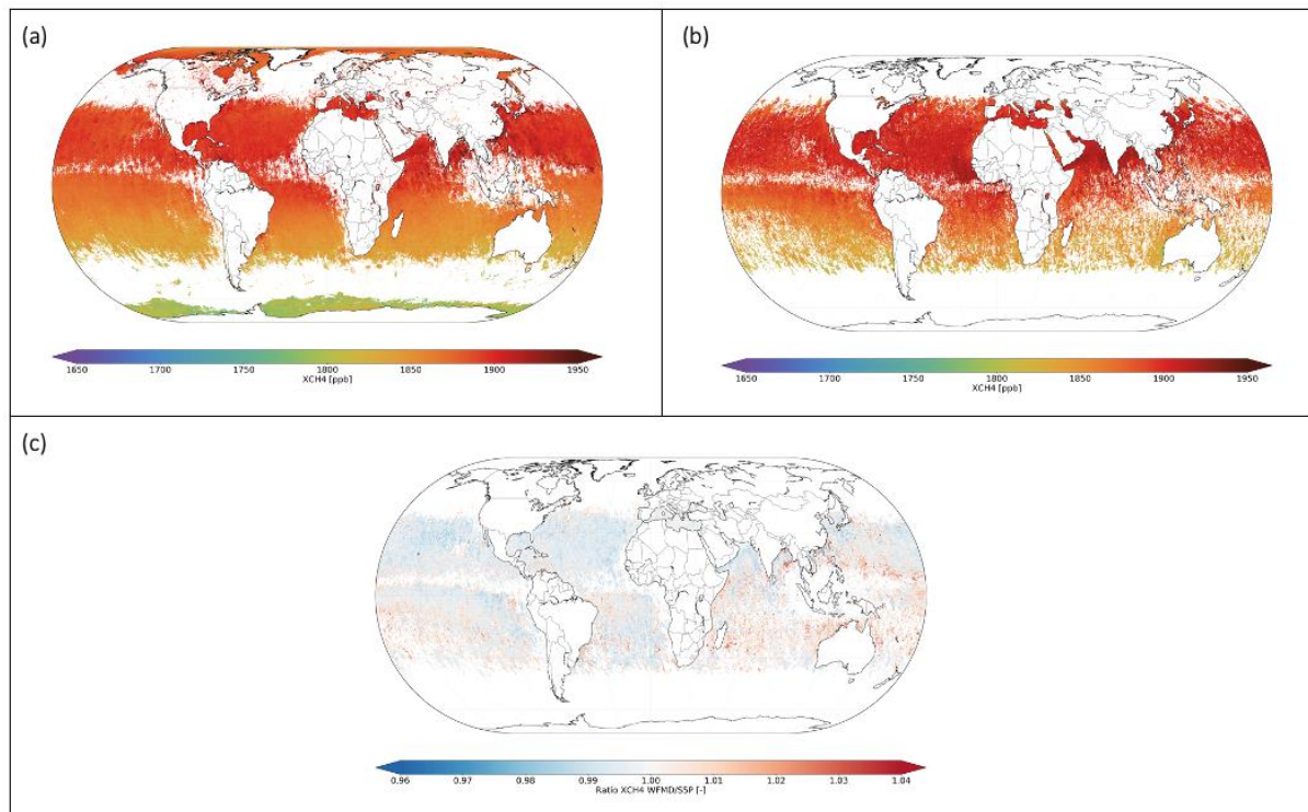
Figure 93: Global distribution of XCH 4 measured by TROPOMI retrieved with (a) WFMD-DOAS retrieval algorithm, (b) the pre-operational retrieval algorithm and (c) the ratio of both. Daily collocations are averaged to a 0.1 x 0.1-degree grid for the year 2022.
