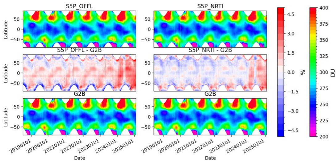
Figure 19: Time series of (the differences between) the zonal mean gridded (level-3) OFFL and NRTI total ozone column data sets.
