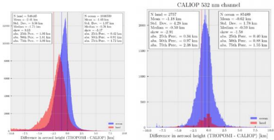
Figure 131: Histogram of differences between CALIOP weighted extinction height and TROPOMI ALH from collocated data between 1 May 2018 and 28 February 2019 (left). The right panel shows the same histogram, but for pixels that were screened for a minimal cost function (chi-squared) smaller than 1E5.
