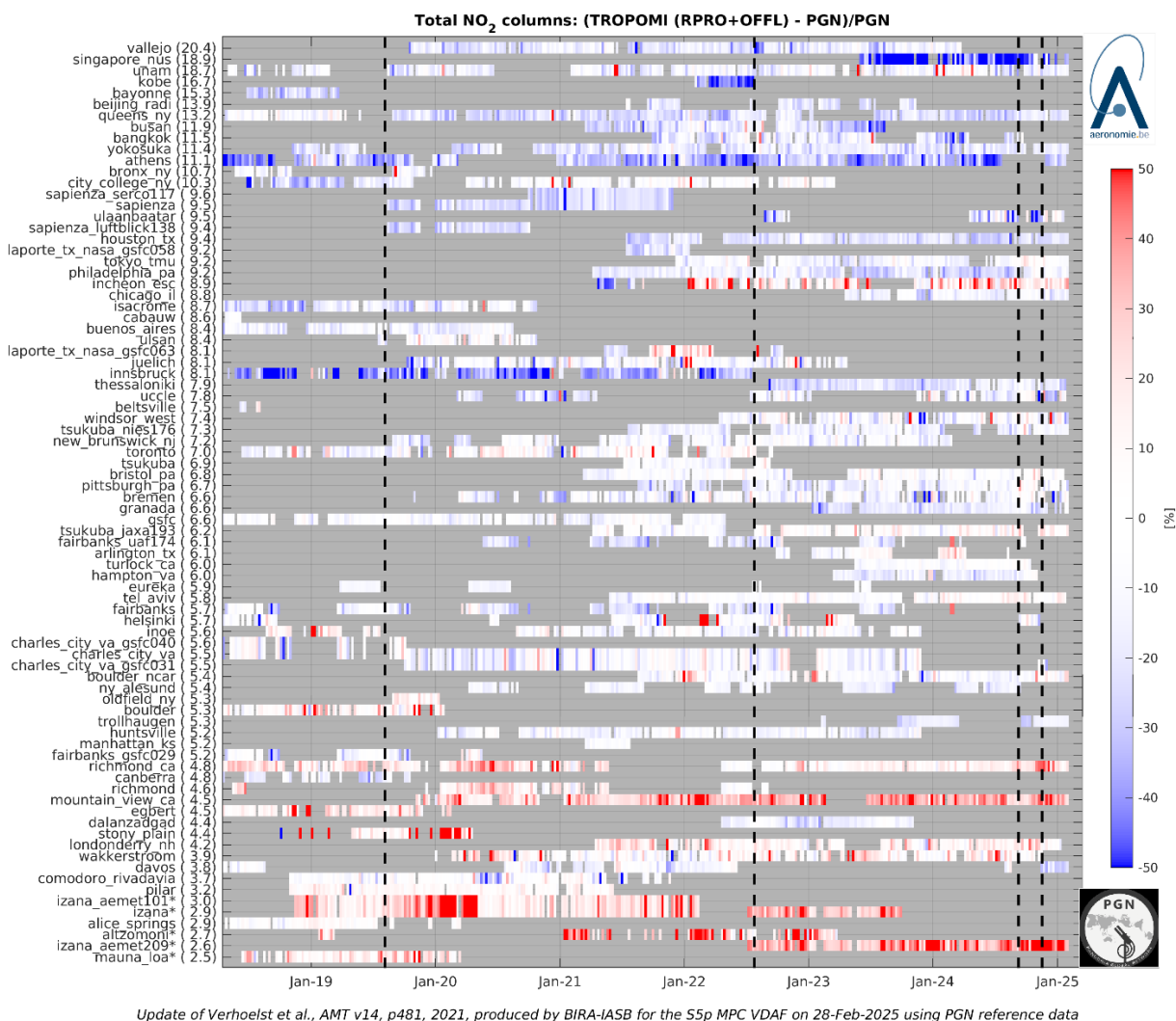
Figure 50: Time series – from May 2018 until February 2025 – of S5P RPRO+OFFL and PGN Pandora NO 2 total column differences, weekly averaged [%]. The black dashed lines indicate, respectively, the activation of the finer horizontal resolution and the switch between the RPRO and operational OFFL data. Stations are ordered by median total column, in brackets.
