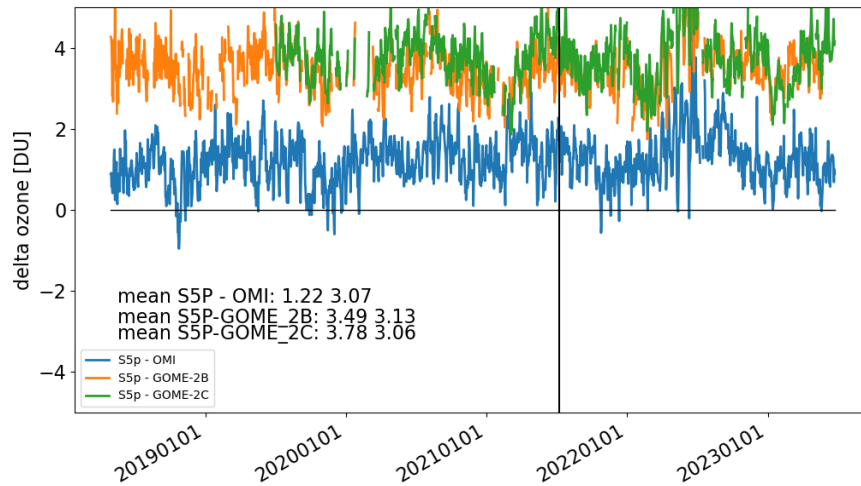
Figure 24: Difference time series of daily tropospheric O 3 column data averaged over the 20°S – 20°N tropical belt. S5P RPRO+OFFL CCD data are compared to OMI (blue), GOME-2B (orange), and GOME-2C (green) satellite data; positive values indicate a high bias of S5P w.r.t. the reference. The black vertical line indicates the transition from the RPRO to OFFL data files (see Table 1).
