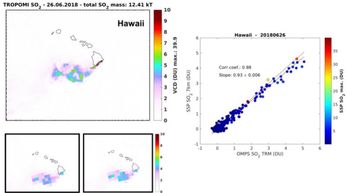
Figure 74: Comparison of TROPOMI and OMPS measurements of the volcanic plume of Kilauea on 26 June 2018. The large figure shows the original TROPOMI data. The two small figures show the spatially degraded TROPOMI data and the OMPS data. The figure right shows the correlation plot of the degraded TROPOMI data versus the collocated OMPS data. Courtesy of C. Li and N. Krotkov, NASA/GSFC.
