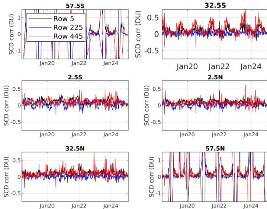
Figure 81: Temporal evolution of the averaged SO 2 SCD for selected 5° latitude bands and 3 detector rows from December 2018 to February 2025. The values are close to zero and show relatively small day-to-day variations. The larger variations in August 2019 are caused by strong volcanic eruptions. Courtesy Nicolas Theys (BIRA-IASB).
