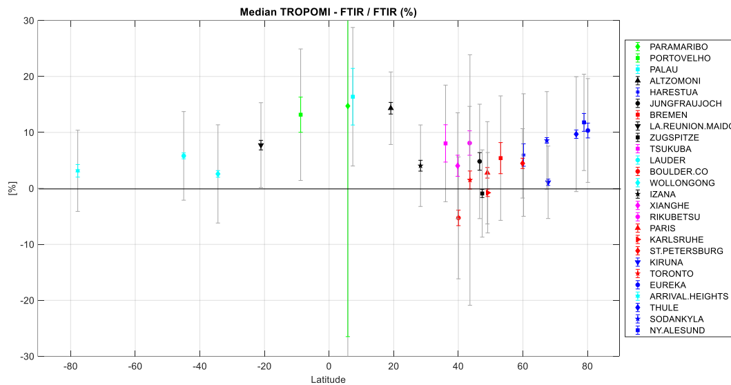
Figure 44: Median bias at each NDACC FTIR station as a function of latitude, calculated as the median of the percentage difference between S5P L2_NO 2 and the FTIR NO 2 stratospheric column measurement. The grey bars are the scaled MAD (see Sect. 6.2.1), and the coloured bars are the \pm 2\sigma error on the bias.
