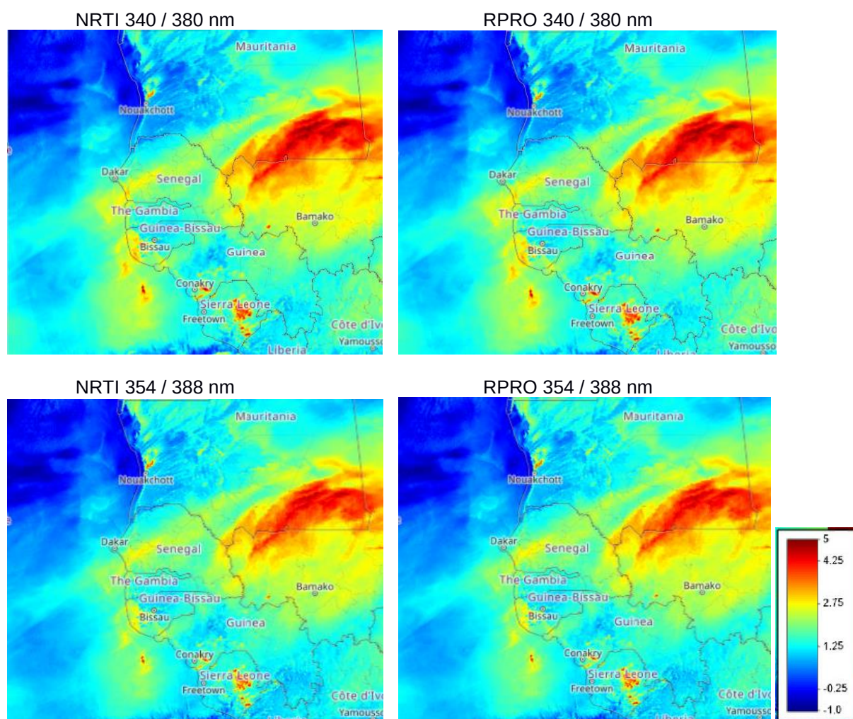
Figure 123: Comparison of the S5P TROPOMI near real time and reprocessed UVAI for a selected area on October 4, 2022 for the two wavelength pairs (top: 340 / 380 nm, bottom: 354 / 388 nm).
