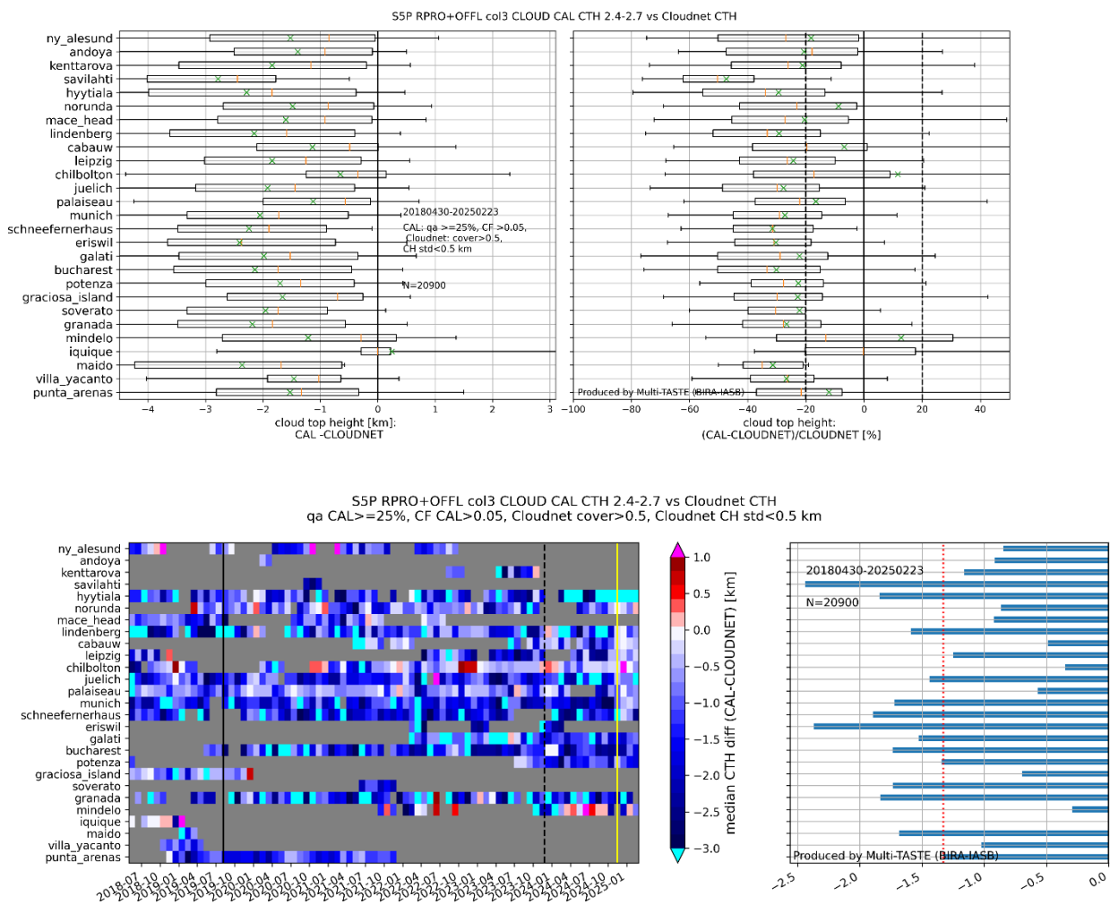
Figure 111: Top panel: Boxplots of S5P L2_CLOUD CAL CTH minus CLOUDNET CTH, per station. Boxplot conventions: box bounds are at first and third quartile. Orange line is median. Whiskers are at 5 and 95 percentiles. Green cross is mean. Right panel: Similar as upper panel but now for the relative difference. Sensing date range is indicated on the plot. Bottom left panel: monthly median of CLOUD CAL CTH-CLOUDNET CTH, per station. Pixel size switch (2019/08/06) and the following updates CLOUD v2.6.1 (2023/11/26), and CLOUD v2.7.0 (2024/11/16) are indicated on the plot. Right panel: median difference per station. The red dashed line gives the median over the median differences.
