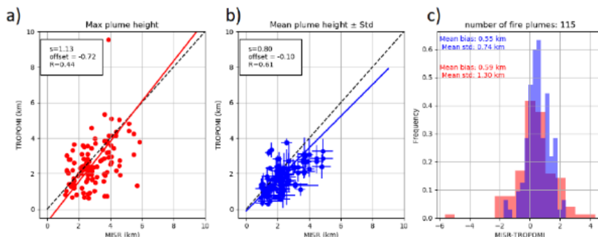
Figure 132: Comparison of TROPOMI ALH (processor version before v02.05.00) and MISR plume height for 115 fires over Northern America in 2018. See Griffin et al, 2019 for details.
