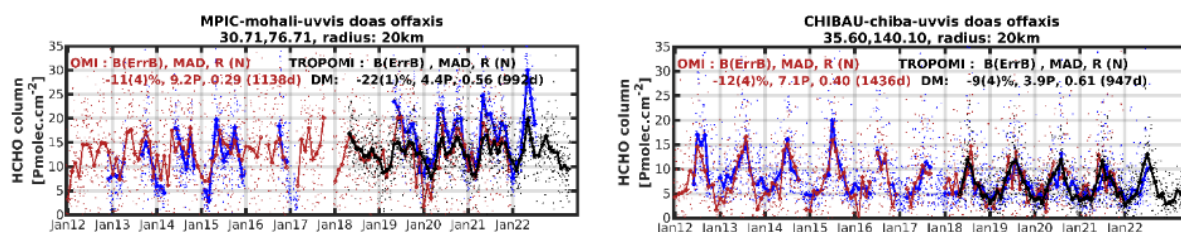
Figure 65: OMI, TROPOMI and MAX-DOAS HCHO time series at Mohali and Chiba. Time frame is Jan 2012 to May 2023.
