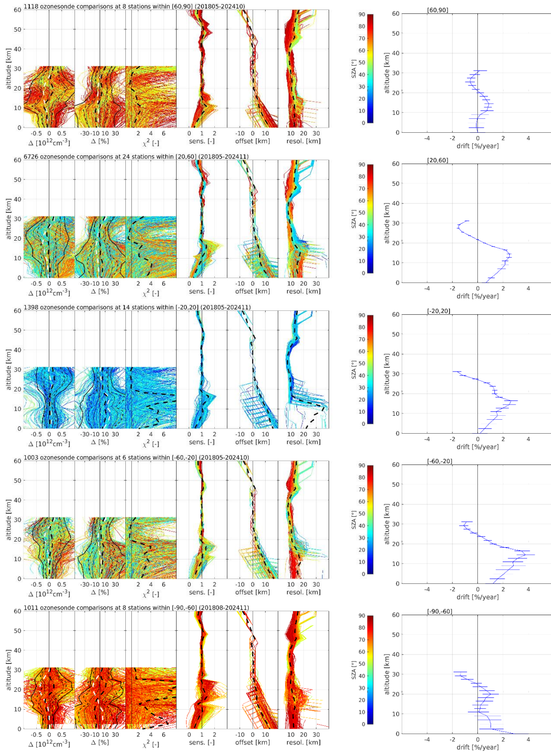
Figure 32: Comparison between S5P RPRO/OFFL ozone profiles (v2.4-8, May 2018 to November 2024) and co-located ozonesonde data in five latitude zones (Arctic to Antarctic, from top to bottom). Every row shows, from left to right: the difference and percent relative difference between S5P and ozonesonde data as a function of altitude, the chi-square, the vertical sensitivity, the altitude registration offset, the S5P averaging kernel FWHM, and the linear temporal drift. Colours indicate the SZA. Black dashed lines show mean values (thick lines) and standard deviations (thin lines, around the mean), while white, dashed lines indicate the mean difference between the a-priori profile and the reference measurement. Dotted black lines indicate the total ex-ante uncertainty of TROPOMI and the reference measurements combined (around the mean difference). Horizontal bars in the drift plots indicate 2-sigma uncertainty estimates on the drift using a bootstrapping technique with 1000 samples.
