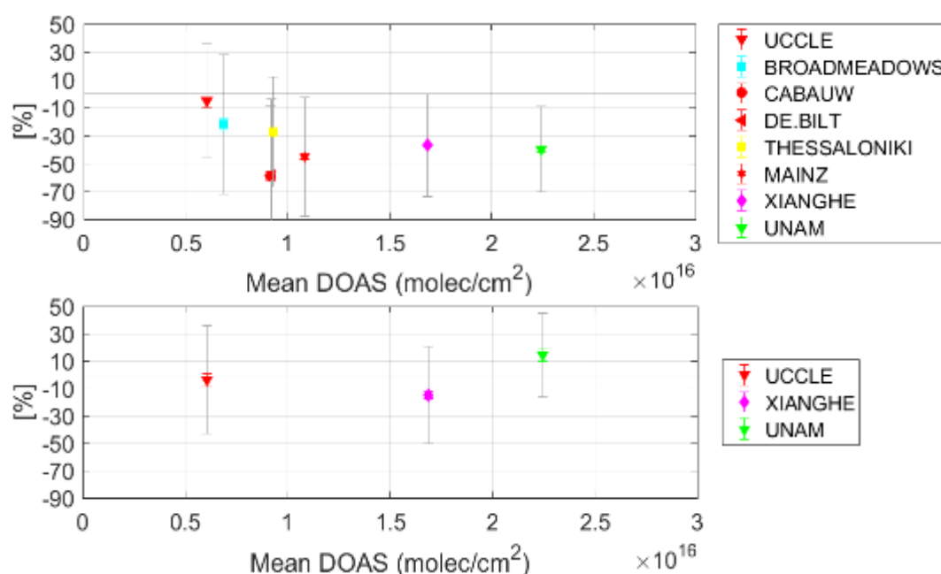
Figure 60: Bias at each station (%) as a function of the mean DOAS total columns ( 10^{16} \text{ molec/cm}^2 ). The grey bars are the systematic uncertainty on the differences, and the coloured error bars are the 2-σ error on the bias. Top panel: normal DOAS data without any modification. Bottom panel: DOAS data after Rodgers and Connor (2003) is applied (a priori substitution and smoothing with the TROPOMI averaging kernels).
