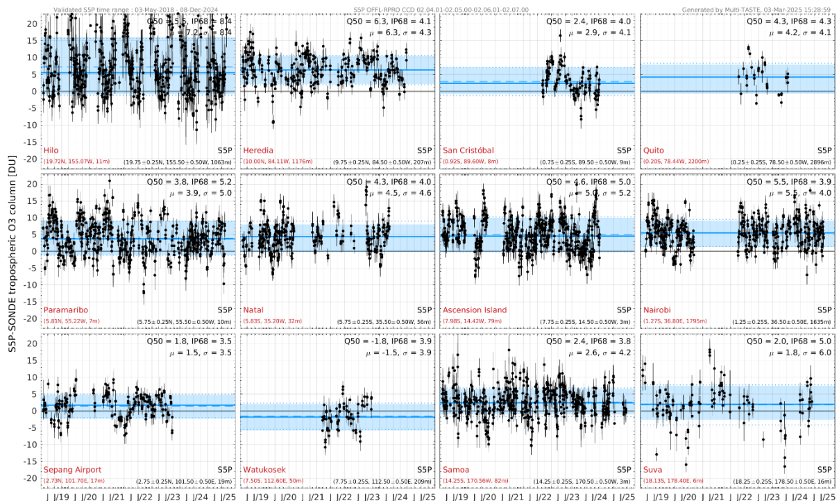
Figure 23: Time series of the absolute difference between spatially and temporally co-located S5P and ozonesonde tropospheric O 3 column data. The blue line and shaded area show the median value and the range between the 16 % and 84 % percentiles. Positive values indicate a high bias of S5P w.r.t. the reference.
