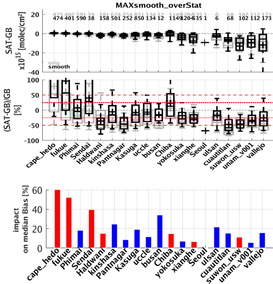
Figure 37: Box-and-whisker plots summarizing the bias and spread of the difference between S5P TROPOMI RPRO+OFFL v2.4/2.5/2.6/2.7/2.8 and MAX-DOAS NO 2 tropospheric columns (grey) and the smoothed MAX-DOAS NO 2 tropospheric columns (black). The third panel presents bar plot summarizing the change on the median bias between the original comparisons and the smoothed ones. Absolute values of the relative median biases are shown, where reductions are marked in blue bars and increases in red bars. The time frame is for all available data from May 2018 to end December 2024. The median difference is represented by a vertical solid line inside the box, which marks the 25 and 75% quantiles. The whiskers cover the 9-91% range of the differences and the crosses denotes the mean differences.
