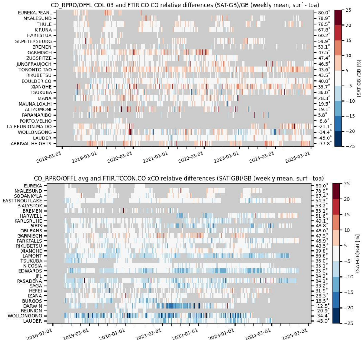
Figure 89: Relative bias between S5P L2_CO OFFL and ground-based CO column data at NDACC (top), TCCON (bottom) FTIR stations. Over the April 2018 – January 2025 period the plots do not show a clear meridian dependence or temporal change in the weekly averaged biases. Colour bar gradients are chosen such that they match with the measurement's uncertainties.
