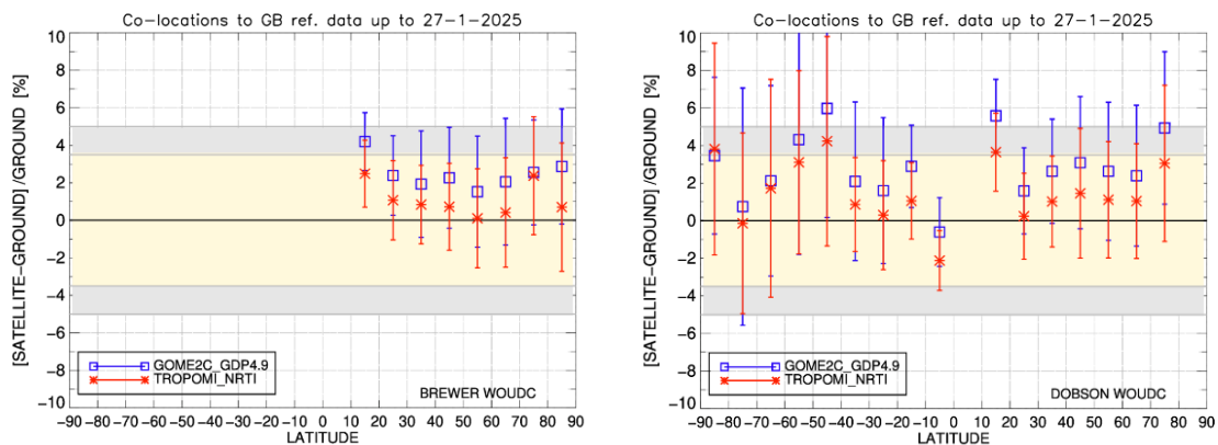
Figure 14: Comparison of the mean percentage differences between two satellite products (S5P TROPOMI L2_O3 NRTI and GOME-2C GDP4.9) and ground-based total ozone data, versus latitude. The Brewer network comparisons are shown in the left-hand panel, and the Dobson network comparisons are depicted in the right-hand panel, both datasets are downloaded from WOUDC. The period of data is July 2022 – January 2025 (limited by ground-based data availability).
