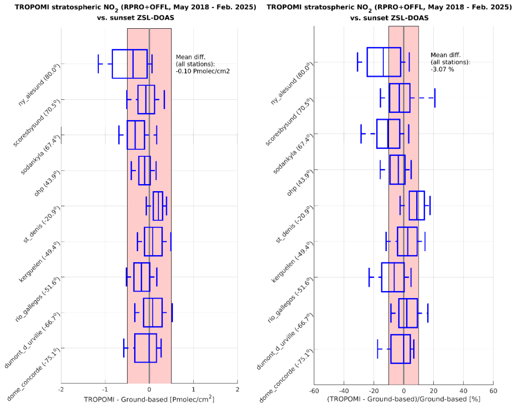
Figure 42: Pole to pole bias and spread (absolute differences in the left-hand panel, relative differences in the right-hand panel) of S5P TROPOMI RPRO+OFFL and NDACC ZSL-DOAS NO 2 stratospheric columns. For the current report, only the SAOZ data sets covering the full mission lifetime are shown. The median difference per station is represented by a vertical solid line inside the box, which marks the 25 and 75% quantiles and the whiskers denote the 9-91% range. The red shaded area represents either the mission requirement of 0.5 Pmolec/cm 2 for the random part of the uncertainty (left-hand panel) or that of 10% on the systematic uncertainty (right-hand panel). Station name and latitude of the station are added on the left. The time frame is May 2018 to February 2025.
