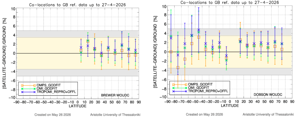
Figure 5: Comparison of the mean percentage differences between three satellite products (S5P L2_O3 OFFL, OMI collection 4 GODFIT v4 and OMPS GODFIT v4) and ground-based total ozone data, versus latitude. The Brewer network comparisons are shown in the left-hand panel, and the Dobson network comparisons are depicted in the right-hand panel, both datasets are downloaded from Woudc. The period of data used for these plots is April 2018 – April 2026 (limited due to ground-based data availability). TROPOMI OFFL total ozone is reprocessed until 3 August 2022 and the operational OFFL product is used afterwards.
