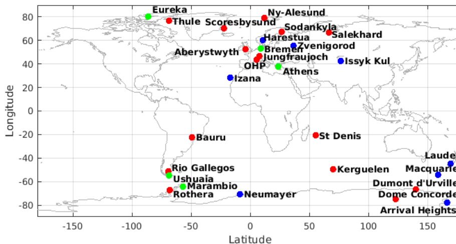
Figure 31: Geographical distribution of the NDACC ZSL-DOAS instruments routinely measuring stratospheric NO 2 and yielding co-locations with the current S5P L2_NO2 datasets. Stations marked with a red dot contribute fast delivery data coming from the LATMOS_RT facility. Blue and green dots depict the NDACC stations that contributes ZSL-DOAS data directly through the NDACC DHF and the AO project NIDFORVAL, respectively.
