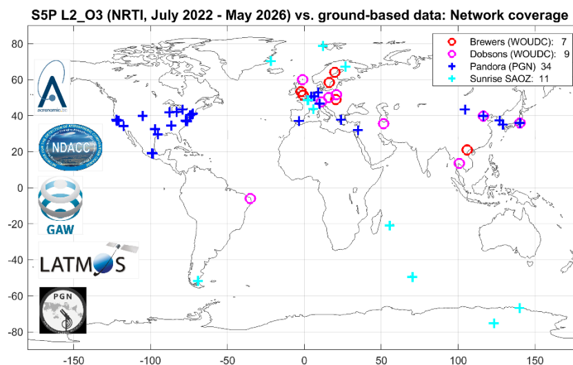
Figure 13: Geographical distribution of Brewer, Dobson, Pandora and ZSL-DOAS ground-based stations for which co-locations with S5P L2_O3 NRTI ozone data have been used (July 2022 until May 2026).
