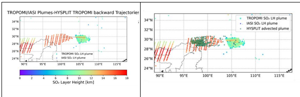
Figure 79: Demonstration of the revert in the overpasses between TROPOMI (~13:30 pm) and IASI-B/C (~9.30 am) (a) original TROPOMI SO 2 layer height, IASI-B SO 2 plume height on November 25, 2025 and backward TROPOMI SO 2 layer height at the overpass time of 9:30 am using HYSPLIT backward air mass trajectories.
