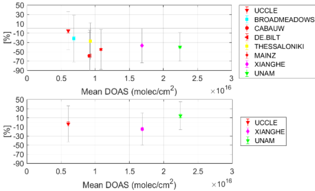
Figure 56: Bias at each station (%) as a function of the mean DOAS total columns ( 10^{16} molec/cm 2 ). The grey bars are the systematic uncertainty on the differences, and the coloured error bars are the 2-σ error on the bias. Top panel: normal DOAS data without any modification. Bottom panel: DOAS data after Rodgers and Connor (2003) is applied (a priori substitution and smoothing with the TROPOMI averaging kernels).
