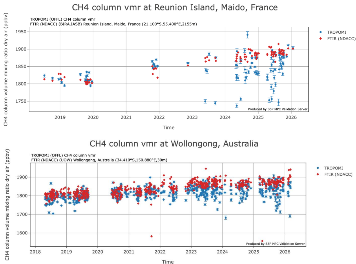
Figure 92: S5P L2_CH 4 XCH 4 time series over La Réunion where an increased number of low values of XCH 4 are observed for several days and especially more frequently as of February 2023 onwards.
