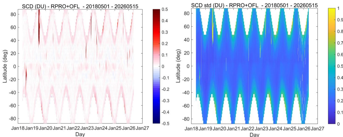
Figure 74: Zonal averaged time-series (for each day and 5° latitude bin) of SO 2 slant columns (left) and their standard deviation (right). (RPRO+OFFL data from May 2018 to May 2026). Courtesy Nicolas Theys (BIRA-IASB).
