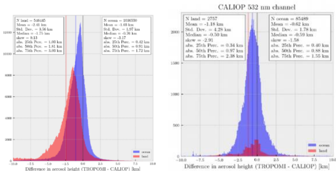
Figure 120: Histogram of differences between CALIOP weighted extinction height and TROPOMI ALH from collocated data between 1 May 2018 and 28 February 2019 (left). The right panel shows the same histogram, but for pixels that were screened for a minimal cost function (chi-squared) smaller than 1E5.
