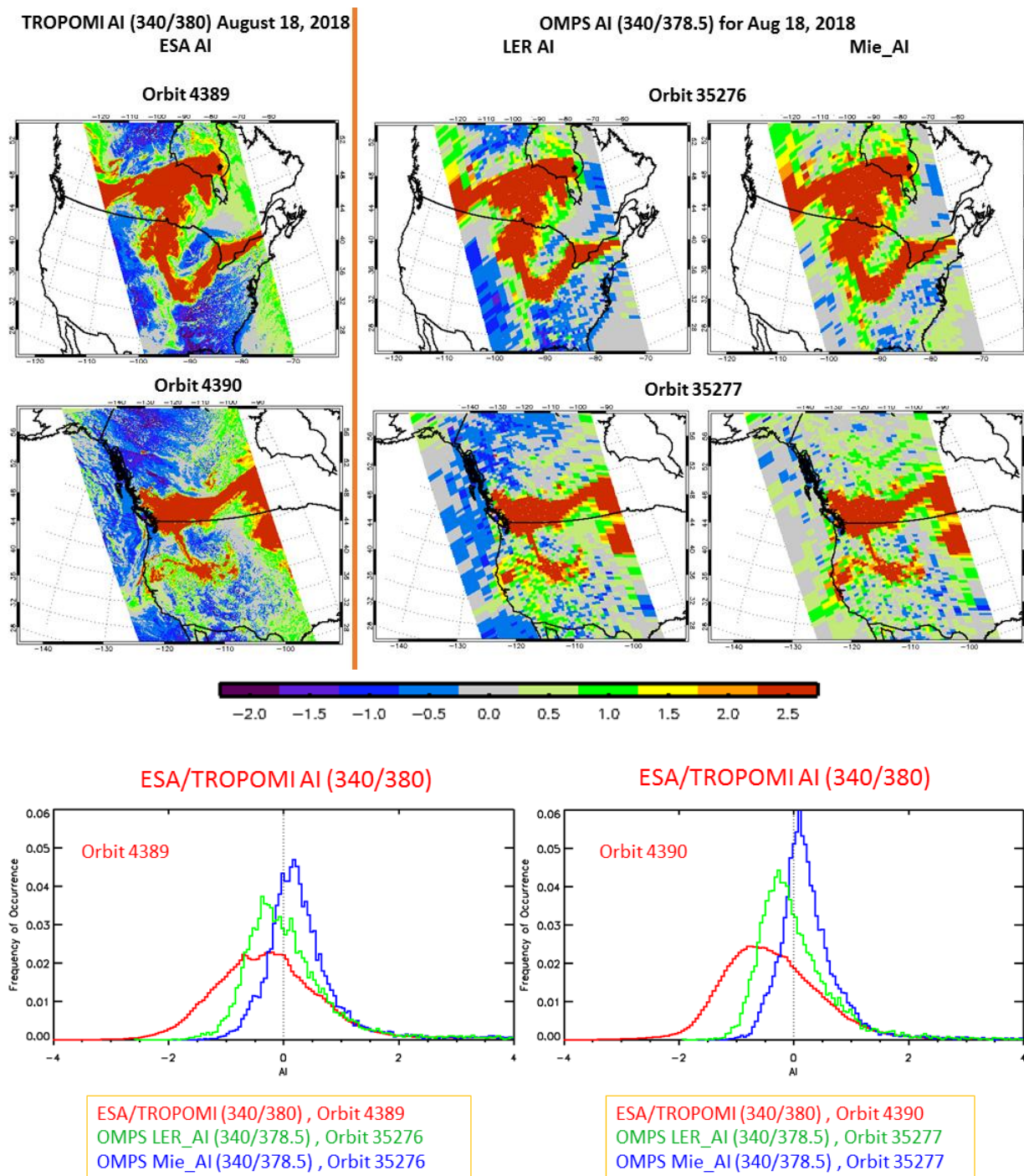
Figure 107: Comparison of UVAI from TROPOMI and OMPS for an observation of a biomass burning plume (18 Aug. 2018). For OMPS UVAI are calculated assuming either LER or Mie clouds. The UVAI for Mie clouds yields results that are more consistent. TROPOMI and OMPS LER results show very good agreement. However, the frequency distribution is broader for TROPOMI observations (courtesy of Omar Torres and Changwoo Ahn, NASA-GSFC).
