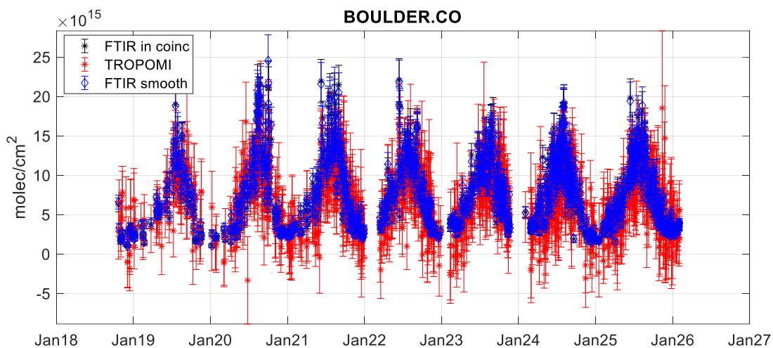
Figure 60: TROPOMI and FTIR HCHO column time series at Boulder. Period is May 2018 to January 2026.
