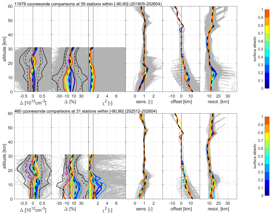
Figure 28: Comparison between S5P L2_O3_PR RPRO/OFFL ozone number density profile data and all co-located ground-based reference measurements (grey), originating from ozonesondes for L2 v02.04-09 covering eight full years of data (top, 2018/05 to 2026/04) and for v02.09 only (bottom, 2025/12 to 2026/04). Every plate shows six graphs, respectively, from left to right: the difference and the percent relative difference between S5P and reference data, the chi-square profile, the vertical sensitivity, the altitude registration offset, and the averaging kernel FWHM associated with the S5P retrieval. The coloured lines indicate median results for the surface albedo intervals shown in the colour scale. Black dashed lines show median values (thick lines) and standard deviations (thin lines, around the median), while magenta, dashed lines indicate the median difference between the a-priori profile and the reference measurement. Dotted black lines indicate the total ex-ante (inductive) uncertainty of TROPOMI and the reference measurements combined (around the median difference).
