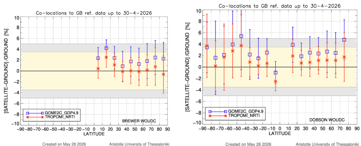
Figure 15: Comparison of the mean percentage differences between two satellite products (S5P TROPOMI L2_O3 NRTI and GOME-2C GDP4.9) and ground-based total ozone data, versus latitude. The Brewer network comparisons are shown in the left-hand panel, and the Dobson network comparisons are depicted in the right-hand panel, both datasets are downloaded from WOUDC. The period of data is July 2022 – April 2026 (limited by ground-based data availability).
