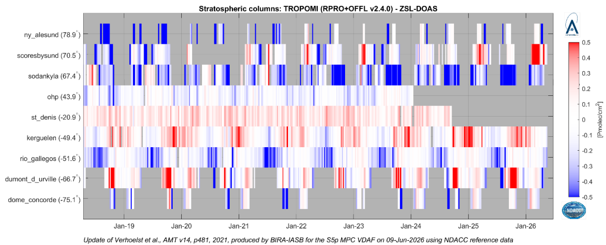
Figure 41: Time series – from May 2018 until May 2026 – of S5P RPRO+OFFL L2_NO 2 and NDACC ZSL-DOAS NO 2 stratospheric column differences, weekly averaged [Pmolec/cm 2 ]. For the current report, only the SAOZ data sets covering (mostly) the full mission lifetime are shown.
