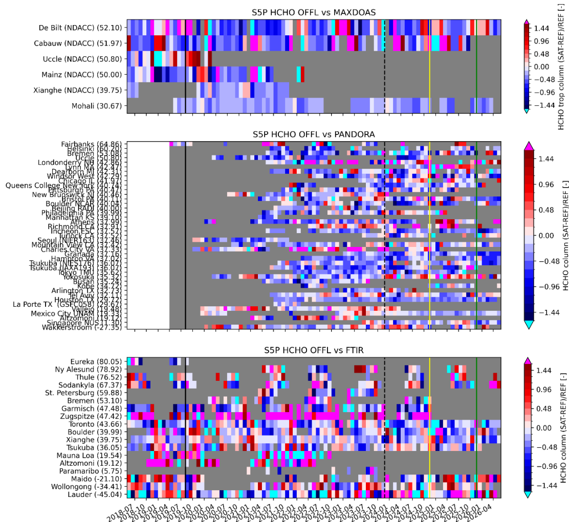
Figure 53: Time series of monthly mean relative differences [%] of S5P OFFL/RPRO V02.04.01-02.06.01 HCHO versus MAXDOAS, PANDORA, and FTIR. Data was obtained from the VDAF Automated Validation Server until 2026/05/31. Indicated are the pixel size switch (2019/08/16), the update to v2.6.1 (2023/11/26), the update to v2.7.0 (2024/11/16) and the update to v2.8.0 (2025/11/22).
