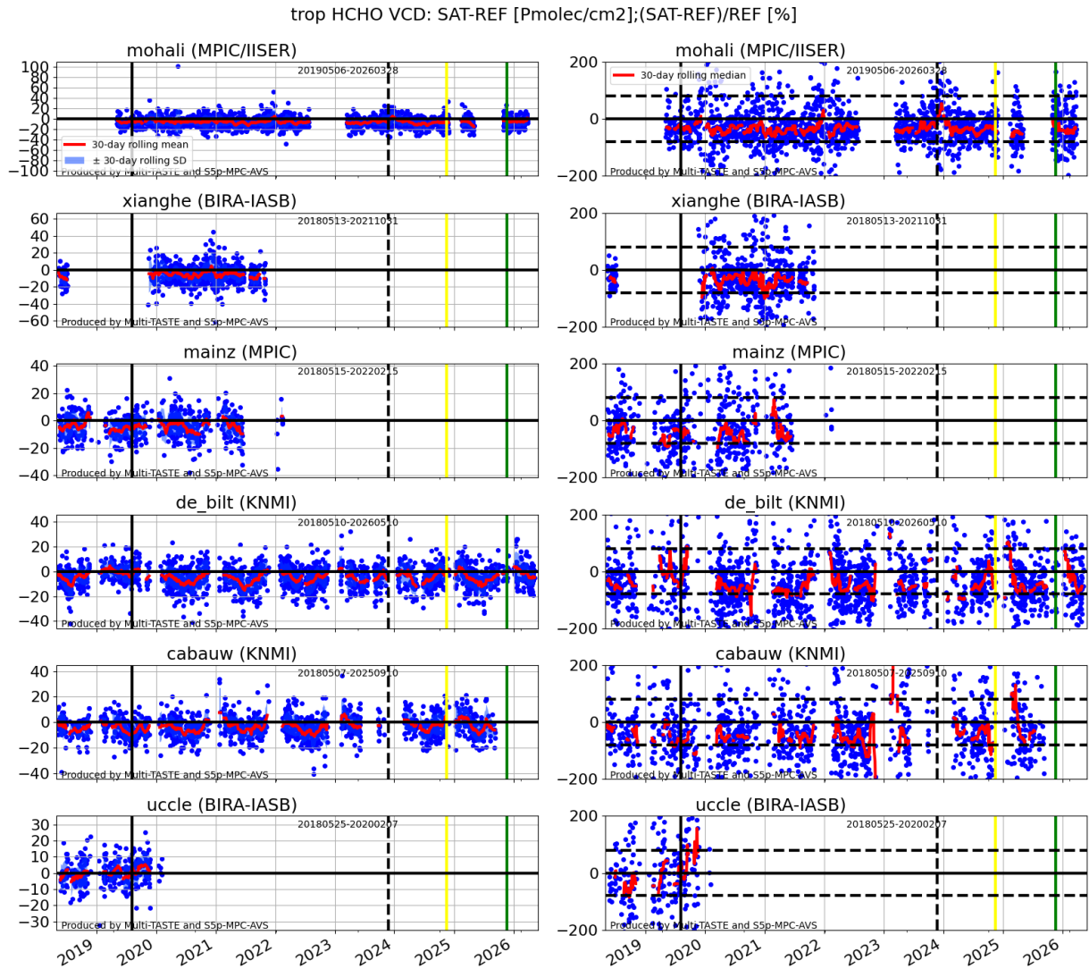
Figure 55: Time series of the difference [Pmolec/cm 2 ] and relative difference [%] between S5P RPRO+OFFL and MAX-DOAS HCHO column data at six stations. Data was obtained from the VDAF Automated Validation Server until 2026/05/31. Indicated are the pixel size switch (2019/08/16) the update to v2.6.1 (2023/11/26) to v2.7.0
