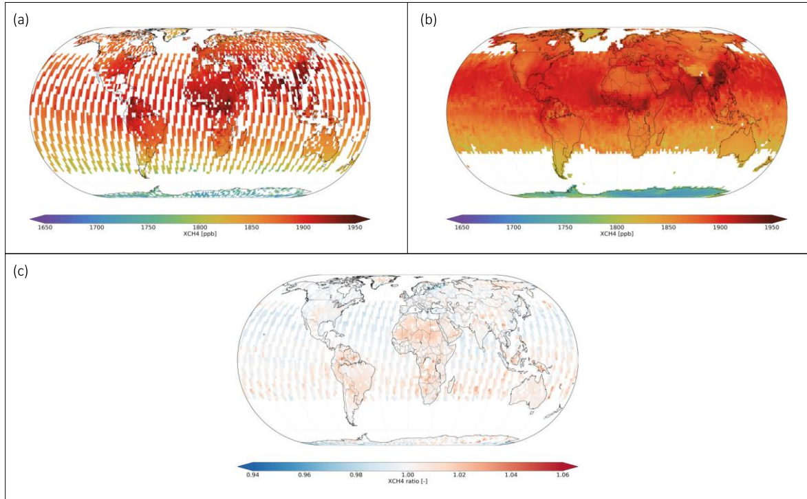
Figure 85: Global distribution of XCH 4 measured by (a) GOSAT and (b) TROPOMI and (c) the ratio of GOSAT to TROPOMI XCH 4 . Daily collocations are averaged to a 2x2 degree grid for the year 2022.
