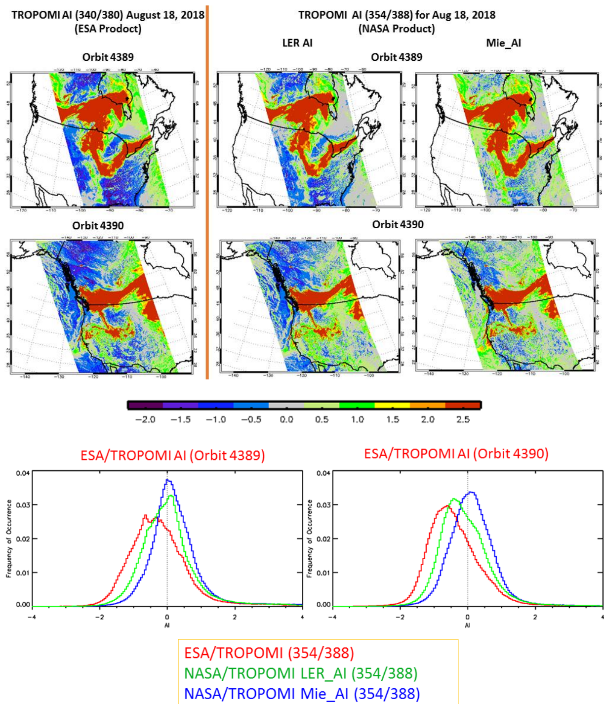
Figure 108: Comparison of UVAI from the operational TROPOMI UVAI product and TROPOMI UVAI analysed using the OMPS algorithm for an observation of a biomass burning plume (18 Aug. 2018). Like in the previous comparison, good agreement is found, but still the frequency distribution for the operational product is slightly broader than for the results using the OMPS algorithms (courtesy of Omar Torres and Changwoo Ahn, NASA-GSFC).
