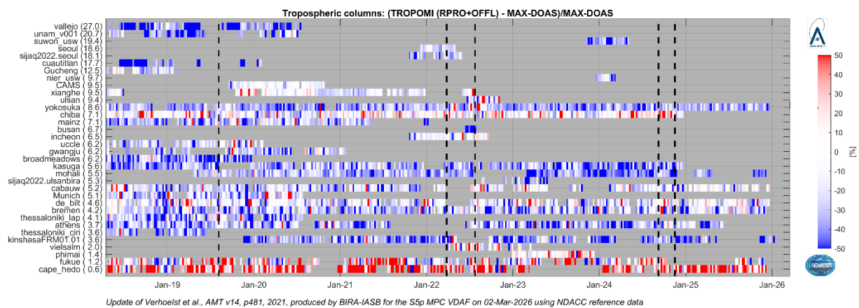
Figure 32: Time series – from May 2018 until end January 2026 – of the weekly averaged relative difference [%] between S5P RPRO+OFFL v02.04/02.05/02.06/02.07/02.08/02.09 and MAX-DOAS NO 2 tropospheric column data. Stations are ordered by median tropospheric column, in brackets.
