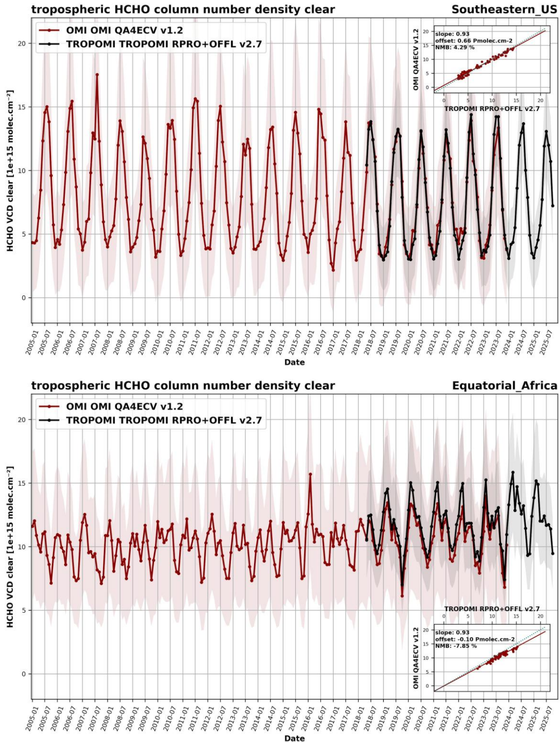
Figure 58: Example of monthly averaged HCHO columns ( tropospheric HCHO column number density clear ) retrieved from OMI (2005–2023, in red) and TROPOMI collection 3 (2018–2025, in black) over two regions: South-eastern US (top) and Equatorial Africa (bottom). Statistical results of a regression line between OMI and TROPOMI observations are provided inset each plot.
