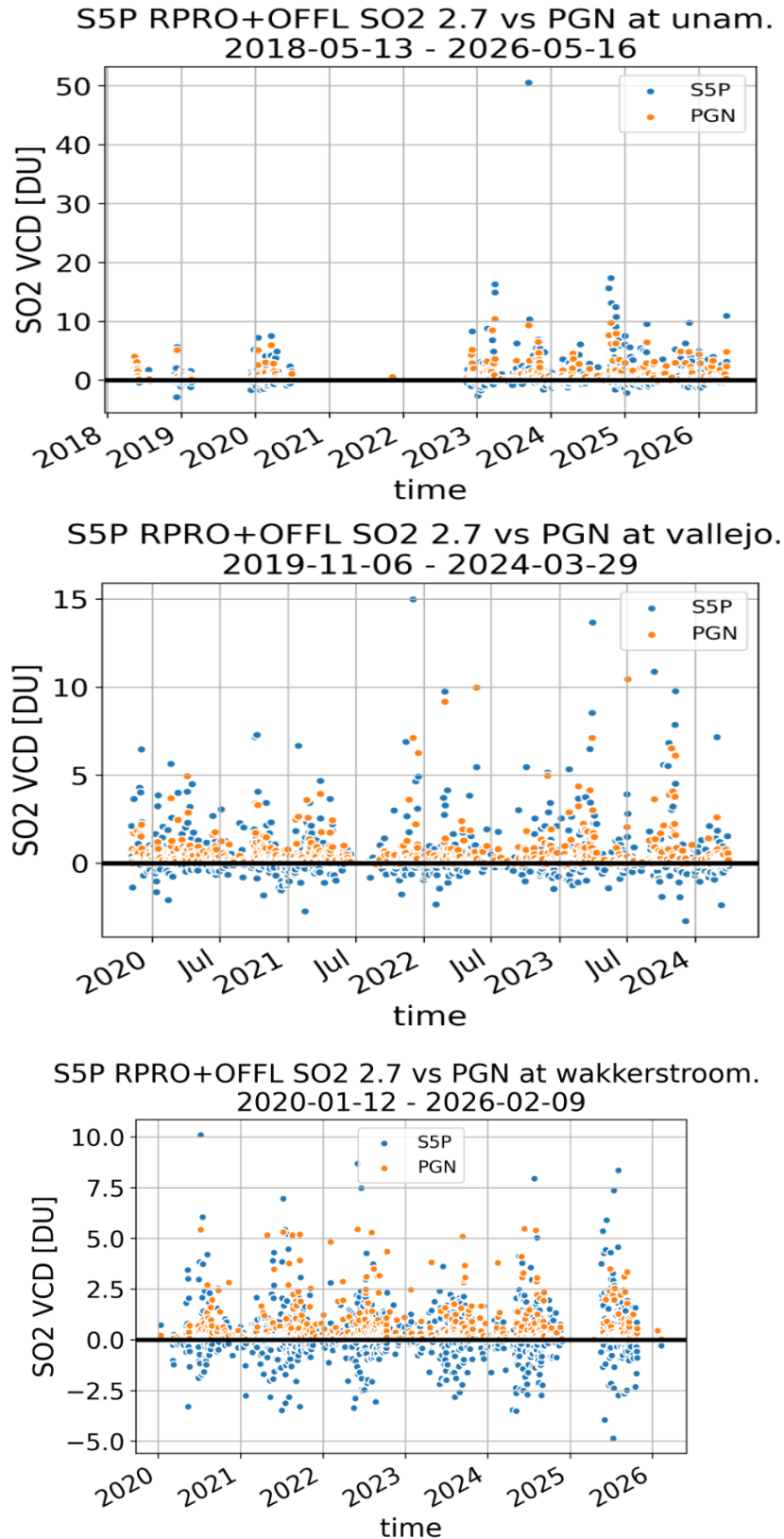
Figure 73: Comparison of TROPOMI SO 2 VCDs (RPRO and offline) to Pandora measurements (daily means) at Observatorio Atmosferico Altzomoni, UNAM, Mexico (3985m altitude), Vallejo (Mexico City), and Wakkerstroom to ground-based reference measurements from the Pandonia Global Network. Courtesy Steven Compennolle (BIRA-IASB).
