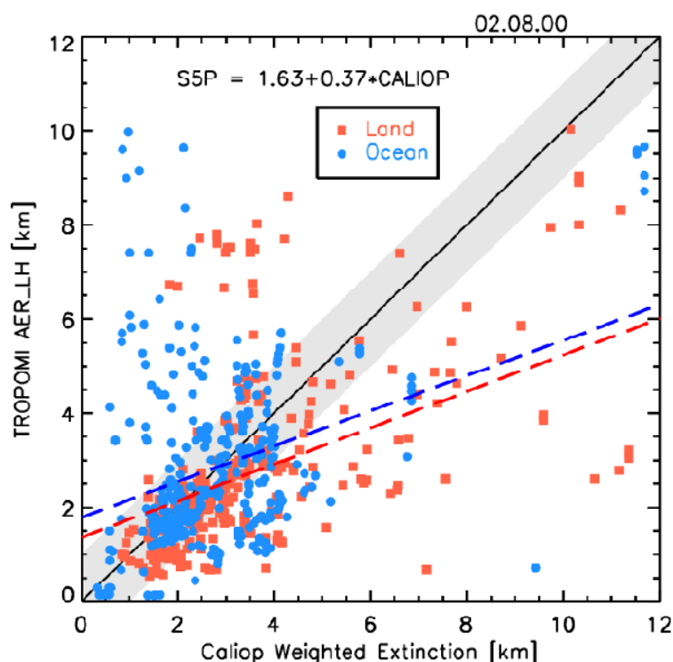
Figure 118: Comparison of ALH from TROPOMI and CALIOP weighted extinction height for the cases presented. Pixels over land are plotted in orange and pixels over water in blue.
