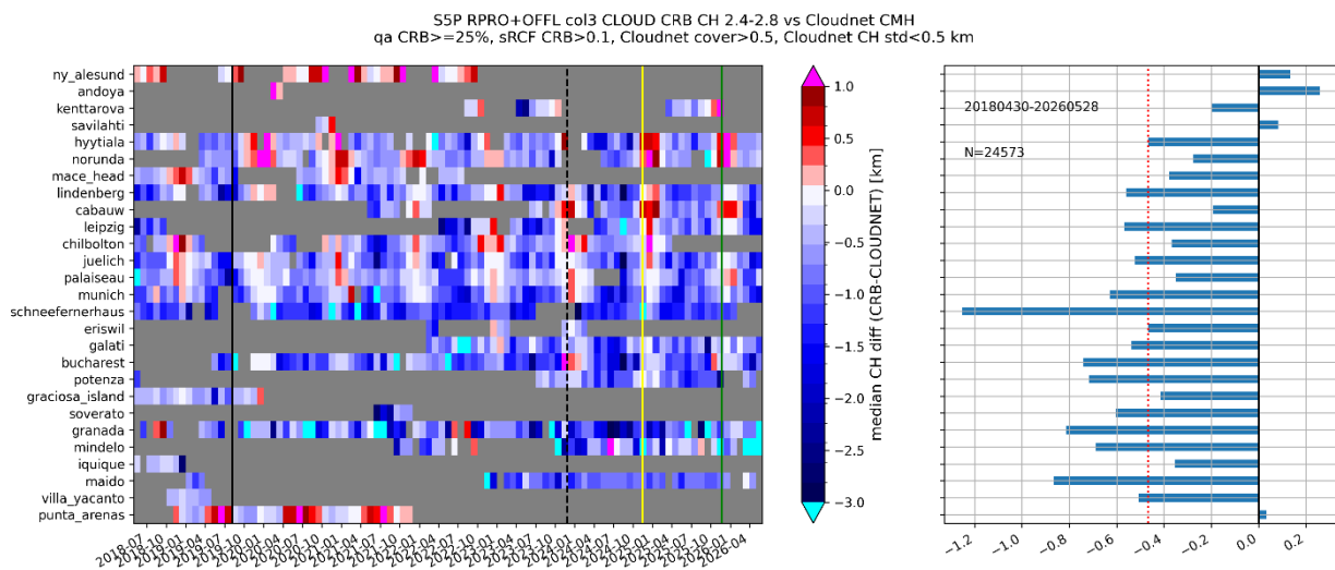
Figure 102: Upper panel: Boxplots of S5P L2_CLOUD CRB RPRO+OFFL CH minus CLOUDNET CH (upper left) and of the relative difference (upper right), per station. The same conventions as for Table 13 apply. Sensing time range is indicated on the figure. Bottom left panel: monthly median of CLOUD CRB CH-CLOUDNET CMH, per station. Pixel size switch (2019/08/06) and the following updates CLOUD v2.6.1 (2023/11/26), v2.7.0 (2024/11/16), and v2.8.0 (2025/11/22) are indicated on the plot. Bottom right panel: median difference per station. The dashed red line indicates the median over the median differences.
