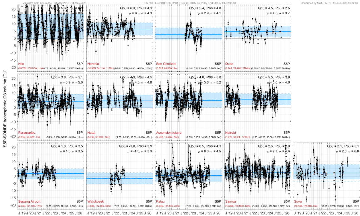
Figure 23: Time series of the absolute difference between spatially and temporally co-located S5P and ozonesonde tropospheric O 3 column data at 13 SHADOZ sites. The blue line and shaded area show the median value and the range between the 16 % and 84 % percentiles. Positive values indicate a high bias of S5P w.r.t. the reference.
