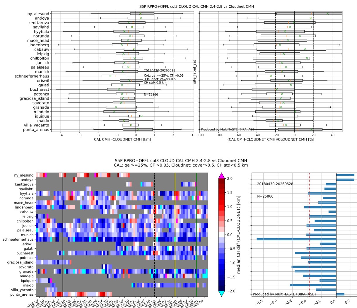
Figure 101: Top panel: Boxplots of S5P L2_CLOUD CAL CMH minus CLOUDNET CMH, per station. Boxplot conventions: box bounds are at first and third quartile. Orange line is median. Whiskers are at 5 and 95 percentiles. Green cross is mean. Right panel: Similar as upper panel but now for the relative difference. Sensing date range is indicated on the plot. Bottom left panel: monthly median of CLOUD CAL CMH-CLOUDNET CMH, per station. Pixel size switch (2019/08/06) and the following updates: CLOUD v2.6.1 (2023/11/26), CLOUD v2.7.0 (2024/11/16), and v2.8.0 (2025/11/22) are indicated on the plot. Right panel: median difference per station. The red dashed line gives the median over the median differences.
