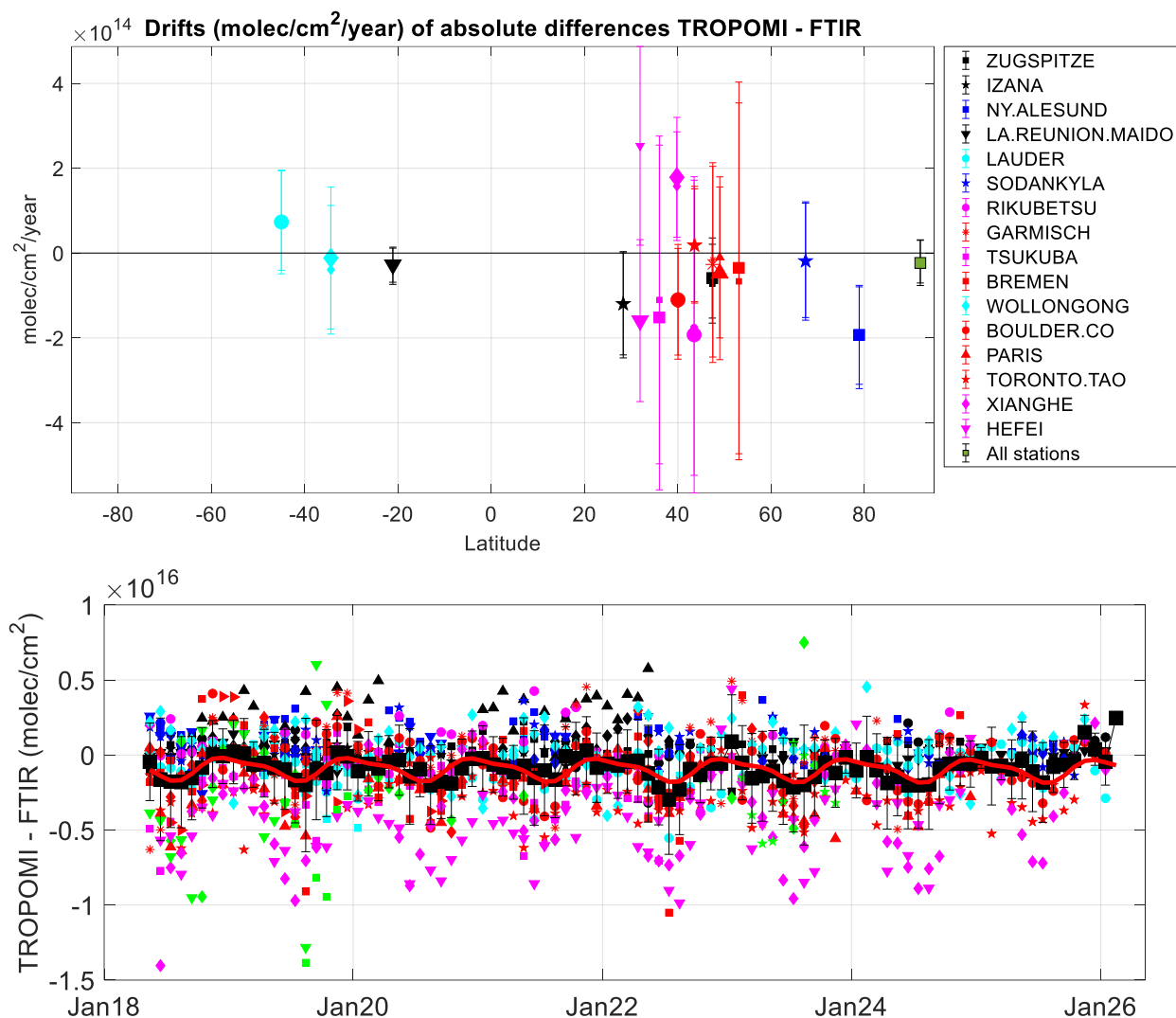
Figure 68: a (top panel): Drifts (trends in the absolute differences between the monthly means of TROPOMI and FTIR data. The smaller markers are for direct comparisons (no smoothing) and the larger ones are with smoothing (Rodgers and Connor 2003). The drift when all stations are considered simultaneously is added (92 latitude). b (bottom panel): all monthly means differences at individual sites and in black squares with error bars are shown the means of the differences (between TROPOMI and smoothed FTIR) at all sites for each month. The red curve is the regression model which includes a trend and a seasonal cycle.
