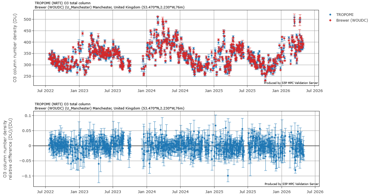
Figure 19: Time series of S5P TROPOMI NRTI (v2.4.1 and higher) and Brewer total ozone data (and their differences) at the station of Manchester in the United Kingdom (data courtesy J. Rimmer, University of Manchester).
