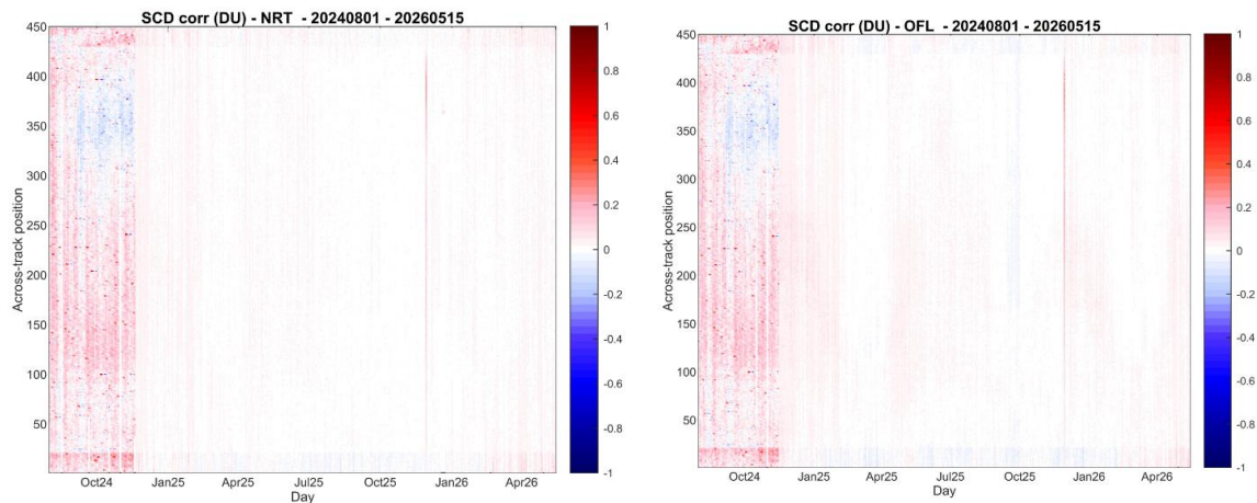
Figure 75: Time series of background corrected SO 2 SCDs (left: NRT, right: OFFL) for all 450 detector rows from August 2024 to May 2026. Most of the short time features (vertical stripes) are caused by individual volcanic eruptions. The strong reduction of the noise after November 2024 represents the change to the new COBRA SO 2 product. (courtesy of Nicolas Theys, BIRA-IASB).
