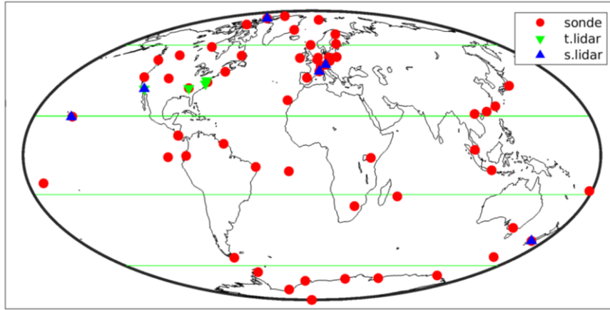
Figure 27: Geographical distribution of the ozonesonde and tropospheric (t.) and stratospheric (s.) lidar stations with which co-locations with S5P L2_O3_PR data have been identified and used in the data comparisons reported hereafter.
