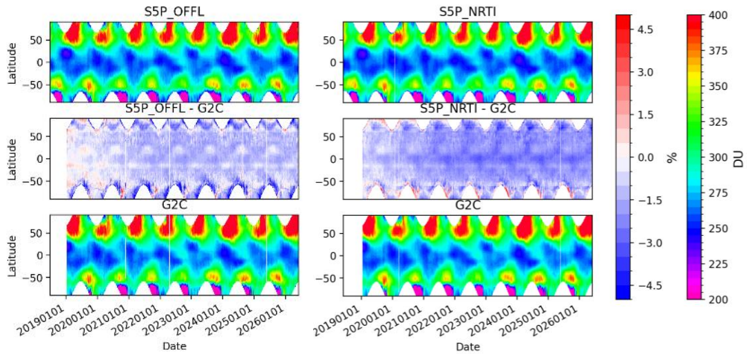
Figure 21: Zonal mean comparison between S5P TROPOMI and Metop-C GOME 2 total ozone columns, for both OFFL (left-hand panel) and NRTI (right-hand panel).
