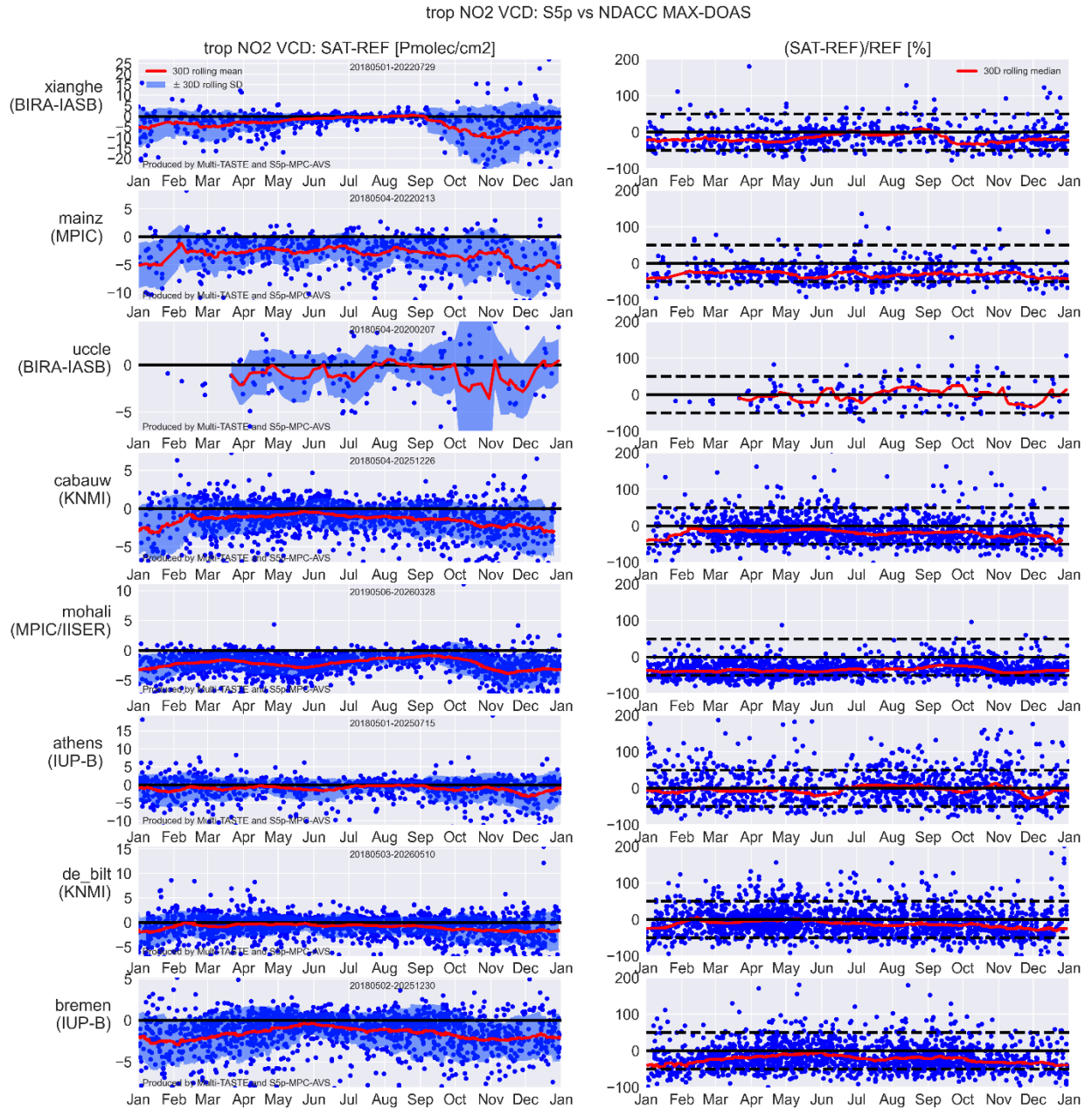
Figure 37: Seasonal cycle (with data mapped to one generic year) of the difference between S5P RPRO+OFFL and MAX-DOAS NO 2 tropospheric column data at eight stations. Difference (left) and relative difference (right). On the left column, the lowest 2.5 % data is not shown for visibility. Data was obtained from the VDAF Automated Validation Server on 2026/06/03.
