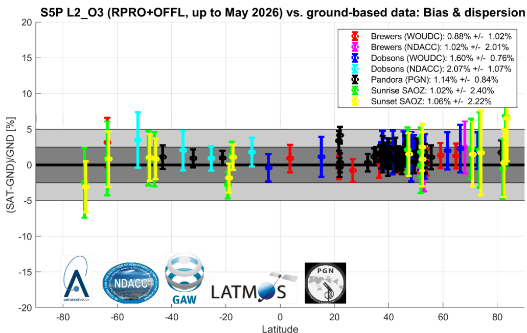
Figure 4: Meridian dependence of the median (the circular markers) and spread ( \pm 1 sigma, the error bars) of the percent relative difference between S5P TROPOMI L2_O3 (RPRO+OFFL up to May 2026) and ground-based (GND) ozone column data, represented at individual stations from the Antarctic to the Arctic and per measurement type. The values in the legend correspond to the median and spread of all median (per station) differences. For clarity, sunrise and sunset ZSL-DOAS results are represented separately (offset by -0.5° and +0.5° in latitude).
