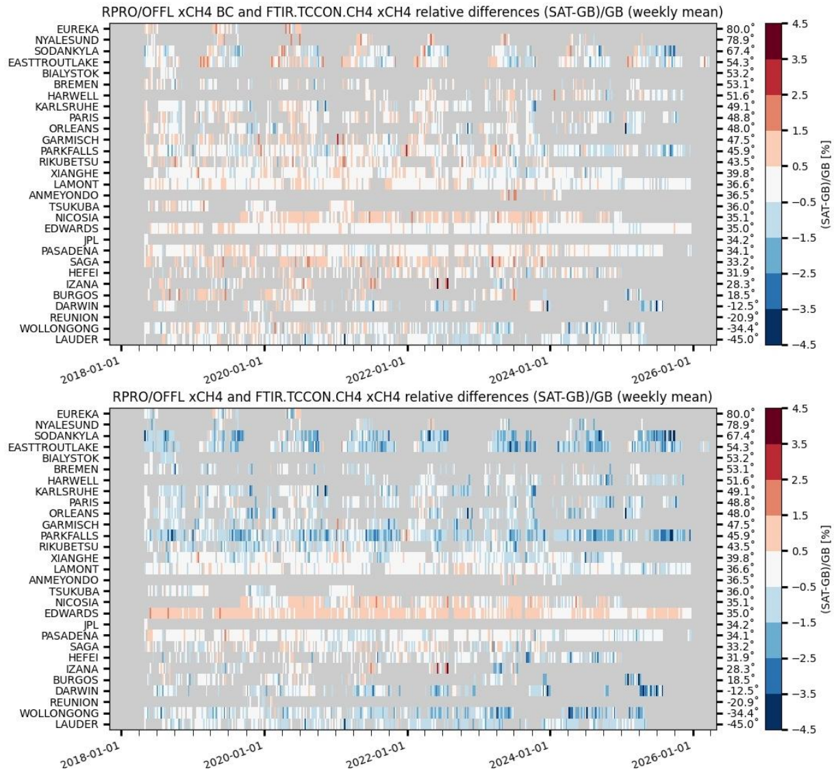
Figure 88: Mosaic plots of relative biases between S5P L2_CH4 RPRO+OFFL and ground-based CH4 TCCON column data for the bias corrected (top) and standard (bottom) methane products. Over the April 2018 – April 2026 period the plots do not show a clear meridian dependence or temporal change in the weekly averaged biases. Colour bar gradients are chosen such that they match with the measurement's uncertainties.
