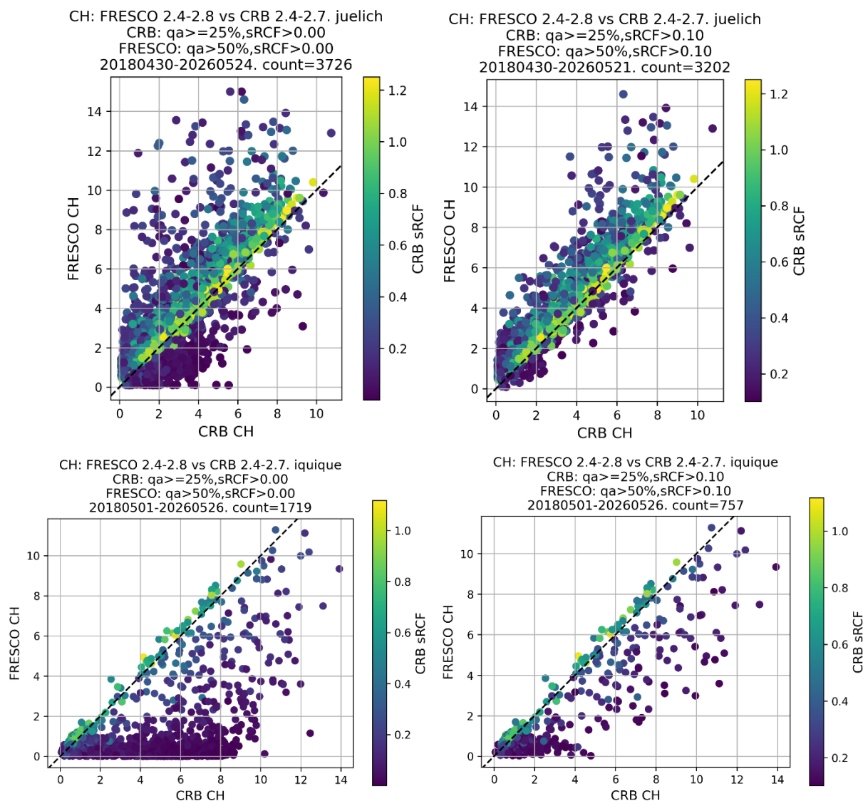
Figure 105. Scatter plot between FRESCO and CLOUD CRB cloud height, with points colored according to CRB sRCF, for the sites Juelich and Iquique, and for two screening settings: sRCF > 0. For both CRB and FRESCO, and sRCF > 0.1 (which is the default to calculate bias and dispersion).
