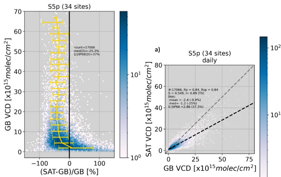
Figure 33: Left: 2D-histogram of S5P vs MAX-DOAS relative difference. The yellow line with error bar represents the median with [P16, P84] dispersion, per MAX-DOAS NO 2 VCD bin. Right: scatter density plots for the daily median comparisons from May 2018 until end January 2026 between S5P RPRO+OFFL v02.04-09 and MAX-DOAS NO 2 tropospheric column data.
