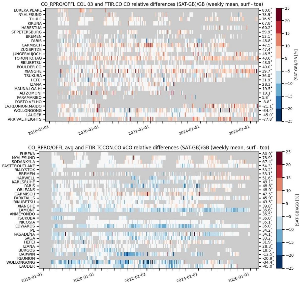
Figure 82: Relative bias between S5P L2_CO OFFL and ground-based CO column data at NDACC (top), TCCON (bottom) FTIR stations. Over the April 2018 – April 2026 period the plots do not show a clear meridian dependence or temporal change in the weekly averaged biases. Colour bar gradients are chosen such that they match with the measurement's uncertainties.
