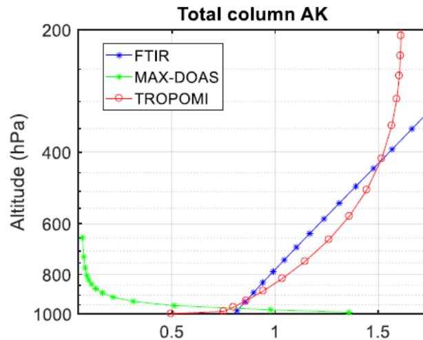
Figure 57: Typical total column averaging kernels for S5P TROPOMI and the two ground-based instrument types: FTIR (blue), MAX-DOAS (green), and TROPOMI (red). This illustrates the problem of the vertical smoothing difference error in these comparisons, as the instruments “see” different parts of the column.
