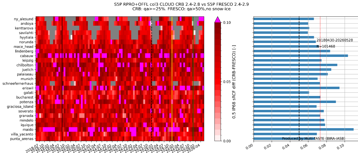
Figure 98. Left. Monthly \frac{1}{2} IP68 of scaled cloud fraction difference of CLOUD OFFL vs FRESCO OFFL, per month and per station. Indicated is the pixel size switch (2019/08/06) and the following updates: CLOUD v2.6.1 & FRESCO v2.6.0 (2023/11/26), FRESCO v2.7.1 (2024/09/11), CLOUD v2.7.0 & FRESCO v2.8.0 (2024/11/16), and CLOUD v2.8.0 & FRESCO 2.9.1. Right: \frac{1}{2} IP68 of scaled cloud fraction difference (CLOUD CRB-FRESCO), per station.
