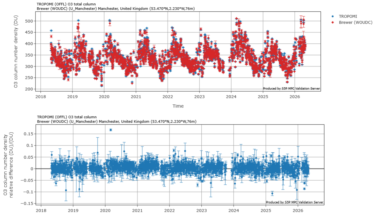
Figure 12: Time series of S5P TROPOMI OFFL and Brewer total ozone data (and their differences) at the station of Manchester in the United Kingdom (data courtesy J. Rimmer, University of Manchester).
