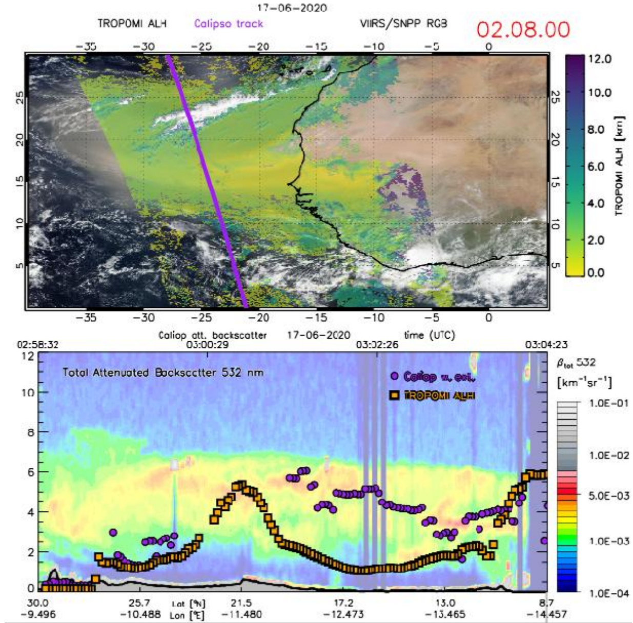
Figure 115: Same as above, but for 17 June 2020.
