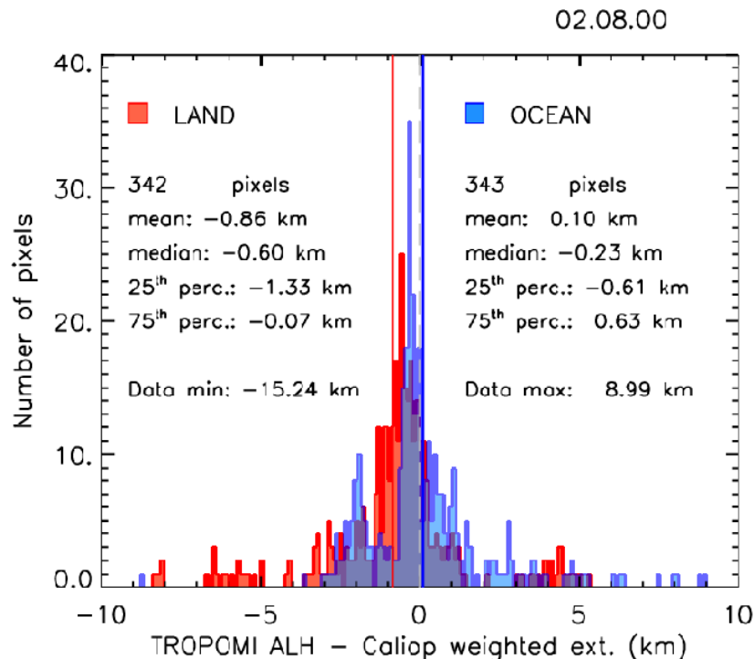
Figure 119: Histogram of the difference between the ALH from TROPOMI and CALIOP weighted extinction for the cases presented. Pixels over land are plotted in red and pixels over water in blue.
