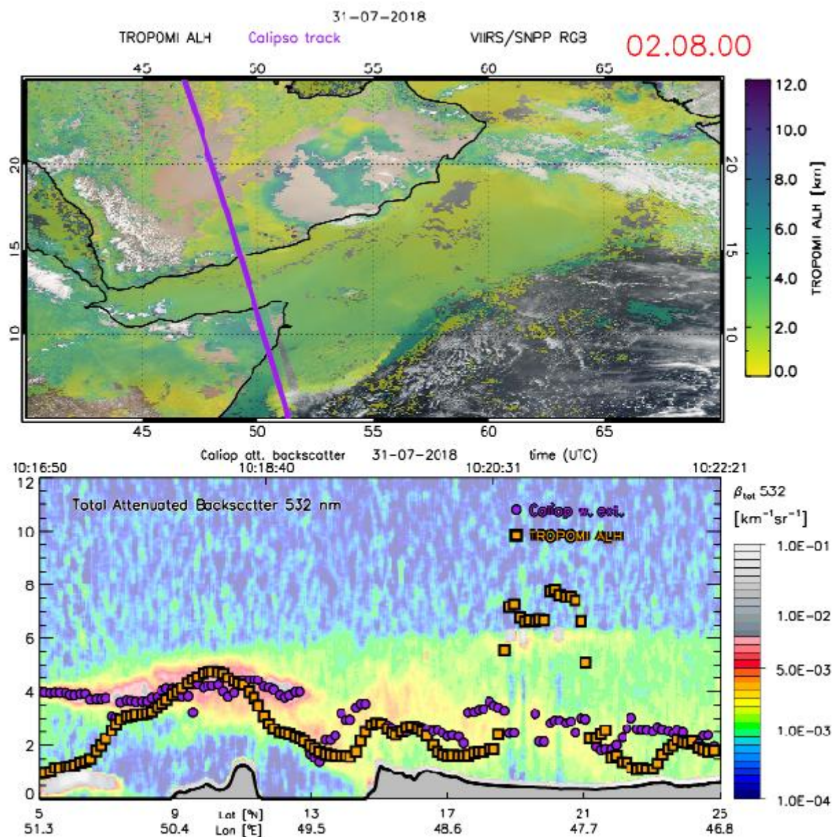
Figure 114: Same as above, but for 31 July 2018 near the Arabian Peninsula.
