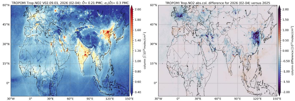
Figure 38: (Left) TROPOMI V02.09.01 tropospheric NO 2 mean columns (February to April 2026). The data is averaged in bins of 0.1° latitude/longitude for [-10°S, 60°N, -30°W, 150°E]. A qa_value > 0.75 and a cloud fraction CF < 0.2 are used to reduce the amount of data and exclude cloudy scenes. Columns are plotted as the third root of values to better cover the dynamics. (Right) The absolute column difference of the period from the left figure subtracted by the same period from one year before.
