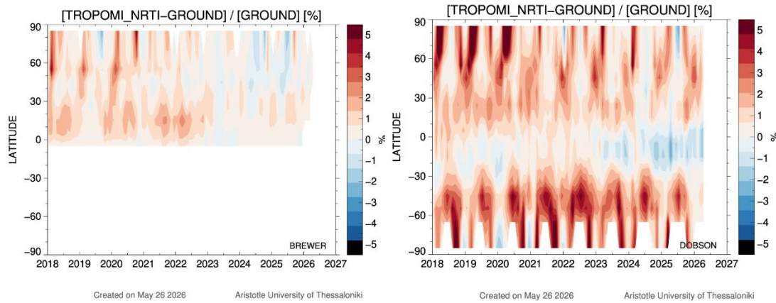
Figure 16: Time and latitude resolved analysis of the differences between NRTI total ozone and Brewer measurements (left-hand panel) and Dobson measurements (right-hand panel). Strong seasonal features in the Dobson comparisons are due (1) to the use of a fixed effective temperature in the Dobson measurement processing, and (2) due to the poorer representation of difficult surface albedo conditions before the adoption of the GE_LER surface albedo product in July 2020.
