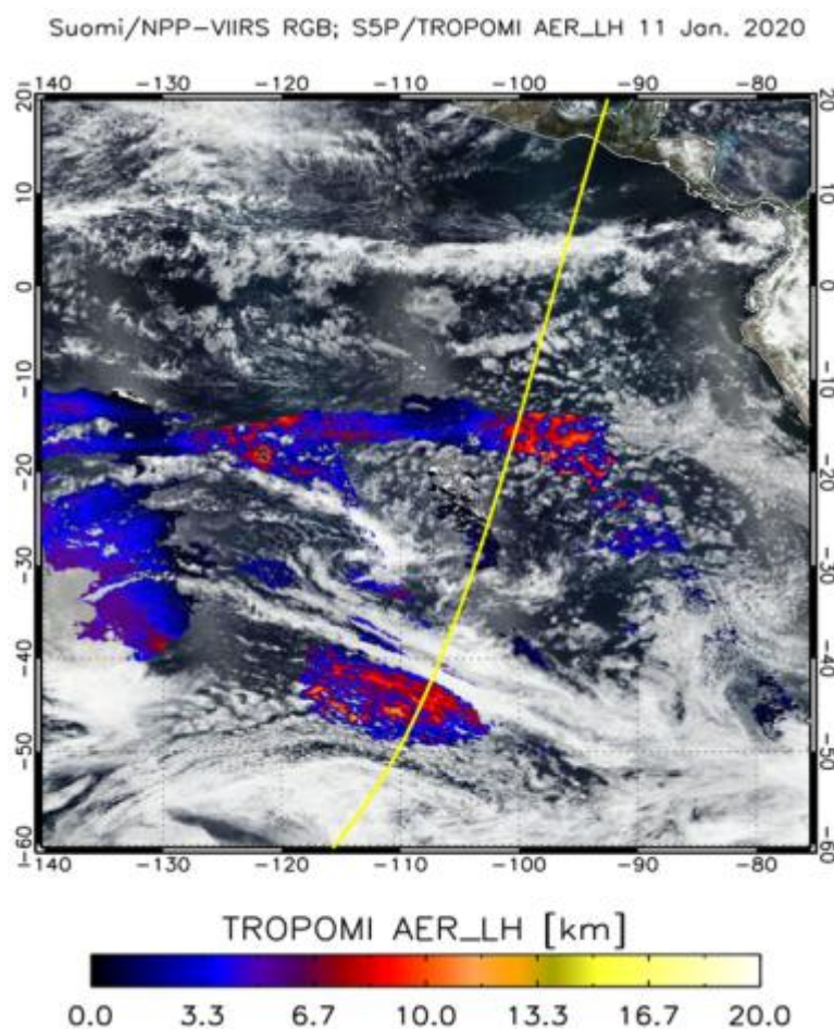
Figure 125: NPP/VIIRS RGB image with S5P/TROPOMI AER_LH on 11 January over the south Pacific with the CALIPSO track of that day overlaid in yellow.
