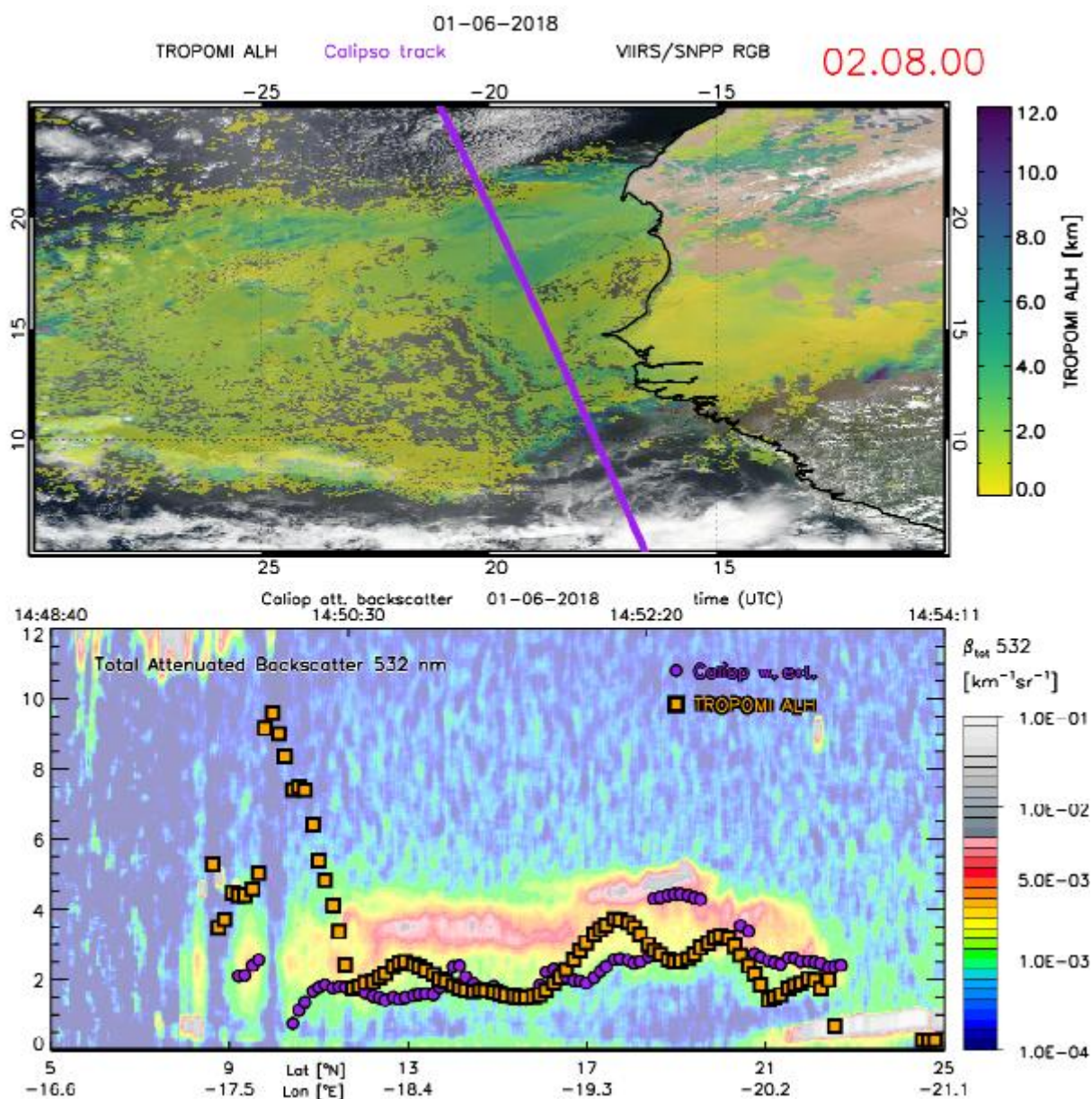
Figure 113: ALH (v02.08.00) for a desert dust case on 1 June 2018 retrieved by TROPOMI (top panel) and the CALIOP total attenuated backscatter image (bottom panel). The purple line and dots show the CALIPSO track and CALIOP weighted extinction averaged along the track, respectively. In the bottom panel the ALH retrieved by TROPOMI along the CALIOP orbit track is shown by the orange squares.
