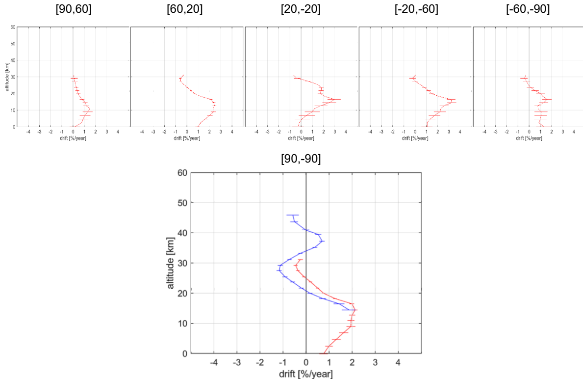
Figure 30: Comparison between S5P RPRO/OFFL ozone profiles for eight full years of data (v2.4-9, May 2018 to April 2026) and co-located ozonesonde data in five latitude zones (top, Arctic to Antarctic). Every column shows the linear temporal drift within the latitude band specified above. Global drift results for ozonesonde (red, 60 stations) and stratospheric lidar (blue, 6 stations) comparisons for the same eight years of data are shown in the bottom plot. Horizontal bars in the drift plots indicate 2-sigma uncertainty estimates on the drift using a bootstrapping technique with 1000 samples.
