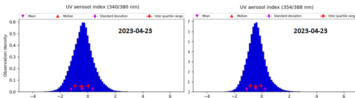
Figure 110: Frequency distribution of the UVAI (left: 340/380nm, right: 354/388 nm) for April 23, 2023.
