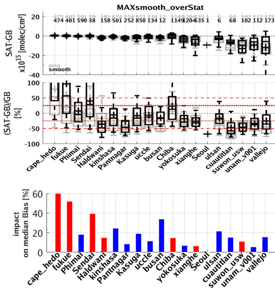
Figure 34: Box-and-whisker plots summarizing the bias and spread of the difference between S5P TROPOMI RPRO+OFFL v2.4/2.5/2.6/2.7/2.8 and MAX-DOAS NO 2 tropospheric columns (grey) and the smoothed MAX-DOAS NO 2 tropospheric columns (black). The third panel presents bar plot summarizing the change on the median bias between the original comparisons and the smoothed ones. Absolute values of the relative median biases are shown, where reductions are marked in blue bars and increases in red bars. The period is from May 2018 to end December 2024 for all available data. A vertical solid line inside the box, which marks the 25 and 75% quantiles, represents the median difference. The whiskers cover the 9-91% range of the differences and the crosses denote the mean differences.
