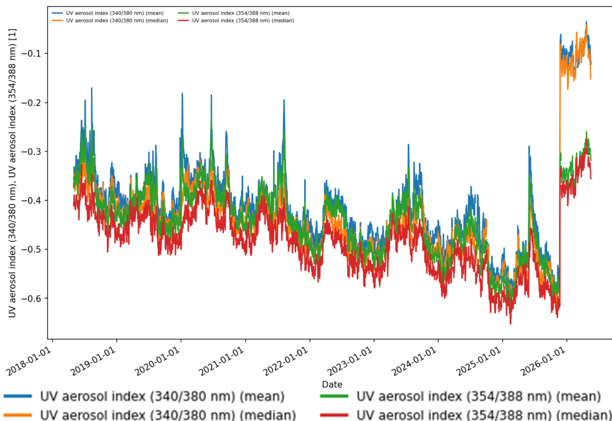
Figure 109: Comparison of the global daily mean and median for both L2_AER_AI UVAI wavelength pairs (340/380 and 354/388 nm), for the reprocessed data set from 20 July 2018 through 17 May 2026. Starting with version 2.9.1 (Nov 2025), a positive offset has been introduced due to a change in the lookup table (LUT) where the NO 2 absorption has been included. This change is being evaluated and will be updated in a future version of the data processor (likely Q4 2026) and prior to any reprocessing activity to ensure a consistent data record for the entire mission.
