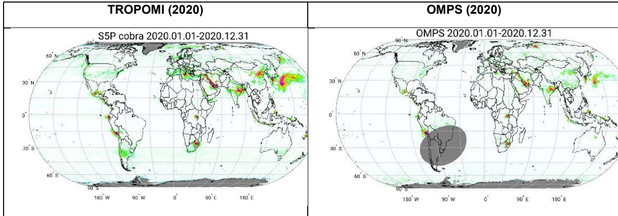
Figure 70: Comparison of TROPOMI (left) and OMPS (right) average SO 2 vertical columns for the year 2020 at the global scale. Courtesy Nicols Theys (BIRA- IASB).
