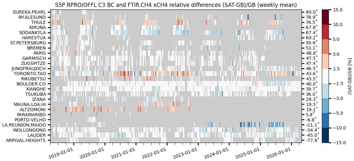
Figure 89 Mosaic plots of relative biases between S5P L2_CH4 RPRO+OFFL and ground-based CH 4 NDACC column data for the bias corrected methane products. Over the April 2018 – April 2026 period the plots do not show a clear meridian dependence or temporal change in the weekly averaged biases. At Maïdo and Wollongong an increased number of negative outliers are observed.
