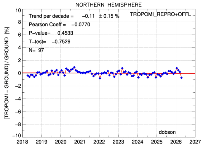
Figure 11: Drift assessment of S5P OFFL total ozone columns versus all Dobsons in the Northern hemisphere, based on de-seasonalized differences (accounting for the seasonal cycle in the differences induced by the assumed constant effective temperature in the Dobson processing).
