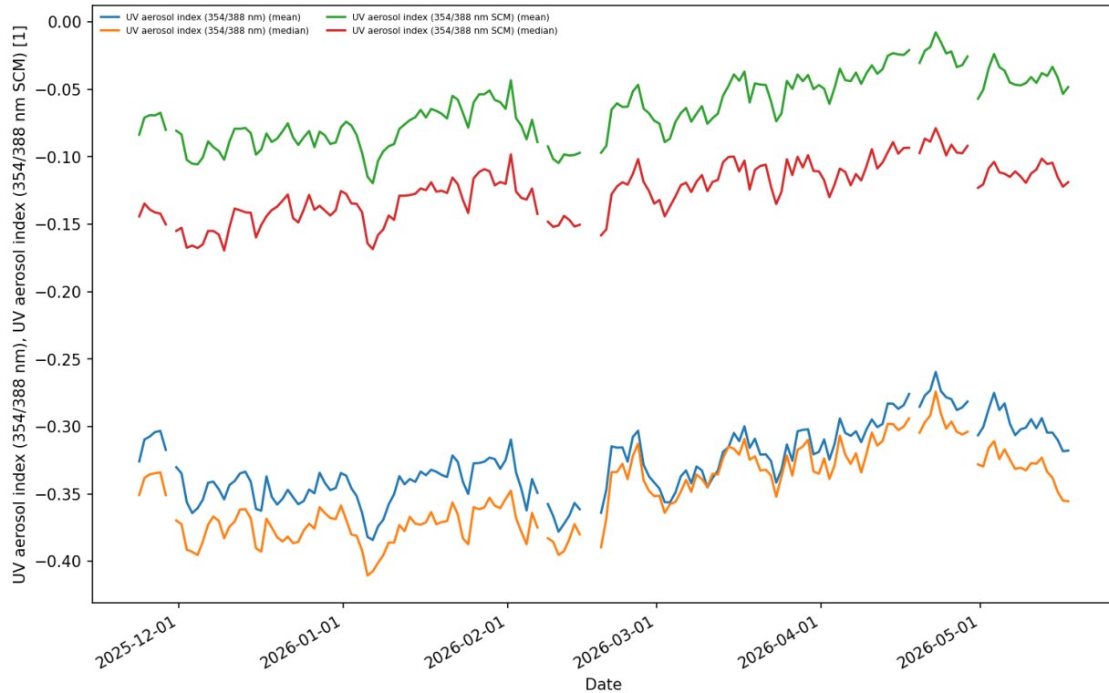
Figure 111: Comparison of the global daily mean and median aerosol index for the pair 354/388 calculated using a scattering cloud model with the standard UVAI for the same pair (Nov 2025 to May 2026).
