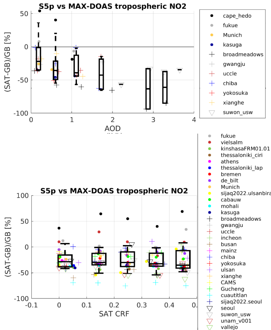
Figure 35: Relative differences between S5p TROPOMI RPRO+OFFL and MAX-DOAS NO 2 tropospheric columns as a function (upper panel) of MAX-DOAS AOD and (lower panel) S5p cloud radiance fraction (CRF). The time frame is from May 2018 until end of May 2025.
