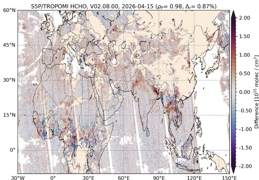
Figure 69: Difference between HCHO (v02.08.00) NRTI and OFFL column data for 2026-04-15 (binned to 0.1^\circ \times 0.1^\circ resolution). The difference is only calculated for columns above 0.5 \text{ Pmolec/cm}^2 and a qa\_value above 0.5.
