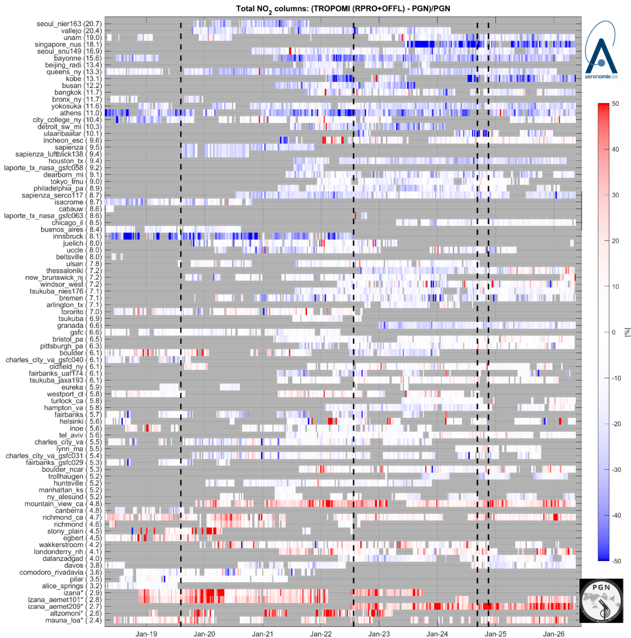
Figure 48: Time series – from May 2018 until May 2026 – of S5P RPRO+OFFL and PGN Pandora NO 2 total column differences, weekly averaged [%]. The black dashed lines indicate, respectively, the activation of the finer horizontal resolution and the switch between the RPRO and operational OFFL data. Stations are ordered by median total column, in brackets.
