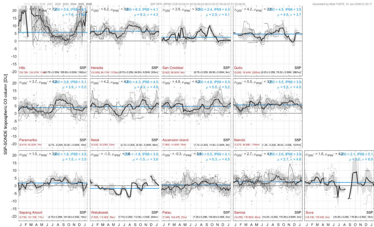
Figure 26: Annual cycle of the absolute difference between spatially and temporally co-located S5P and ozonesonde tropospheric O 3 column data. Individual comparison pairs are grey-shaded by year. Lines indicate the 29-day moving mean of the absolute difference for each year individually (thin grey) and all years combined (thin black). The blue line shows the median value over all comparison pairs. Positive values indicate a high bias of S5P w.r.t. the reference.
