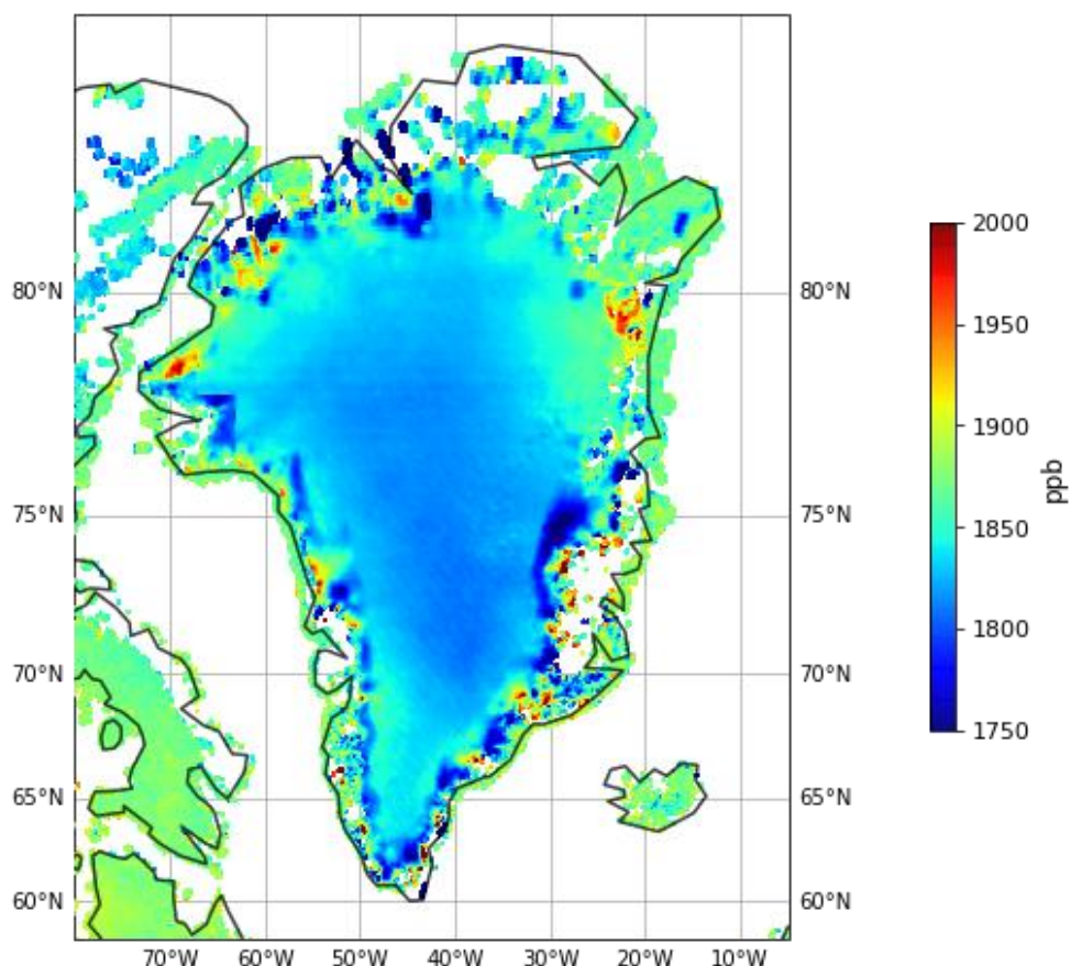
Figure 93: Map showing XCH 4 concentrations above Greenland and parts of North America for three years averaged data with pixels with qa_value > 0.5. The XCH 4 pixels in Greenland shows outliers along the mountain and coastline regions. Similar features are observed at the Antarctic.
