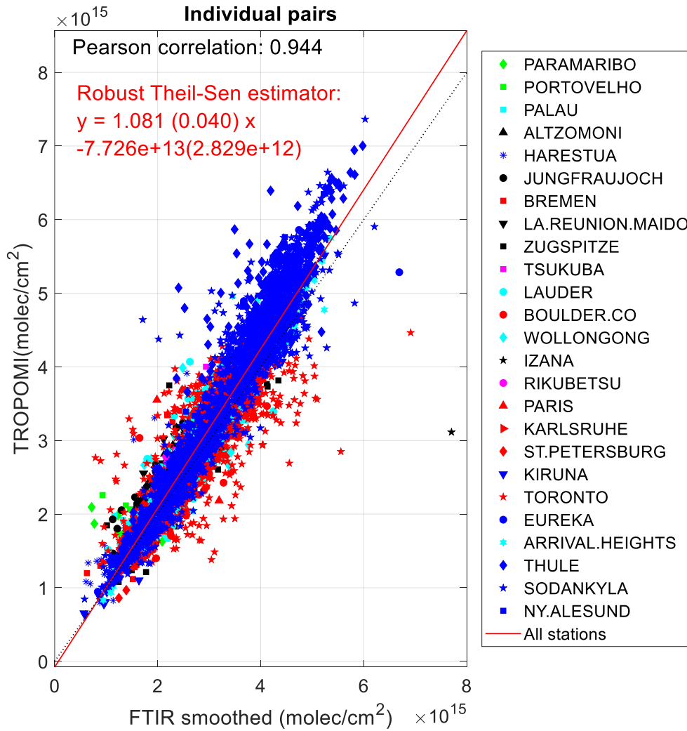
Figure 43: Scatter plot of co-located S5P TROPOMI and NDACC FTIR stratospheric NO 2 column data.
