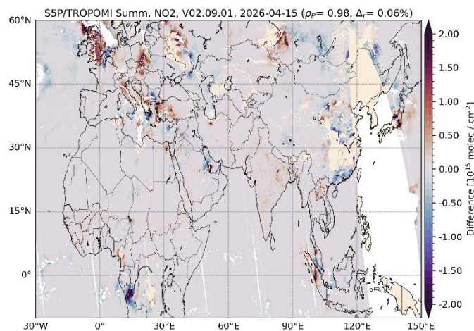
Figure 51: Difference between TROPOMI NRTI and OFFL V2.9.1 summed NO 2 columns for 2026-04-15. The difference is only calculated for columns > 0.5 Pmolec/cm 2 , cloud fractions < 0.6 and a qa_value > 0.5. Data is binned on 0.1° x 0.1° grid cells.
