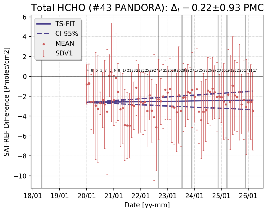
Figure 67: Time series – from January 2020 until April 2026 – of TROPOMI RPRO+OFFL and PGN Pandora HCHO column differences, monthly averaged over all station [Pmolec/cm 2 ]. The number of stations is superimposed. Vertical grey lines show the version changes. Blue lines show the Theil-Sen regression slope and 95% confidence interval.
