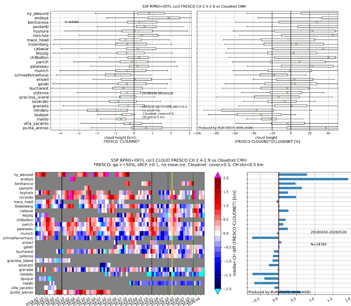
Figure 103: Upper panel: Boxplots of S5P L2_CLOUD FRESCO RPRO+OFFL v1.3-v1.4 CH minus CLOUDNET CH (upper left) and of the relative difference (upper right), per station. The same conventions as for Table 13 apply. Sensing time range is indicated on the figure. Bottom left panel: monthly median of FRESCO CH - CLOUDNET CH, per station. Pixel size switch (2019/08/06) and the following updates: FRESCO v2.6.0 (2023/11/26), v2.7.1 (2024/09/11), v2.8.0 (2024/11/16), and v2.9.1 (2025/11/22) are indicated on the plot. Bottom right panel: Median difference per station. The red dashed line indicates the median of the median differences.
