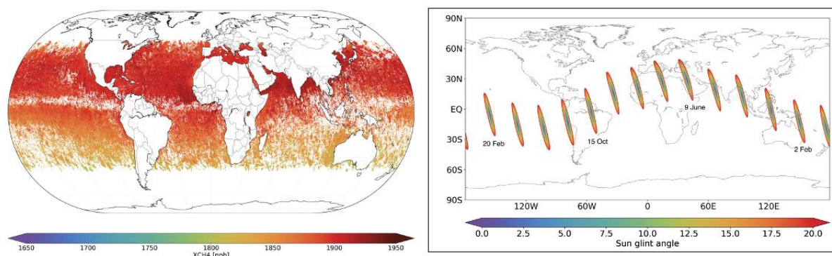
Figure 94: (left) Annual coverage of XCH 4 retrievals over the ocean for the year 2022, and (right) seasonal cycle of the sun-glint geometry.
