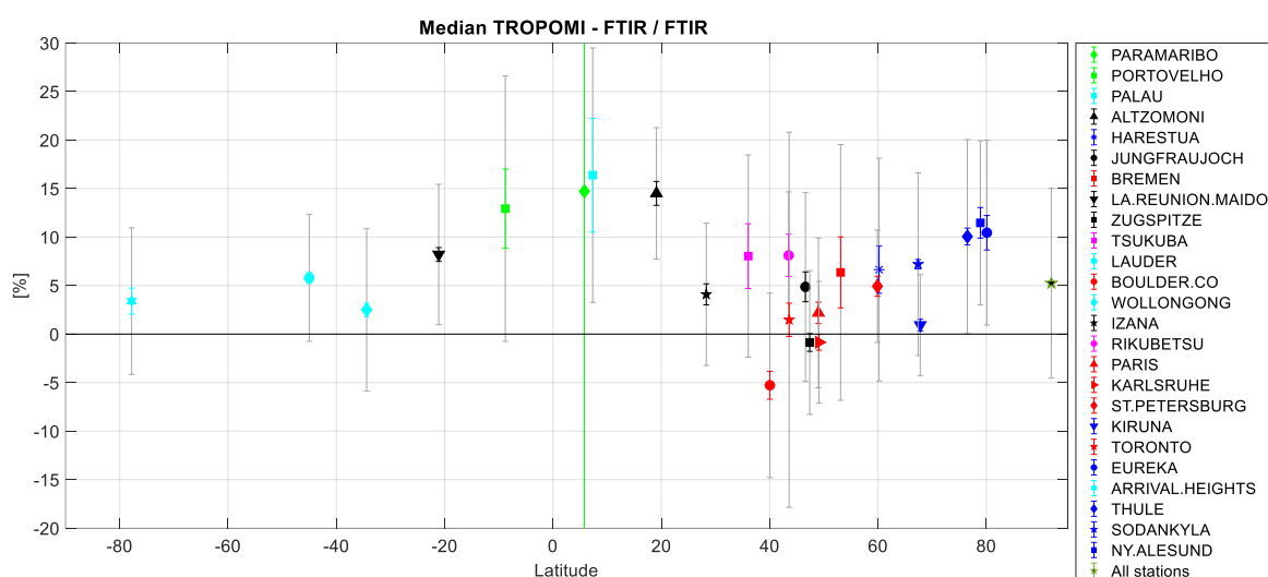
Figure 42: Median bias at each NDACC FTIR station as a function of latitude, calculated as the median of the percentage difference between S5P L2_NO 2 and the FTIR NO 2 stratospheric column measurement. The grey bars are the scaled MAD (see Sect. 6.2.1), and the coloured bars are the \pm 2\sigma error on the bias.
