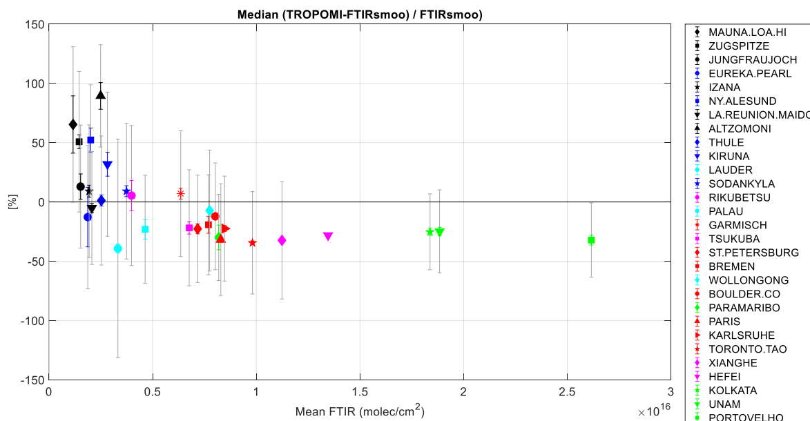
Figure 54: Percent bias between S5P L2_HCHO and NDACC FTIR HCHO column data at each station as a function of the mean FTIR total column ( 10^{16} molec/cm 2 ). The grey bars are the systematic uncertainty on the difference, and the coloured error bars are the 2- \sigma errors on the bias. The temporal range is May 2018 to January 2026 (updated from Vigouroux et al. (2020), Fig. 3).
