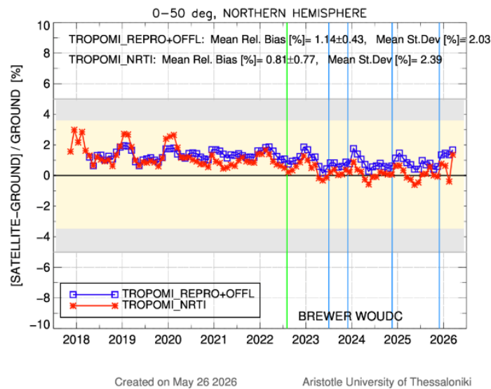
Figure 6: Time series of the monthly mean difference for the comparisons against Brewers in the Northern hemisphere for both the RPRO+OFFL product (blue) and the NRTI product (red). The colored vertical lines denote processor changes (to 2.4.1, to 2.5.0, to 2.6.1, to 2.7.0, and to 2.8.0, respectively).
