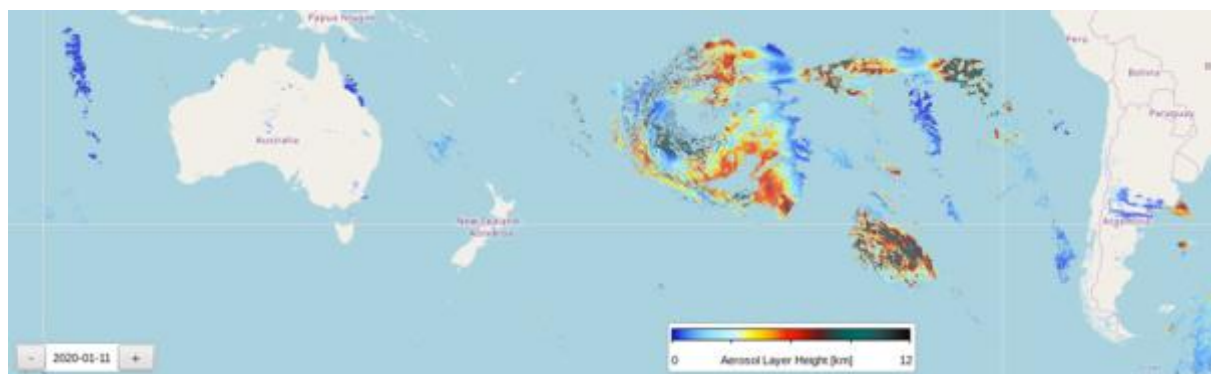
Figure 124: TROPOMI AER_LH product (processor version before v02.05.00) on 11 January 2020 over the south Pacific, showing the altitude as derived by the S5P AER_LH algorithm of the fires smoke from Australian bush fires.
