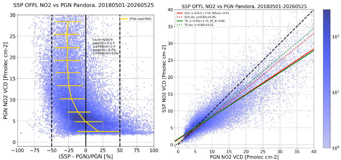
Figure 47 (Left) 2D-histogram of S5P vs PGN relative difference. The yellow line with error bar represents the median with [P16, P84] dispersion, per PGN NO 2 VCD bin. (Right) correlation density plot of S5P vs PGN, with ordinary and robust Theil-Sen linear regression, y vs x and x vs y. RPears: Pearson correlation. KT-N: Normed Kendall-tau correlation.
