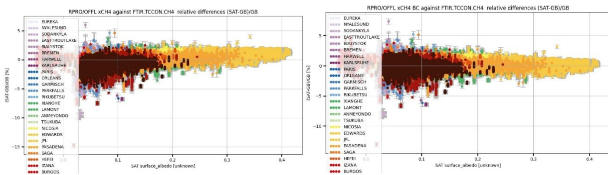
Figure 91: Dependence of the S5P-TCCON relative difference on surface albedo. The left column shows the standard S5P product and the right column the bias corrected S5P product. The bias correction removes the surface albedo dependence of the standard S5P product.
