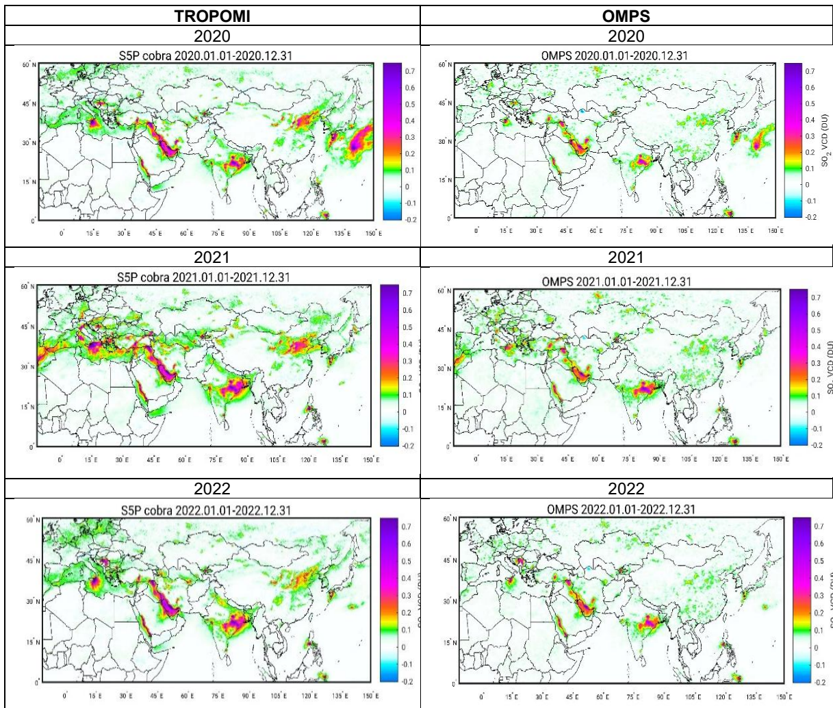
Figure 71: Comparison of TROPOMI (left) and OMPS (right) average SO 2 vertical columns for different years for a region covering Europe, the Middle East, India and China. The slight differences in the absolute values are caused by different profile assumptions in the AMF calculations. Courtesy Nicols Theys (BIRA-IASB).
