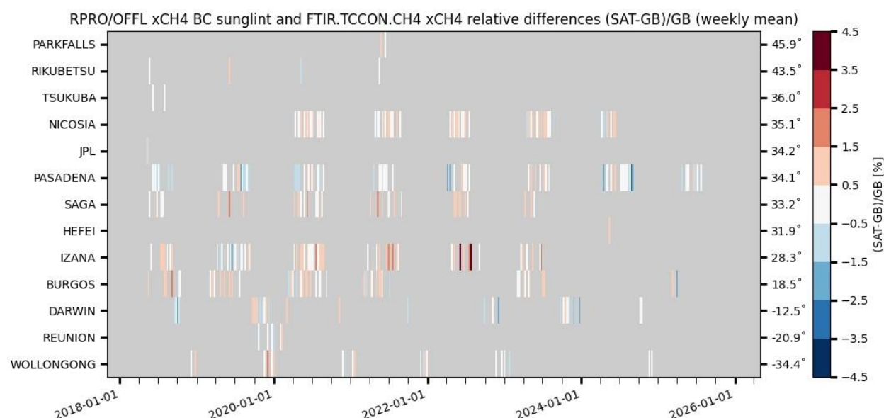
Figure 95: Mosaic plots of relative biases between S5P scientific L2_CH 4 product and ground-based CH 4 TCCON column data for the bias corrected methane products.
