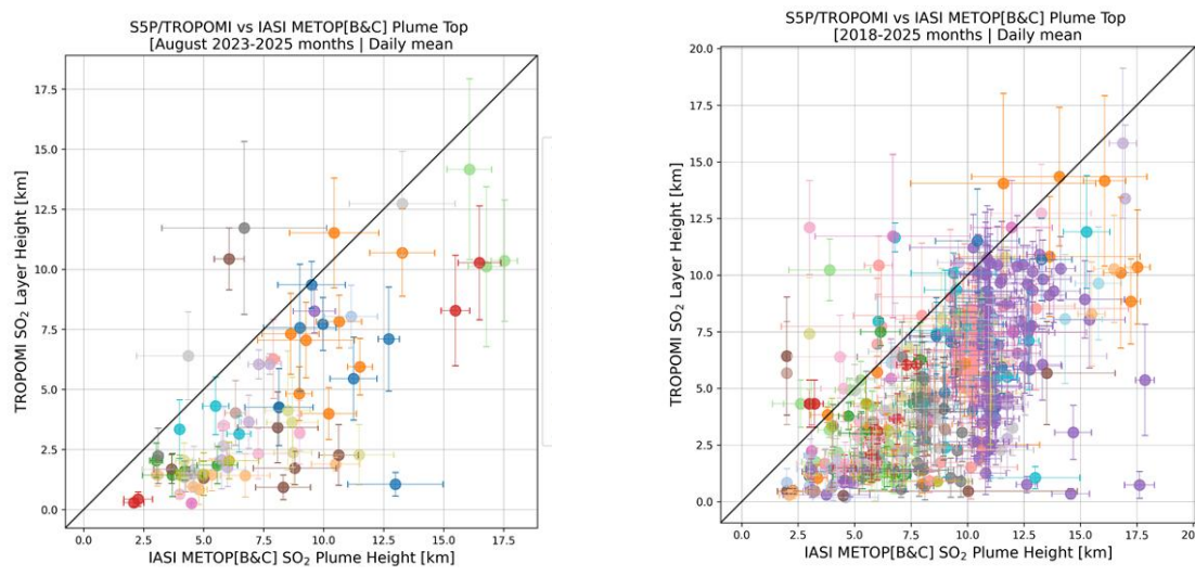
Figure 80: Scatter plot between the daily mean TROPOMI SO 2 layer height observations (y-axis) and combined IASI/Metop-[B&C] observations (x-axis) retrieved during volcanic eruptions for the period August 2023- December 2025 (left), color-coded by the volcano. Same scatter plot on the right for the whole data set including the RPRO data from August 2018 to December 2025.
