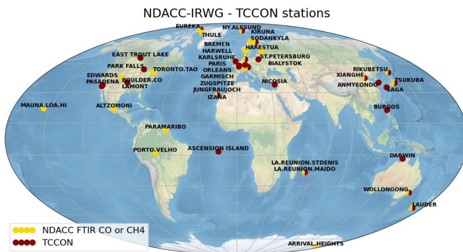
Figure 81: Geographical distribution of NDACC and TCCON FTIR stations measuring atmospheric carbon monoxide column data. Some stations contribute to the two networks.
