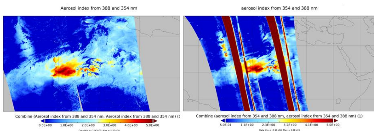
Figure 106: Comparison of S5P TROPOMI RPRO UVAI (orbits 24007 & 24008, left) and OMI OMAERO UV Aerosol Index (orbits 95097 & 95098, right) for Saharan dust on 1 June 2022. In general very good agreement is found (the stripes in north-south direction in the OMI data are caused by the OMI row anomaly and should be ignored).
