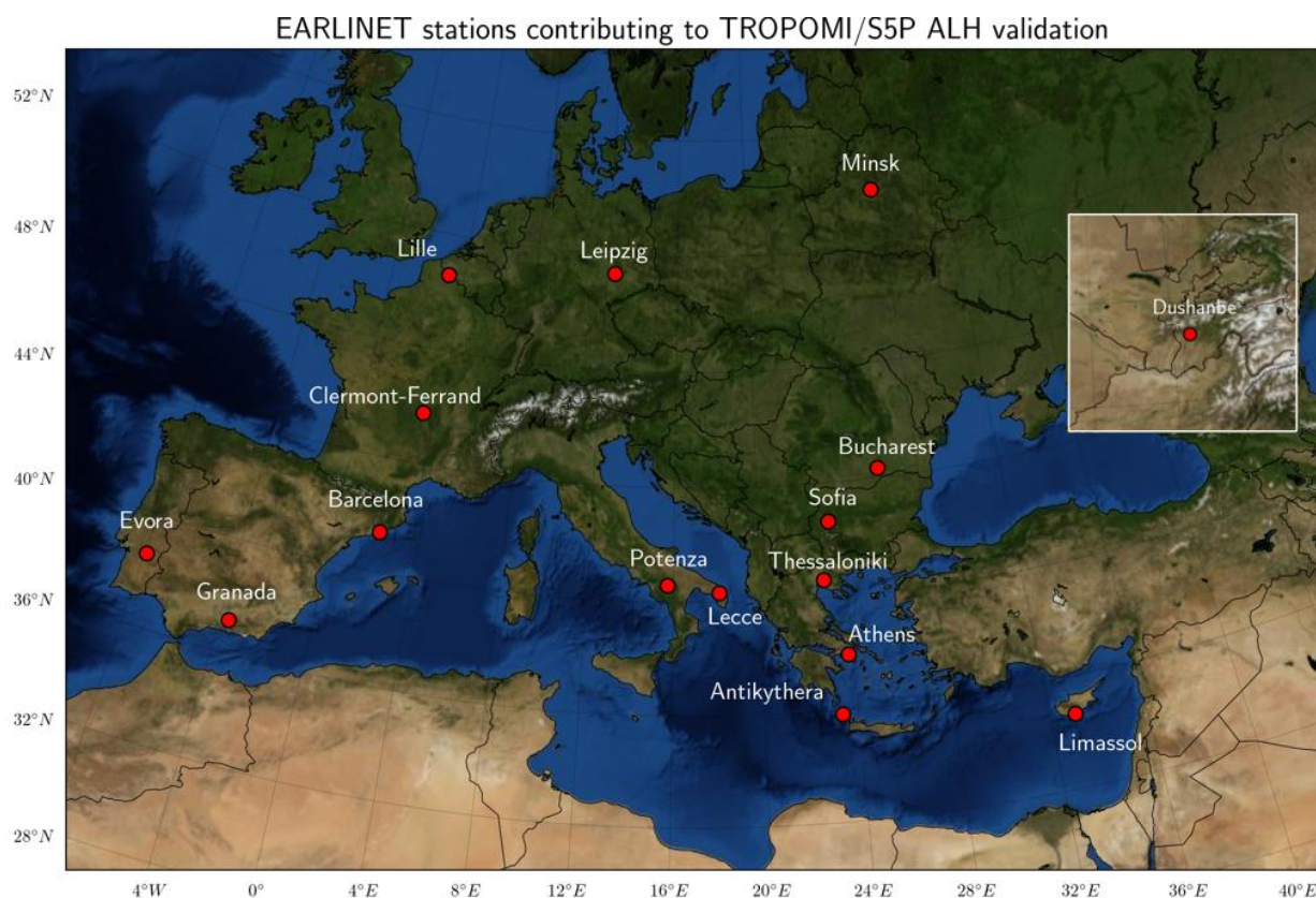
Figure 123: Geographical distribution of EARLINET ground-based stations for which co-locations with S5P L2 AER_LH data were used (period May 2018 – February 2026).
