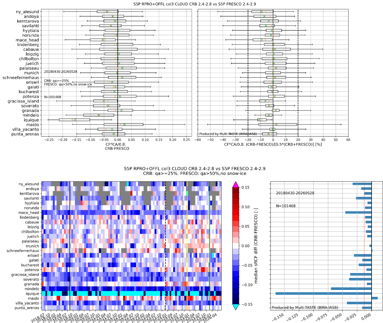
Figure 97. Top left. Box plots of S5P CLOUD CRB OFFL cloud fraction minus S5P FRESCO OFFL cloud fraction, after both have been rescaled to a cloud albedo of 0.8. Left: same but for the normed relative difference. The 20% bias requirement is indicated in dashed lines. Bottom left: monthly median of scaled cloud fraction difference, per month and per station. Indicated are the pixel size switch (2019/08/06), and the following updates: CLOUD v2.6.1 & FRESCO v2.6.0 (2023/11/26), FRESCO v2.7.1 (2024/09/11) CLOUD v2.7.0 & FRESCO v2.8.0 (2024/11/16), and CLOUD v2.8.0 & FRESCO 2.9.1 (2025/11/22). Bottom right: Median of scaled cloud fraction differences per station. The red dashed line gives the median of these median differences.
