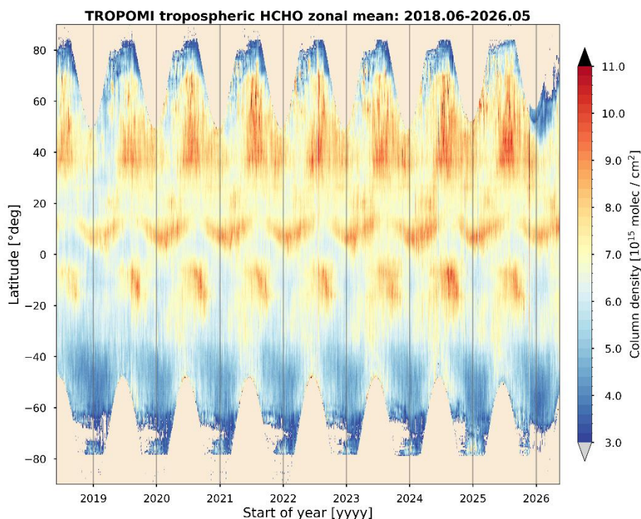
Figure 66: TROPOMI HCHO column data [ 10^{15} molec/ \text{cm}^2 ] as a function of day and latitude. The period is June 2018 to May 2026 (V02.08.00). Grid box size in latitude direction is 0.5^\circ . The grey vertical lines mark the processor version changes, the black lines the beginning of each year.
