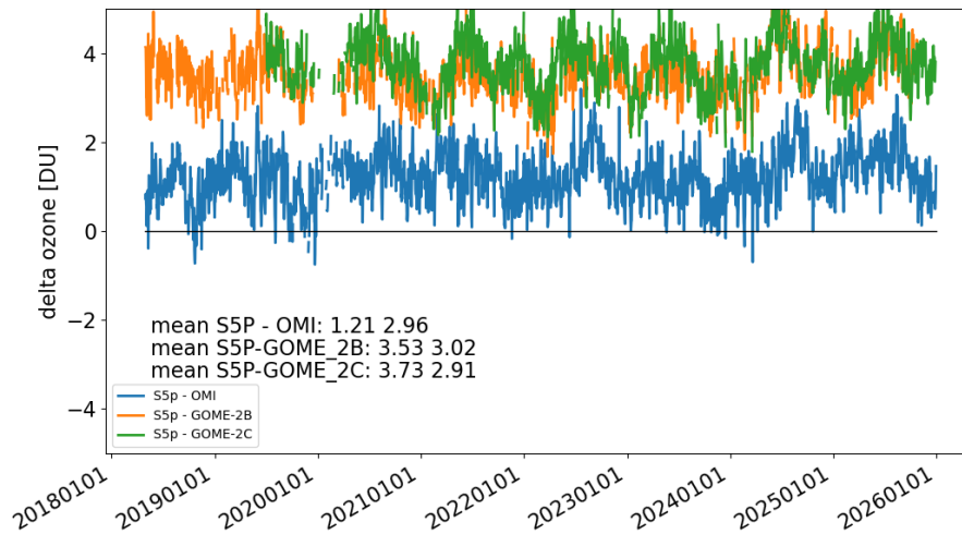
Figure 24: Difference time series of daily tropospheric O 3 column data averaged over the 20°S – 20°N tropical belt. S5P RPRO+OFFL CCD data are compared to OMI (blue), GOME-2B (orange), and GOME-2C (green) satellite data; positive values indicate a high bias of S5P w.r.t. the reference.
