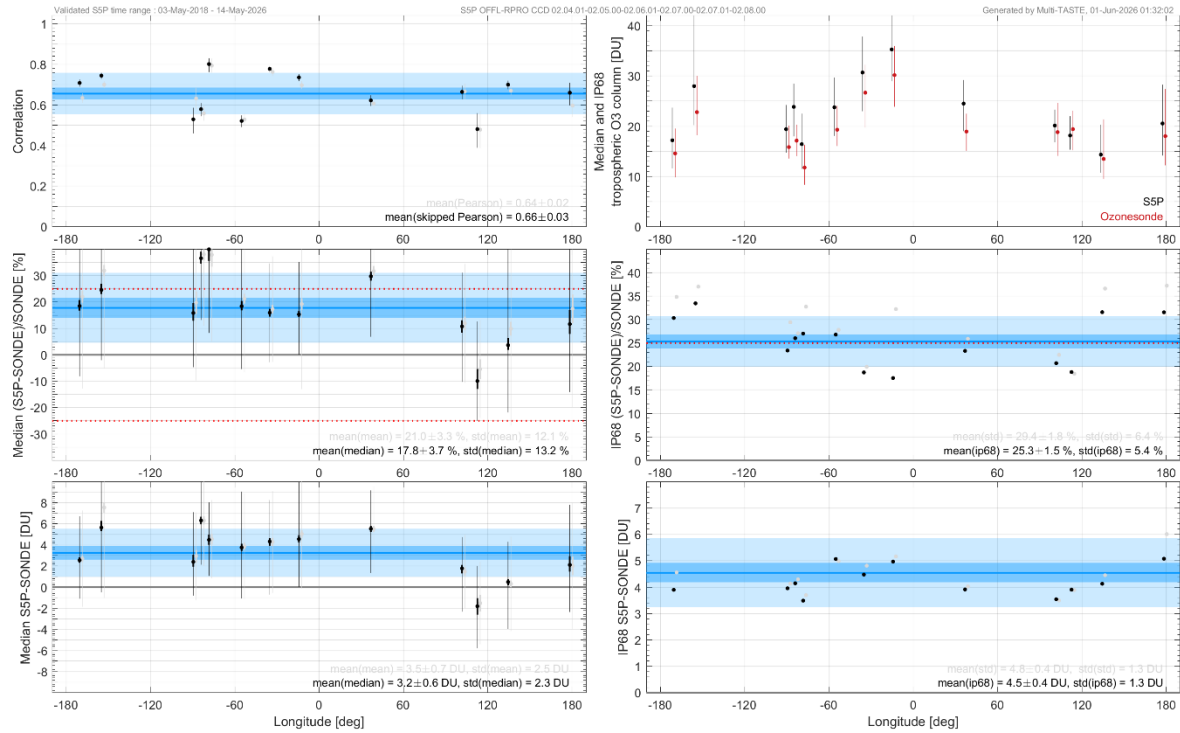
Figure 25: Overview of correlation (top left), median bias (middle & bottom left) and dispersion of the difference (middle & bottom right) of S5P tropospheric O 3 column data for each SHADOZ station (black markers). Black vertical bars represent the 68 % interpercentile of the difference. The mean, standard error of the mean (1σ) and standard deviation (1σ) of the quality indicator across the network are shown as a horizontal blue line and shaded areas.
