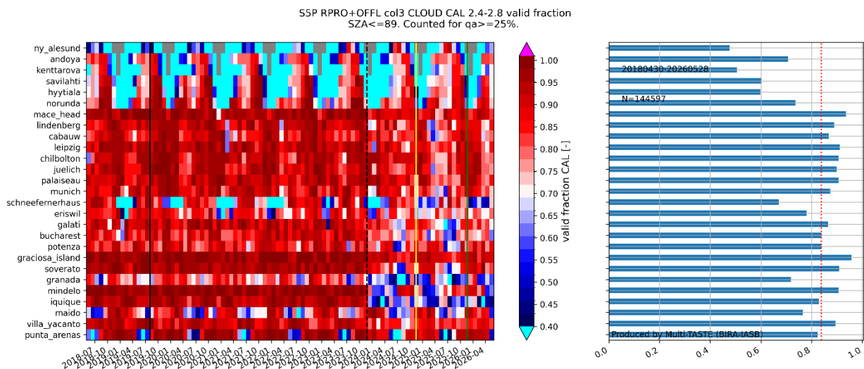
Figure 96: Fraction of valid pixels ( qa\_value \geq 25\% ) for S5P CLOUD CAL. Indicated are the pixel size switch (2019/08/06), the update to CLOUD v2.6.1 (2023/11/26), v2.7.0 (2024/11/16), and v2.8.0 (2025/11/22). Note the colour bar centred at 0.7 and with lower cut-off at 0.4.
