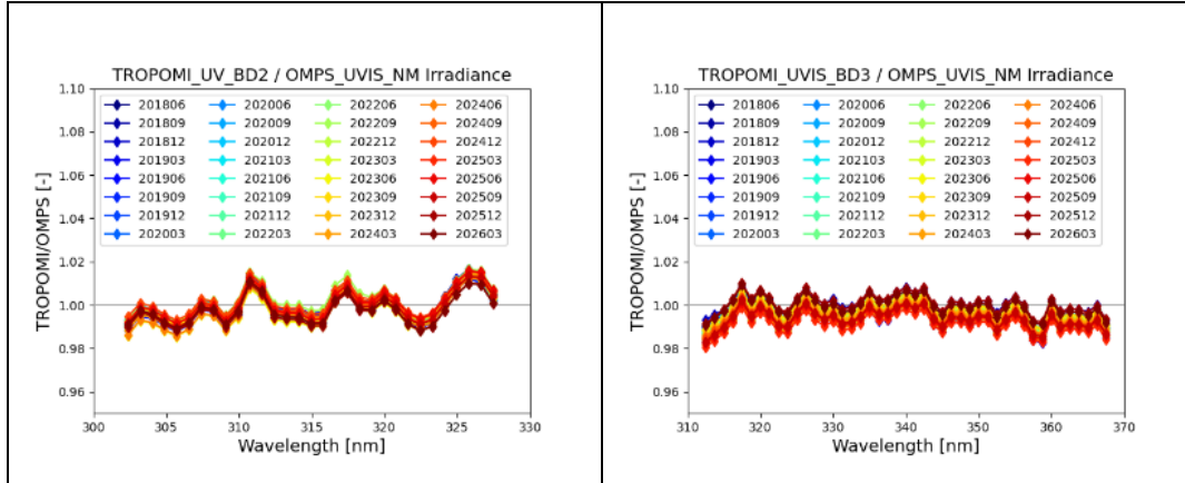
Figure 2: Ratio between TROPOMI L1B_UVN version 02.01.00/03.00.00 irradiance and OMPS irradiance as a function of wavelength for two spectral intervals. Left: 300-330nm, TROPOMI band 2 vs. OMPS-NM. Right: 310-370nm, TROPOMI band 3 vs. OMPS-NM.
