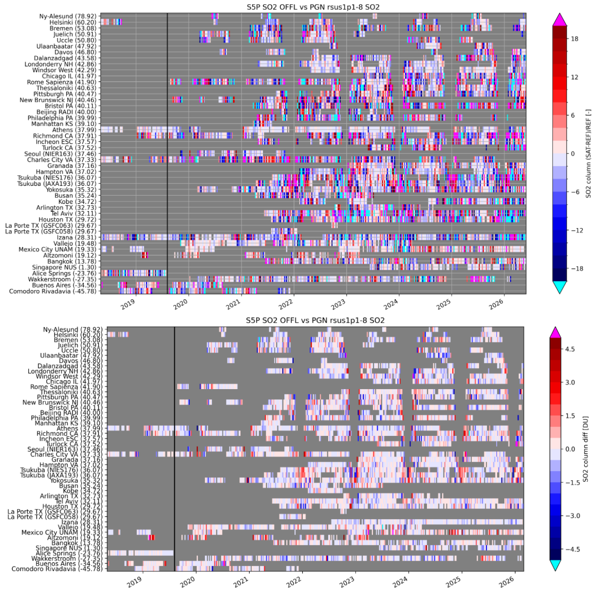
Figure 72: Weekly mean differences between TROPOMI SO 2 VCDs (RPRO+OFFL) ground-based measurements from several Pandora stations. Note that for most stations the SO 2 VCDs are below the detection limit for the satellite and ground-based observations. Courtesy Steven Compennolle (BIRA- IASB).
