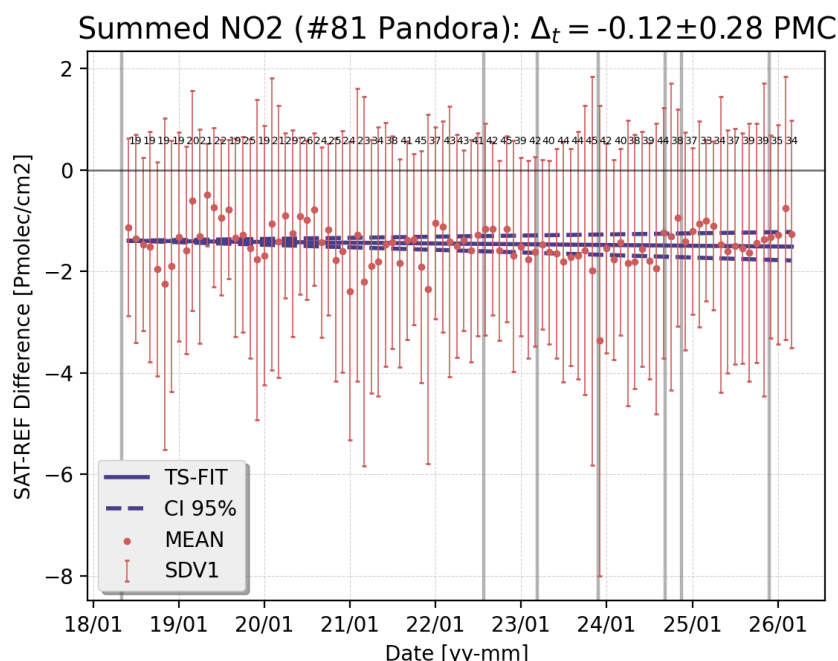
Figure 49: Time series – from May 2018 until April 2026 – of S5P RPRO/OFFL and PGN Pandora NO 2 total column differences that are monthly averaged over all stations available [Pmolec/cm 2 ]. The number of stations is superimposed. Blue lines show the Theil-Sen regression slope and 95% confidence interval. Vertical grey lines show the version changes up to version 02.09.01.
