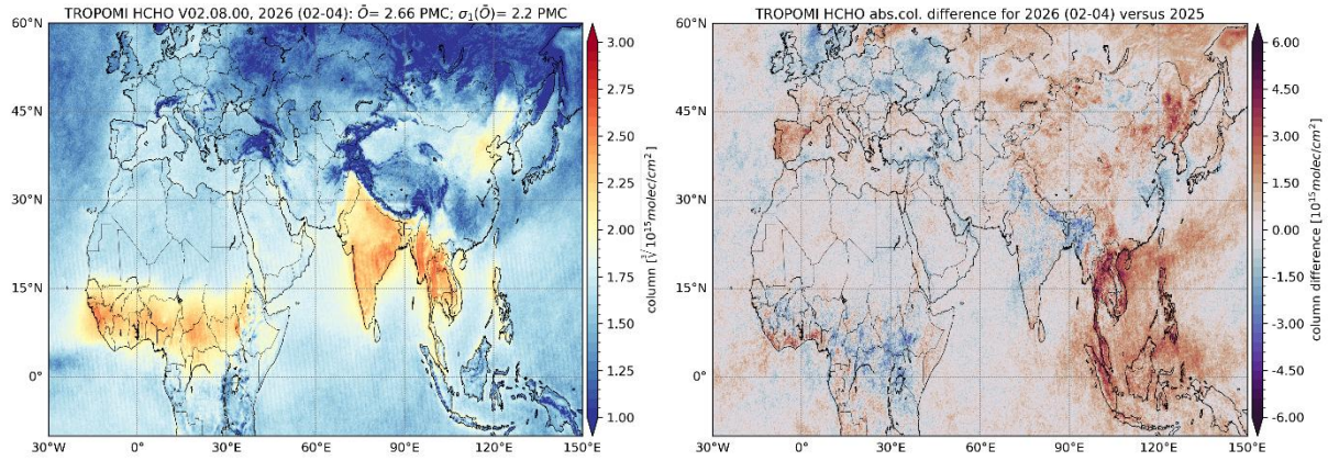
Figure 64: (left) S5P RPRO/OFFL HCHO v02.08.00 [-10°S, 60°N, -30°W, 150°E]. The data is binned on a grid of 0.1° latitude/longitude for February-April 2026. Data with a qa_value > 0.5 and a cloud fraction CF < 0.9 are used. Columns are shown as the third root of values to better cover the HCHO dynamics. (right) The map shows the difference of the left map versus the same period from one year ago (v02.08.00).
