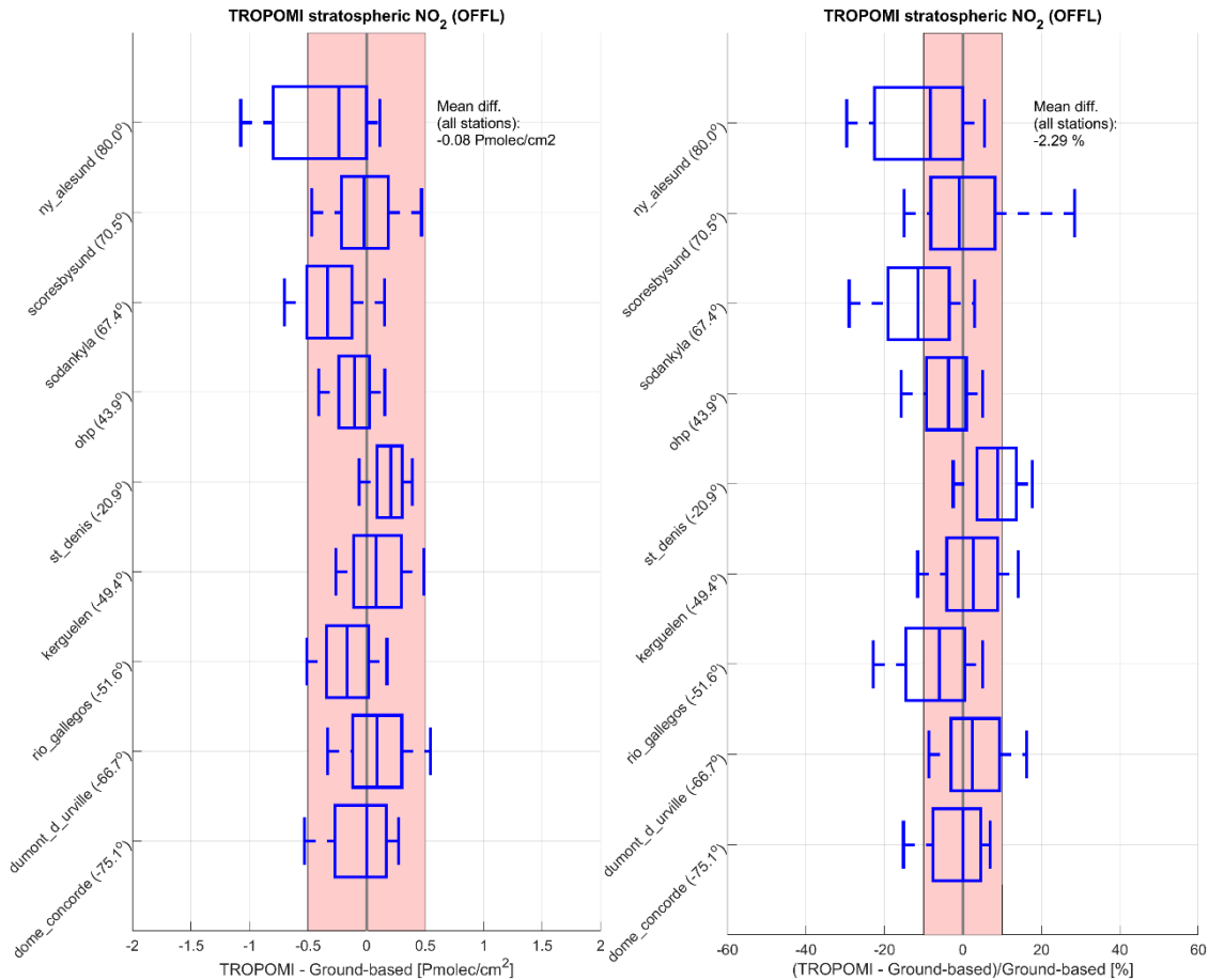
Figure 40: Pole to pole bias and spread (absolute differences in the left-hand panel, relative differences in the right-hand panel) of S5P TROPOMI RPRO+OFFL and NDACC ZSL-DOAS NO 2 stratospheric columns. For the current report, only the SAOZ data sets covering the full mission lifetime are shown. A vertical solid line inside the box, which marks the 25 and 75% quantiles, represents the median difference per station and the whiskers denote the 9-91% range. The red shaded area represents either the mission requirement of 0.5 Pmolec/cm 2 for the random part of the uncertainty (left-hand panel) or that of 10% on the systematic uncertainty (right-hand panel). Station name and latitude of the station are added on the left. The period is May 2018 to May 2026.
