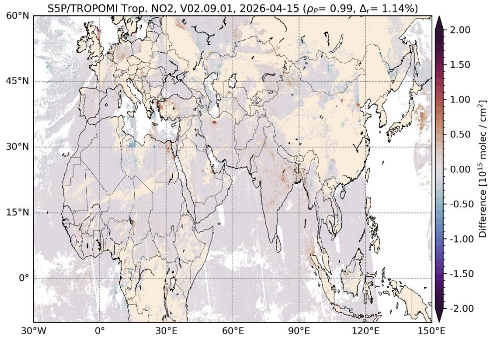
Figure 50: Difference between S5P NRTI and OFFL v2.9.1 tropospheric NO 2 columns on 2026-04-15. The difference is calculated for columns > 0.5 Pmolec/cm 2 , cloud fractions < 0.2 and a qa_value > 0.75. Data was binned on 0.1° x 0.1° grid cells.
