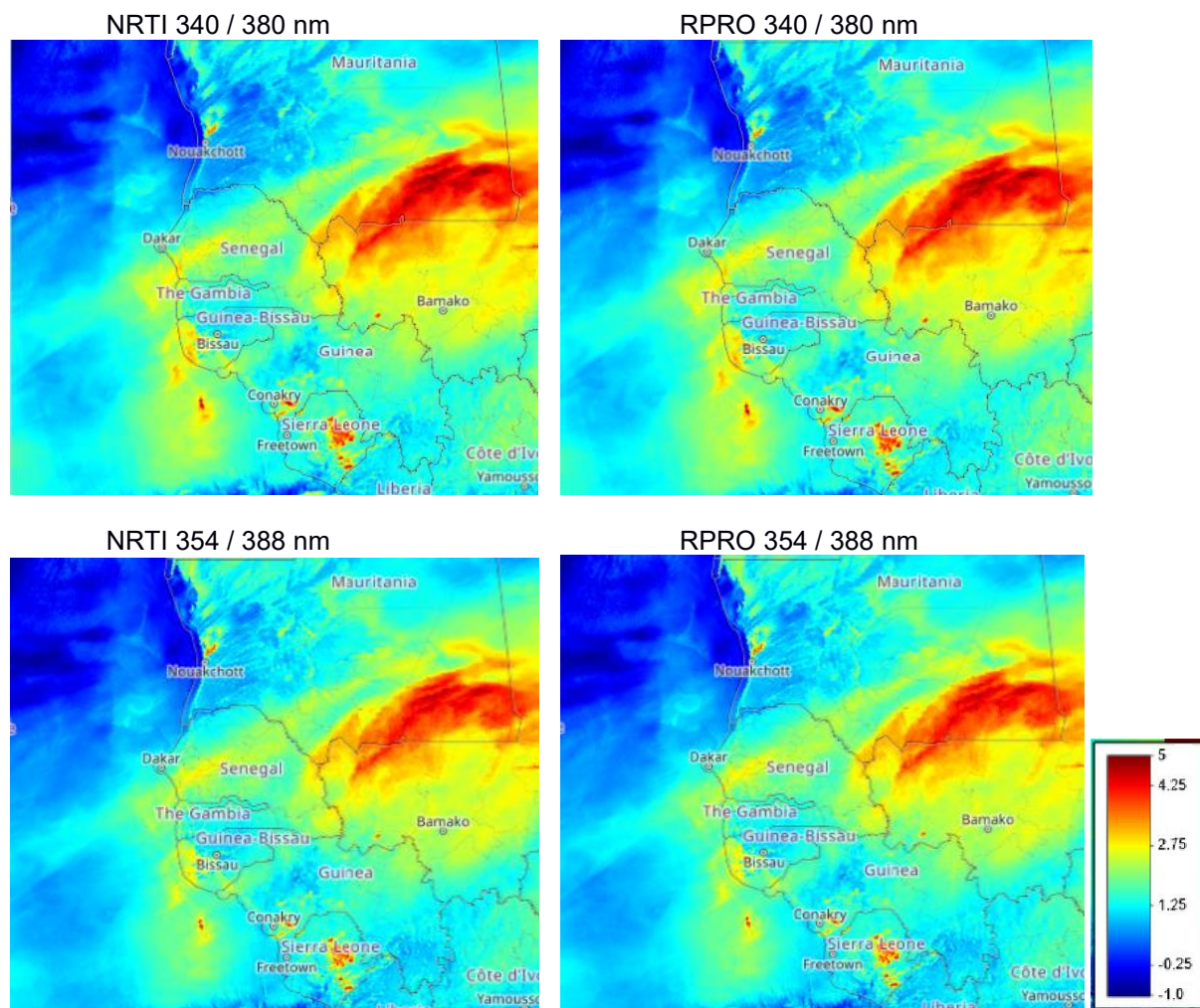
Figure 112: Comparison of the S5P TROPOMI near real time and reprocessed UVAI for a selected area on October 4, 2022, for the two wavelength pairs (top: 340 / 380 nm, bottom: 354 / 388 nm).
