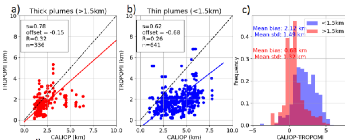
Figure 122: Comparison of TROPOMI ALH (processor version before v02.05.00) and CALIOP average aerosol layer height (top minus bottom of aerosol layer as defined by the feature mask) for collocated pixels near fires over Northern America in 2018. See Griffin et al, 2019, for details.
