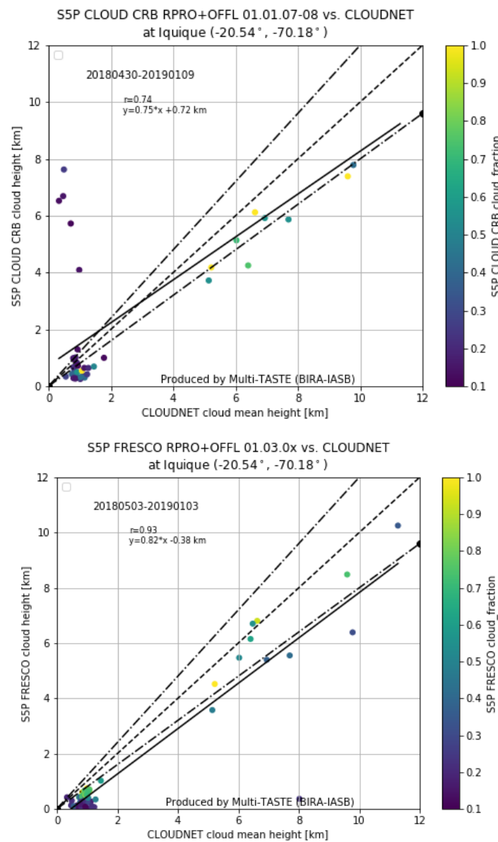
Figure 96. Top. S5p CLOUD CRB CH vs CLOUDNET CH correlation plot. Bottom. S5p FRESCO CH vs CLOUDNET CH correlation plot.
