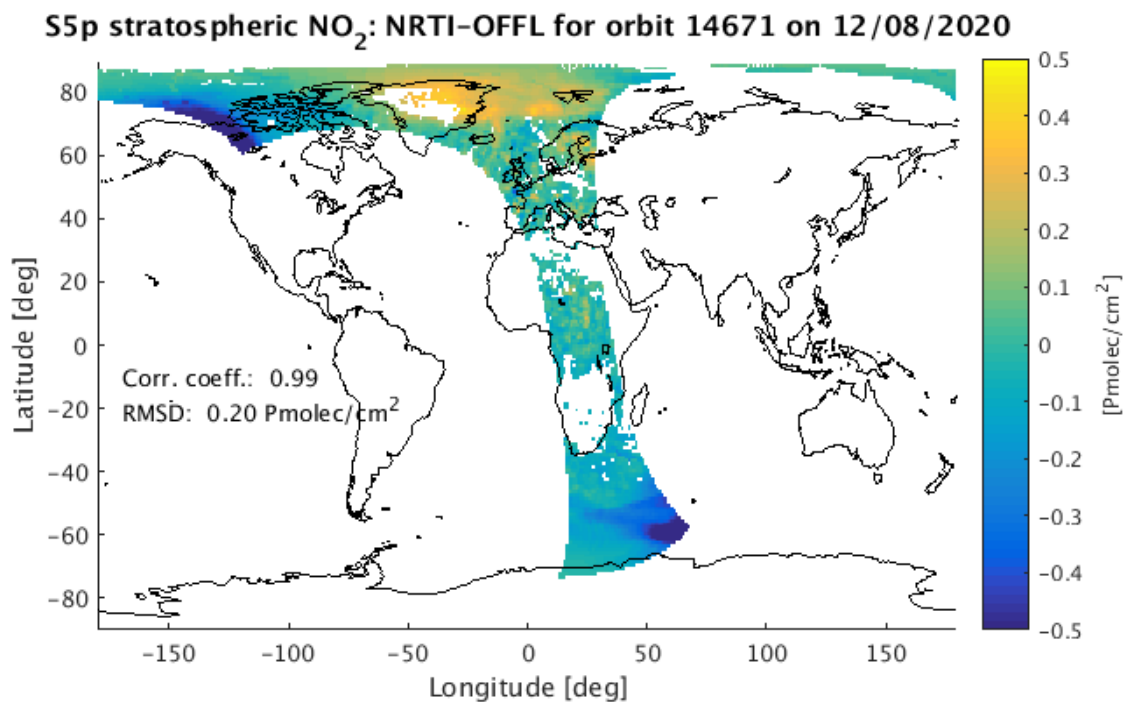
Figure 41: Difference between S5P NRTI and OFFL stratospheric NO 2 column data for a single orbit (gridded to 1°x1° resolution).
