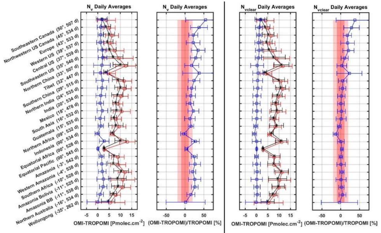
Figure 49: Absolute and relative bias between OMI and TROPOMI HCHO daily averaged columns using cloud corrected AMF (left) or clear-sky AMF (right) for a selection of regions. Regions are displayed by decreasing latitude. The mean OMI (red) and TROPOMI (black) columns are plotted together with the absolute bias.
