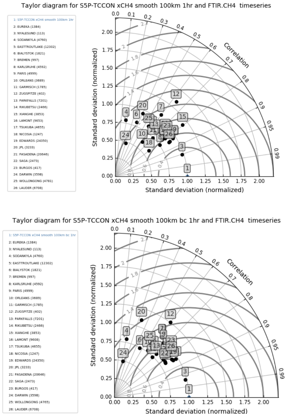
Figure 80: Taylor diagrams for differences between S5P L2_CH4 RPRO/OFFL and TCCON methane column data: standard (top) and bias corrected (bottom) S5P methane columns. At almost all sites the variability of the S5P column data is higher compared to the variability in the TCCON data.
