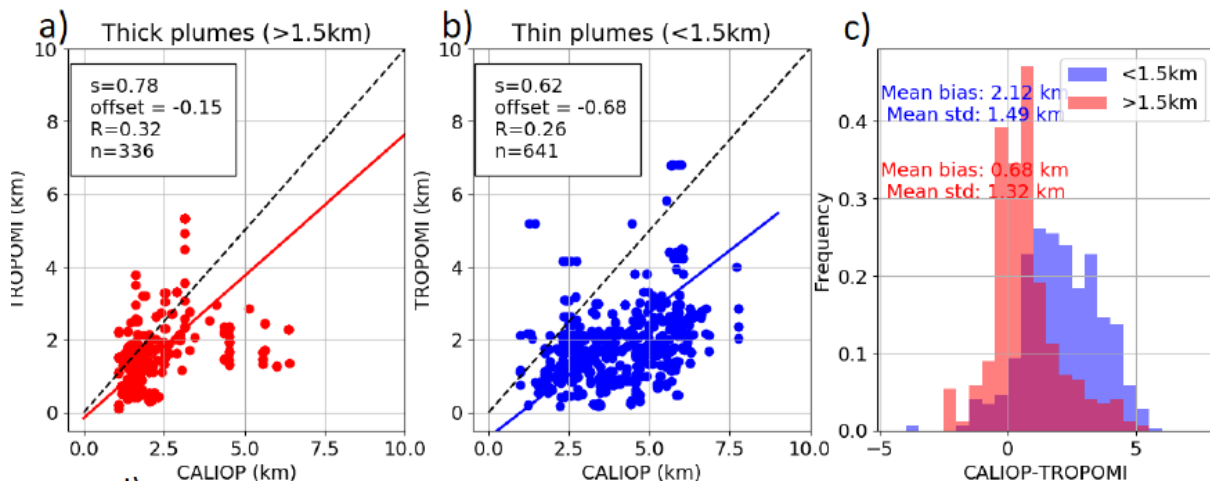
Figure 113: Comparison of TROPOMI ALH and CALIOP average aerosol layer height (top minus bottom of aerosol layer as defined by the feature mask) for collocated pixels near fires over Northern America in 2018. See Griffin et al, 2019, for details.
