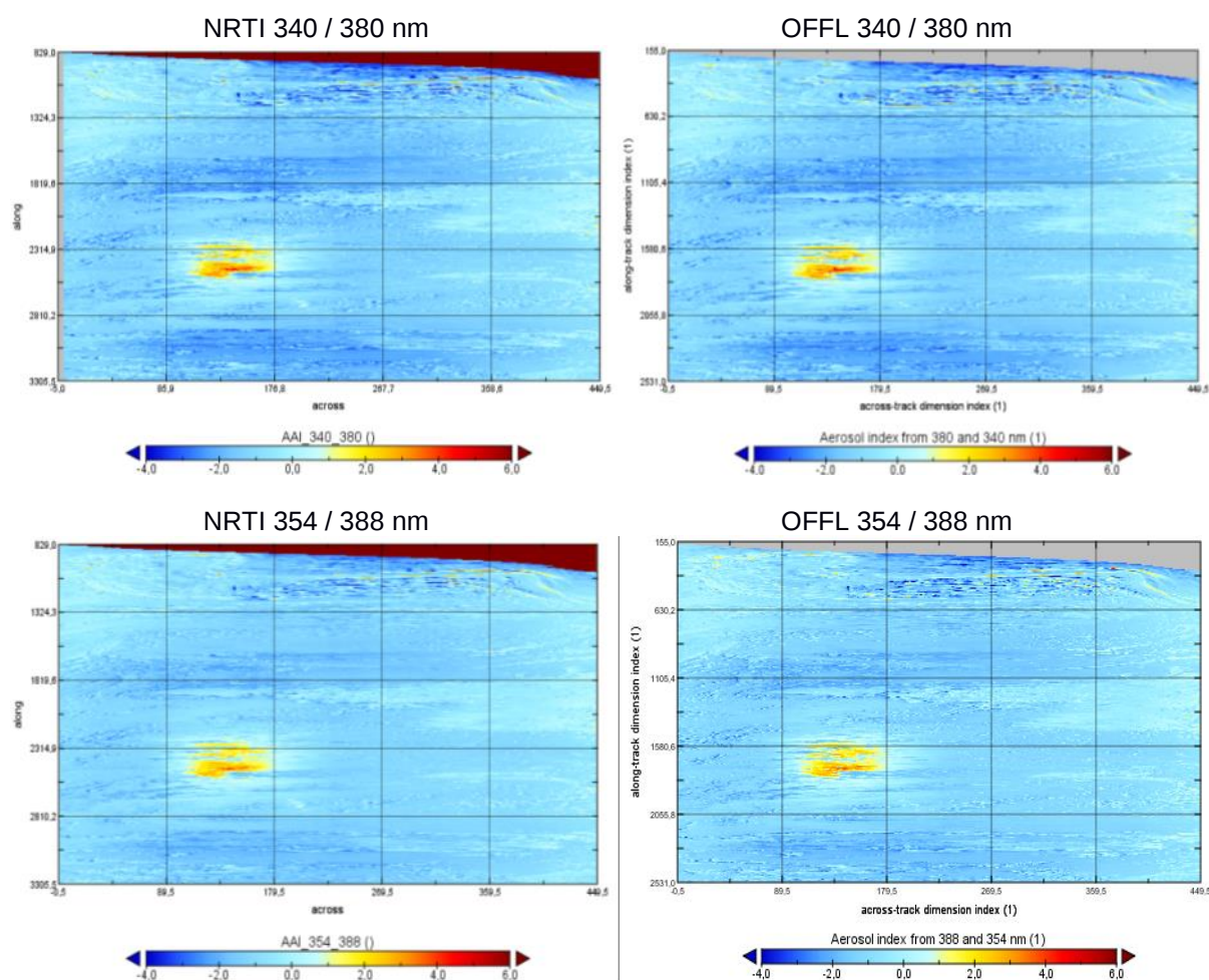
Figure 107: Comparison of the S5P TROPOMI UVAI for a selected orbit (#05033) on 3 October 2018 for the two wavelength pairs (top: 340 / 380 nm, bottom: 354 / 388 nm). While the geographical patterns are the same, the absolute values differ slightly with the NRT values (left) slightly higher than the offline values (right).
