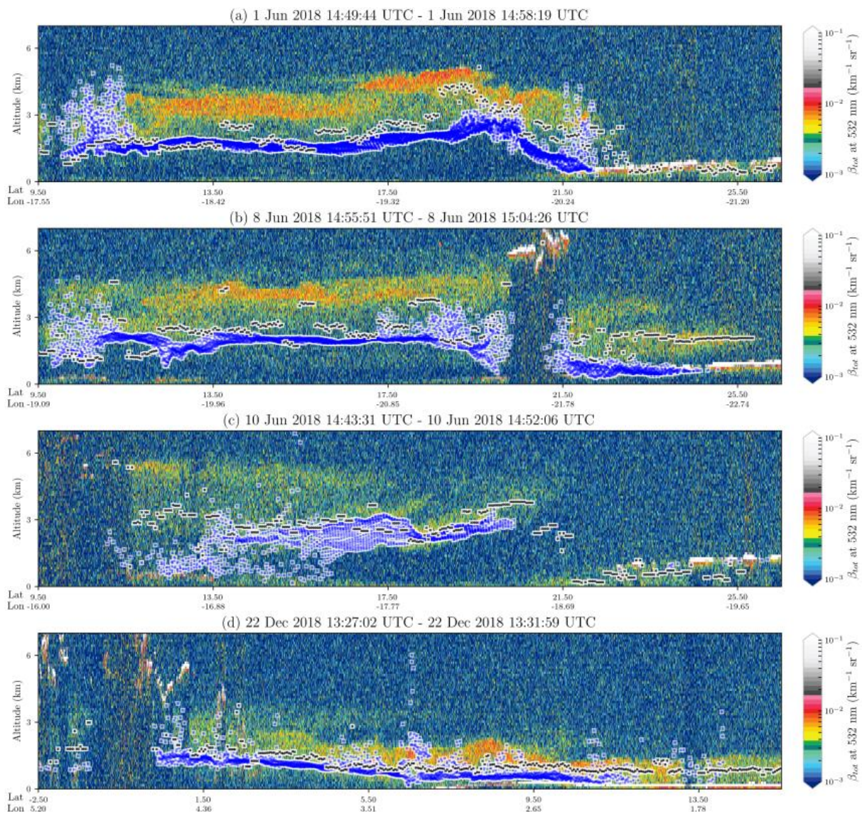
Figure 109: Curtain plots from CALIOP, showing the total attenuated backscatter at 532 nm for the four cases in Figure 108 . Overplotted on the coloured background image of the total attenuated backscatter are the weighted extinction heights as derived from the backscatter coefficient in black-and-white, and the ALH from collocated TROPOMI pixels in blue-and-white.
