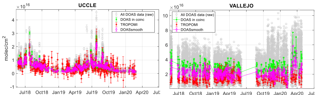
Figure 51: TROPOMI and DOAS time series at Uccle and Vallejo.
