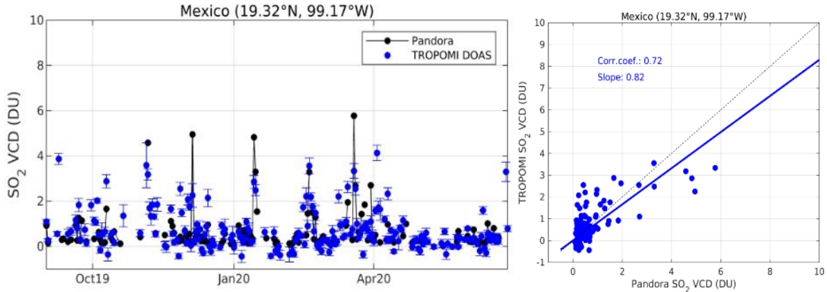
Figure 62: Comparison of TROPOMI SO 2 VCDs to preliminary Pandora measurements (daily means) at Mexico City from September 2019 to August 2020. The following selection criteria were applied: distance < 25km, CF<0.2, time window +/- 1h around overpass. Courtesy of N. Theys (BIRA-IASB), Martin Tiefengraber and Alexander Cede (Luftblick). Pandora data are still in demonstration phase.
