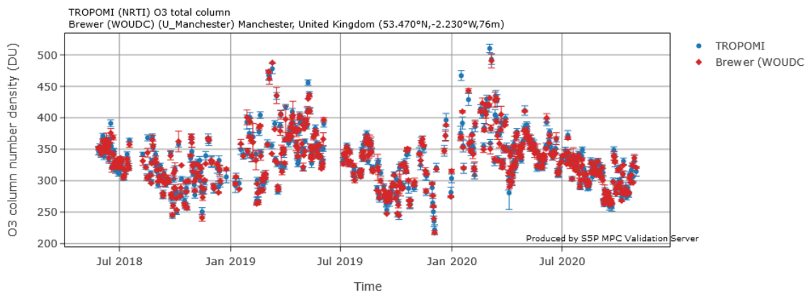
Figure 7: Time series of S5P TROPOMI NRTI and Brewer total ozone data at the station of Manchester in the United Kingdom (data courtesy J. Rimmer, University of Manchester).
