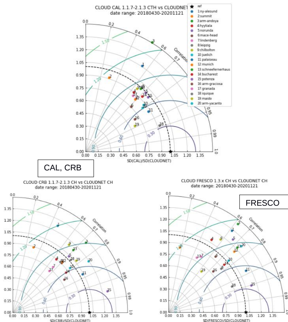
Figure 94: Taylor diagrams of CLOUD CAL vs CLOUDNET CTH, CLOUD CRB vs CLOUDNET CH and FRESCO CH vs CLOUDNET CH. The radius represents SD(S5p)/SD(CLOUDNET) , the angle represents correlation and the circular contour lines represents the relative dispersion SD(S5p-CLOUDNET)/SD(CLOUDNET) .
