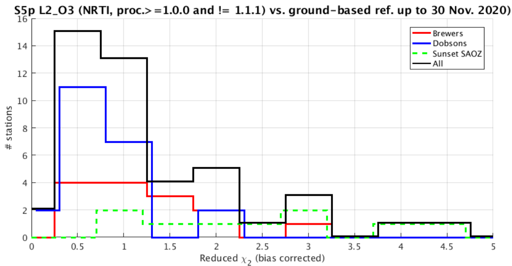
Figure 5: Histogram of the \chi_r^2 values (one per reference instrument) for S5p NRTI total ozone versus different ground-based instruments.
