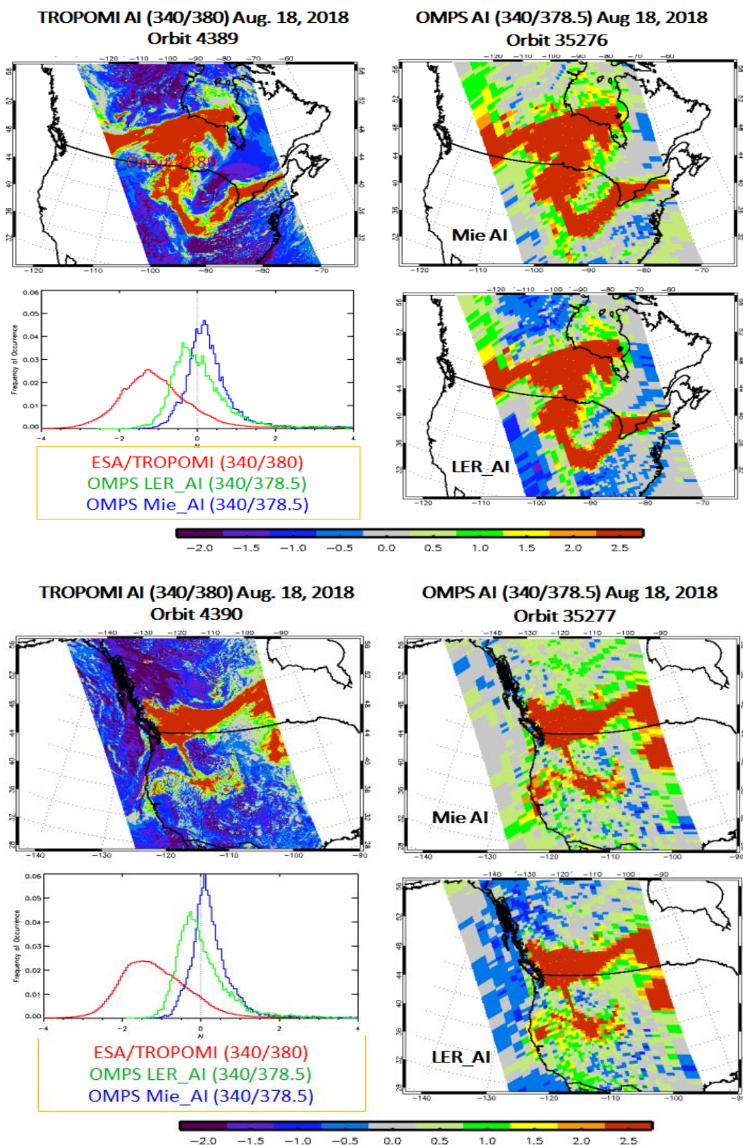
Figure 103: Comparison of UVAI from TROPOMI and OMPs for an observation of a biomass burning plume (18 Aug. 2018). For OMPS UVAI are calculated assuming either LER or Mie clouds. The UVAI for Mie clouds yields more consistent results. In contrast to early TROPOMI observations, values have systematically decreased and the spread of the UVAI values has become larger (courtesy of Omar Torres and Changwoo Ahn, NASA-GSFC).
