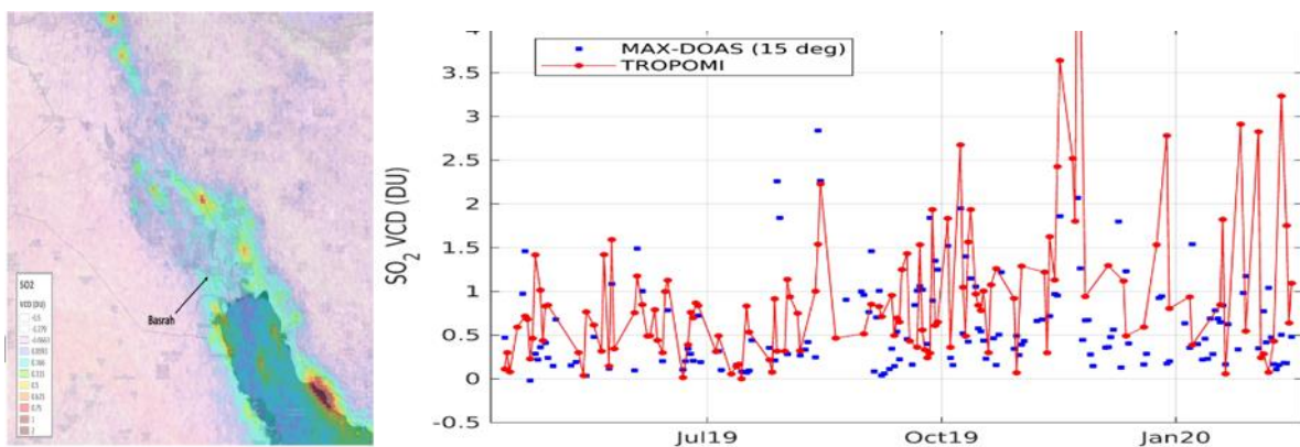
Figure 61: Comparison of TROPOMI SO 2 VCDs to MAX-DOAS measurements (daily means) at Basra (Iraq) from April 2019 to March 2020. The following selection criteria were applied: distance < 25km, CF<0.2, AMF>0.2, time window +/- 1h around overpass. Courtesy of N. Theys (BIRA-IASB), data provided by Nayyef Almaliki, Mustafa Aldossary, Ali Almasoudii, Sebastian Donner, Steffen Dörner, Thomas Wagner.
