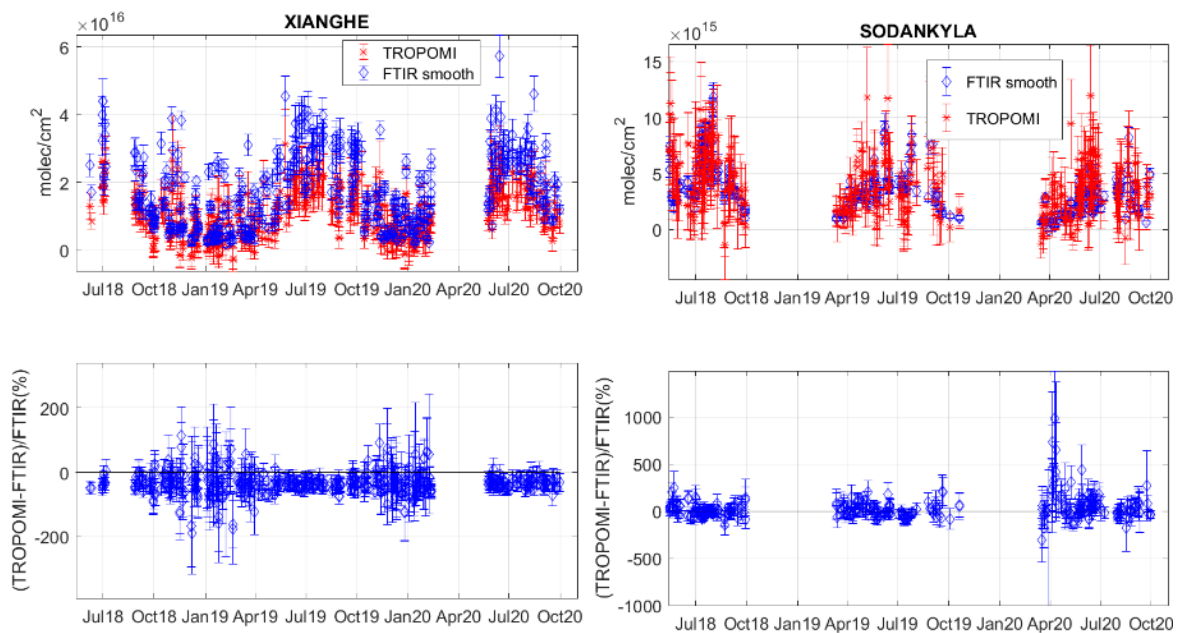
Figure 55: Time series of the HCHO columns [Pmolec/cm 2 ] and difference [%] between S5P and smoothed FTIR HCHO for the stations Xianghe and Sodankyla.
