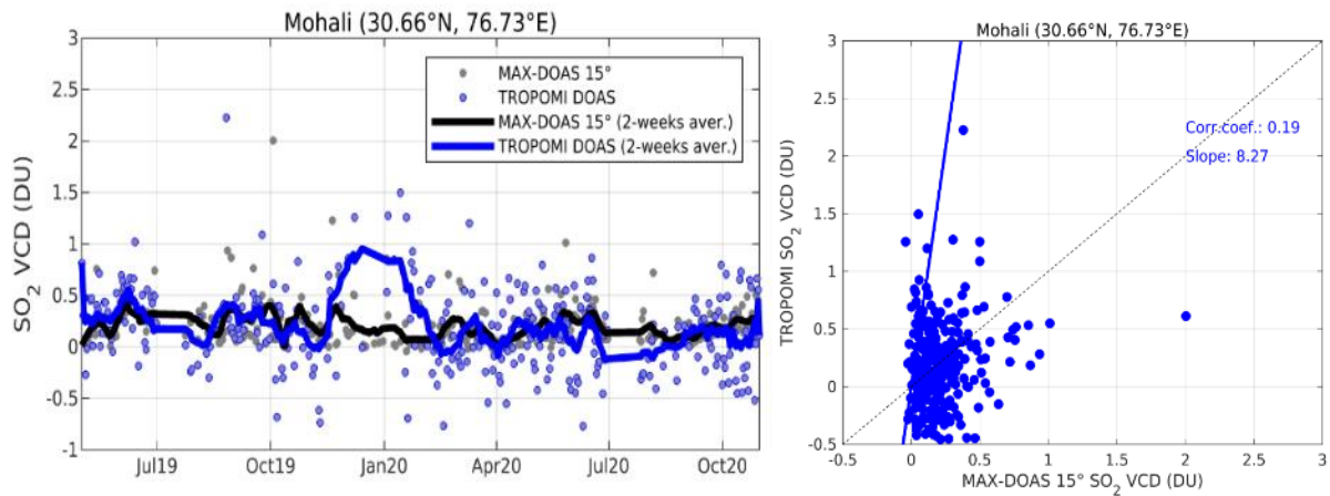
Figure 63: Comparison of TROPOMI SO 2 VCDs to MAX-DOAS measurements (daily means) at Mohali (India) from June 2019 to November 2020. The following selection criteria were applied: distance < 25km, CF<0.2, AMF>0.2, time window +/- 1h around overpass. Courtesy of N. Theys (BIRA-IASB), data provided by, Vinod Kumar, Vinayak Sinha, Sebastian Donner, Steffen Dörner, Thomas Wagner.
