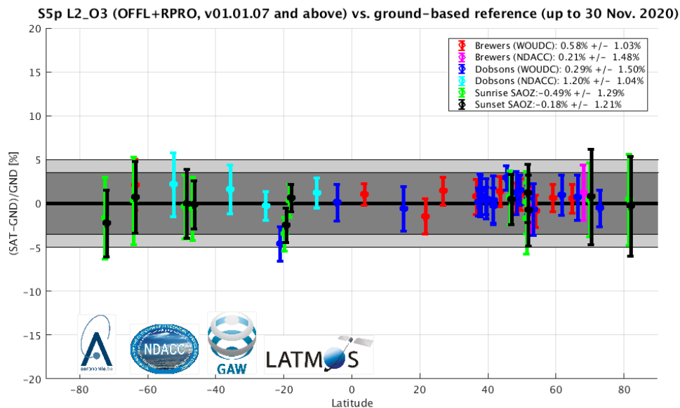
Figure 10: Meridian dependence of the median (the circular markers) and spread ( \pm 1 sigma, the error bars) of the percent relative difference between S5P TROPOMI L2_O3 (PDGS OFFL processors v1.1.7, v1.1.8, and v2.1.3) and ground-based (GND) ozone column data, represented at individual stations from the Antarctic to the Arctic and per measurement type (Brewer, Dobson, and ZSL-DOAS). The values in the legend correspond to the median and spread of all median (per station) differences. For clarity, sunrise and sunset ZSL-DOAS results are represented separately (offset by -0.5° and +0.5° in latitude).
