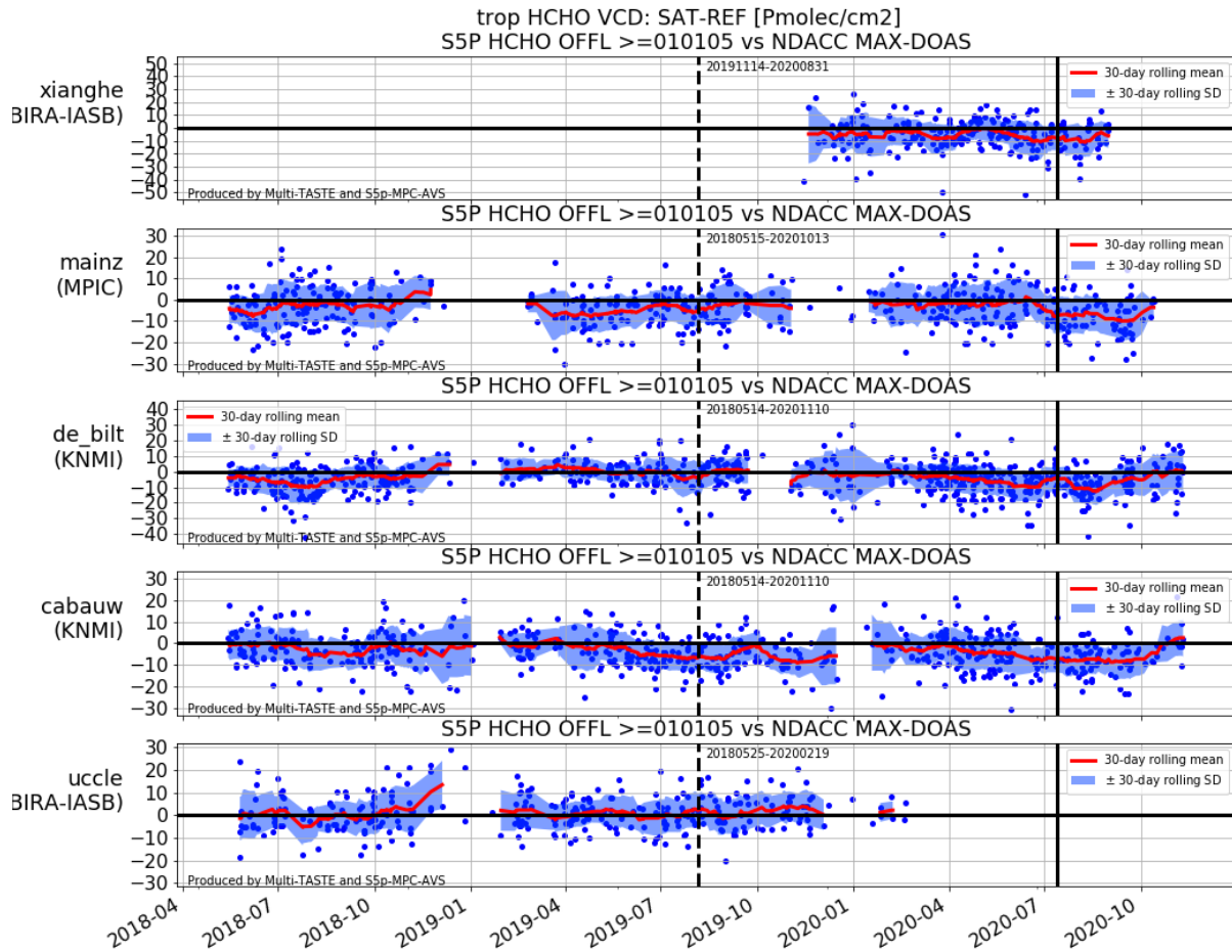
Figure 54: Time series of the difference [Pmolec/cm 2 ] between S5P RPRO+OFFL and MAX-DOAS HCHO column data at five stations. Data was obtained from the VDAF Automated Validation Server on 2020/11/25. Dashed line: pixel size switch at 2019/08/06. Full vertical line: OFFL processor version change on 2020/07/13.
