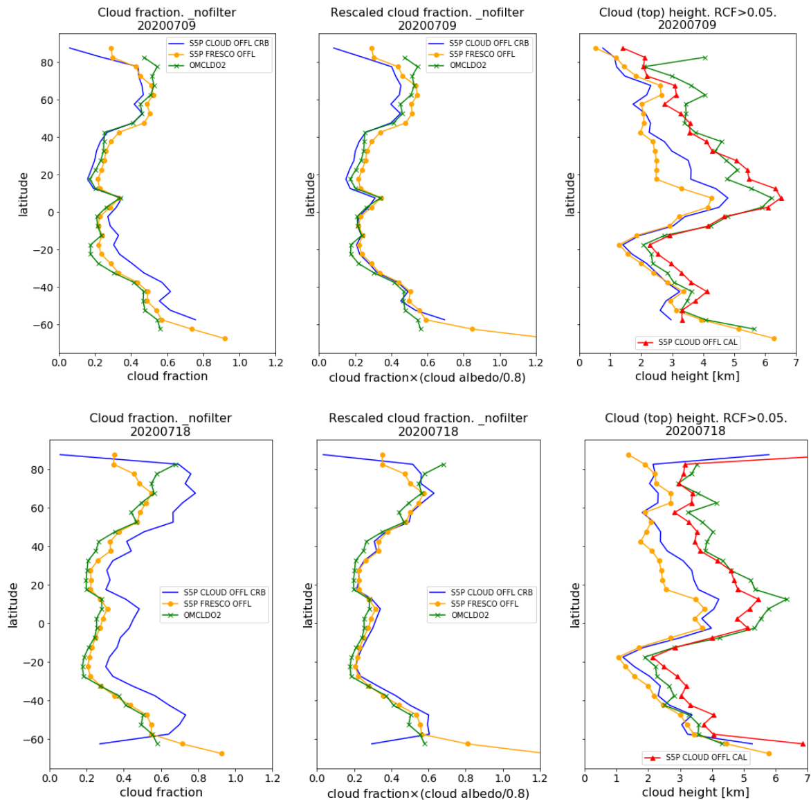
Figure 98: Latitudinal variation of zonal means of cloud fraction (left), scaled cloud fraction (middle) and cloud (top) height (right) of the cloud products S5p OFFL CLOUD (CAL and CRB), S5p OFFL FRESCO and Aura/OMI OMCLDO2. Top: at 2020/07/09 (UPAS version = 1.1.8). Bottom: at 2020/07/18 (UPAS version = 2.1.3).
