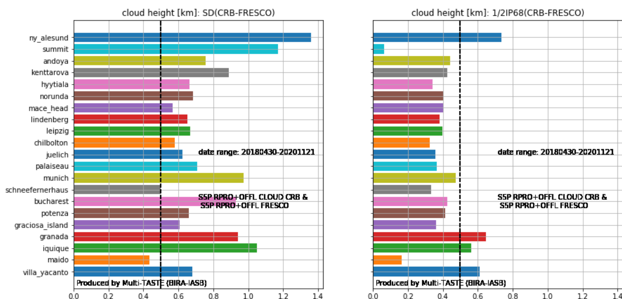
Figure 95: Standard deviation (left) and \frac{1}{2} IP68 (right) of S5p CLOUD CRB CH minus S5p FRESCO CH. Sensing date range is indicated on the figure.
