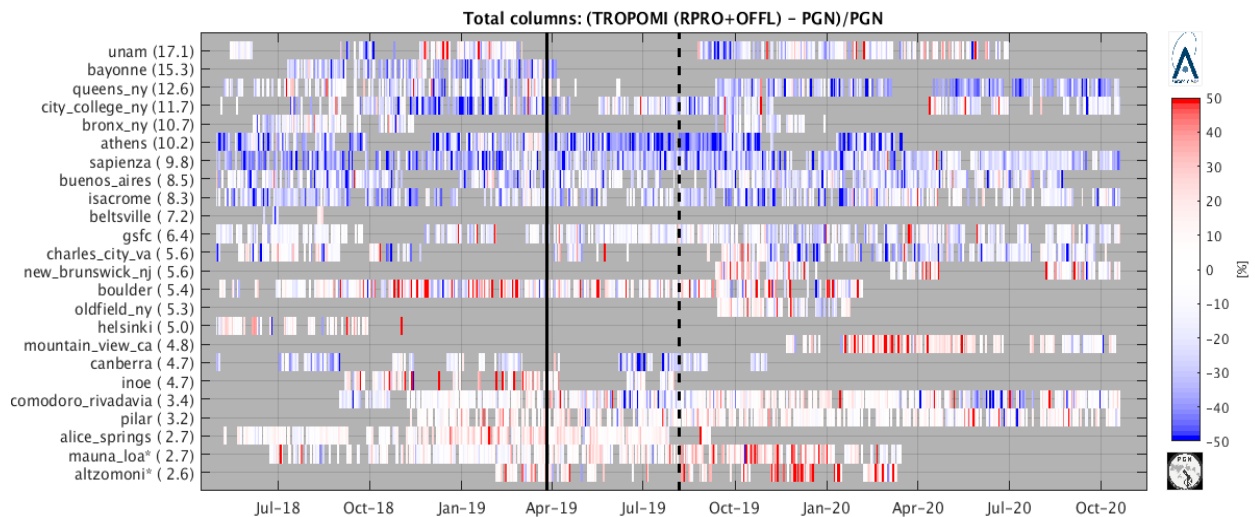
Figure 40: Time series – from May 2018 until October 2020 – of S5P RPRO+OFFL and PGN Pandora NO 2 total column differences [%]. The black solid and dashed lines indicate, respectively, the processor switch from 1.2.2 to 1.3.0 and the activation of the finer horizontal resolution. Stations are ordered by median total column.
