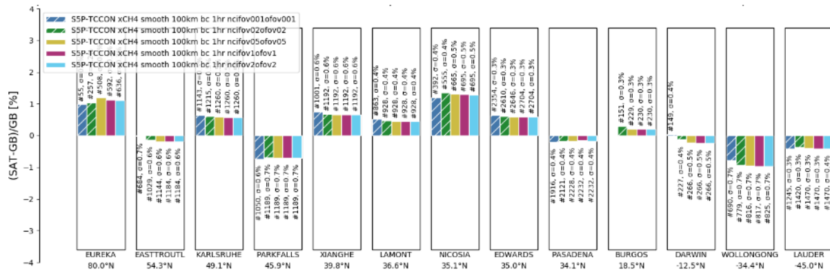
Figure 82: charts of relative mean difference between S5P L2_CH4 and FTIR CH 4 column data at 13 TCCON sites within the time range 11 March 2020 till 19 July 2020. The sites are sorted with decreasing latitude. Top panel plot is for the old CF definition and the bottom panel plot is for the new CF definition. Different colors represent the different CF threshold applied for the filtering.
