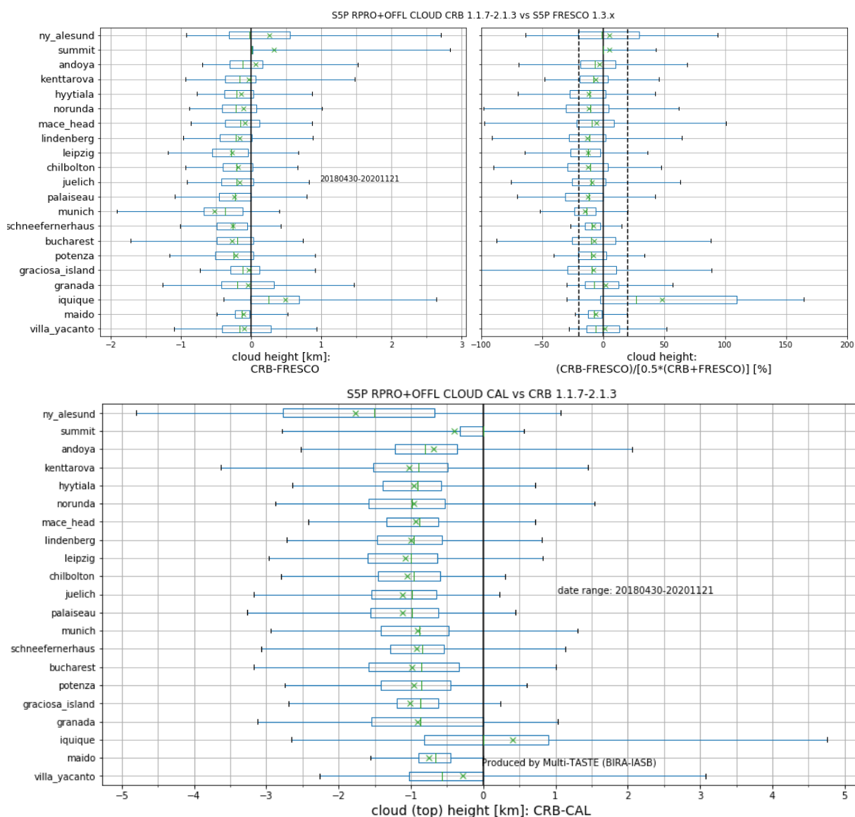
Figure 93: Top. Boxplots of S5p CLOUD CRB CH minus S5p FRESCO CH (left) and of the normed difference (right). Bottom. Boxplots of S5p CLOUD CRB CH minus S5p CLOUD CAL CTH.
