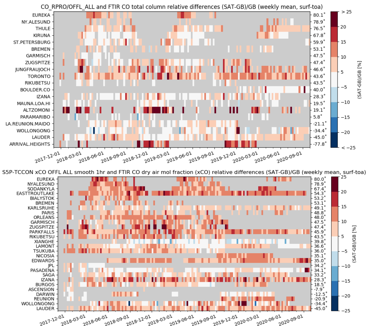
Figure 69: Relative bias between S5P L2_CO OFFL and ground-based CO column data at NDACC (top) and TCCON (bottom) FTIR stations. Over the Nov. 2017 – October 2020 time period the plots do not show a clear meridian dependence or temporal change in the weekly averaged biases.
