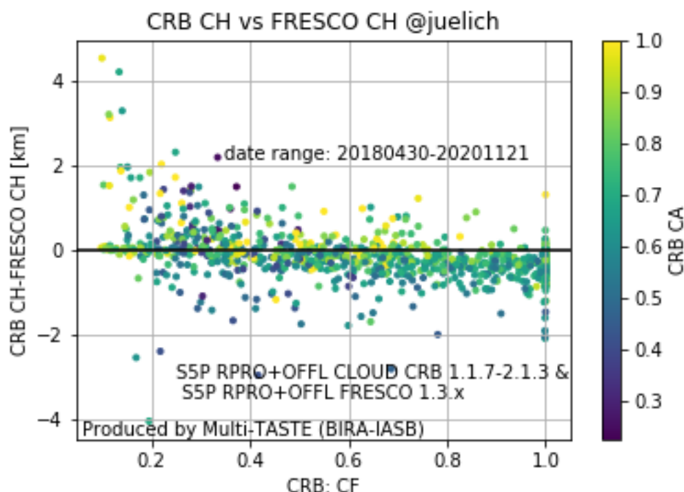
Figure 97: Cloud height difference between S5p CLOUD CRB and S5p FRESCO, in function of CLOUD CRB cloud fraction. Color scale is CLOUD CRB cloud albedo.
