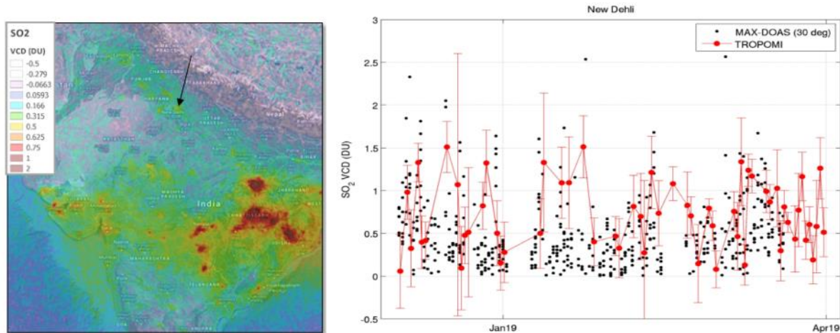
Figure 59: Comparison of TROPOMI SO 2 VCDs to MAX-DOAS measurements at Greater Noida (close to New Delhi, India). The following selection criteria were applied: distance < 15km, CF<0.2, AMF>0.2, MAX-DOAS +/- 1h around S5P overpass. Courtesy of M. Sharma (Sharda University, India) S. Donner, S. Dörner, T. Wagner (MPIC), N. Theys (BIRA-IASB).
