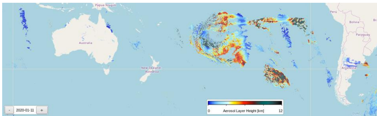
Figure 115: TROPOMI AER_LH product on 11 January 2020 over the south Pacific, showing the altitude as derived by the S5P AER_LH algorithm of the fires smoke from Australian bush fires.
