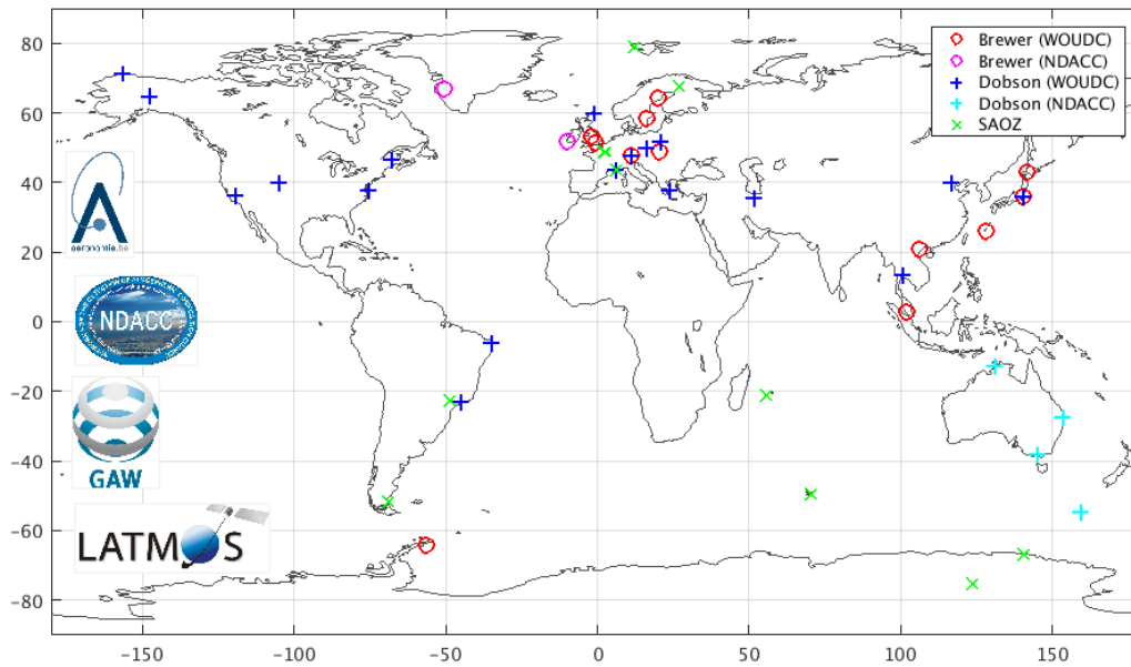
Figure 1: Geographical distribution of Brewer, Dobson and ZSL-DOAS ground-based stations for which suitable co-locations with S5P L2_O3 NRTI ozone data have been identified (May 2018 until November 2020).
