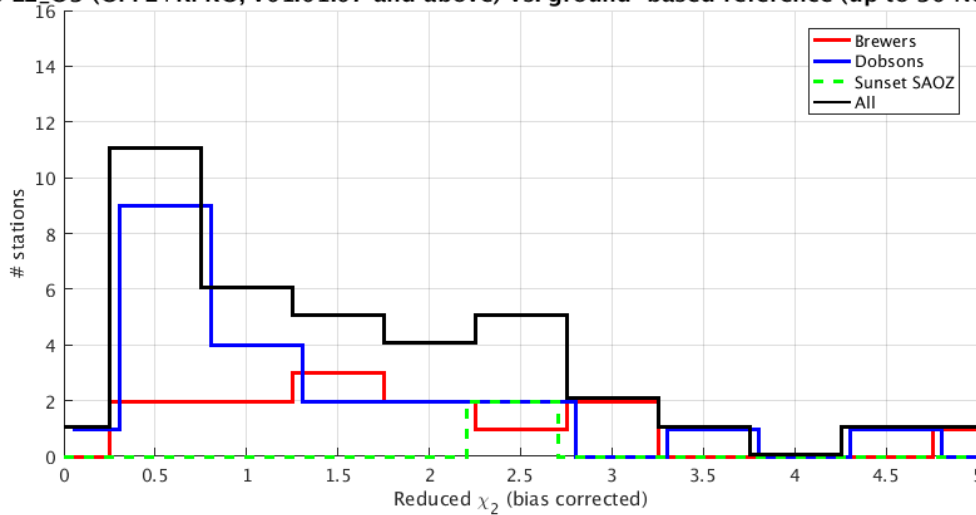
S5p L2_O3 (OFFL+RPRO, v01.01.07 and above) vs. ground-based reference (up to 30 Nov. 2020)
