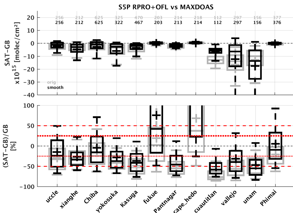
Figure 32: Box-and-whisker plots summarizing the bias and spread of the difference between S5p TROPOMI RPRO+OFFL and MAX-DOAS NO 2 tropospheric columns (grey) and the smoothed MAX-DOAS NO 2 tropospheric columns (black). The median difference is represented by a vertical solid line inside the box, which marks the 25 and 75% quantiles. The whiskers cover the 9-91% range of the differences and the crosses denotes the mean differences. The time frame is from May 2018 until November 2020.
