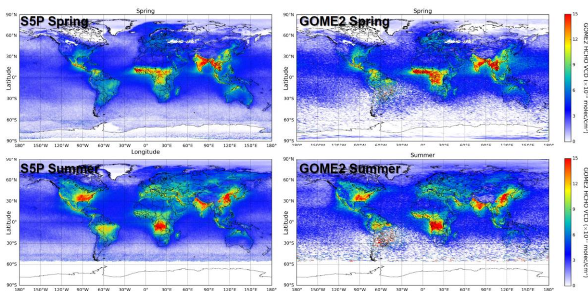
Figure 53: Seasonal average of HCHO vertical column from S5P TROPOMI and MetOp-B GOME 2.
