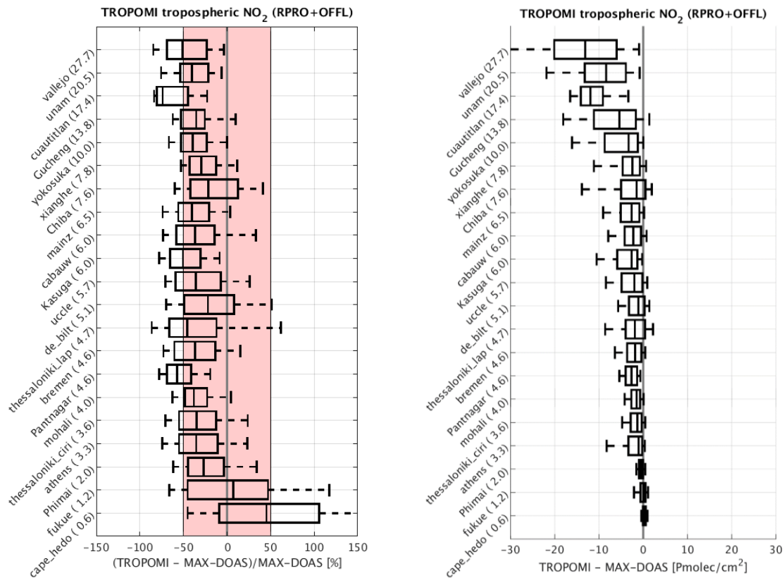
Figure 31: Box-and-whisker plots summarizing the bias and spread of the difference between S5p TROPOMI RPRO+OFFL and MAX-DOAS NO 2 tropospheric columns. The median difference is represented by a vertical solid line inside the box, which marks the 25 and 75% quantiles. The whiskers cover the 9-91% range of the differences. The shaded area represents the mission requirement 50% for the uncertainty. Values between brackets in the labels denote the median tropospheric column at the station. The time frame is from May 2018 until October 2020. This graph includes results for processor versions 1.1.0 and later. Stations are ordered by median tropospheric column.
