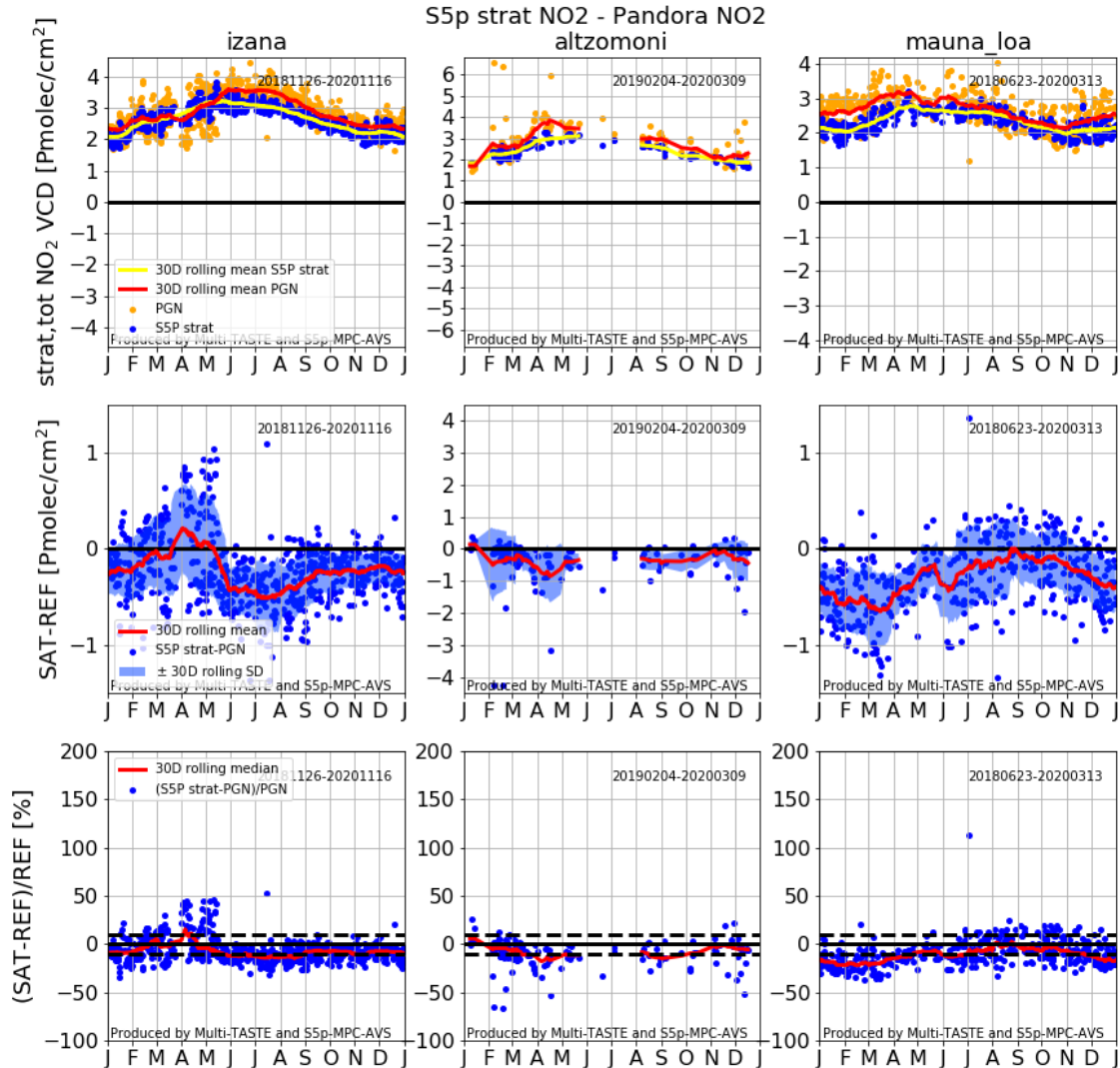
Figure 26: Seasonal cycle plots of the S5P stratospheric NO 2 column and Pandora total column at 3 mountain sites. Upper: S5P and PGN Pandora together; middle: their difference; lower: their percent relative difference. Plain lines represent the 30-day rolling mean or (for relative difference) the 30-day rolling median (cyclic boundary conditions). The data is mapped to one generic year and obtained from validation server on 2020/11/26.
