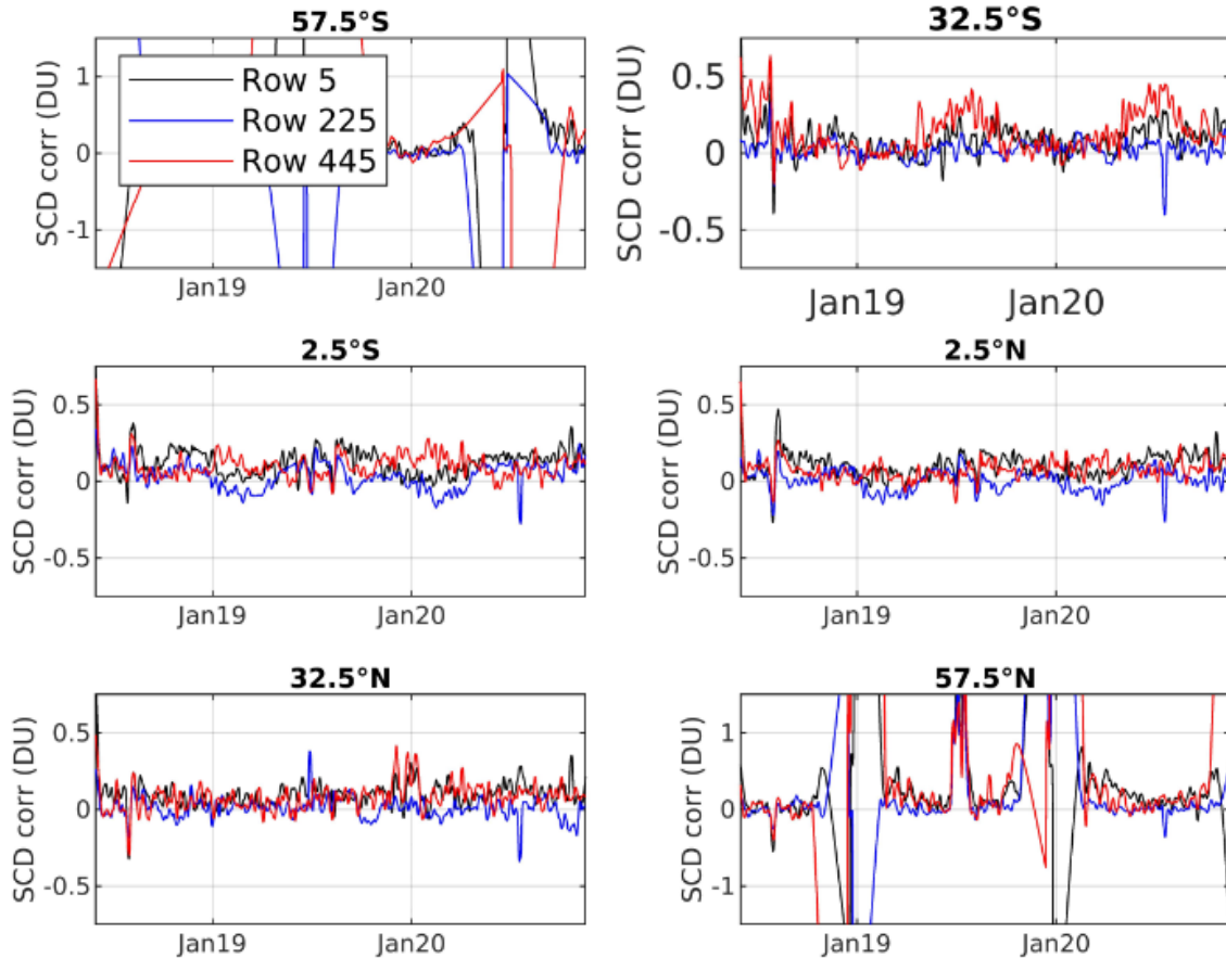
Figure 66: Temporal evolution of the averaged SO 2 SCD for selected 5° latitude bands and 3 detector rows from December 2018 to November 2020. The values are close to zero and show relatively small day to day variations. The larger variations in August 2019 are caused by strong volcanic eruptions. Courtesy of Nicolas Theys (BIRA-IASB).
