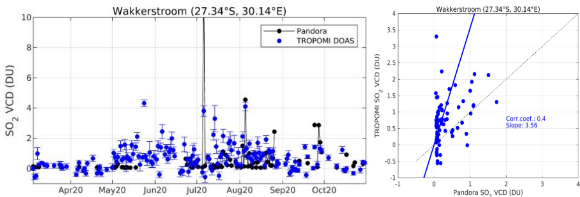
Figure 64: Comparison of TROPOMI SO 2 VCDs to preliminary Pandora measurements (daily means) at Wakkerstroom (South Africa) from March 2020 to November 2020. The following selection criteria were applied: distance < 25km, CF<0.2, time window +/- 1h around overpass. Courtesy of N. Theys (BIRA-IASB), Martin Tiefengraber and Alexander Cede (Luftblick). Pandora data are still in demonstration phase.
