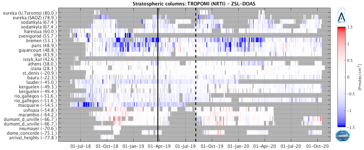
Figure 27: Time series – from August 2018 until October 2020 – of S5P NRTI L2_NO2 and NDACC ZSL-DOAS NO 2 stratospheric column differences [Pmole/cm 2 ]. The black solid and dashed lines indicate, respectively, the processor switch from 1.2.2 to 1.3.0, and the activation of the finer horizontal resolution. Data processed both in NRT mode (LATMOS_RT) and with the LATMOS_v3 processor for stations appearing twice. Both are shown in order to illustrate the consistency.
