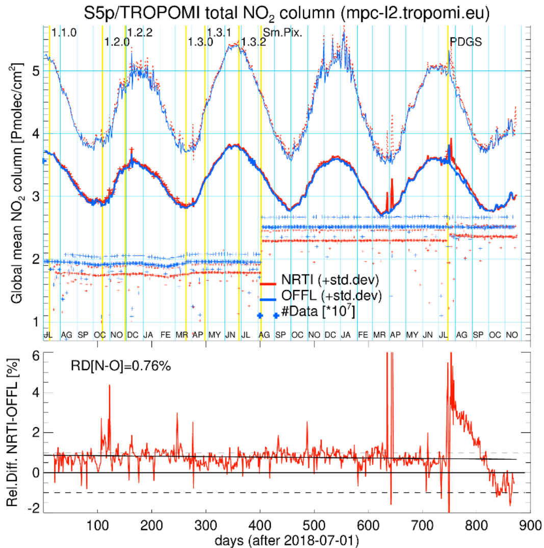
Figure 44: Time series for phase E2 (July 2018 – November 2020) of the global mean of NRTI (red) and OFFL (blue) NO 2 total column data [Pmolec/cm²]. The added 1 \sigma standard deviations are shown as thin lines and the number of NRTI/OFFL data points as crosses with values divided by 10 7 . Superimposed are the points of processor changes, small pixel switch, and latest PDGS switch to 2.7.0 as yellow vertical lines. The lower plot shows the difference [%] between OFFL vs. NRTI daily means. Data is taken from the TROPOMI QC portal.
