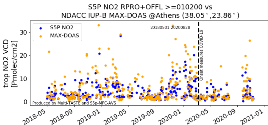
Figure 29: Tropospheric NO 2 column at Athens, as observed by S5P TROPOMI and MAX-DOAS. First nation-wide measures (closures of schools and universities) to contain COVID-19 started on March 10 2020 (dashed line), with further restrictions on later days (source: https://www.bloomberg.com/news/articles/2020-04-17/humbled-greeks-show-the-world-how-to-handle-the-virus-outbreak ). Note how both TROPOMI and MAX-DOAS capture the drop in tropospheric NO 2 and return to normal values in summer.
