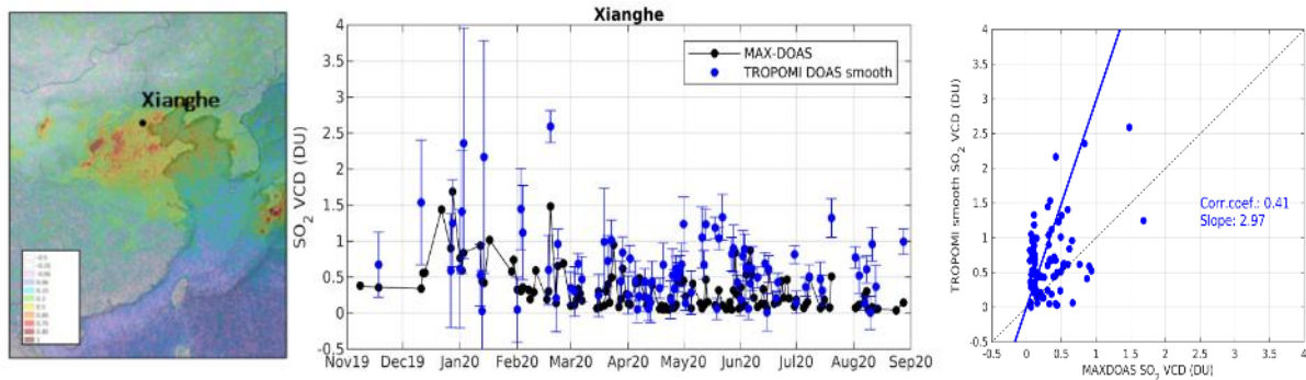
Figure 60: Comparison of TROPOMI SO 2 VCDs to MAX-DOAS measurements (daily means) at Xianghe (China). The following selection criteria were applied: distance < 25km, CF<0.2, AMF>0.2, time window +/- 1h around overpass. Courtesy of N. Theys (BIRA-IASB).
