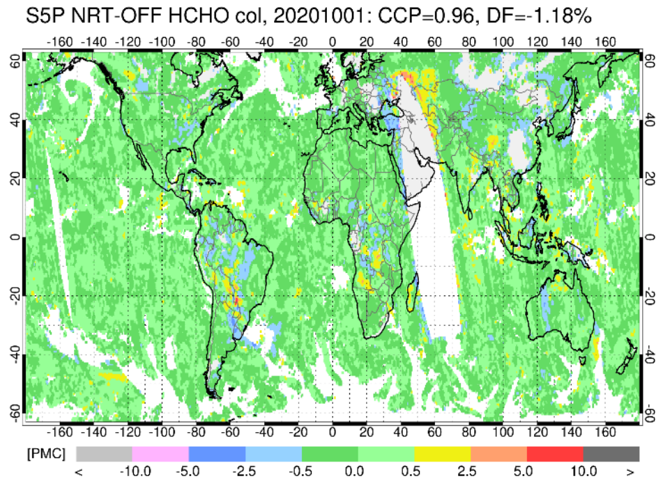
Figure 56: Difference between S5P NRTI and OFFL tropospheric HCHO column data for 2020-10-01 (binned to 0.5°x0.5° resolution). The difference is only calculated for columns above 0.5 Pmolec/cm 2 . Due to the missing NRTI orbit an artefact due to binning is visible.
