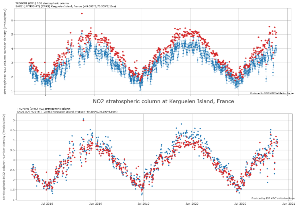
Figure 25: Time series of S5P OFFL L2_NO2 stratospheric NO 2 column data (blue dots) co-located with ground-based SAOZ twilight measurements (red dots) at sunset performed by LATMOS at the NDACC southern mid-latitude station of Kerguelen Island. In the upper plot, the photochemical correction is deactivated to offset the two time series and better see the day-to-day variability. The time frame is July 2018 to November 2020.
