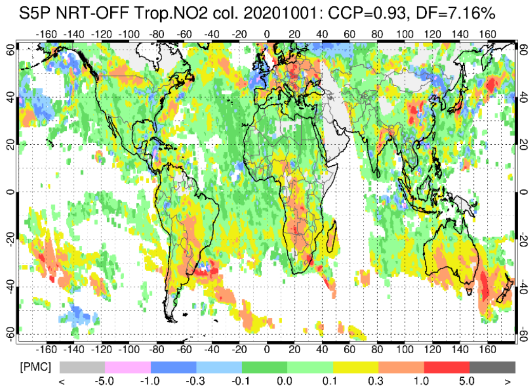
Figure 43: Difference between S5P NRTI and OFFL tropospheric NO 2 column data for one day (gridded to 0.5°x0.5° resolution). The difference is only calculated for columns above 0.5 Pmolec/cm 2 .
