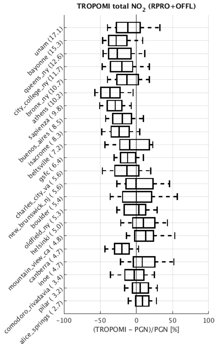
Figure 39: Box-and-whisker plots summarizing the relative bias and spread [%] between S5p TROPOMI RPRO+OFFL (processor version 1.2.2 and later) and PGN Pandora NO 2 total column data. Conventions of the boxplots are identical to Fig. 21. Stations are ordered by median total column. The time frame is May 2018 to October 2020.
