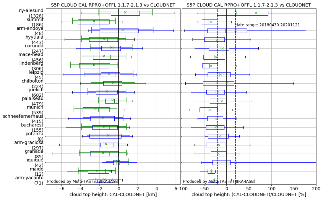
Figure 89: Left panel: Boxplots of S5P L2_CLOUD CAL CTH minus CLOUDNET CTH, per site. Boxplot conventions: box bounds are at first and third quartile. Green line is median. Whiskers are at 5 and 95 percentiles. Slightly offset green cross is mean, with green error bar \pm the standard deviation. Right panel: Similar as upper panel but now for the relative difference, and without indication of the standard deviation. Sensing date range is indicated on the plot.
