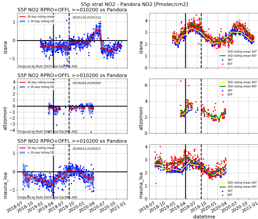
Figure 28: Time series of the difference (left) between S5P RPRO+OFFL L2_NO2 NO 2 stratospheric columns and PGN Pandora total NO 2 columns at 3 mountain sites. The S5P and Pandora time series are on the right. Full vertical line: OFFL processor version change on 2019/03/20. Dashed line: pixel size switch at 2019/08/06. Data covers the period June 2018 until November 2020 and is obtained from the validation server on 2020/11/26.
