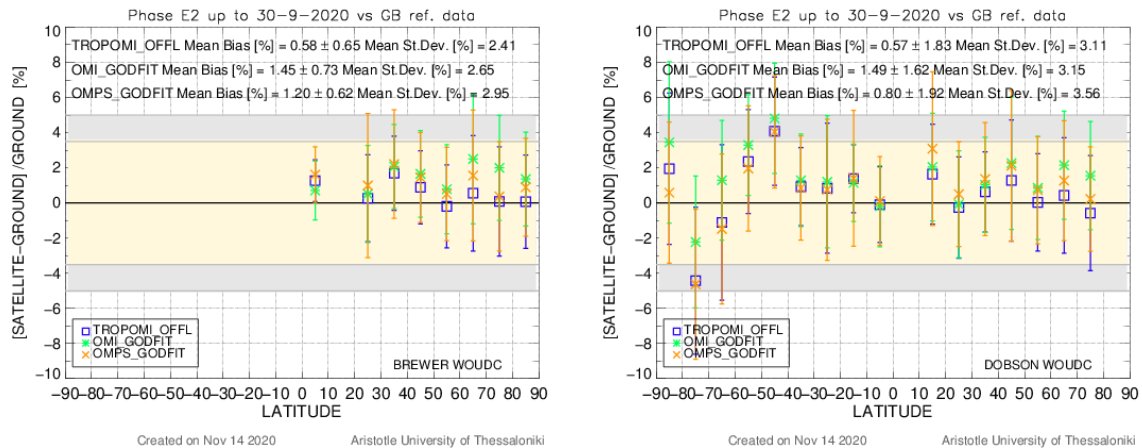
Figure 11: Comparison of the mean percentage differences between three satellite data products (S5P L2_O3 OFFL, OMI GODFIT v4 and OMPS GODFIT v4) and ground-based total ozone data, versus latitude. The Brewer network comparisons are shown in the left-hand panel and the Dobson network comparisons in the right-hand panel. Both datasets are downloaded from the Woudc. The time period of data used for these plots is May 2018 – September 2020.
