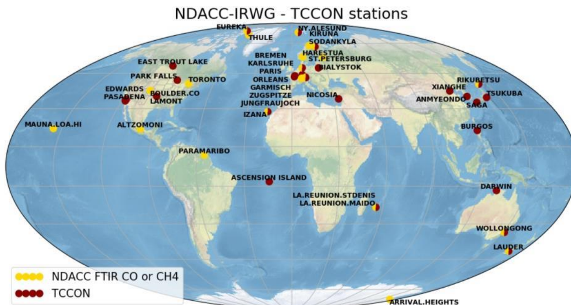
Figure 68: Geographical distribution of NDACC and TCCON FTIR stations measuring atmospheric carbon monoxide column data. Some sites contribute to both networks.
