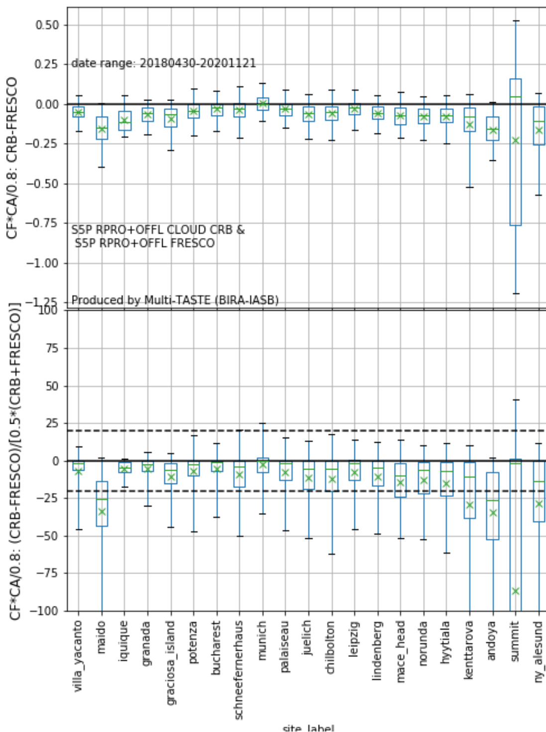
Figure 85. Top. Box plots of S5p CLOUD CRB cloud fraction minus S5p FRESCO cloud fraction, after both have been rescaled to a cloud albedo of 0.8. Bottom: same but for the normed relative difference.
