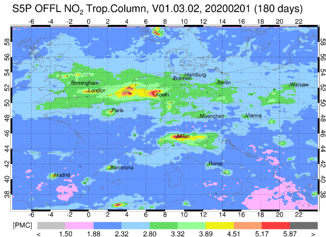
Figure 38: S5P OFFL tropospheric NO 2 over central Europe. The data was binned on a 0.5°x0.5° grid for a 6-month period starting February 2020 using processor versions 01.03.02. A qa\_value > 0.5 and a cloud fraction CF < 0.6 were chosen to reduce the amount of data and exclude cloudy scenes. 1 PMC means 1 Pmole/cm 2 .
