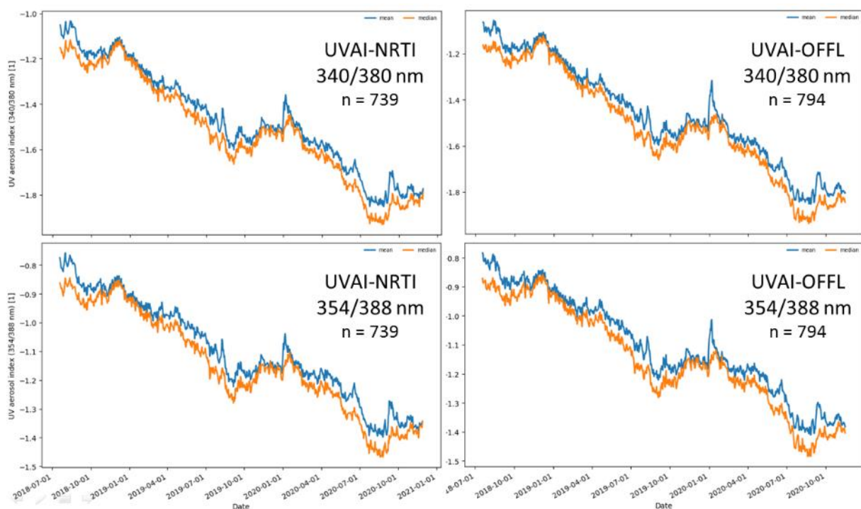
Figure 105: Comparison of the global daily mean (blue) and median (orange) for both L2_AER_AI UVAI wavelength pairs (340/380 and 354/388 nm) and for the NRTI and OFFL data streams, from 20 July 2018 through November 2020.
