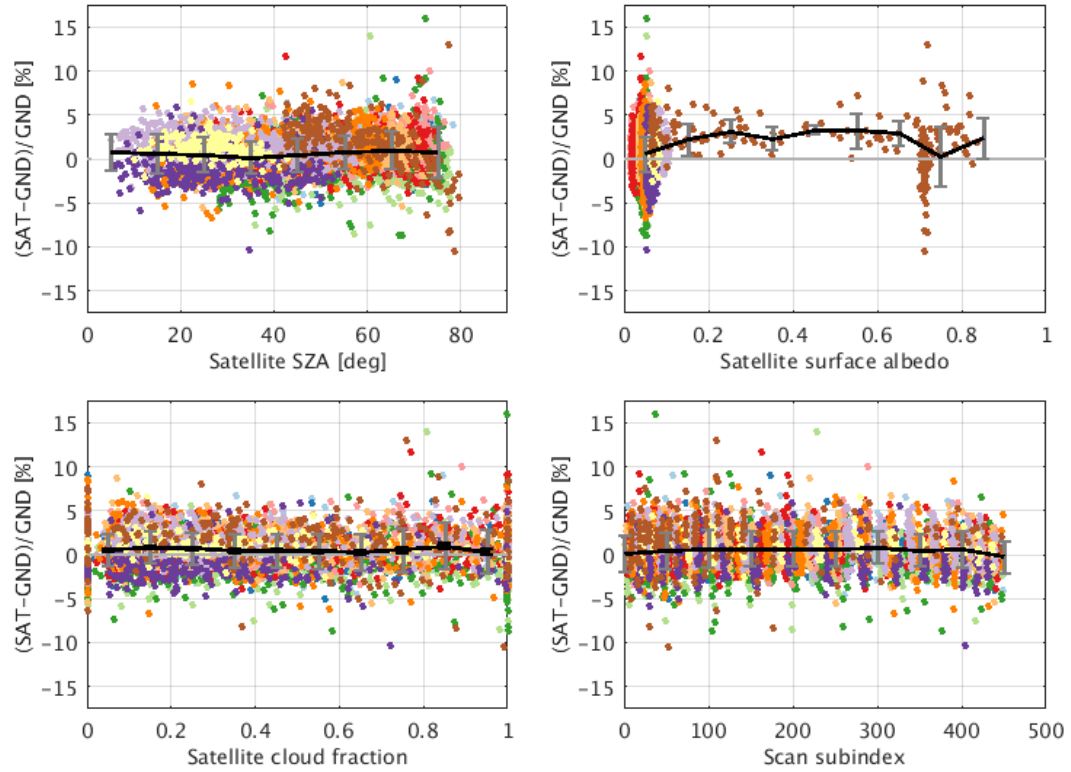
Figure 14: Dependence of the difference between S5P OFFL and ground-based Brewer total ozone data on the solar zenith angle (SZA), the surface albedo, the fractional cloud cover, and the scan sub-index of the satellite measurement. Black curve: mean and standard deviation over bins of 10 degrees of SZA, 0.1 of surface albedo, 0.05 of cloud fraction, and 50 pixels over across-track scan.
