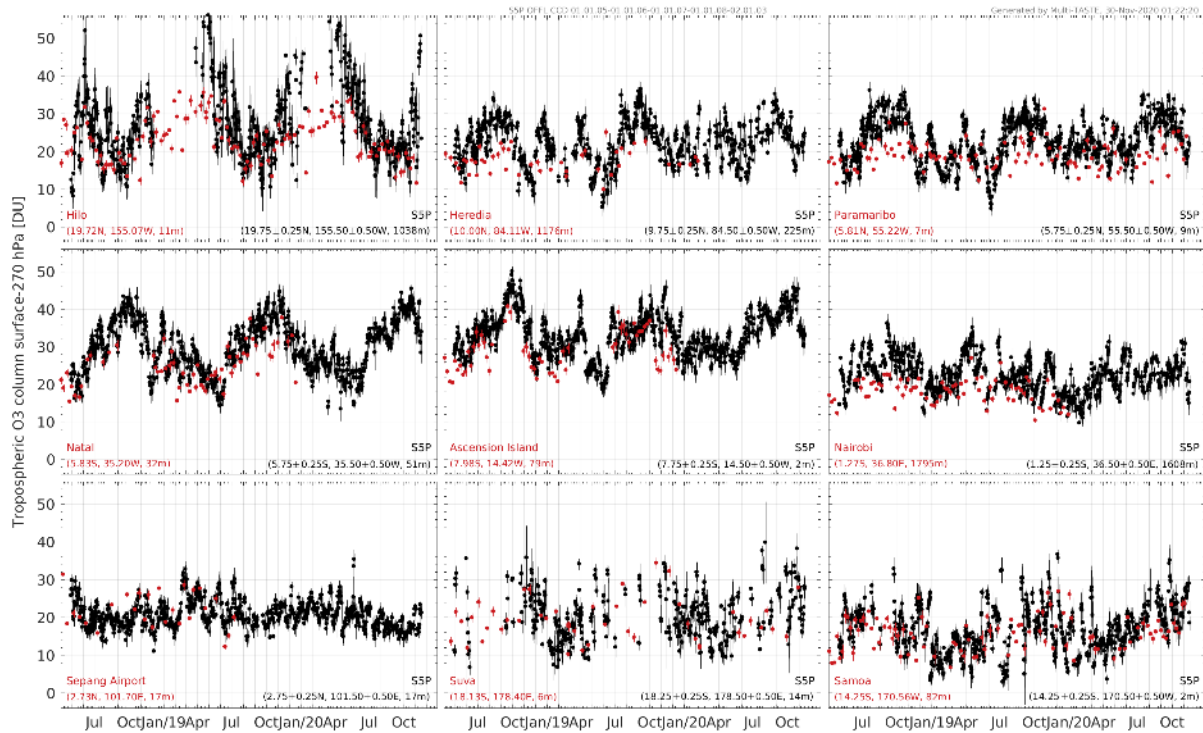
Figure 18: Time series of spatially co-located tropospheric O 3 column data by ozonesonde (red) and by S5P OFFL v01.01.05-v02.01.03 (black). All data were screened following recommendations by the data providers.
