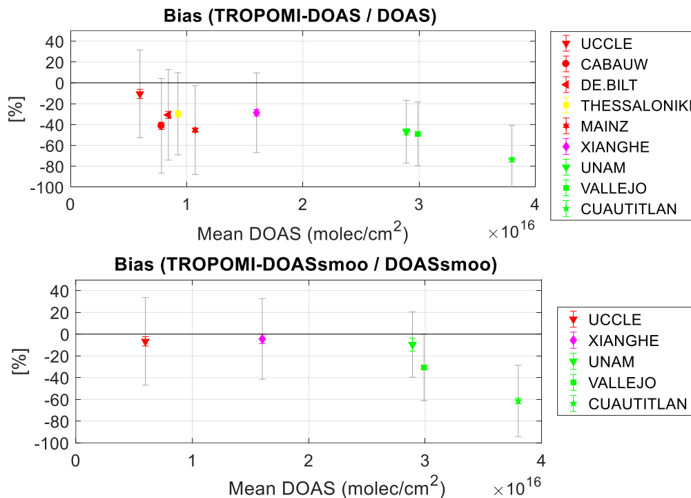
Figure 47: Bias at each station (in %) as a function of the mean DOAS total columns (10 16 molec/cm 2 ). The gray bars are the systematic uncertainty on the differences, and the colored error bars are the 2-σ error on the bias. Top panel: DOAS is the normal product without any modification. Bottom panel: DOAS data after Rodgers and Connor (2003) is applied (a priori substitution and smoothing with the TROPOMI averaging kernels).
