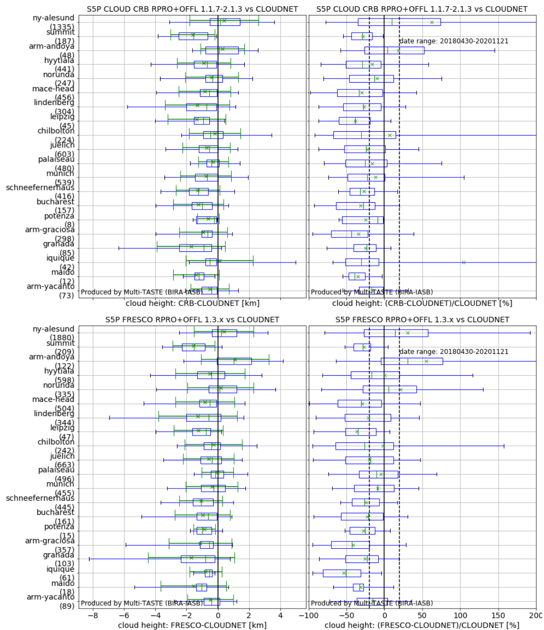
Figure 92: Upper panel: Boxplots of S5P L2_CLOUD CRB RPRO+OFFL 01.01.07-02.01.03 CH minus CLOUDNET CH (upper left) and of the relative difference (upper right), per site. Lower panel: The same but now for the S5P Support product FRESKO RPRO 01.03.02 + OFFL 01.03.00-02. The same conventions as for Figure 89 apply. Sensing time range is indicated on the figure.
