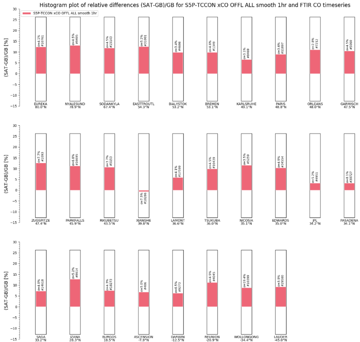
Figure 71: Bar chart of relative mean difference between S5P L2_CO OFFL and FTIR CO column data at 28 TCCON sites for all data within the time range Nov 2017 till October 2020. The sites are sorted with decreasing latitude. The majority of the OFFL biases are below 12% except in the Arctic and mountain station (Izaña and Zugspitze) where the bias is slightly above 12%. Xianghe station lies in a polluted region where we see almost zero bias.
