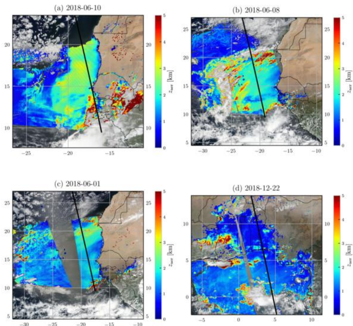
Figure 108: Details of the selected validation cases, showing the ALH on a VIIRS RGB background. The black line represents the Calipso track.
