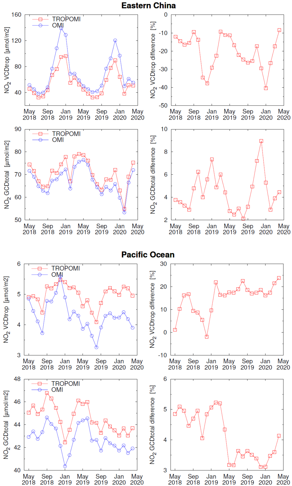
Figure 37: TROPOMI/OMI time evolution for Eastern China [110E,124E][21N,43N] and the Pacific region [170W,130E][60S,60N].
