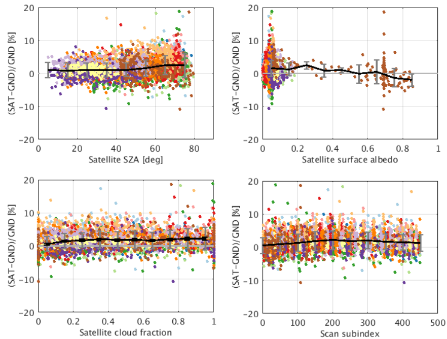
S5p L2_O3 (NRTI, proc.>=1.0.0 and != 1.1.1) vs. Brewer (WOUDC) up to 30 Nov. 2020
