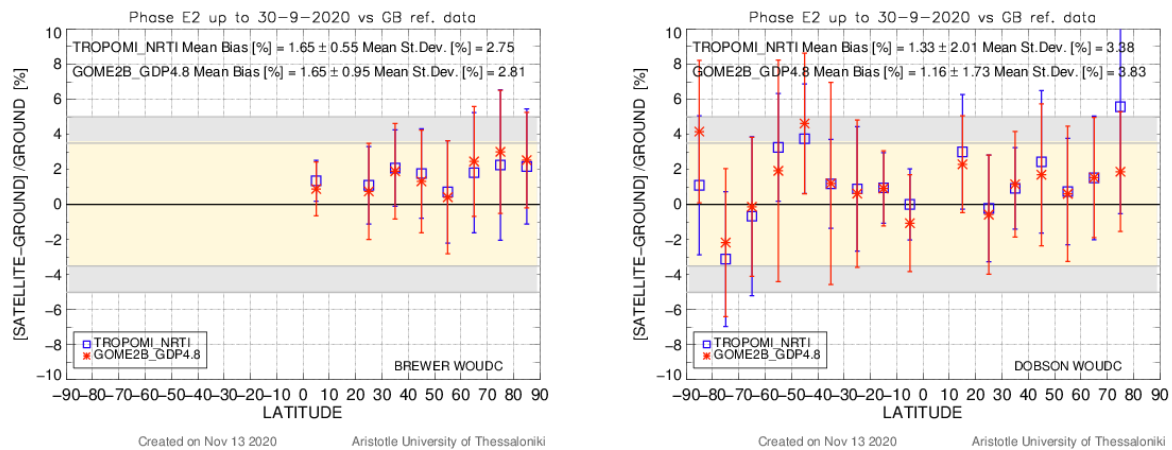
Figure 3: Comparison of the mean percentage differences between two satellite products (S5P TROPOMI L2_O3 NRTI and GOME-2B GDP 4.8) and ground-based total ozone data, versus latitude. The Brewer network comparisons are shown in the left-hand panel and the Dobson network comparisons in the right-hand panel. Both ground-based datasets are downloaded from the Woudc. Time period: is May 2018 – September 2020.
