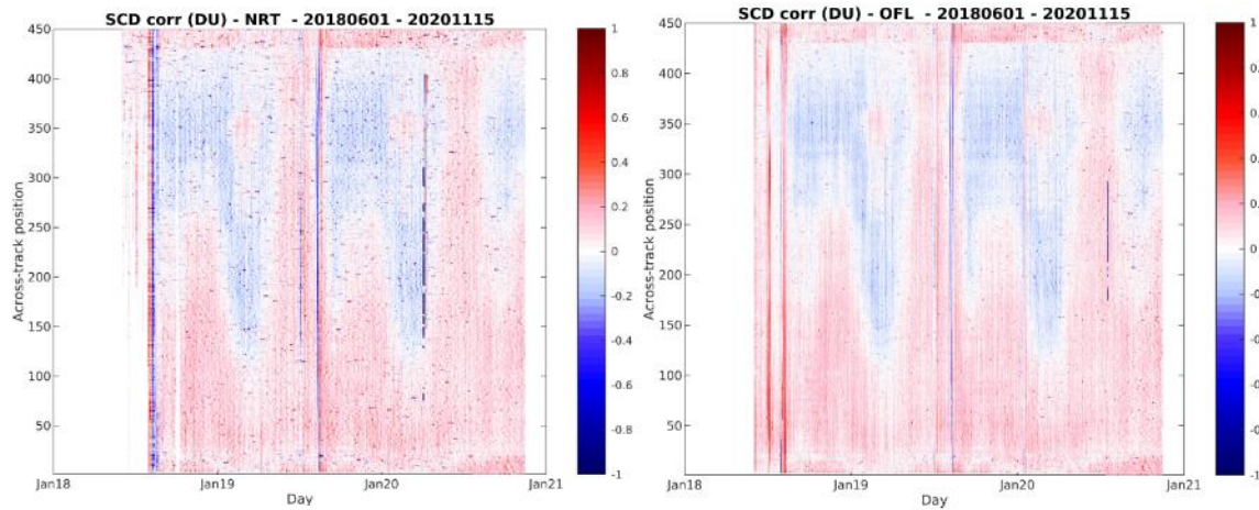
Figure 67: Comparison of the NRT (left) and offline (right) SO 2 data products. Shown are the time series of background corrected SO 2 SCDs for all 450 detector rows from June 2018 to November 2020. Most of the short time features (vertical colored lines) are caused by individual strong volcanic eruptions. For the NRT product, a strong spike occurs in early April 2020, which is caused by a downlink issue that corrupted an irradiance file. The effect of the UPAS processor switch to version 02.01.03 appears but remains modest compared to other features. Courtesy of Nicolas Theys, BIRA-IASB.
