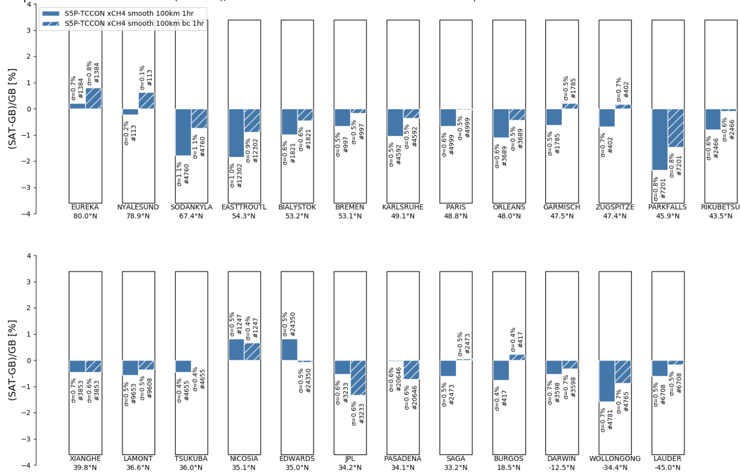
Figure 78: Chart of relative mean difference between S5P L2_CH 4 and FTIR CH 4 column data at 25 TCCON sites within the time range November 2017 till October 2020. The sites are sorted with decreasing latitude. The relative mean difference of the standard xCH 4 product slightly exceeds the mission requirements (bias below 1.5%) only at a few TCCON sites (i.e. Sodankylä, East Trout Lake, Park Falls and Wollongong). However, it never exceeds the mission requirements for the bias corrected product.
