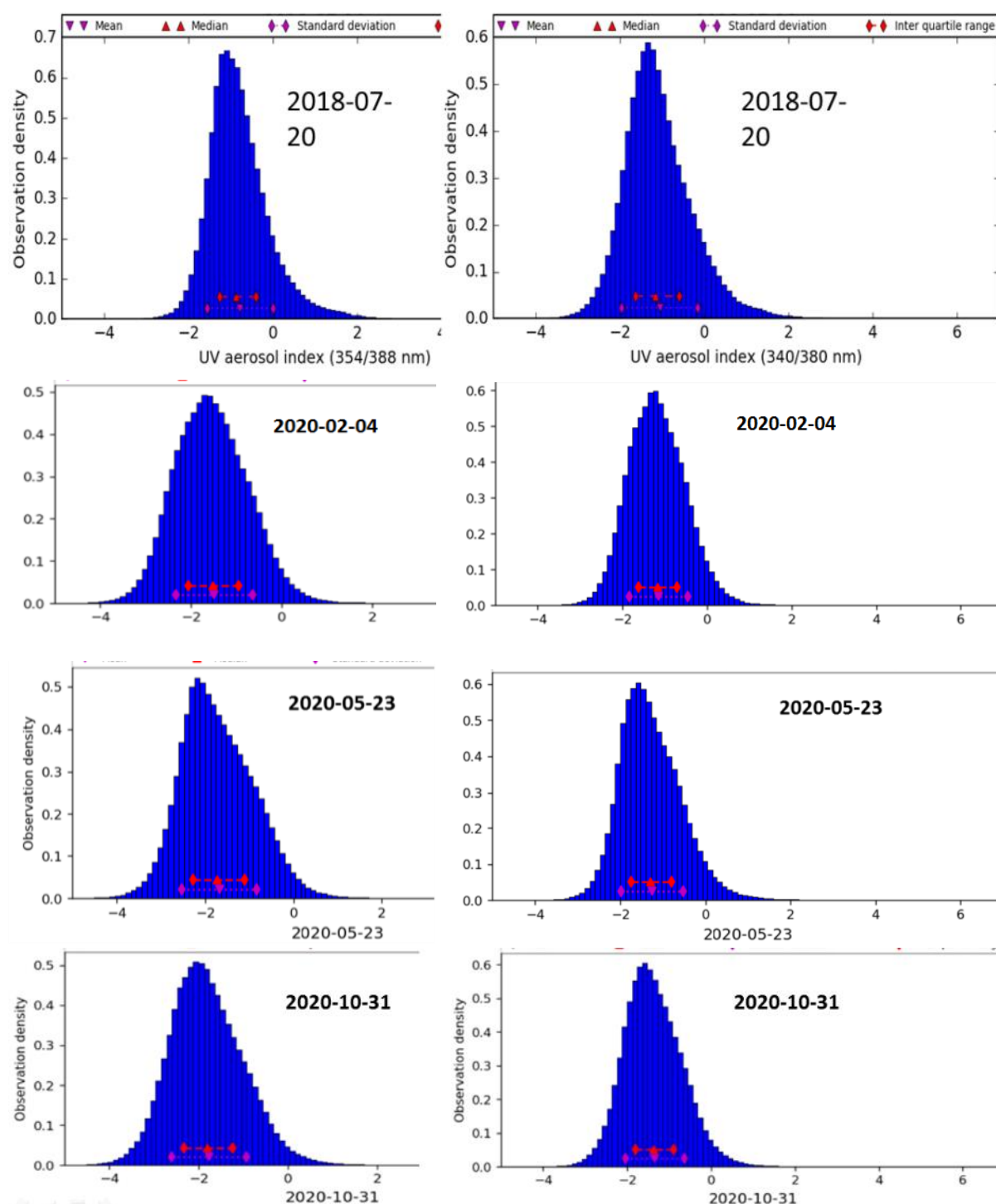
Figure 106: Comparison of the frequency distribution of the UVAI (left: 354/388nm, right: 340/380nm) for four selected days (20 July 2018, 04 February 2020, 23 May 2020, and 31 October 2020).
