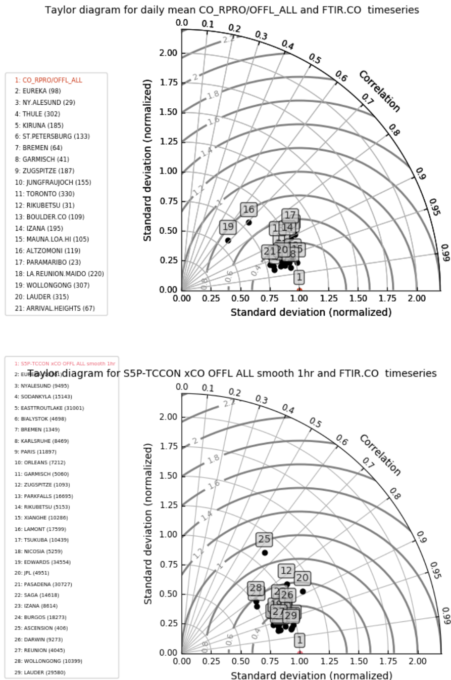
Figure 73: Taylor diagrams for daily mean differences between S5P L2_CO OFFL and ground-based networks CO data: NDACC (top) and TCCON (bottom) for our all case of pixel selection criteria (Boulder and Ascension cover a limited time period), NDACC Wollongong has reduced correlation due to co-location mismatches during the Australian fires in Jan 2020).
