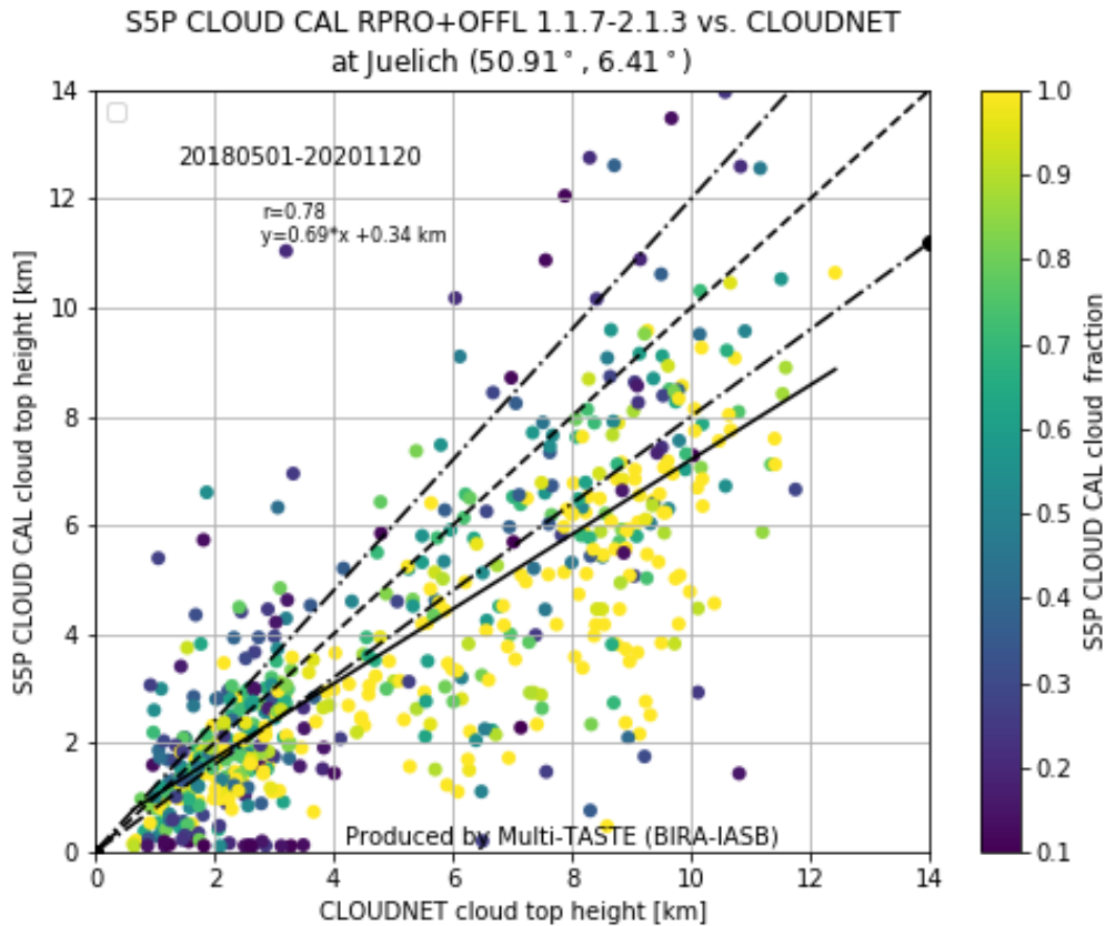
Figure 88: Correlation plot of S5P L2_CLOUD CAL (RPRO+OFFL, processor version 01.01.07-02.01.03) CTH vs. CLOUDNET CTH at Jülich. The colour indicates the S5P L2_CLOUD cloud fraction. Dashed line is the 1:1 line and dash-dotted line the 20% bias requirement.
