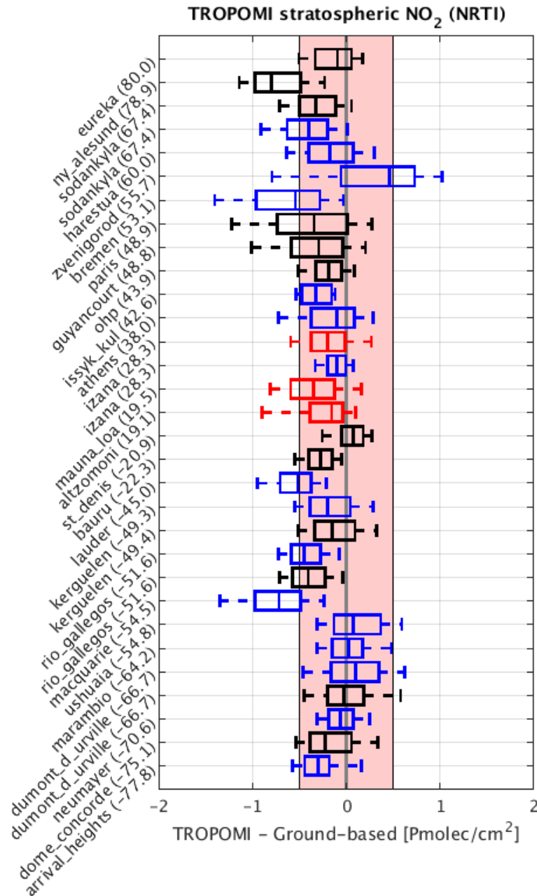
Figure 23: Box-and-whisker plots summarizing the pole to pole bias and spread [Pmolec/cm 2 ] of S5p TROPOMI NRTI and NDACC ZSL-DOAS NO 2 stratospheric columns (SAOZ data in black, other ZSL-DOAS in blue, and mountain-top PGN in red). The median difference is represented by a vertical solid line inside the box, which marks the 25 and 75% quantiles. The whiskers cover the 9-91% range of the differences. The shaded area represents the mission requirement of 0.5 Pmolec/cm 2 for the uncertainty. Station name and latitude of the station are added on the left. The network-wide mean bias and its formal uncertainty are -0.17 and 0.06 Pmolec/cm 2 , respectively. Stations appearing twice have had their data processed both in NRT mode (LATMOS_RT) and with the LATMOS_v3 processor. Both are shown in order to illustrate the consistency. This graph includes results for processor versions 1.1.0 and later. The time frame is May 2018 to October 2020.
