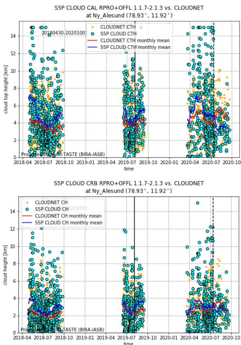
Figure 99: Top. Time series of S5P CLOUD CAL (RPRO and OFFL, processor version 01.01.07-02.01.03) CTH vs. CLOUDNET CTH at Ny-Alesund. The monthly mean of both is also provided. Sensing time range is indicated on the figure. The vertical black solid line indicates the moment of the TROPOMI pixel size switch at 2019/08/06. The vertical black dashed line indicates the version change to UPAS 02.01.03. Bottom. Same but for S5P CLOUD CRB CH vs CLOUDNET CH.
