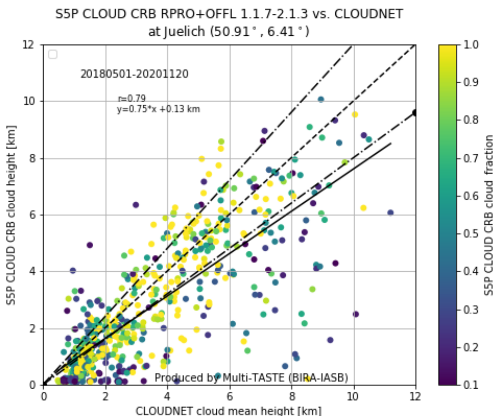
Figure 91: Correlation plot of S5P L2_CLOUD CRB (RPRO and OFFL, processor version 01.01.07-02.01.03) CH vs. CLOUDNET cloud mean height at Jülich. The colour indicates the S5P CLOUD cloud fraction. Dashed line is the 1:1 line and dash-dotted line the 20% bias requirement. Sensing time range is indicated on the figure.
