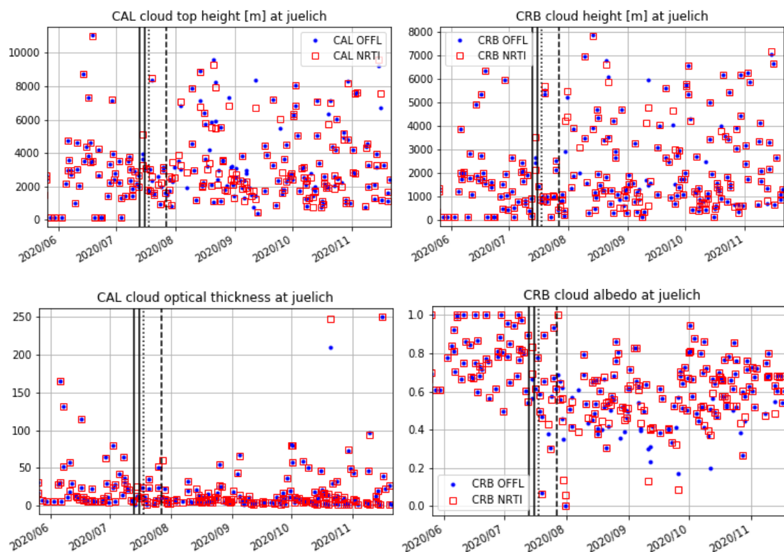
Figure 100: Time series of cloud properties of CLOUD OFFL and CLOUD NRTI at Jülich. Vertical black lines indicate the processor version change from 1.1.7 to 2.1.3; the first one for OFFL (at 2020/07/13), the second one for NRTI (at 2020/07/16).
