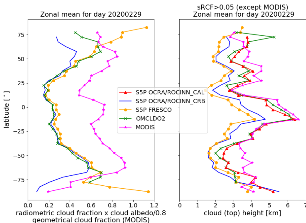
Figure 84. Zonal mean plots (5 deg latitude grid) for 2020-02-29 of radiometric cloud fraction scaled to a cloud albedo of 0.8 of S5P CLOUD CRB, S5P FRESCO and OMI OMCLDO2, and the geometrical cloud fraction of MODIS. Right: cloud (top) height of S5P CLOUD CAL, S5P CLOUD CRB, S5P FRESCO, OMI OMCLDO2 and MODIS. Note that in the right panel, the pixels with scaled radiometric cloud fraction lower than 0.05 are removed (does not apply to MODIS).
