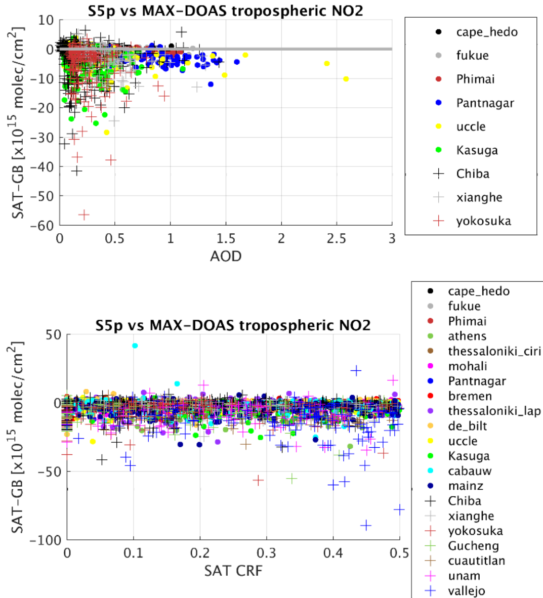
Figure 34: Differences between S5p TROPOMI RPRO+OFFL and MAX-DOAS NO 2 tropospheric columns as a function (upper panel) of MAX-DOAS AOD and (lower panel) S5p cloud radiance fraction (CRF). The time frame is from May 2018 until October 2020.
