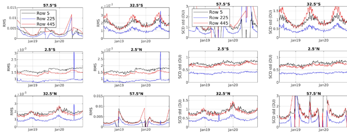
Figure 65: Temporal evolution of the measurement error (left) and the standard deviation (right) for selected 5° latitude bands and 3 detector rows from December 2018 to November 2020. Good qualitative agreement between both quantities is found indicating that the random uncertainty is well characterized by the measurement error. Larger errors (and standard deviations) are found at the edges of the detector and towards high latitudes. The jump in the RMS and standard deviations in low and mid-latitudes in August 2019 are caused by the reduction of the ground pixel size. Courtesy of N. Theys (BIRA-IASB).
