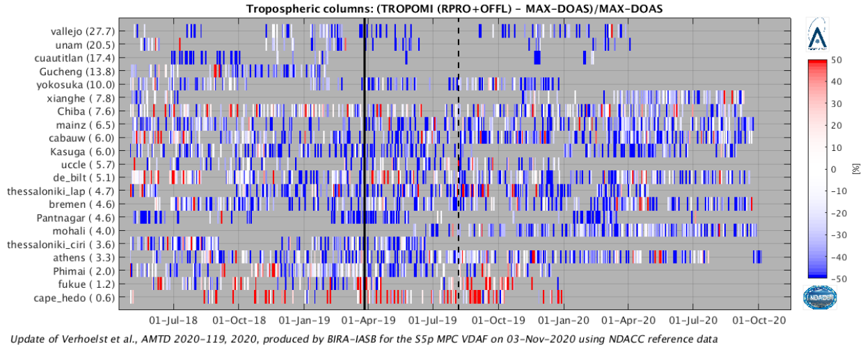
Figure 30: Time series – from May 2018 until October 2020 – of the difference between S5P RPRO+OFFL and MAX-DOAS NO 2 tropospheric column data. The black solid and dashed lines indicate, respectively, the processor switch from 1.2.2 to 1.3.0, and the activation of the finer horizontal resolution. Stations are ordered by median tropospheric column.
