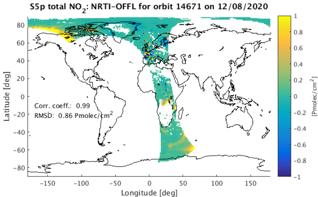
Figure 45: Difference between S5P NRTI and OFFL total NO 2 column data for a single orbit (gridded to 1°x1° resolution).
