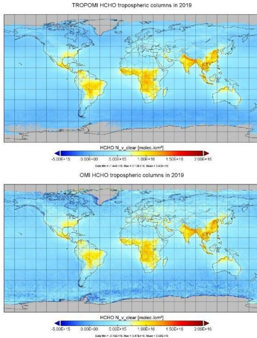
Figure 52: 2019 annual average of S5P TROPOMI (top) and Aura OMI (bottom) HCHO tropospheric column data ( N_{v\_clear} ).
