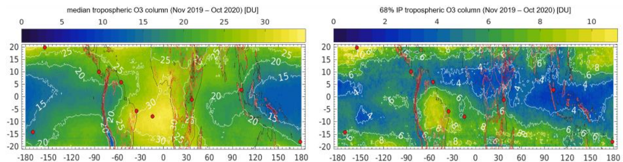
Figure 17: Median value (left) and half-width of 68% interpercentile (right) of S5P OFFL tropospheric ozone column data (CCD) over a full year of operations (November 2019 – October 2020). Red markers locate the nine ground-based ozonesonde stations used in the validation analysis. Red contours indicate surface elevation (500, 1000, 2000 m). These maps provide context to Figure 18 and Figure 19 .
