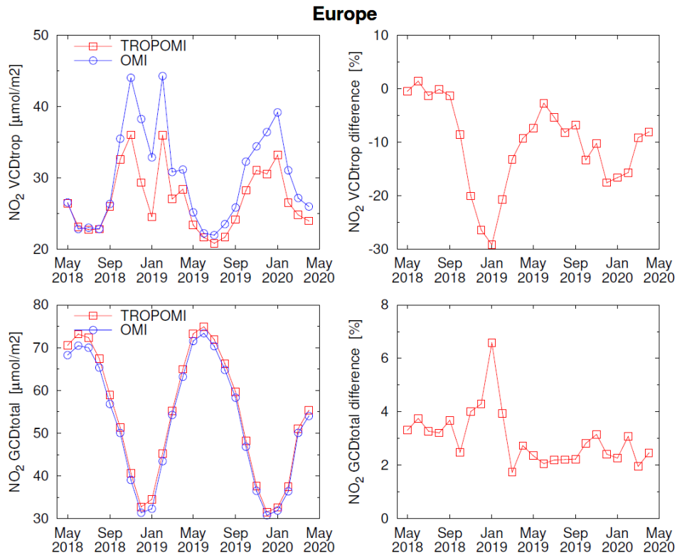
Figure 36: TROPOMI/OMI time evolution for Europe [10W,25E][35N,60N] of the tropospheric NO 2 column (VCDtrop, top rows) and the total geometric column (GCD, bottom rows) in absolute numbers (left columns) and as relative differences. TROPOMI data for pixels with qa_value > 0.75 and OMI/QA4ECV data with cloud radiance fraction < 0.5 (i.e. "clear-sky pixels") have been gridded to a common grid of 0.8°lon x 0.4°lat and averaged over calendar months. The total geometric column is the total slant column divided by the geometric air-mass factor: GCD = SCD / AMF_{geo} . The relative difference is defined as w.r.t. the average between the two.
