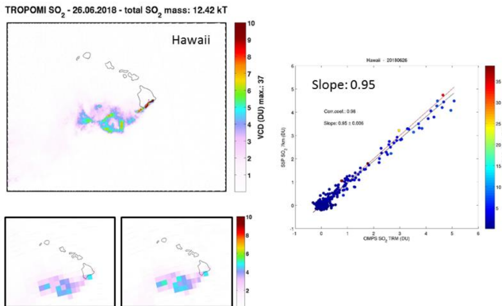
Figure 58: Comparison of TROPOMI and OMPS measurements of the volcanic plume of Kilauea on 26 June 2018. The large figure shows the original TROPOMI data. The two small figures show the spatially degraded TROPOMI data and the OMPS data. The figure right shows the correlation plot of the degraded TROPOMI data versus the collocated OMPS data. Courtesy of C. Li and N. Krotkov, NASA/GSFC.
