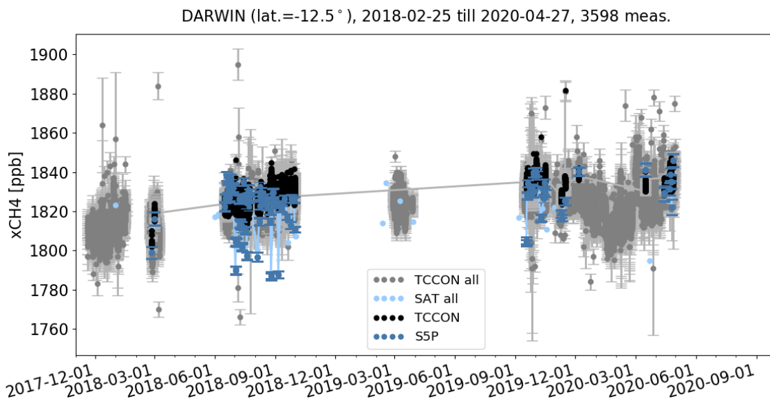
Figure 83: S5P L2_CH4 XCH 4 time series over Darwin where low values of XCH 4 are observed for several days.
