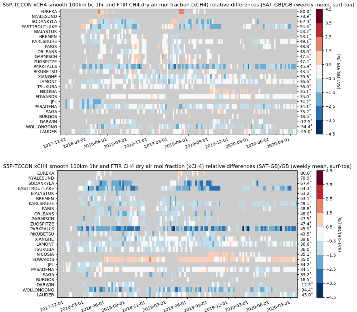
Figure 77: Mosaic plots of relative biases between S5P L2_CH4 RPRO+OFFL and ground-based CH4 TCCON column data for the bias corrected (top) and standard (bottom) methane products. Over the November 2017 – October 2020 time period the plots do not show a clear meridian dependence or temporal change in the weekly averaged biases.
