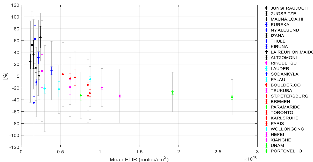
Figure 46: Bias at each station (in %) as a function of the mean FTIR total columns (molec/cm 2 ). The gray bars are the systematic uncertainty on the differences, and the colored error bars are the 2- \sigma error on the bias. Updated from Fig. 3 of Vigouroux et al., 2020; temporal range here is May 2018 to May 2020.
