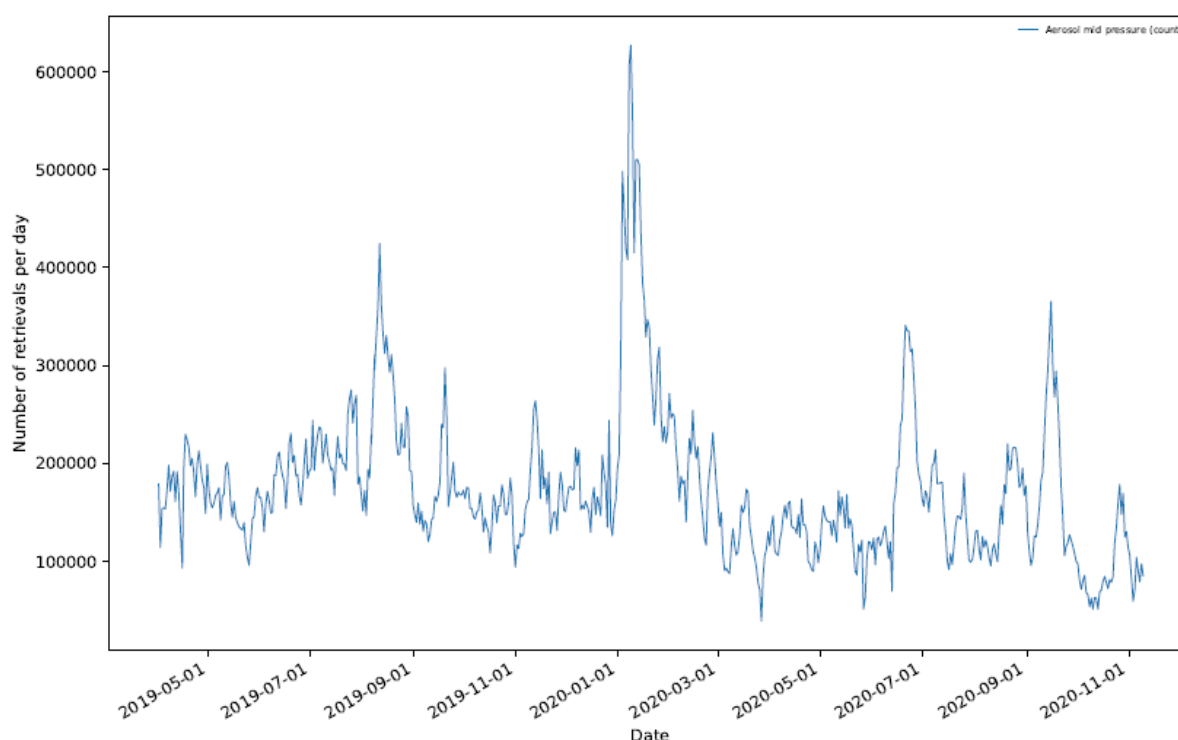
Figure 114: Number of successfully processed ALH pixels per day from April 2019 to November 2020.
