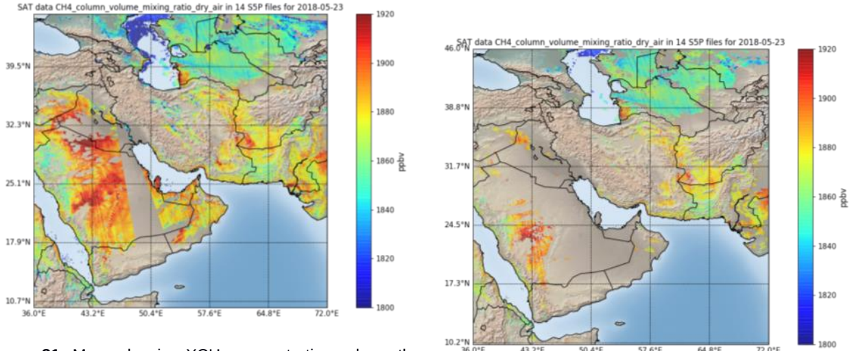
Figure 81: Maps showing XCH 4 concentrations above the Middle East measured by S5P on May 23 2018. The left panel shows all available ground pixels, the right panel shows only pixels with qa_value>0.5. The left panel shows the presence of stripes in the flight direction and the right panel shows the presence of filtered pixels above inland water (Caspian Sea).
