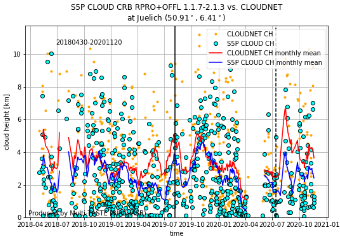
Figure 90: Time series of S5P L2_CLOUD CRB (RPRO and OFFL, processor version 01.01.07-02.01.03) CH vs. CLOUDNET CH at Jülich. The monthly mean of both is also provided. The moment of the switch in TROPOMI pixel size (along track reduction from 7 to 5.5 km) is identified by the bold vertical line, the UPAS processor upgrade to 02.01.03 by the dashed line. Sensing time range is indicated on the figure.
