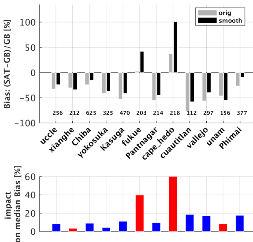
Figure 33: (upper panel) Bar plots summarizing the median bias of the difference between S5p TROPOMI RPRO+OFFL and MAX-DOAS NO 2 tropospheric columns (grey) and the smoothed MAX-DOAS NO 2 tropospheric columns (black). (lower panel) Bar plot summarizing the change on the median bias between the original comparisons and the smoothed ones. Absolute values of the relative median biases are shown, where reductions are marked in blue bars and increases in red bars. The time frame is from May 2018 until October 2020.
