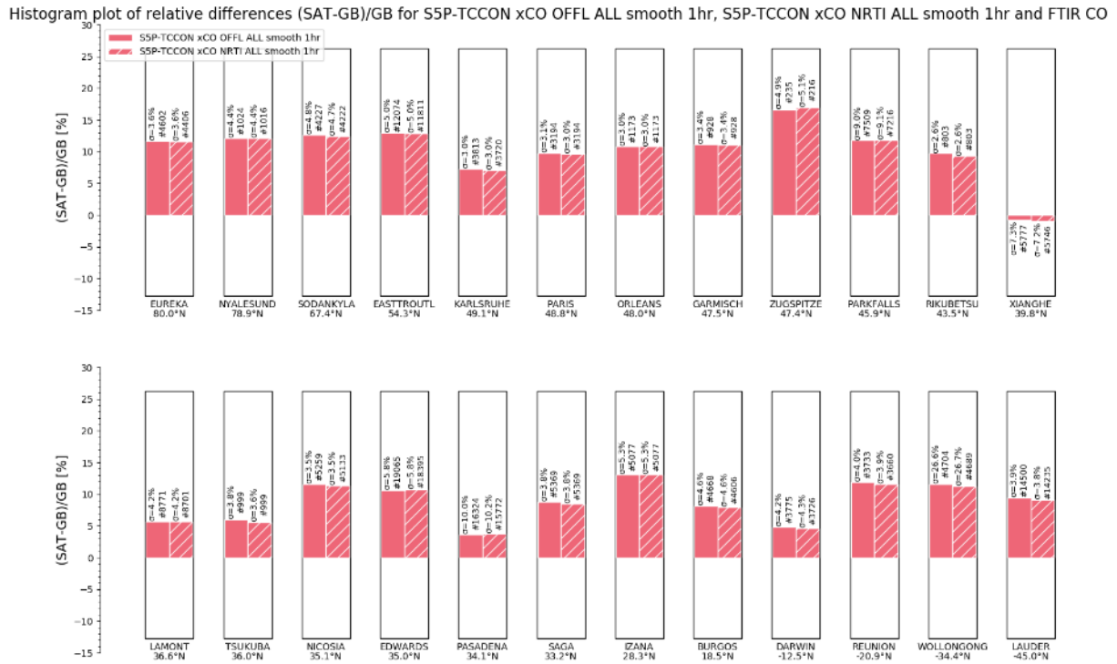
Figure 76: Comparison of relative biases against TCCON CO column data for the S5P L2_CO OFFL and NRTI data versions, from July 3 2019 through October 2020. The quality of both data sets is similar. Over this period the OFFL processor has produced data with a relative mean bias of 9.63\% \pm 5.56\% and a correlation coefficient 0.94 with respect to TCCON data; the NRTI processor has produced data with a relative mean bias 9.49\% \pm 5.58\% and a correlation 0.93.
