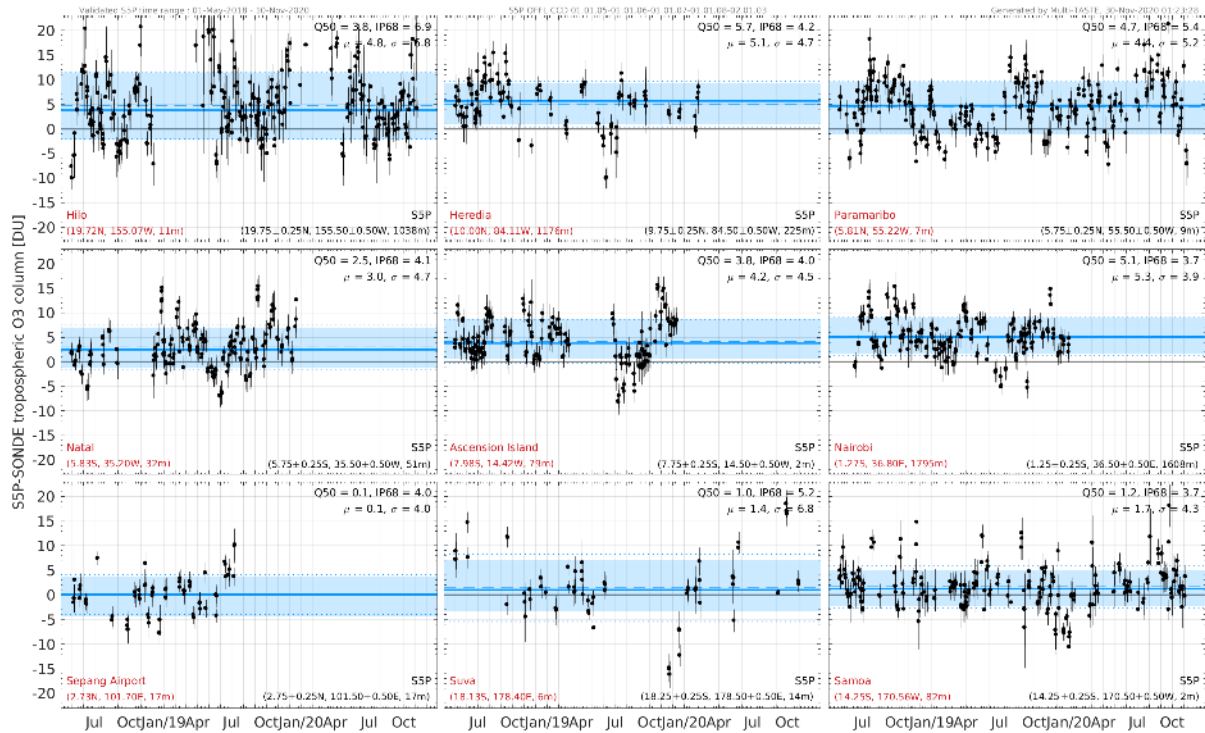
Figure 19: Time series of the absolute difference between spatially and temporally co-located S5P and ozonesonde tropospheric O 3 column data. The blue line and shaded area shows the median value and the range between the 16% and 84% percentiles. Positive values indicate a high bias of S5P w.r.t. the reference.
