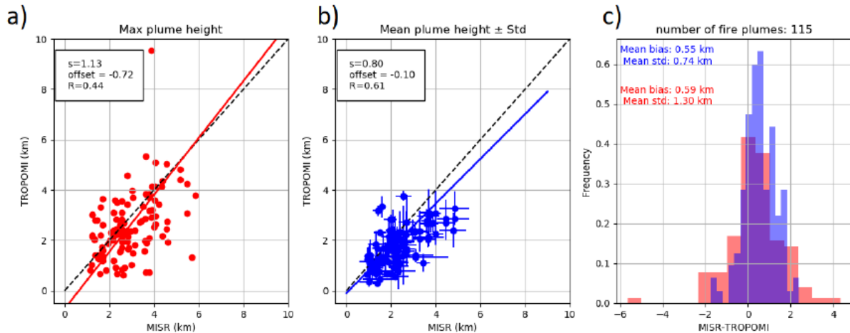
Figure 112: Comparison of TROPOMI ALH and MISR plume height for 115 fires over Northern America in 2018. See Griffin et al, 2019 for details.
