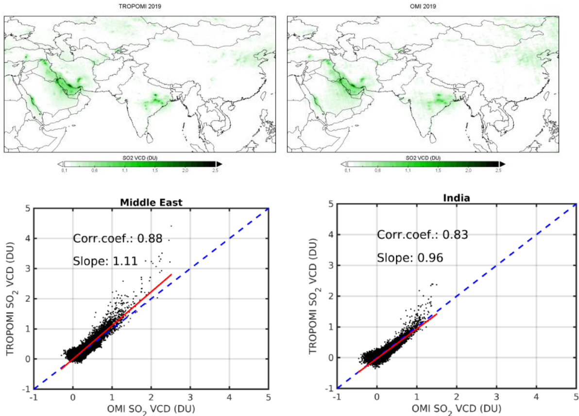
Figure 57: Top: Comparison of the average distribution (01 Jan 2019 – 31 Dec 2019) of the SO 2 VCDs derived from TROPOMI and OMI over regions with strong air pollution. Both data sets show very good agreement. Bottom: Correlation plots TROPOMI versus OMI over the Middle East and India. Note that a fixed AMF of 0.4 was used for both retrievals to exclude the effect of different profile assumptions. Courtesy of Nicolas Theys, BIRA-IASB.
