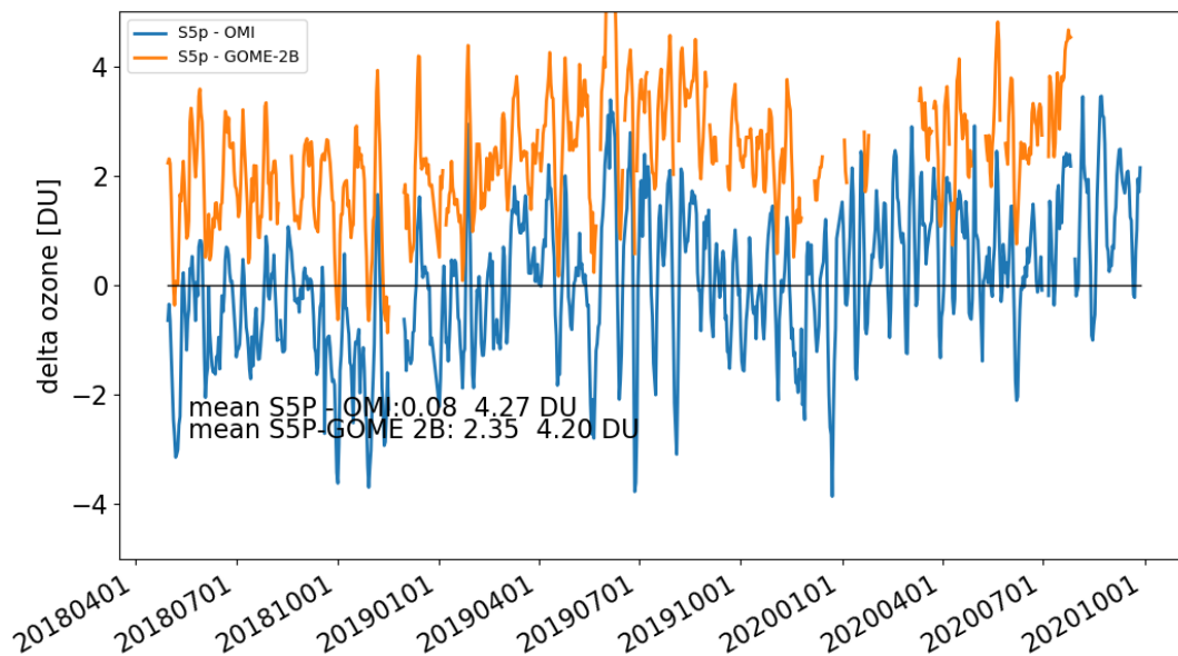
Figure 20: Difference time series of daily tropospheric O 3 column data averaged over the 20°S – 20°N tropical belt. S5P OFFL CCD data are compared to satellite data by OMI and GOME-2B, positive values indicate a high bias of S5P w.r.t. the reference.
