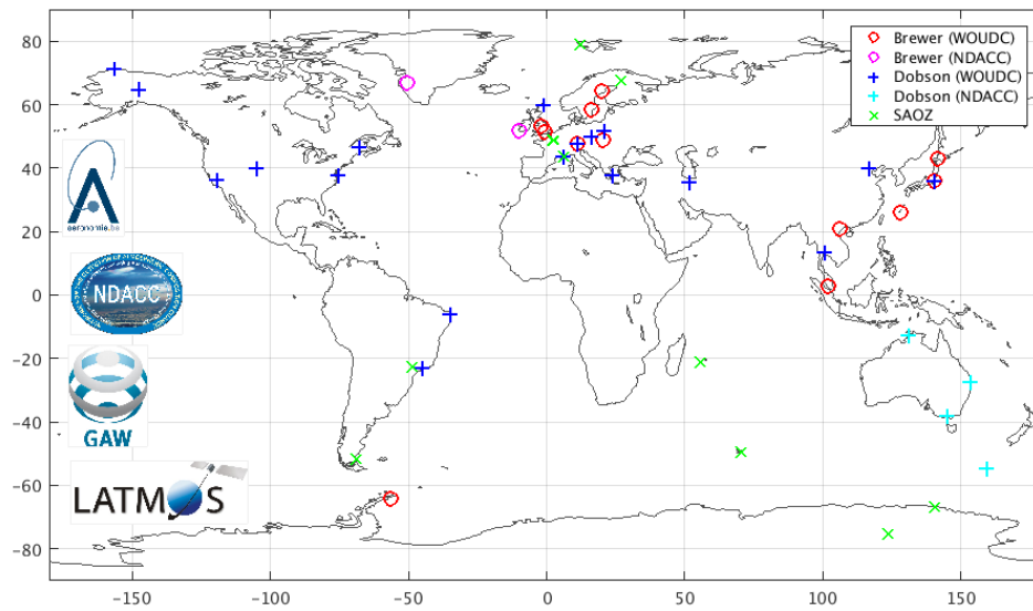
Figure 9: Geographical distribution of Brewer, Dobson and ZSL-DOAS ground-based stations for which suitable co-locations with S5P L2_O3 OFFL ozone data have been identified (period up to November 2020).
