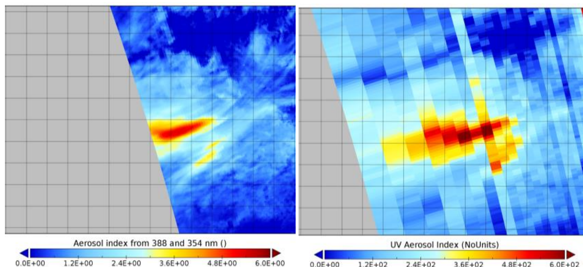
Figure 101: Comparison of S5P TROPOMI UVAI (orbit 00398, left) and OMI OMAERO UV Aerosol Index (orbit 70864, right) for Saharan dust on 10 November 2017. In general very good agreement is found (the stripes in north-south direction in the OMI data are caused by the OMI row anomaly and should be ignored).
